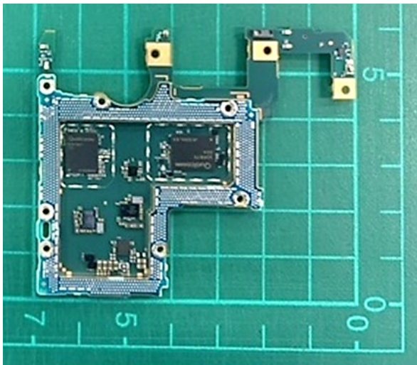
Rear PBA without Shield case (Rear-side)
