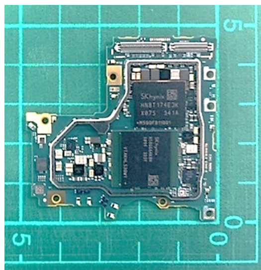
Front PBA without Shield cases (Front-side)
