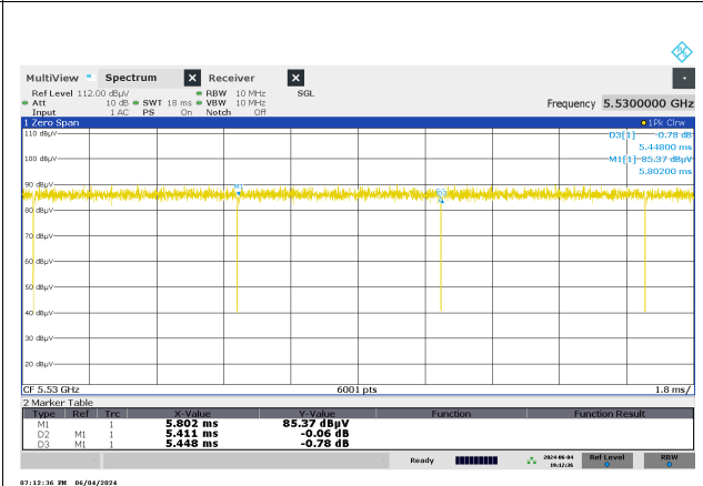
802.11be EHT80, OFDMA, 484T+242T (C), 2Tx
