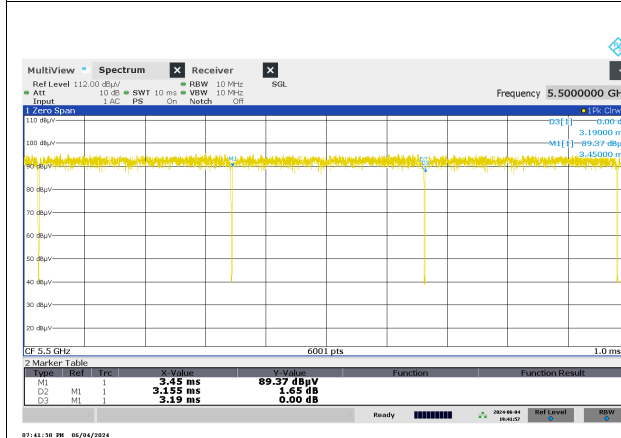
802.11be EHT20, OFDMA, 106T+26T, 2Tx
