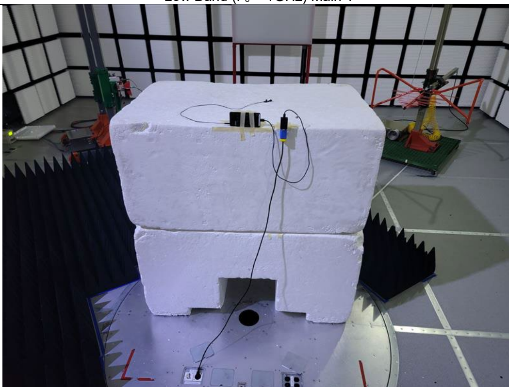
A1G Setup Back Low Band ( F_c < 1\text{GHz} ) Main 1
