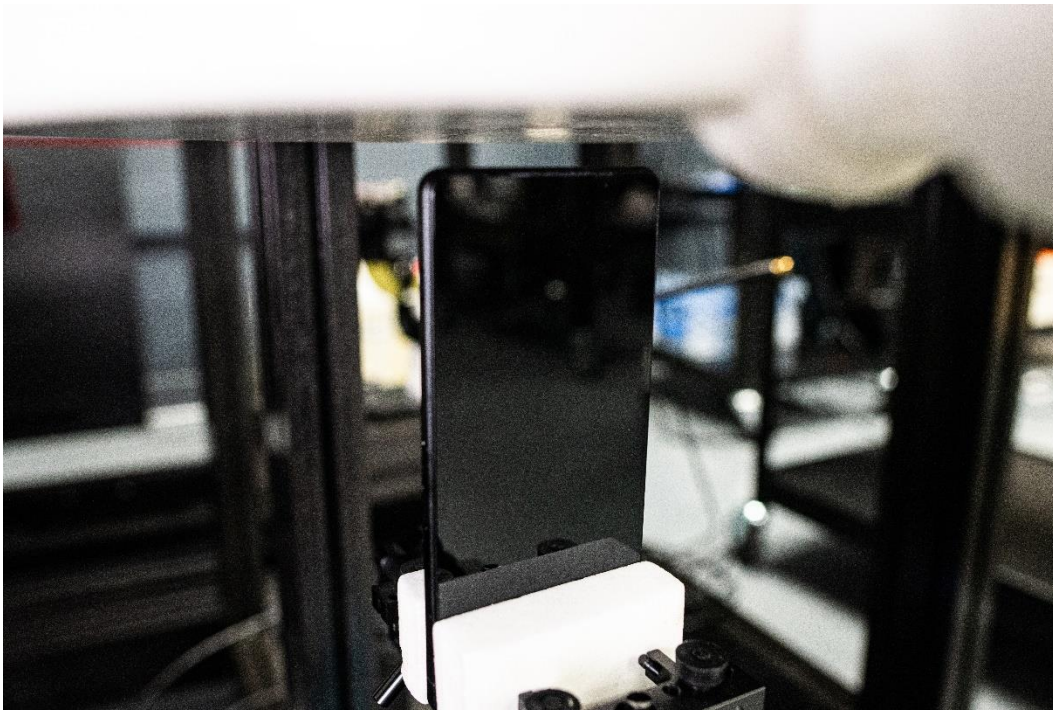
Figure L SAR Test Setup – Hotspot – Bottom 10mm
