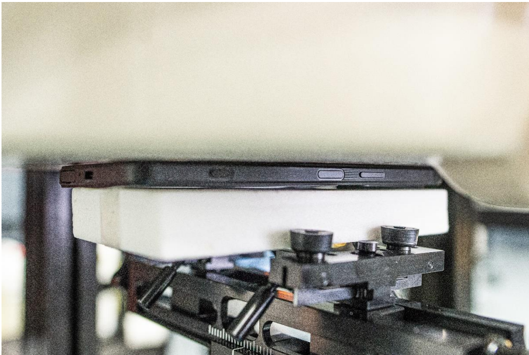
Figure I SAR Test Setup – Phablet – Front 0mm
