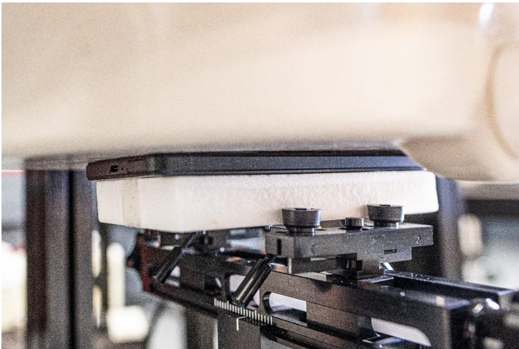
Figure G SAR Test Setup – Phablet – Back 0mm
