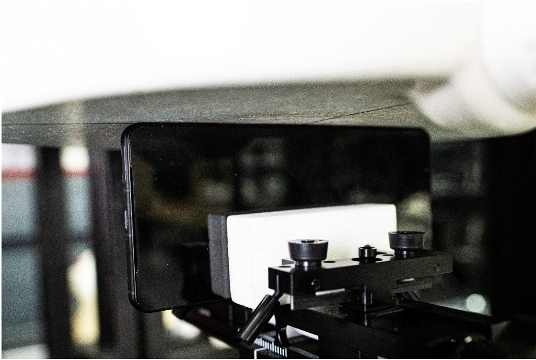
Figure P SAR Test Setup – Phablet – Left 0mm
