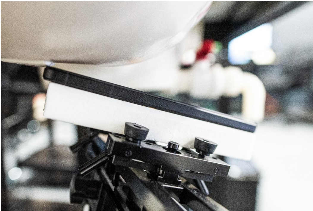
Figure C SAR Test Setup – Head – Right Tilt 0mm
