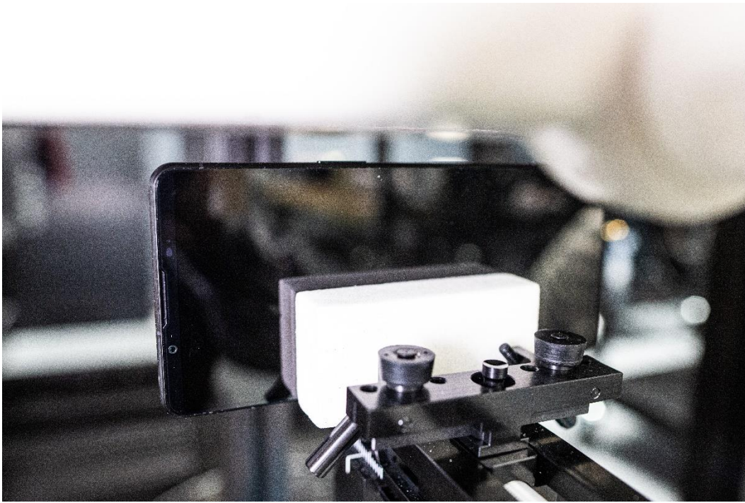
Figure N SAR Test Setup – Hotspot – Right 10mm
