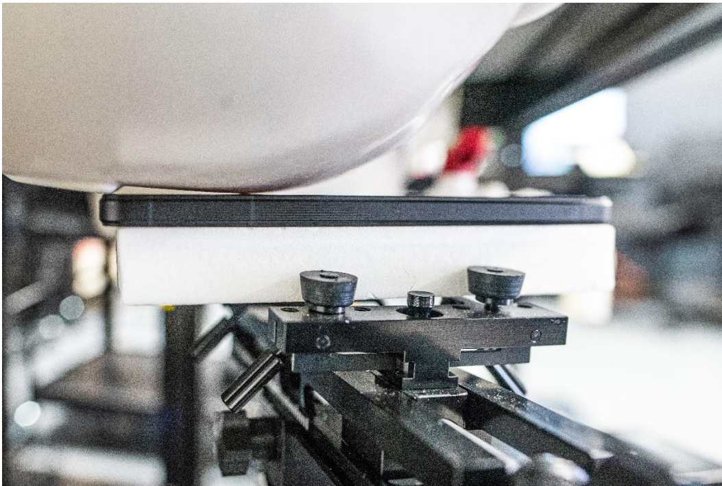
Figure B SAR Test Setup – Head – Right Cheek 0mm
