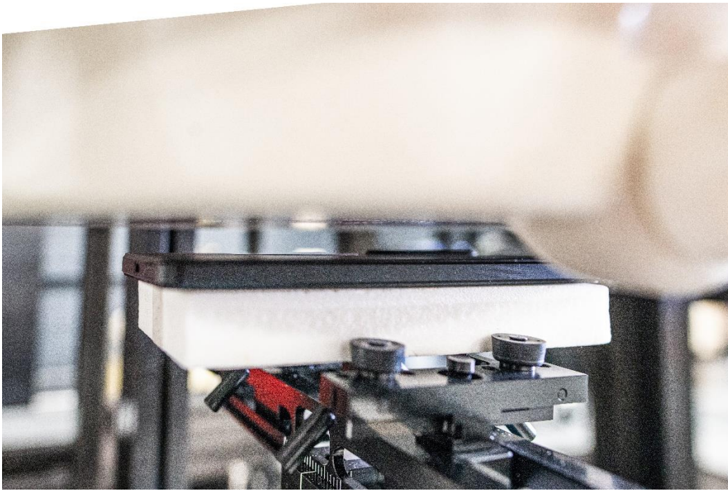
Figure F SAR Test Setup – Body-worn / Hotspot – Back 10mm
