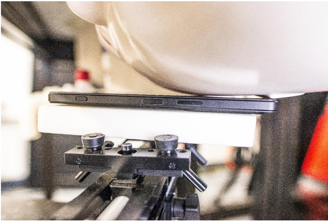
Figure D SAR Test Setup – Head – Left Cheek 0mm
