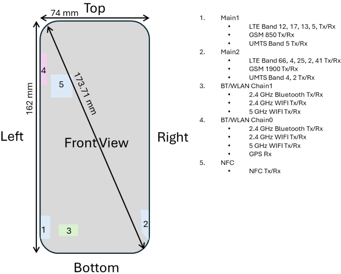
Figure A SAR Test Setup – Antenna Diagram
