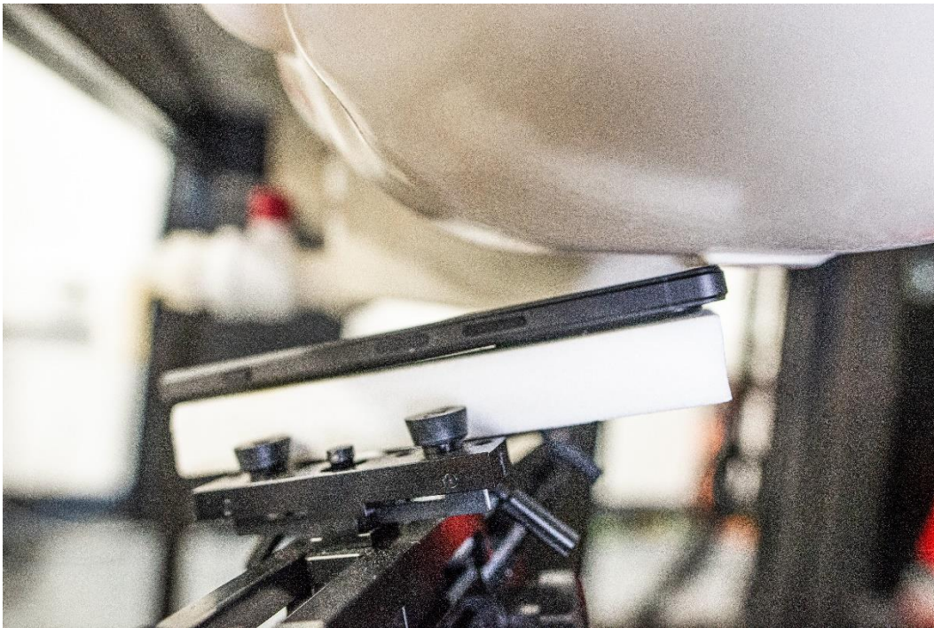
Figure E SAR Test Setup – Head – Left Tilt 0mm
