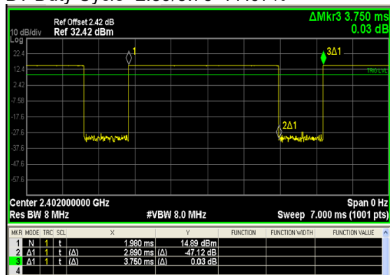
BT Duty Cycle=2.89/3.75=77.07%
