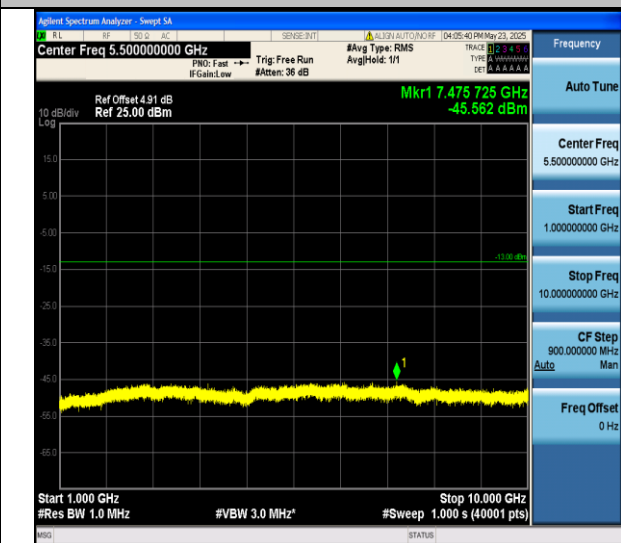
Band V-4233-1000~10000MHz-PASS
