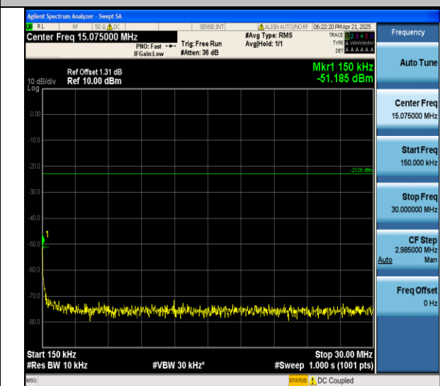
Band V-4233-0.15~30MHz-PASS
