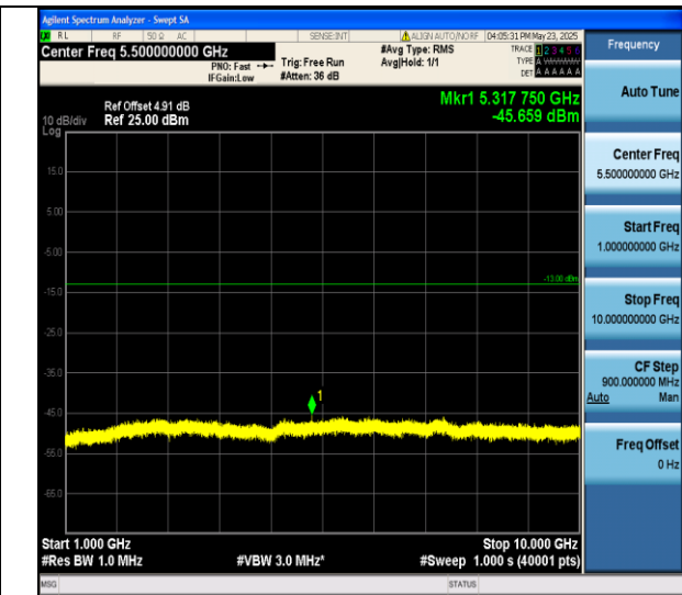
Band V-4182-1000~10000MHz-PASS
