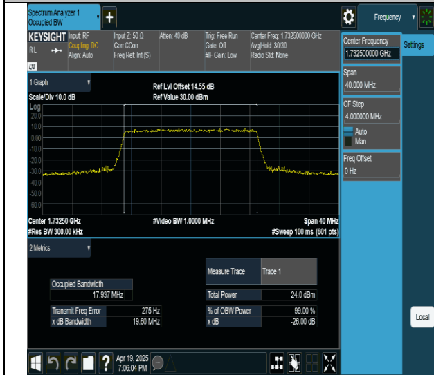
Band4-20MHz-QPSK-20175-100RB#0-PASS
