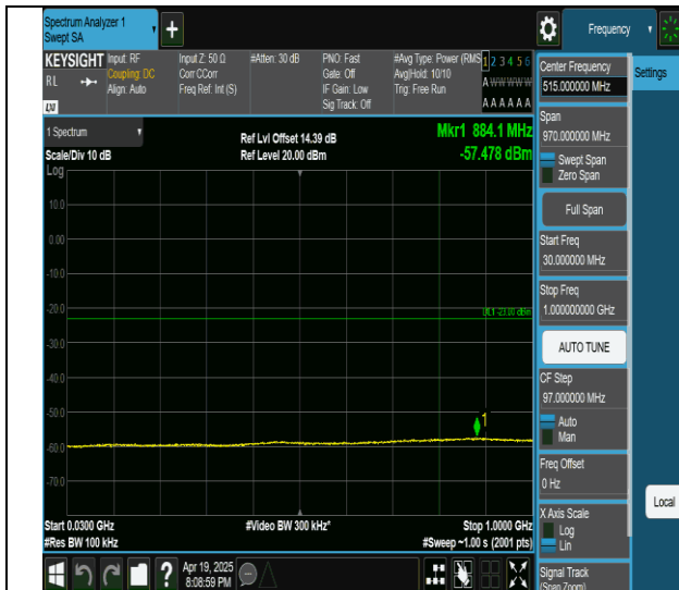
Band4-20MHz-QPSK-20300-1RB#0-30~1000-PASS
