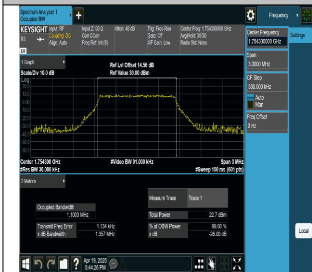
Band4-1.4MHz-64QAM-20393-6RB#0-PASS
