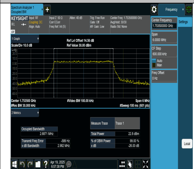
Band4-3MHz-QPSK-20385-15RB#0-PASS
