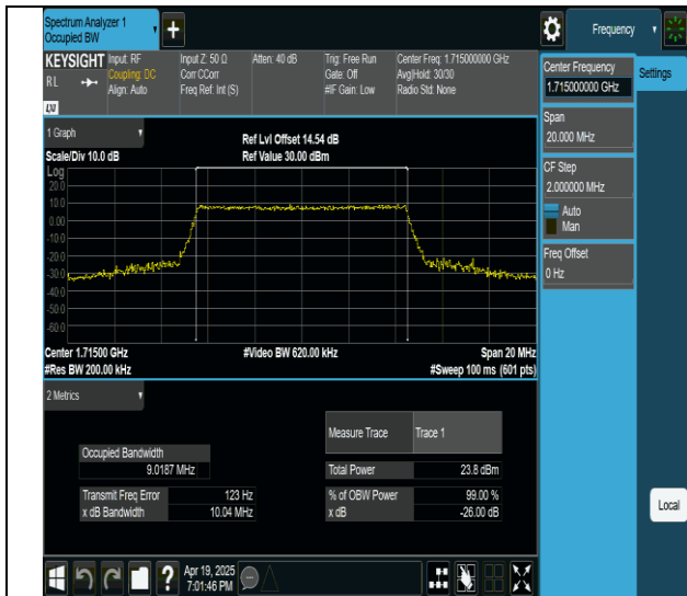
Band4-10MHz-16QAM-20000-50RB#0-PASS
