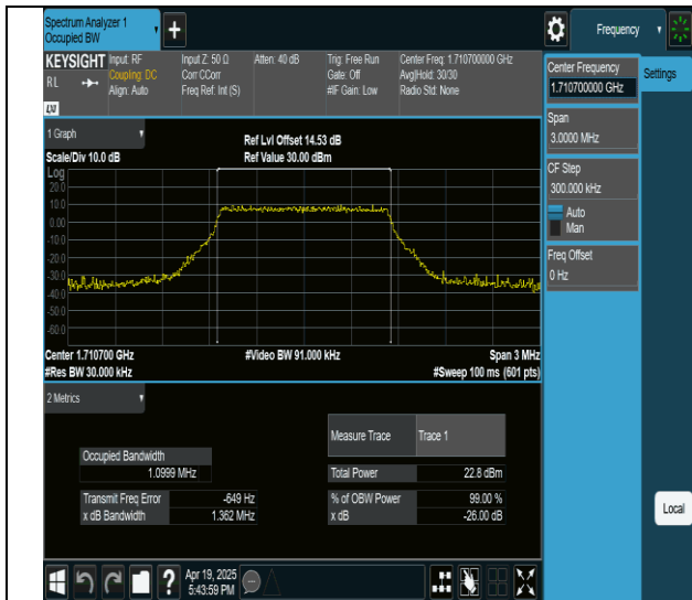
Band4-1.4MHz-64QAM-19957-6RB#0-PASS
