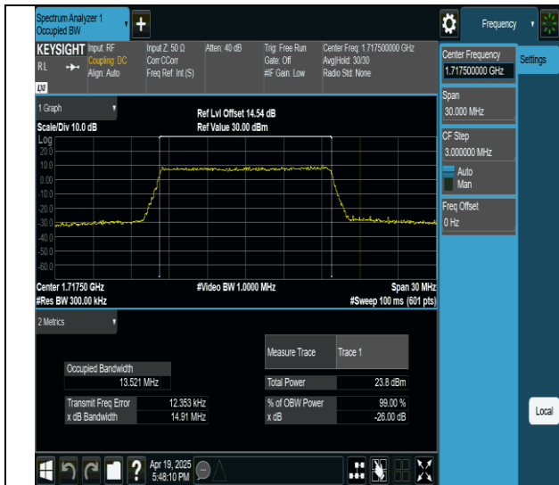
Band4-15MHz-64QAM-20025-75RB#0-PASS
