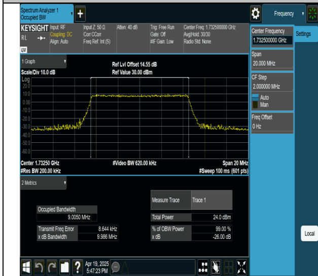
Band4-10MHz-64QAM-20175-50RB#0-PASS
