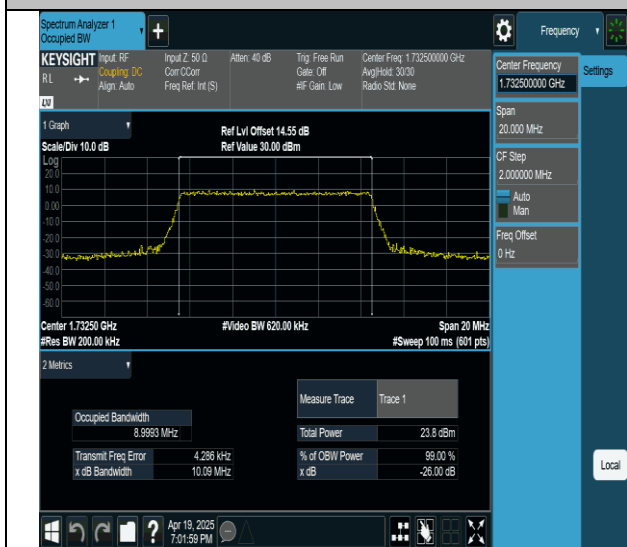
Band4-10MHz-QPSK-20175-50RB#0-PASS
