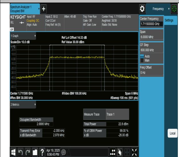
Band4-3MHz-QPSK-19965-15RB#0-PASS
