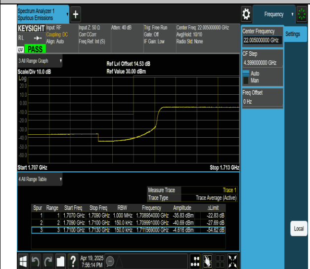
Band4-15MHz-QPSK-20025-75RB#0-PASS
