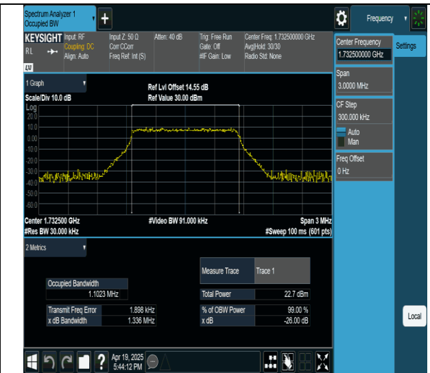
Band4-1.4MHz-64QAM-20175-6RB#0-PASS
