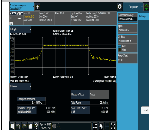
Band4-10MHz-16QAM-20350-50RB#0-PASS
