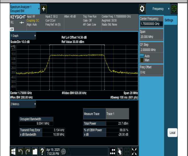
Band4-10MHz-QPSK-20350-50RB#0-PASS
