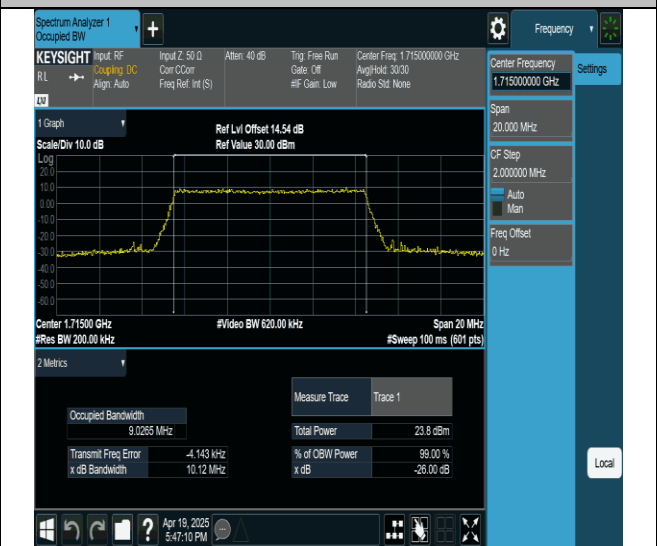
Band4-10MHz-64QAM-20000-50RB#0-PASS
