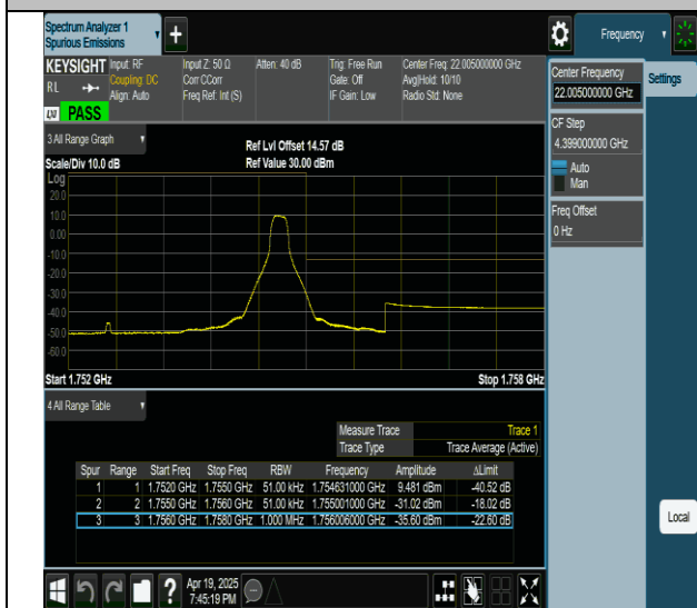
Band4-5MHz-QPSK-20375-1RB#24-PASS
