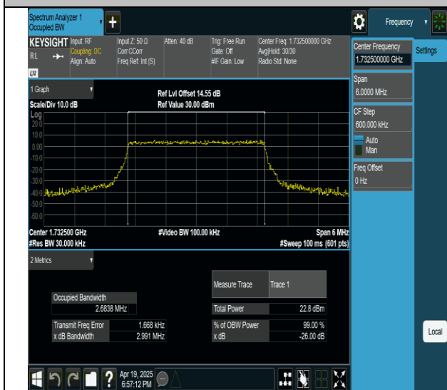
Band4-3MHz-QPSK-20175-15RB#0-PASS
