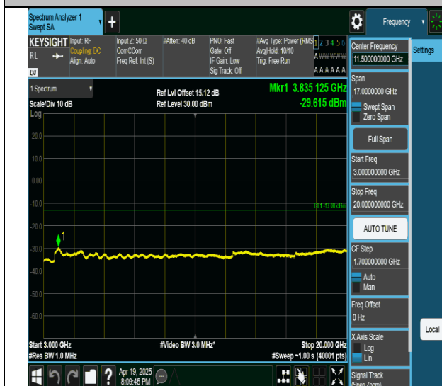
Band4-20MHz-QPSK-20300-1RB#0-3000~20000-PASS
