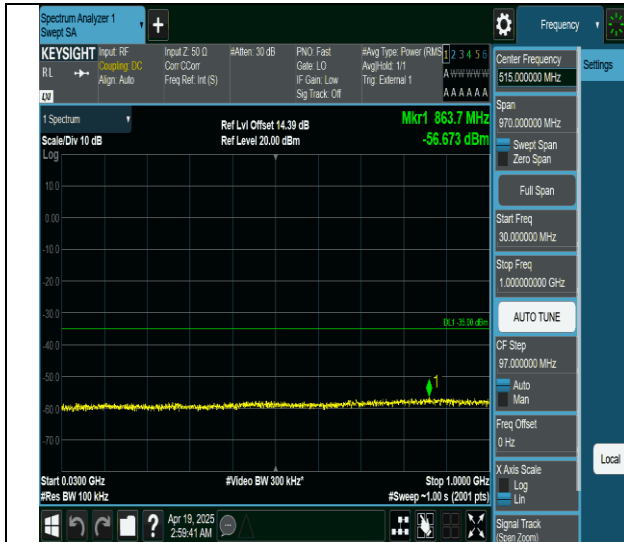
Band41-20MHz-QPSK-41490-1RB#0-30~1000-PASS
