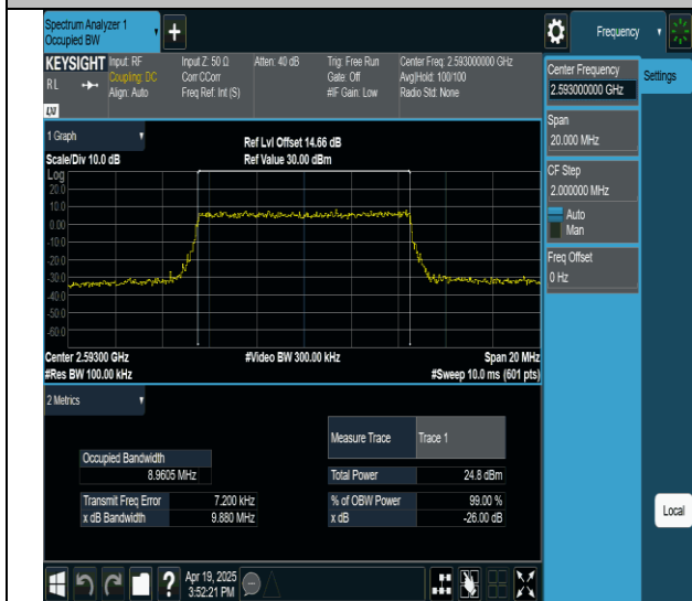
Band41-10MHz-64QAM-40620-50RB#0-PASS
