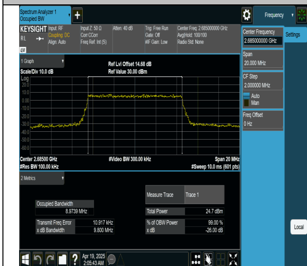
Band41-10MHz-16QAM-41540-50RB#0-PASS
