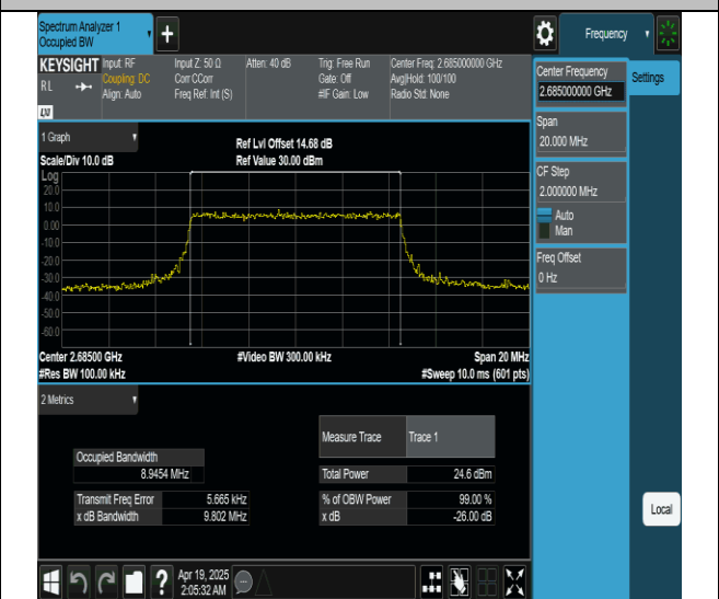
Band41-10MHz-QPSK-41540-50RB#0-PASS
