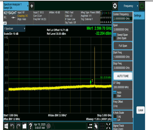
Band41-20MHz-QPSK-41490-1RB#0-1000~3000-PASS
