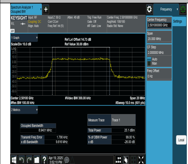
Band41-10MHz-64QAM-39700-50RB#0-PASS
