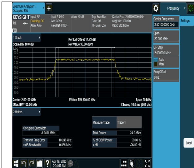
Band41-10MHz-16QAM-39700-50RB#0-PASS
