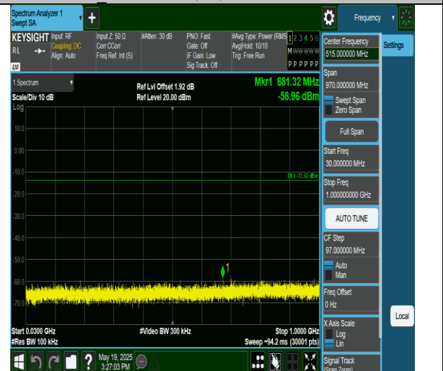
BLE_1M-Ant7-2402-30~1000-PASS
