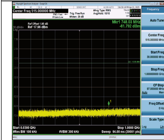
11n20MIMO-Ant6-2462-30~1000-PASS
