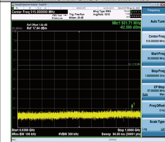
11n20MIMO-Ant7-2412-30~1000-PASS
