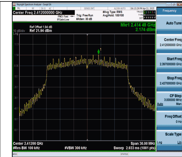
11n20MIMO-Ant7-2412-0~Reference-PASS
