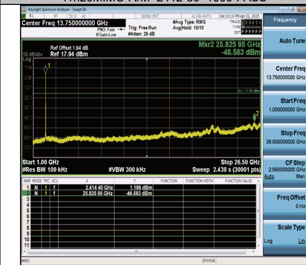
11n20MIMO-Ant7-2412-1000~26500-PASS
