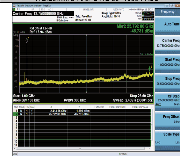
11ax20MIMO-Ant7-2412-1000~26500-PASS
