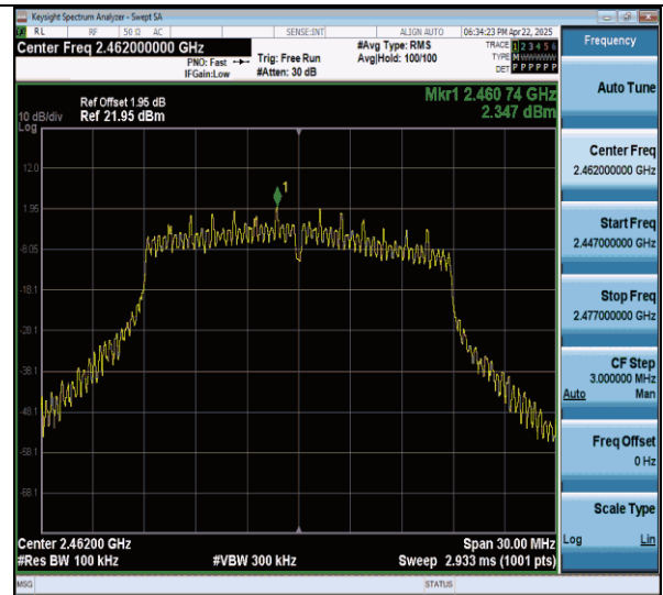
11n20MIMO-Ant7-2462-0~Reference-PASS
