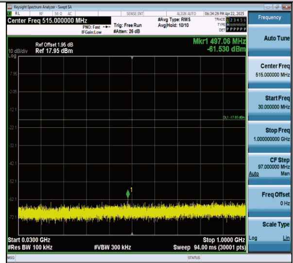
11n20MIMO-Ant7-2462-30~1000-PASS
