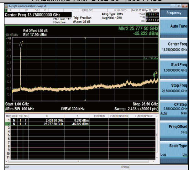
11n20MIMO-Ant7-2462-1000~26500-PASS
