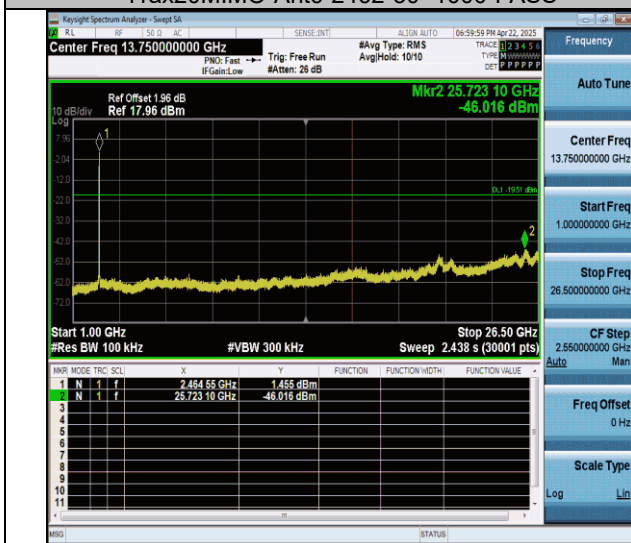
11ax20MIMO-Ant6-2462-1000~26500-PASS
