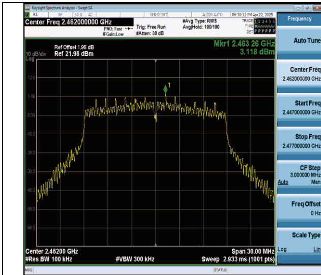
11n20MIMO-Ant6-2462-0~Reference-PASS
