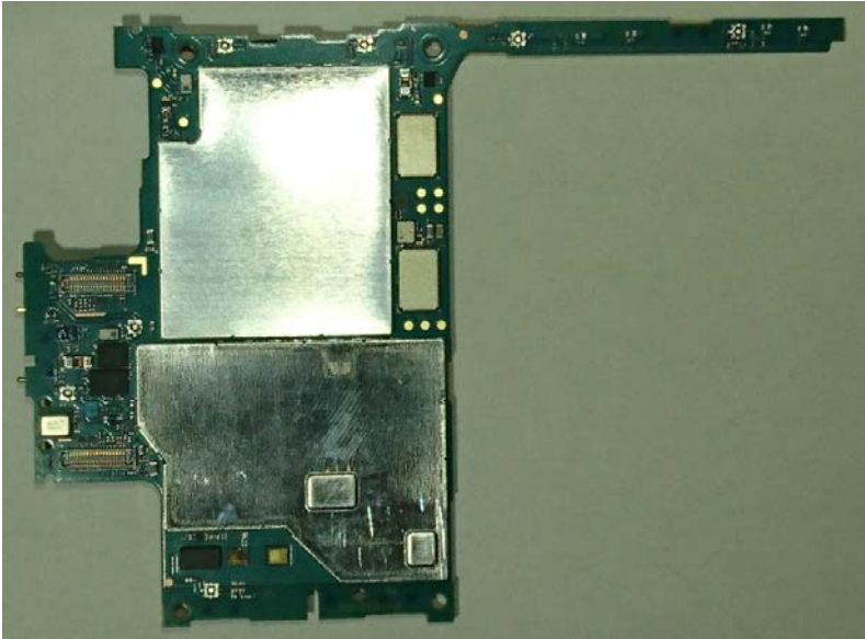
Internal PWB without Shield cases (Rear-side)
