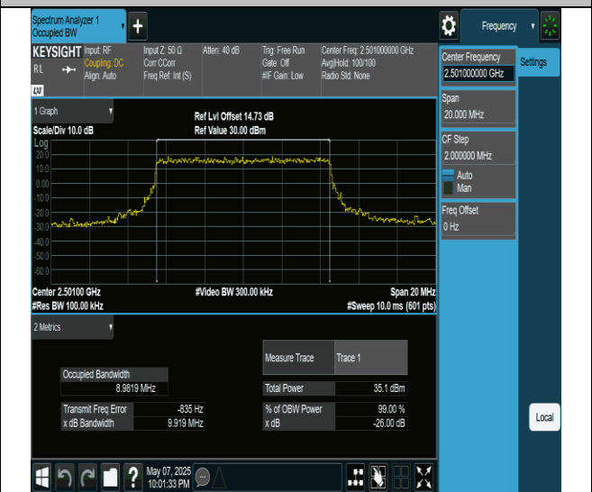
Band41-10MHz-QPSK-39700-50RB#0-PASS
