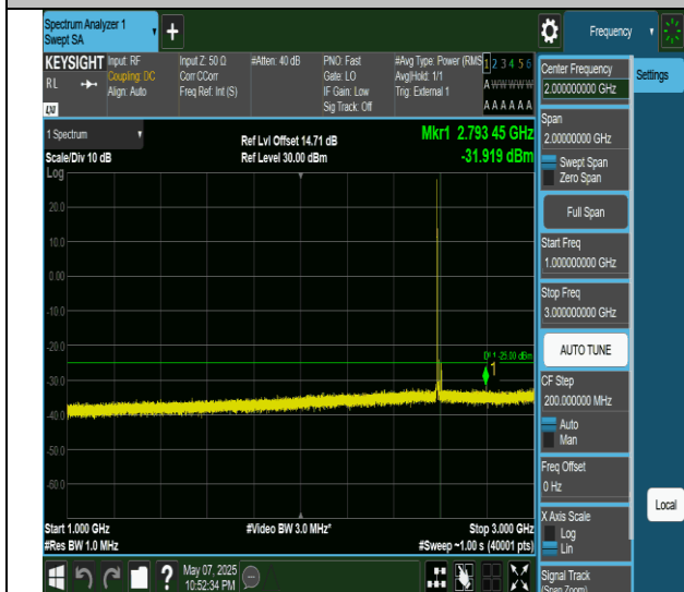
Band41-20MHz-QPSK-40620-1RB#0-1000~3000-PASS
