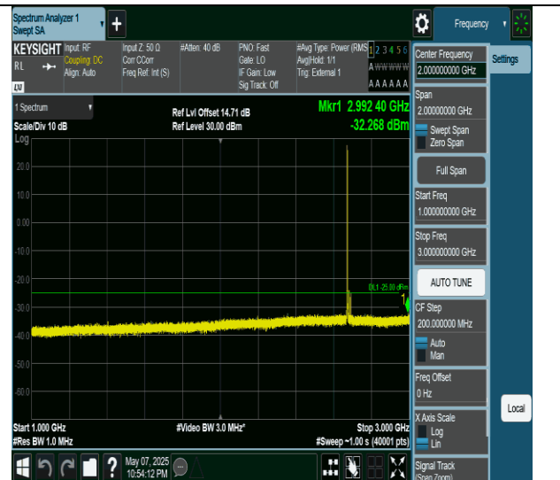
Band41-20MHz-QPSK-41490-1RB#0-1000~3000-PASS
