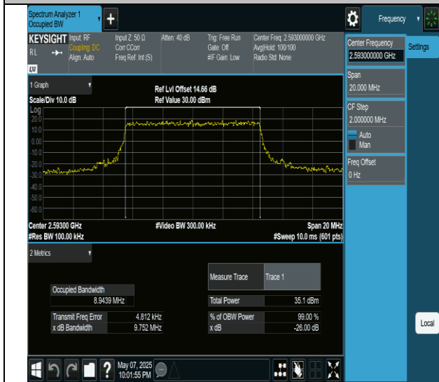
Band41-10MHz-QPSK-40620-50RB#0-PASS
