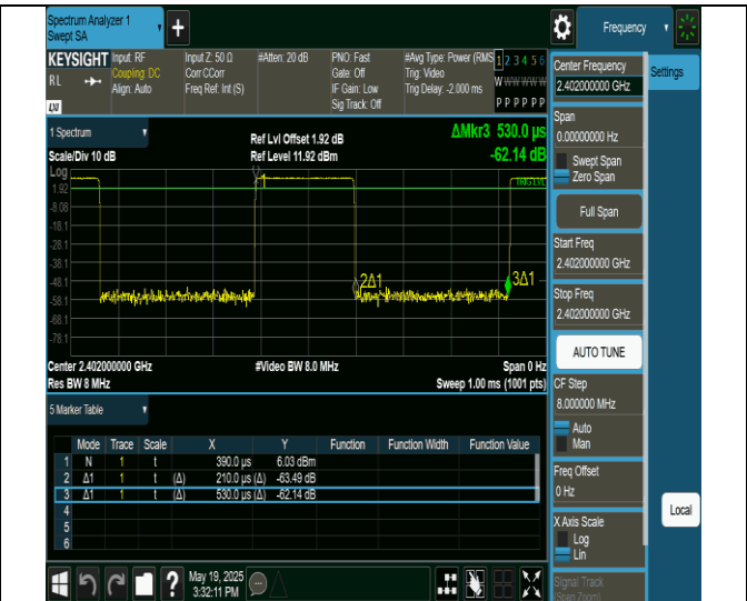
NTVN-BLE 2M-Ant7-2402
