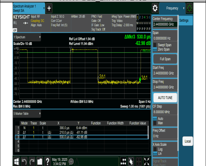
NTVN-BLE 2M-Ant7-2440
