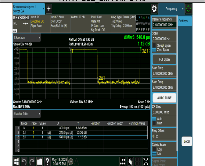
NTVN-BLE 2M-Ant7-2480
