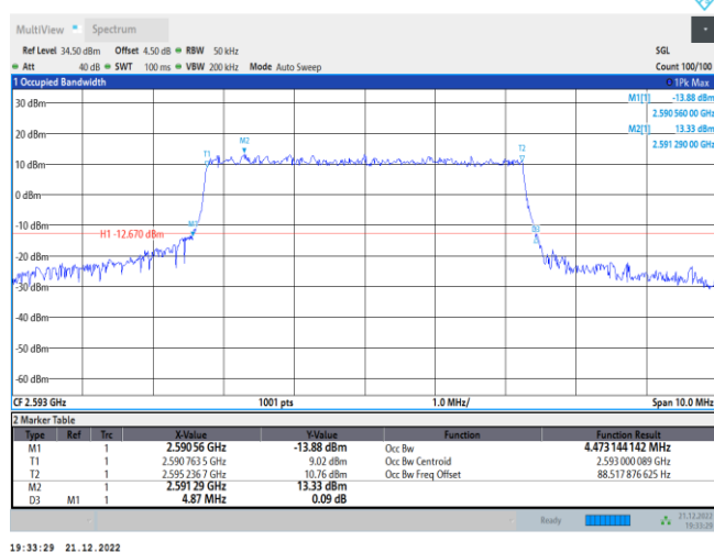
Band41-5MHz-QPSK-40620-25RB#0
