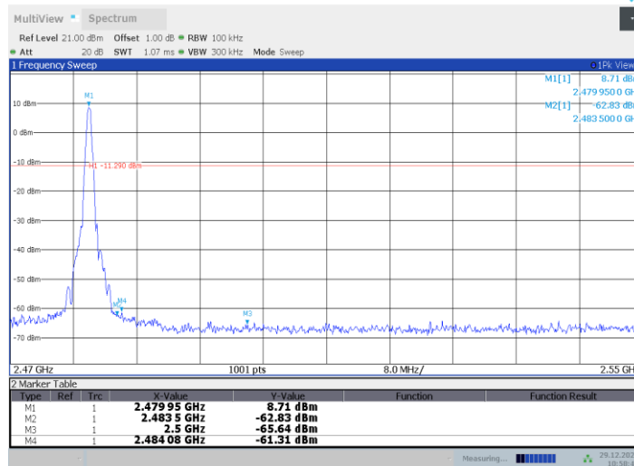
DH5_Ant6_High_2480
