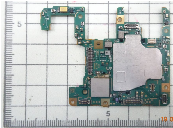
Rear PBA with Shield case (Front-side)
