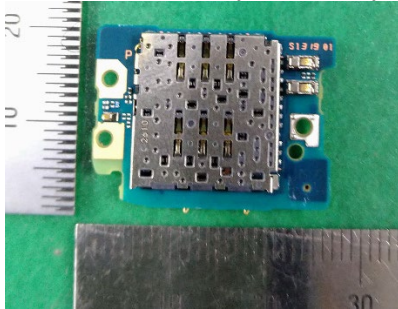
Internal Sub-PWB (Front-side)
