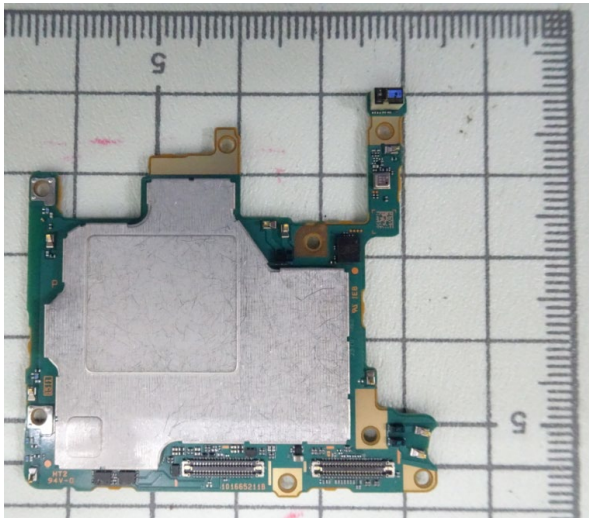
Front PBA with Shield cases (Front-side)
