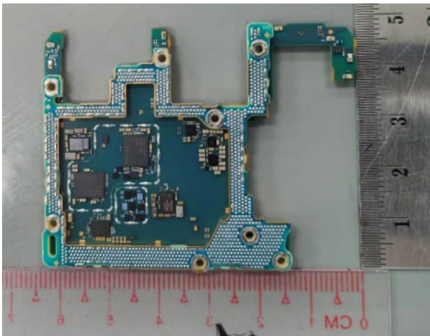
Rear PBA without Shield case (Rear-side)
