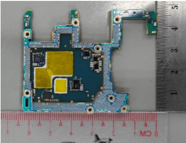
Rear PBA with Shield case (Rear-side)
