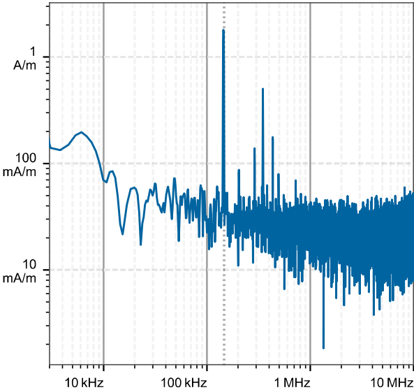
H-field magnitude [RMS] at maximum location
