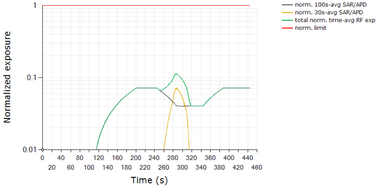
Total Normalized Time-averaged RF Exposure Tech: LTE, Band 66 / Tech: WLAN, Band 5GHz
