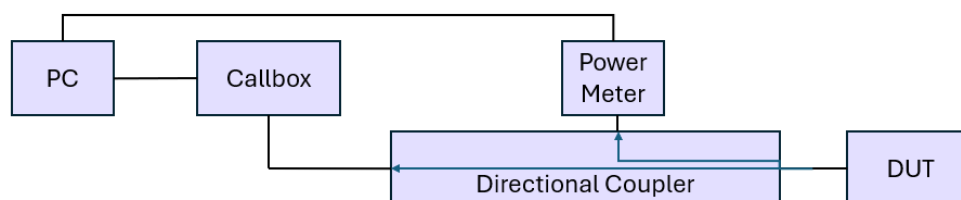
Figure 6-1 Test setup diagram representing connection with 1 Technology
