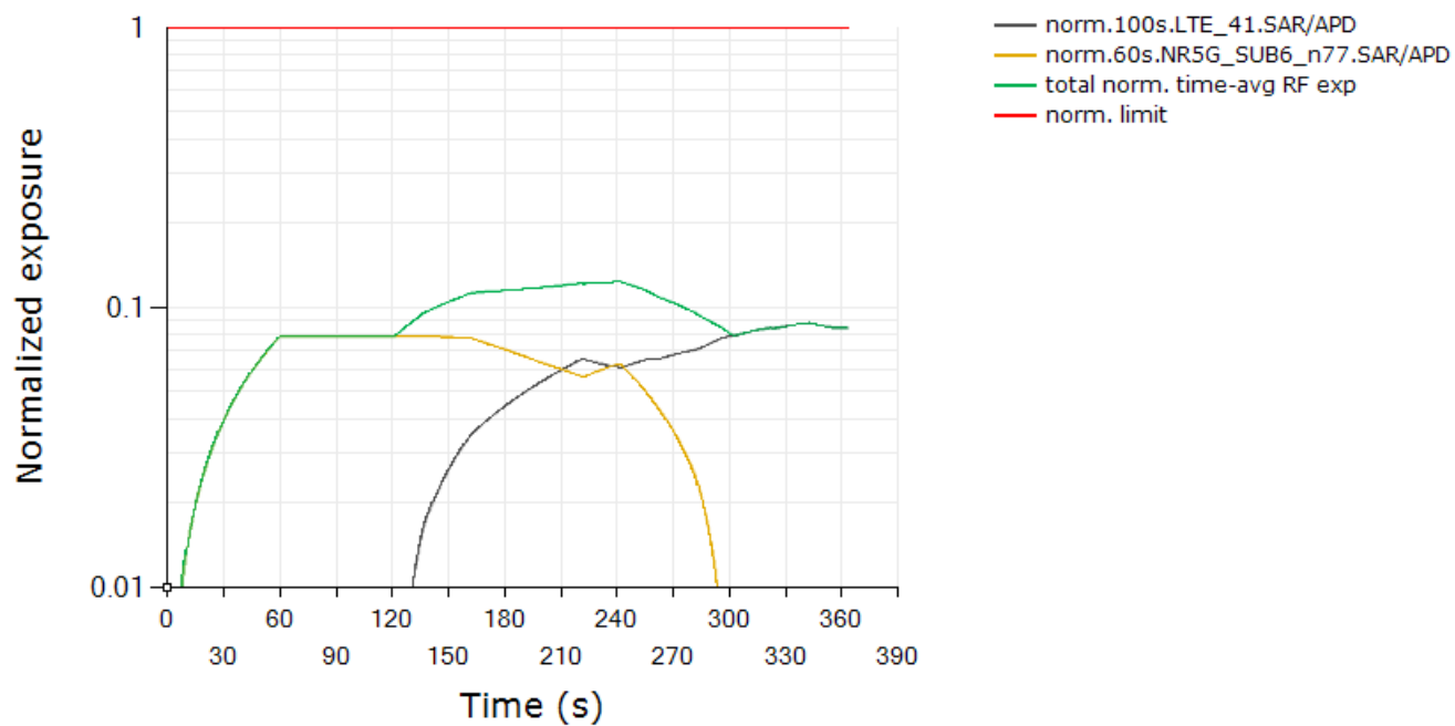
Total Normalized Time-averaged RF Exposure Tech: LTE, Band 41 / Tech: NR5G SUB6, Band n77
