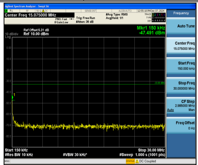
Band IV-1312-0.15~30MHz-PASS
