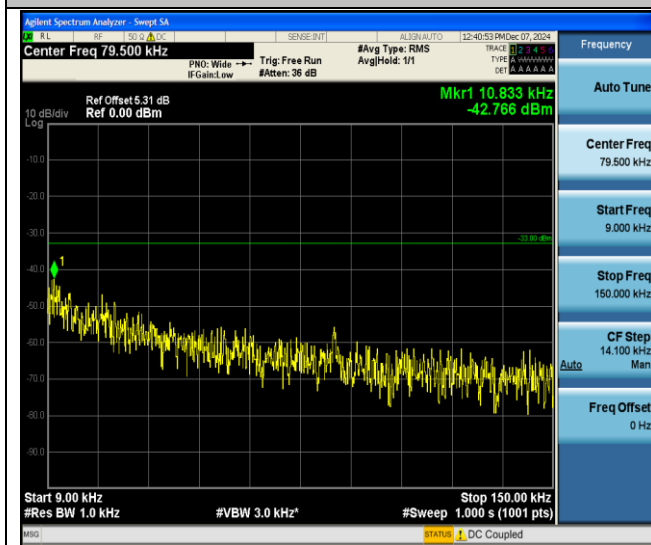
Band V-4233-0.009~0.15MHz-PASS
