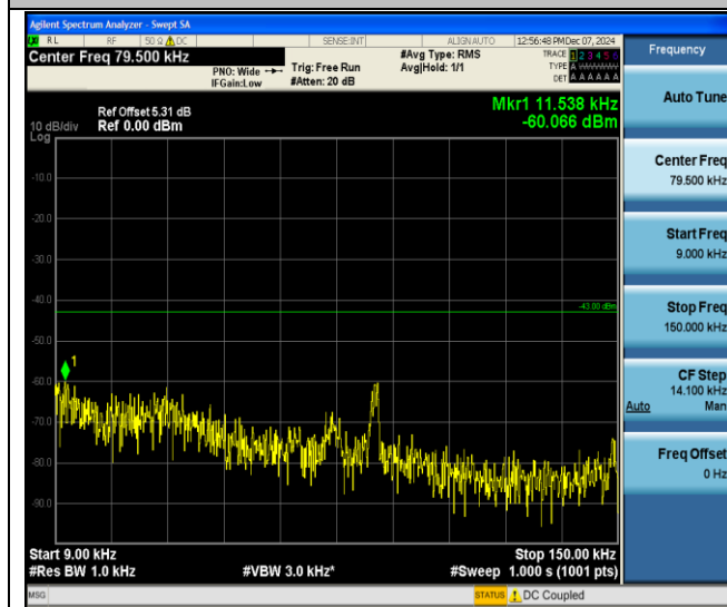
Band IV-1513-0.009~0.15MHz-PASS
