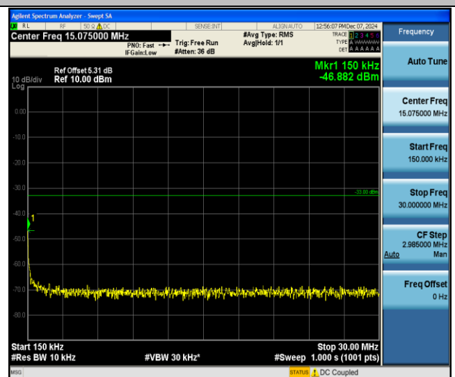
Band IV-1413-0.15~30MHz-PASS
