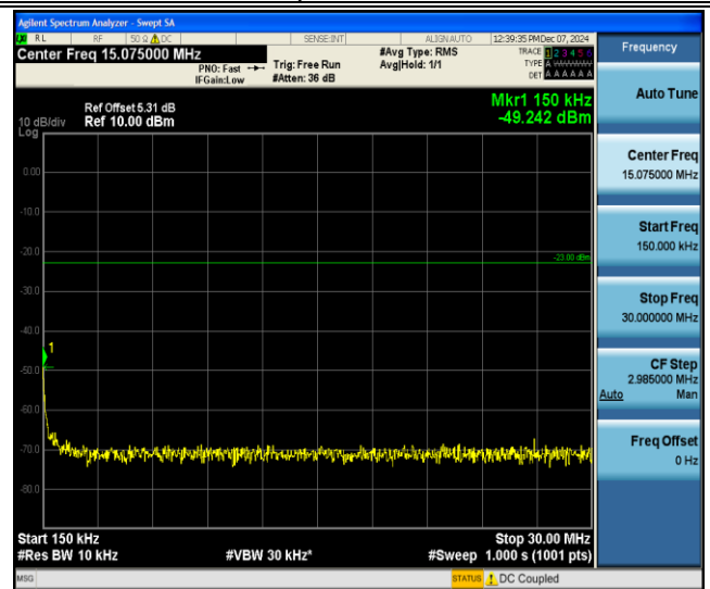
Band V-4132-0.15~30MHz-PASS
