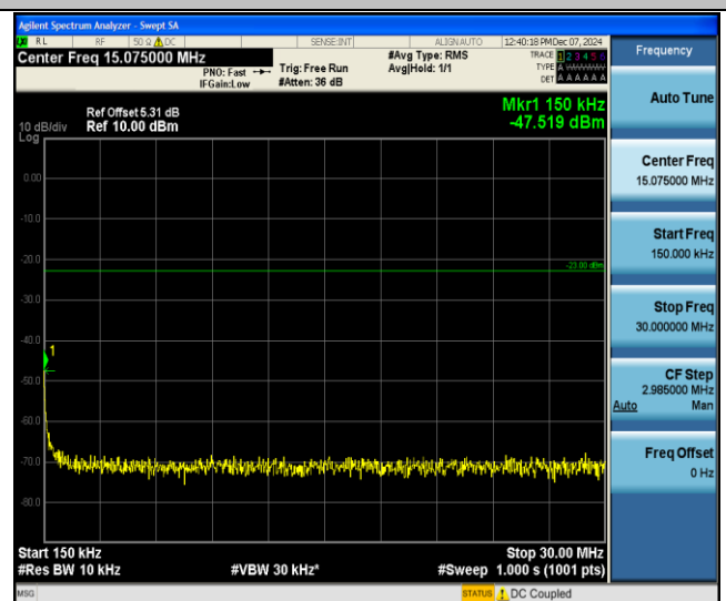
Band V-4182-0.15~30MHz-PASS
