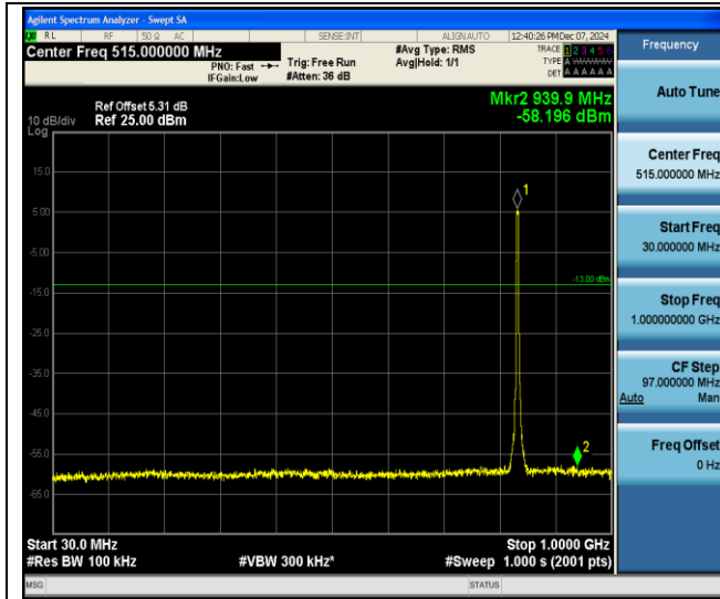
Band V-4182-30~1000MHz-PASS
