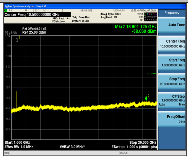
Band IV-1312-1000~20000MHz-PASS
