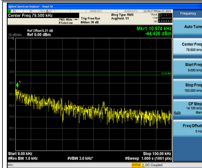
Band V-4132-0.009~0.15MHz-PASS
