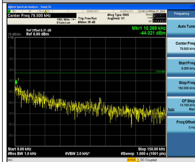
Band V-4182-0.009~0.15MHz-PASS
