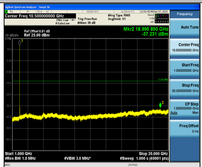
Band II-9538-1000~20000MHz-PASS
