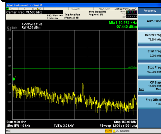
Band IV-1312-0.009~0.15MHz-PASS
