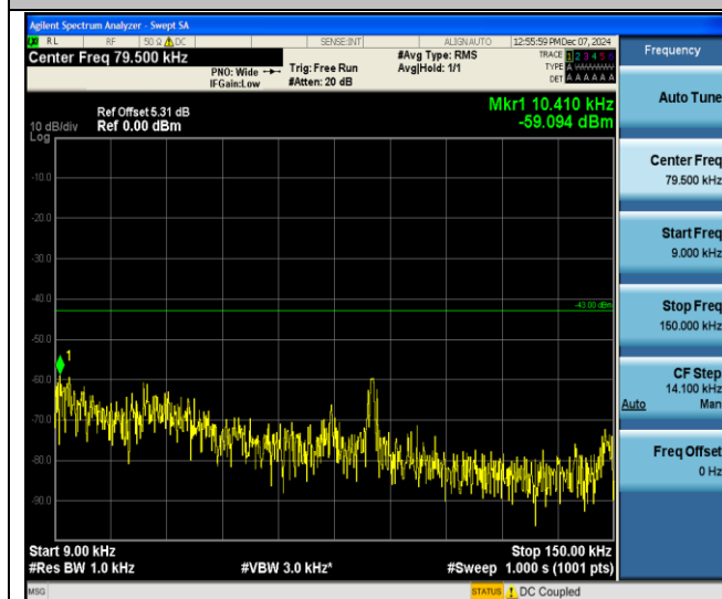
Band IV-1413-0.009~0.15MHz-PASS
