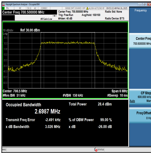
Band12-3MHz-QPSK-23025-15RB#0-PASS
