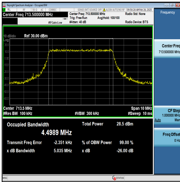
Band12-5MHz-QPSK-23155-25RB#0-PASS
