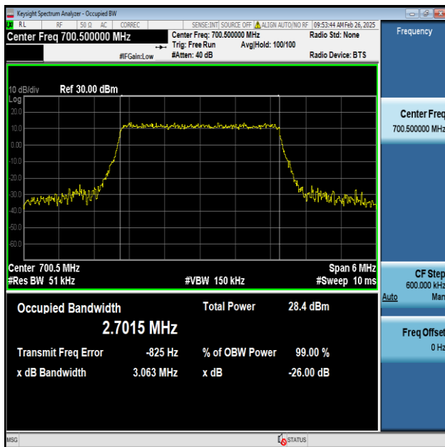
Band12-3MHz-64QAM-23025-15RB#0-PASS
