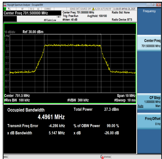
Band12-5MHz-256QAM-23035-25RB#0-PASS
