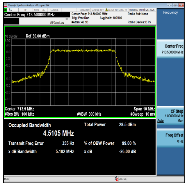
Band12-5MHz-16QAM-23155-25RB#0-PASS
