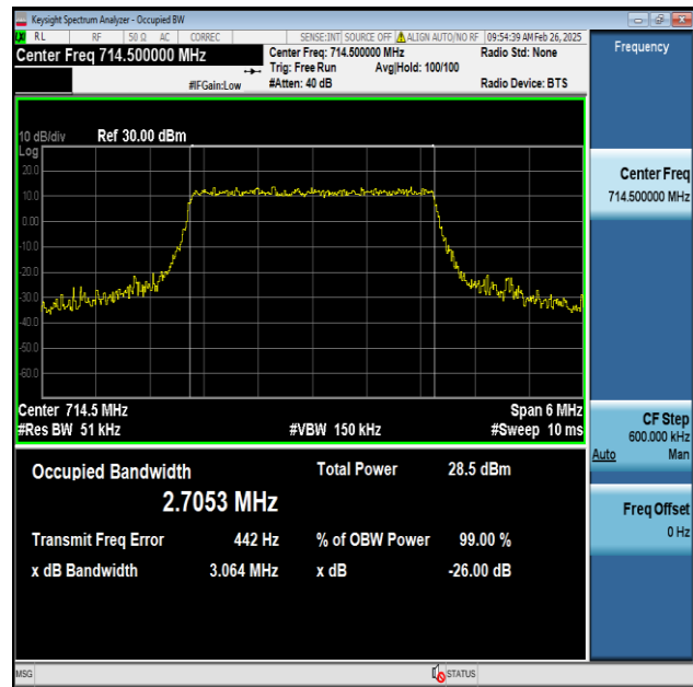
Band12-3MHz-16QAM-23165-15RB#0-PASS
