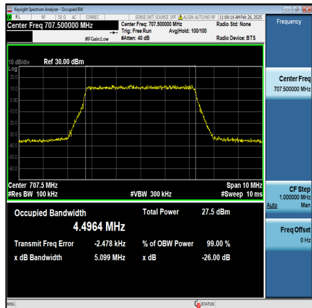
Band12-5MHz-256QAM-23095-25RB#0-PASS
