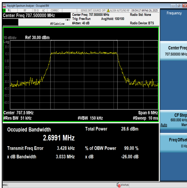
Band12-3MHz-64QAM-23095-15RB#0-PASS
