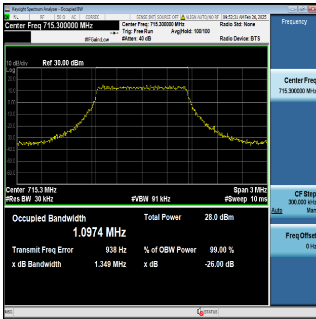
Band12-1.4MHz-QPSK-23173-6RB#0-PASS
