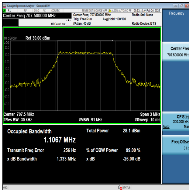
Band12-1.4MHz-64QAM-23095-6RB#0-PASS
