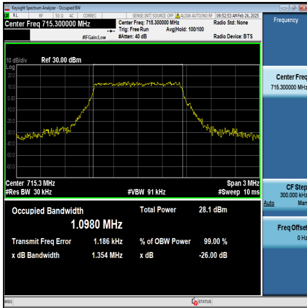
Band12-1.4MHz-64QAM-23173-6RB#0-PASS
