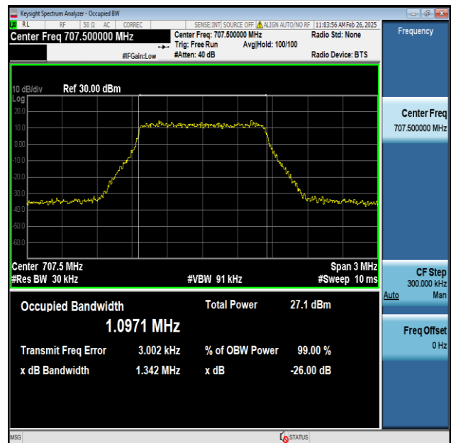
Band12-1.4MHz-256QAM-23095-6RB#0-PASS
