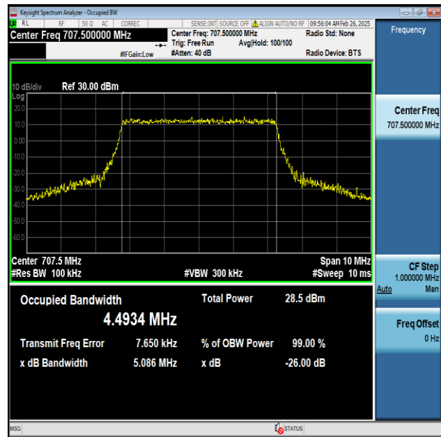
Band12-5MHz-16QAM-23095-25RB#0-PASS
