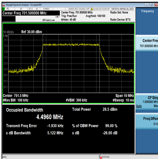
Band12-5MHz-64QAM-23035-25RB#0-PASS
