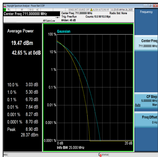
Band12-10MHz-256QAM-23130-50RB#0-PASS
