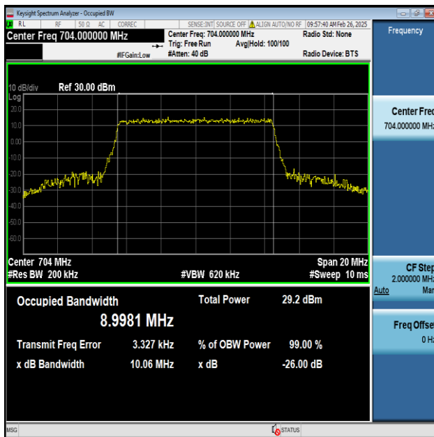
Band12-10MHz-64QAM-23060-50RB#0-PASS
