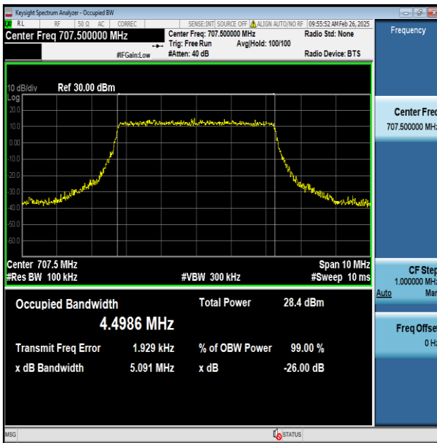
Band12-5MHz-QPSK-23095-25RB#0-PASS
