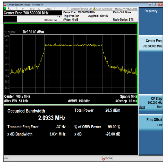
Band12-3MHz-16QAM-23025-15RB#0-PASS
