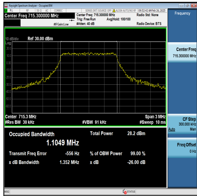
Band12-1.4MHz-16QAM-23173-6RB#0-PASS
