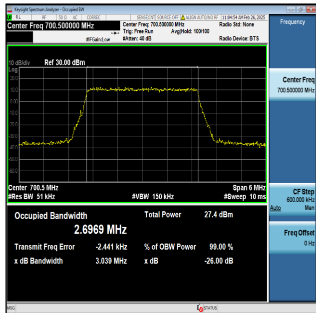
Band12-3MHz-256QAM-23025-15RB#0-PASS
