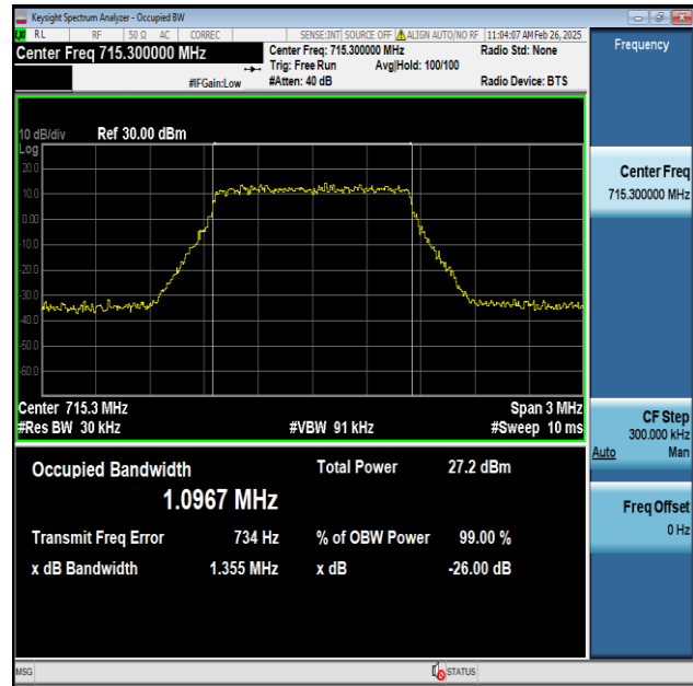
Band12-1.4MHz-256QAM-23173-6RB#0-PASS
