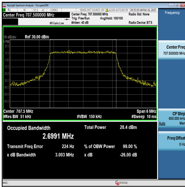
Band12-3MHz-QPSK-23095-15RB#0-PASS
