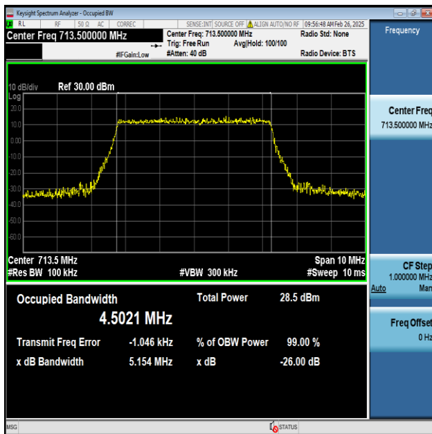
Band12-5MHz-64QAM-23155-25RB#0-PASS
