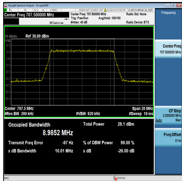
Band12-10MHz-256QAM-23095-50RB#0-PASS
