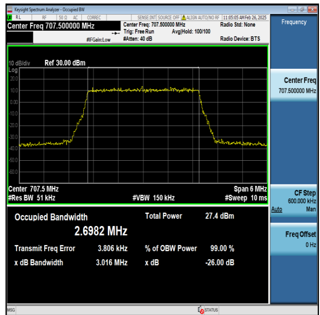
Band12-3MHz-256QAM-23095-15RB#0-PASS
