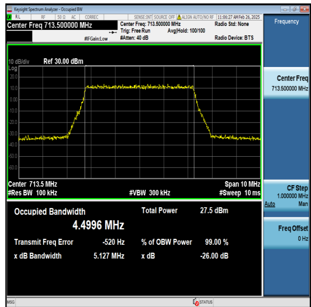
Band12-5MHz-256QAM-23155-25RB#0-PASS
