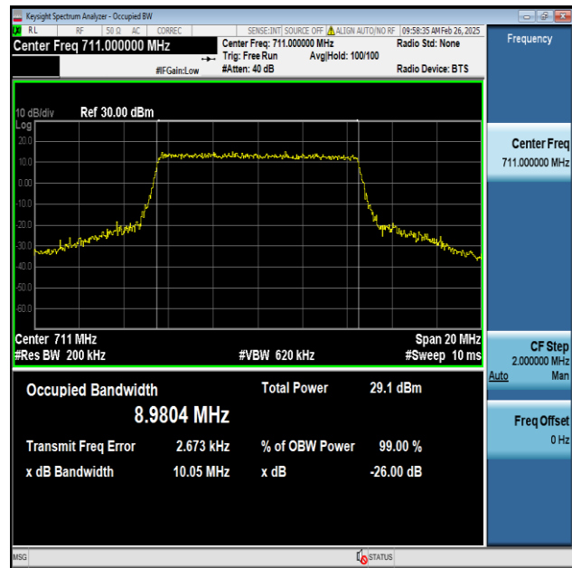
Band12-10MHz-16QAM-23130-50RB#0-PASS
