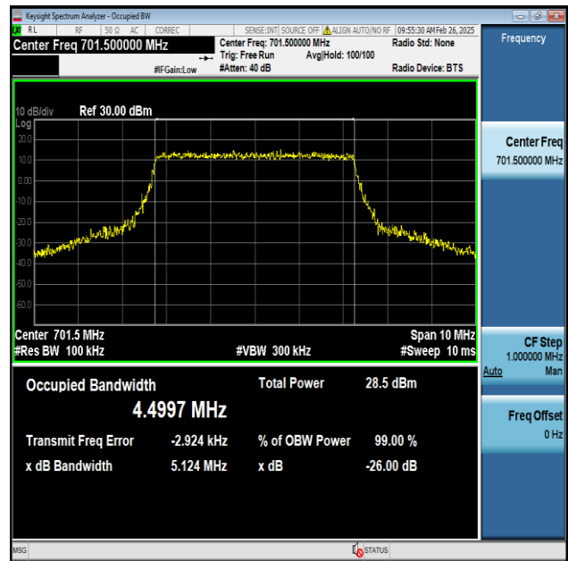
Band12-5MHz-16QAM-23035-25RB#0-PASS
