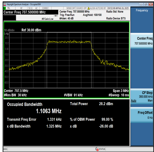
Band12-1.4MHz-16QAM-23095-6RB#0-PASS
