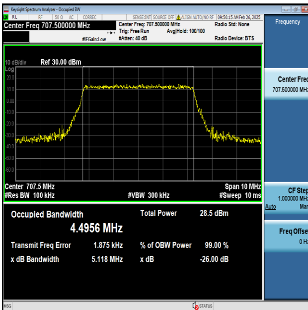
Band12-5MHz-64QAM-23095-25RB#0-PASS
