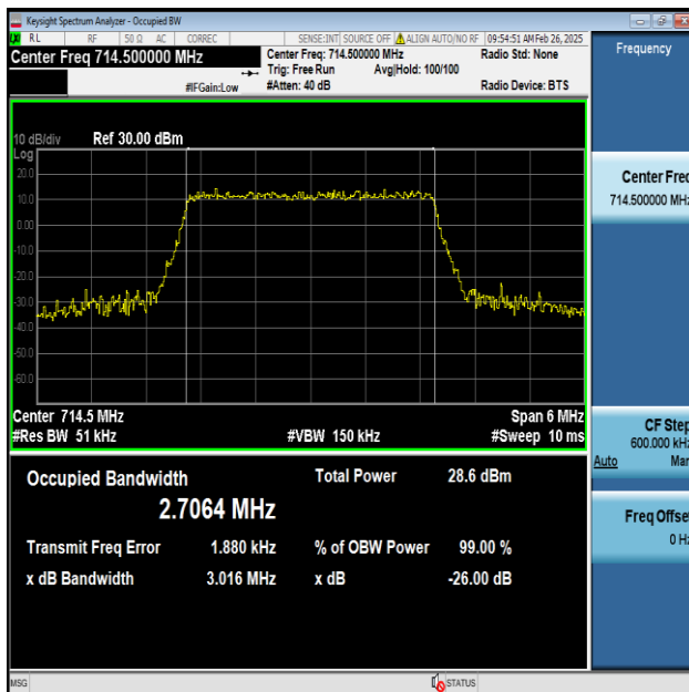
Band12-3MHz-64QAM-23165-15RB#0-PASS
