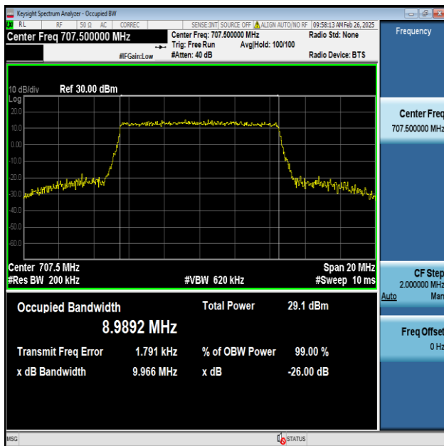
Band12-10MHz-64QAM-23095-50RB#0-PASS
