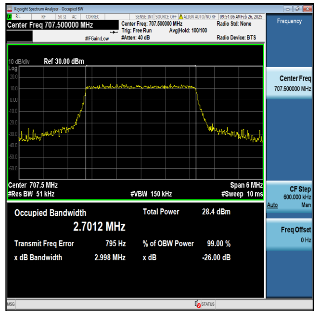
Band12-3MHz-16QAM-23095-15RB#0-PASS
