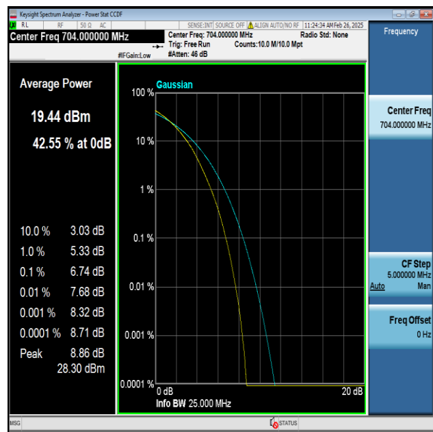
Band12-10MHz-256QAM-23060-50RB#0-PASS
