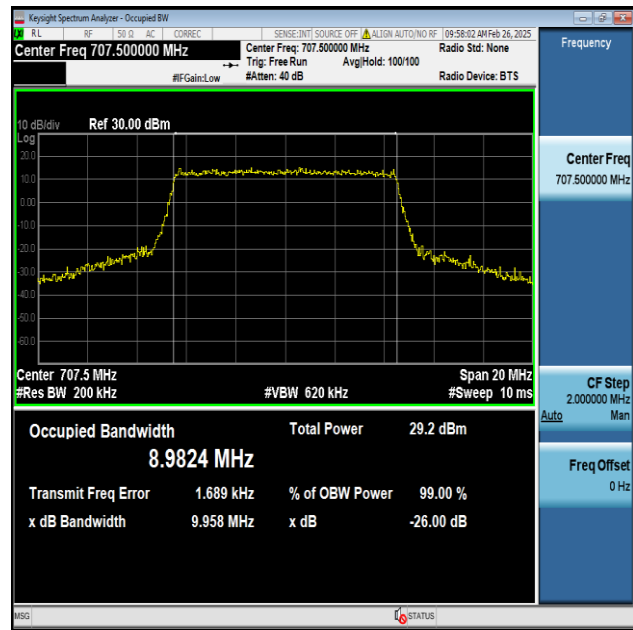
Band12-10MHz-16QAM-23095-50RB#0-PASS
