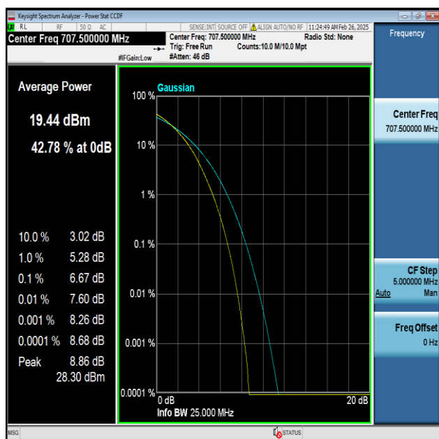
Band12-10MHz-256QAM-23095-50RB#0-PASS
