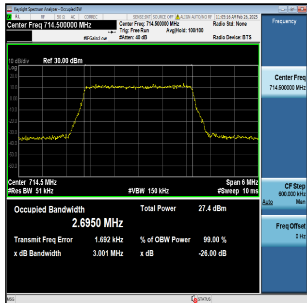
Band12-3MHz-256QAM-23165-15RB#0-PASS
