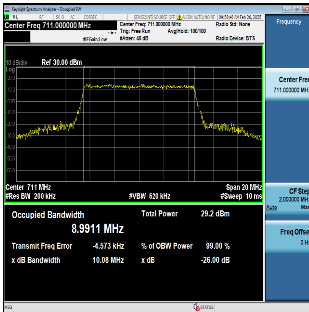
Band12-10MHz-64QAM-23130-50RB#0-PASS
