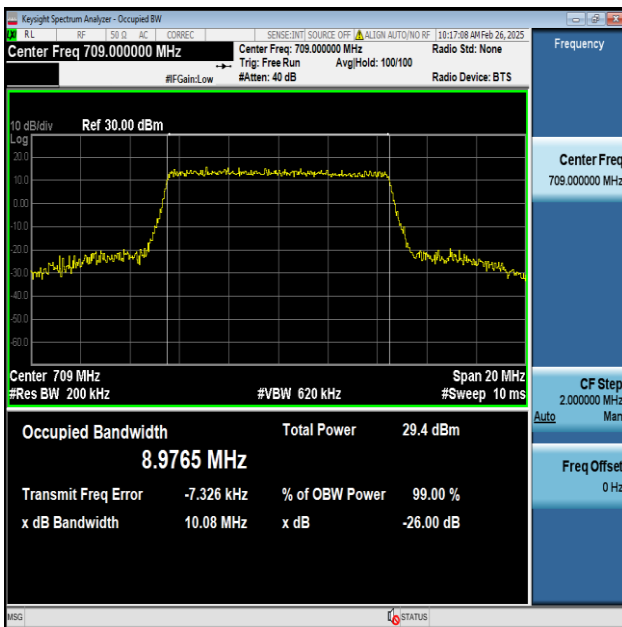
Band17-10MHz-64QAM-23780-50RB#0-PASS
