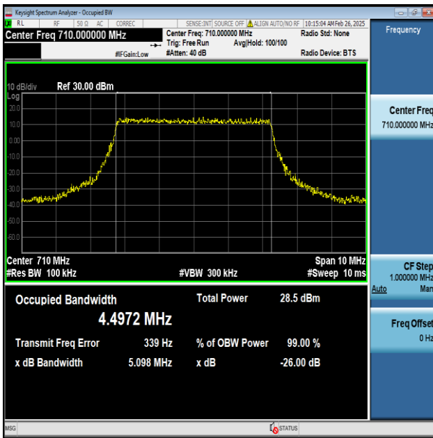
Band17-5MHz-QPSK-23790-25RB#0-PASS
