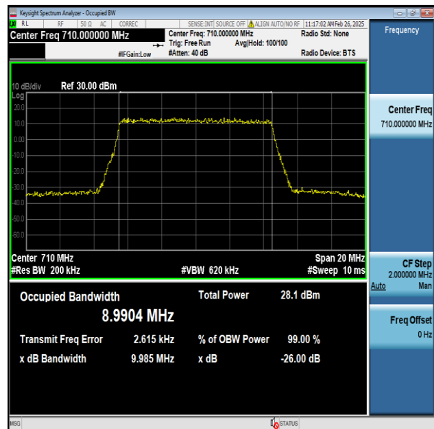
Band17-10MHz-256QAM-23790-50RB#0-PASS
