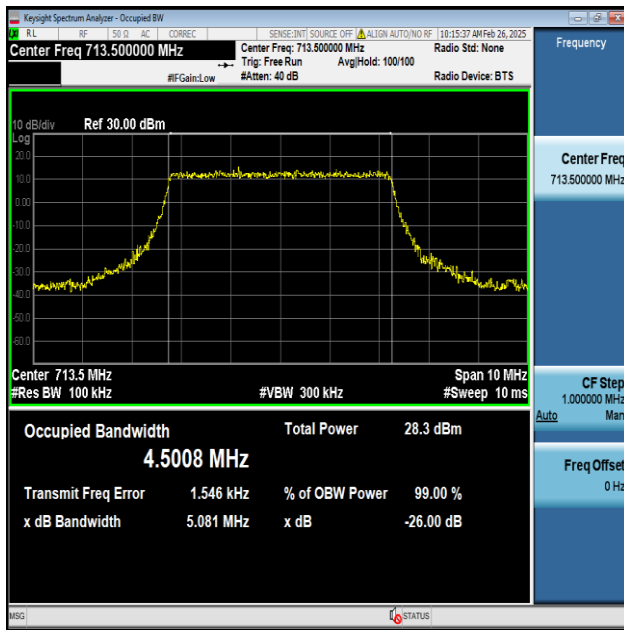
Band17-5MHz-QPSK-23825-25RB#0-PASS
