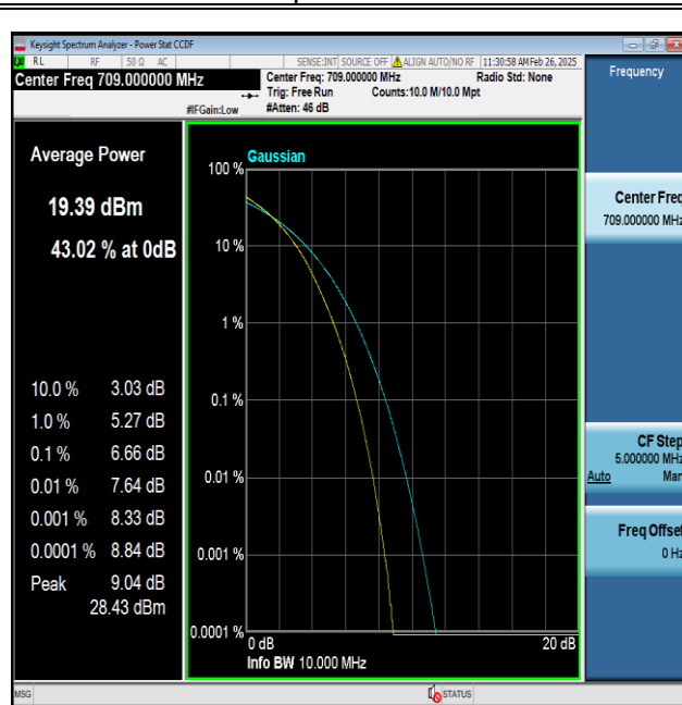
Band17-10MHz-256QAM-23780-50RB#0-PASS
