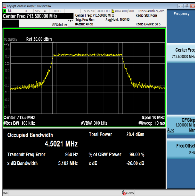
Band17-5MHz-64QAM-23825-25RB#0-PASS
