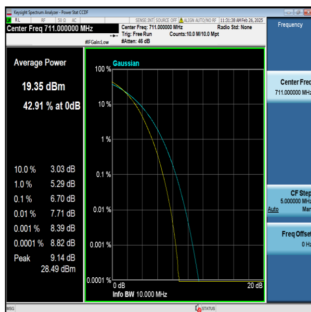
Band17-10MHz-256QAM-23800-50RB#0-PASS
