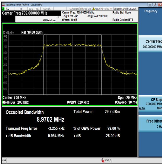
Band17-10MHz-QPSK-23780-50RB#0-PASS
