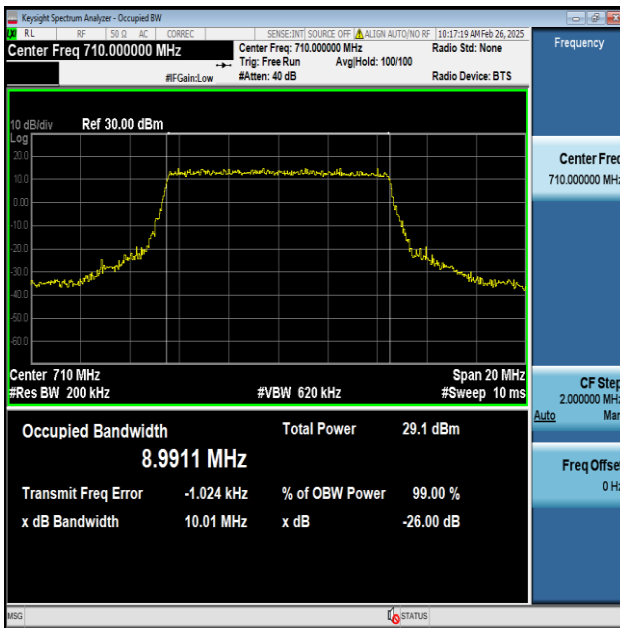
Band17-10MHz-QPSK-23790-50RB#0-PASS
