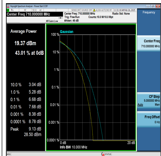
Band17-10MHz-256QAM-23790-50RB#0-PASS
