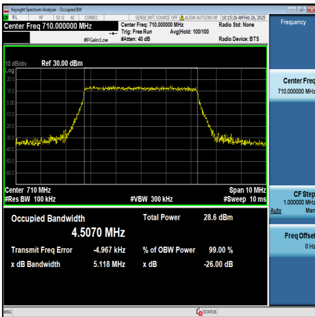
Band17-5MHz-64QAM-23790-25RB#0-PASS
