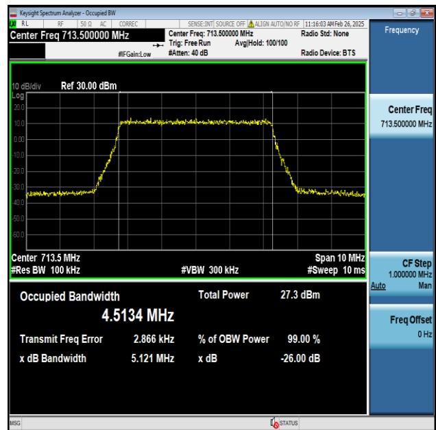
Band17-5MHz-256QAM-23825-25RB#0-PASS
