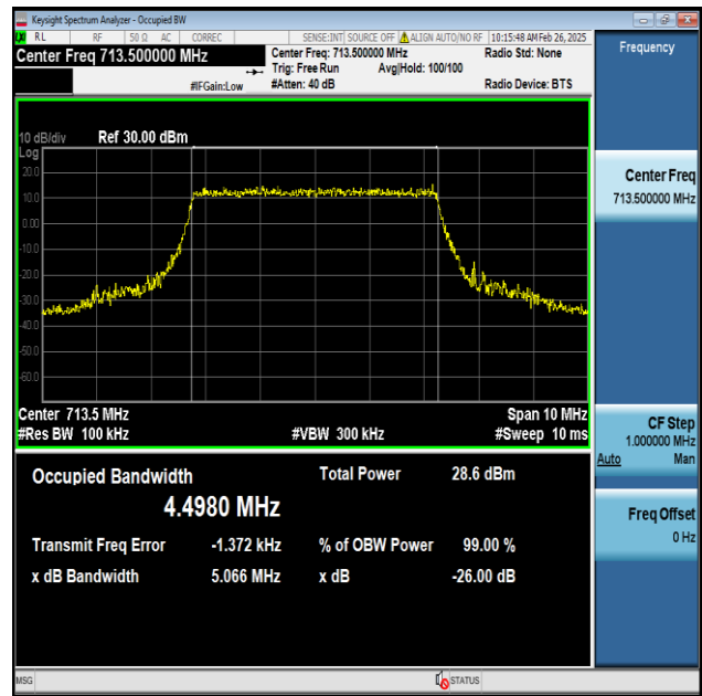
Band17-5MHz-16QAM-23825-25RB#0-PASS
