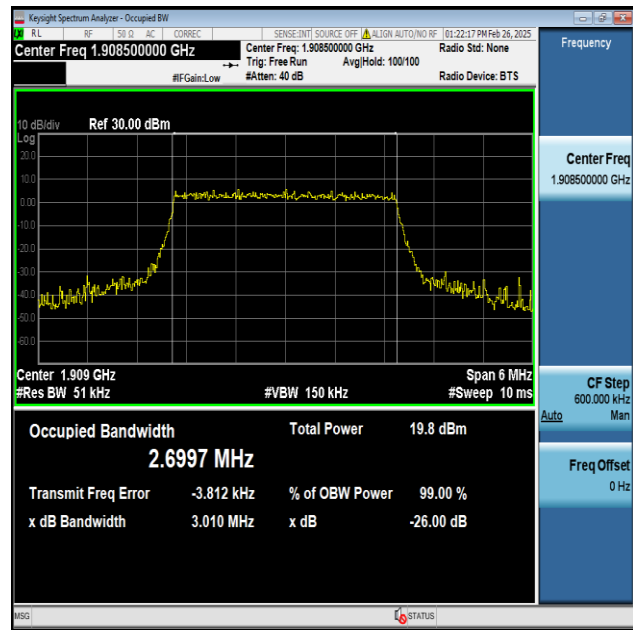
Band2-3MHz-16QAM-19185-15RB#0-PASS
