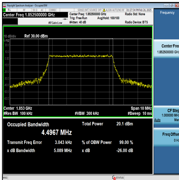
Band2-5MHz-64QAM-18625-25RB#0-PASS
