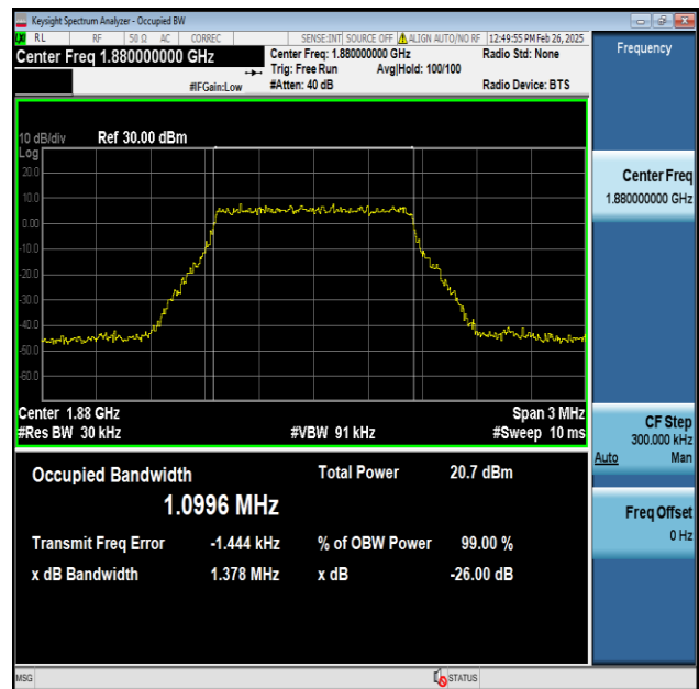
Band2-1.4MHz-256QAM-18900-6RB#0-PASS
