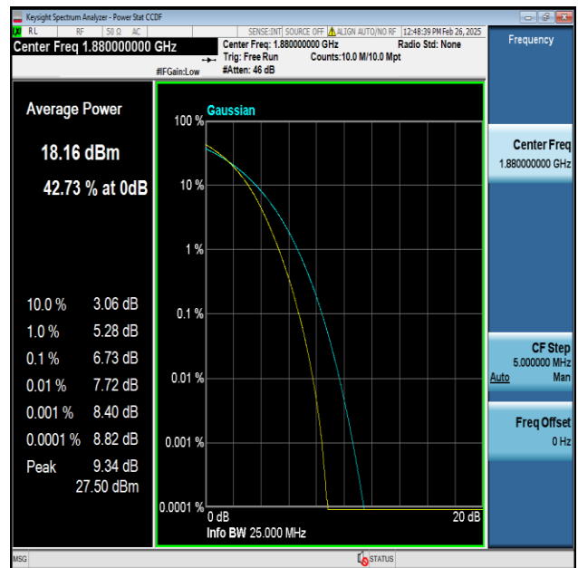
Band2-20MHz-256QAM-18900-100RB#0-PASS
