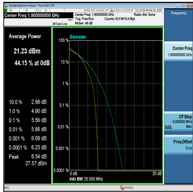
Band2-20MHz-16QAM-19100-100RB#0-PASS
