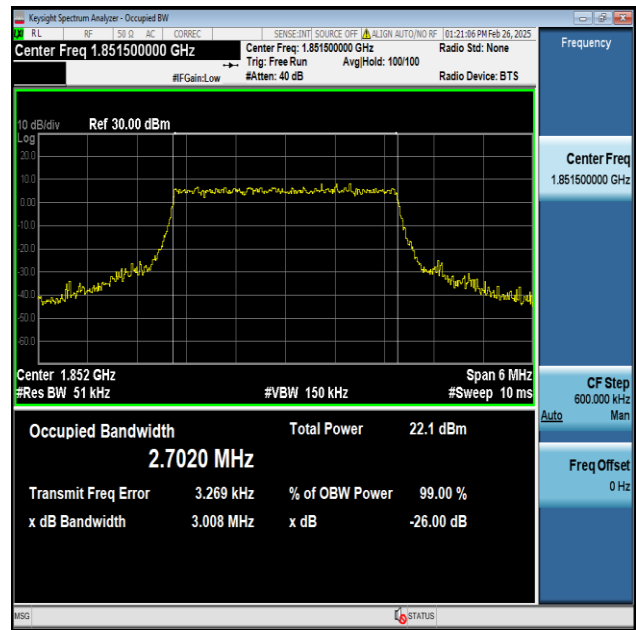
Band2-3MHz-16QAM-18615-15RB#0-PASS
