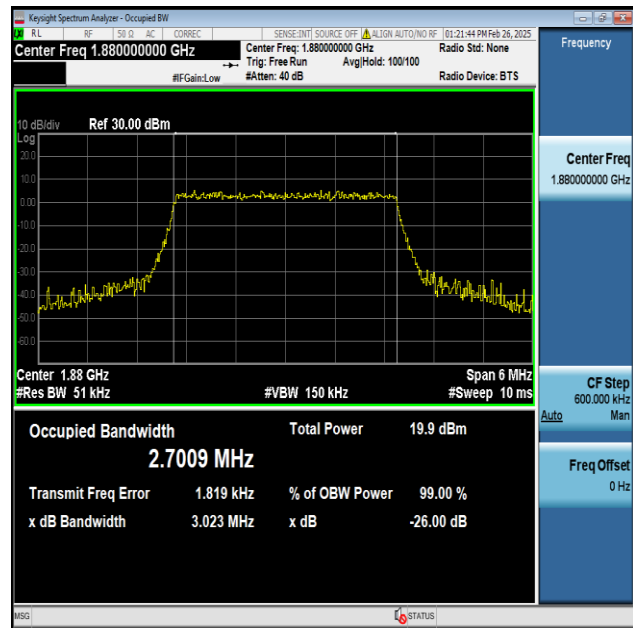
Band2-3MHz-16QAM-18900-15RB#0-PASS
