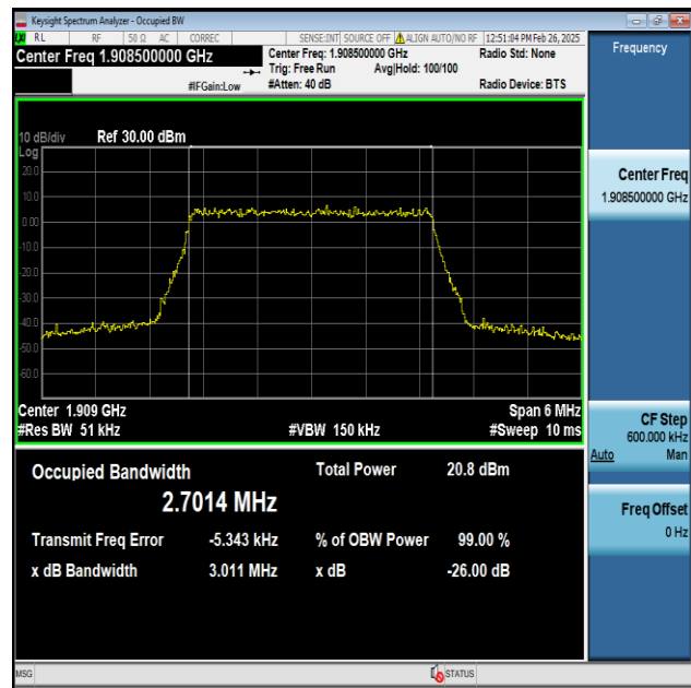
Band2-3MHz-256QAM-19185-15RB#0-PASS
