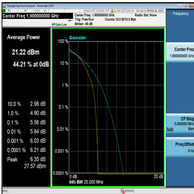
Band2-20MHz-64QAM-19100-100RB#0-PASS
