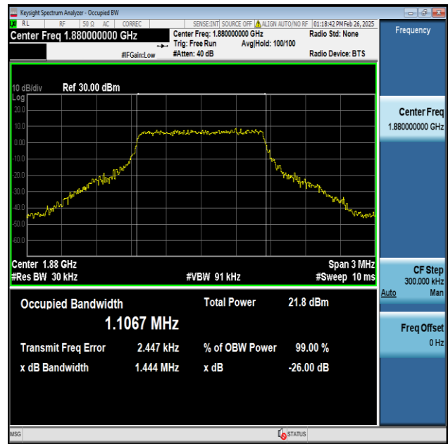
Band2-1.4MHz-16QAM-18900-6RB#0-PASS
