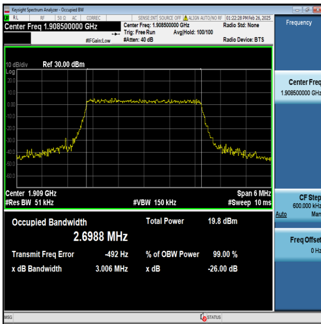
Band2-3MHz-64QAM-19185-15RB#0-PASS
