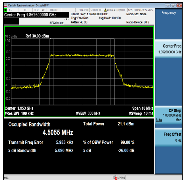
Band2-5MHz-256QAM-18625-25RB#0-PASS
