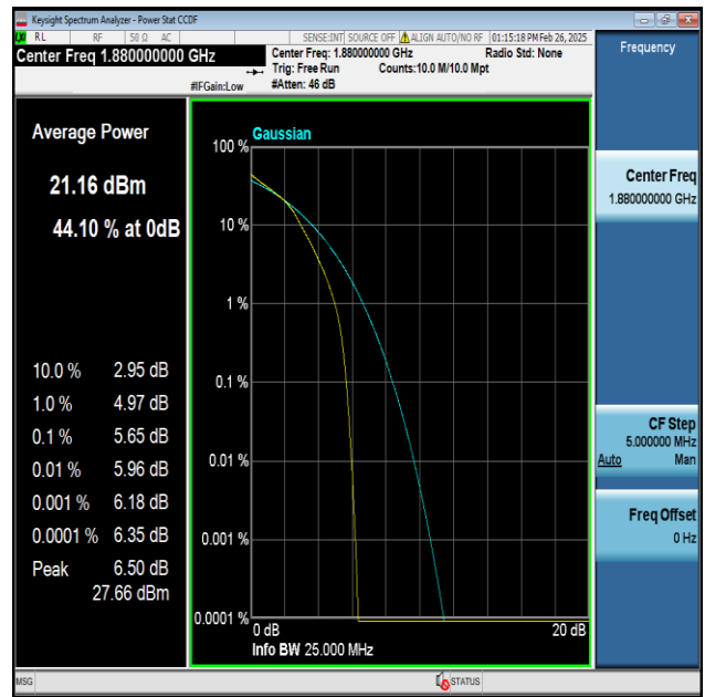
Band2-20MHz-16QAM-18900-100RB#0-PASS
