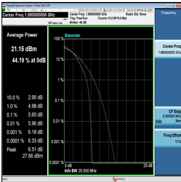
Band2-20MHz-64QAM-18900-100RB#0-PASS
