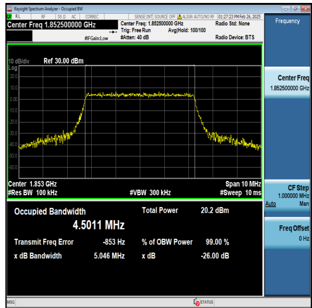
Band2-5MHz-16QAM-18625-25RB#0-PASS
