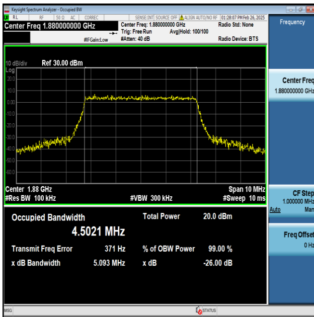
Band2-5MHz-64QAM-18900-25RB#0-PASS
