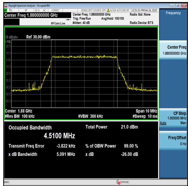
Band2-5MHz-256QAM-18900-25RB#0-PASS
