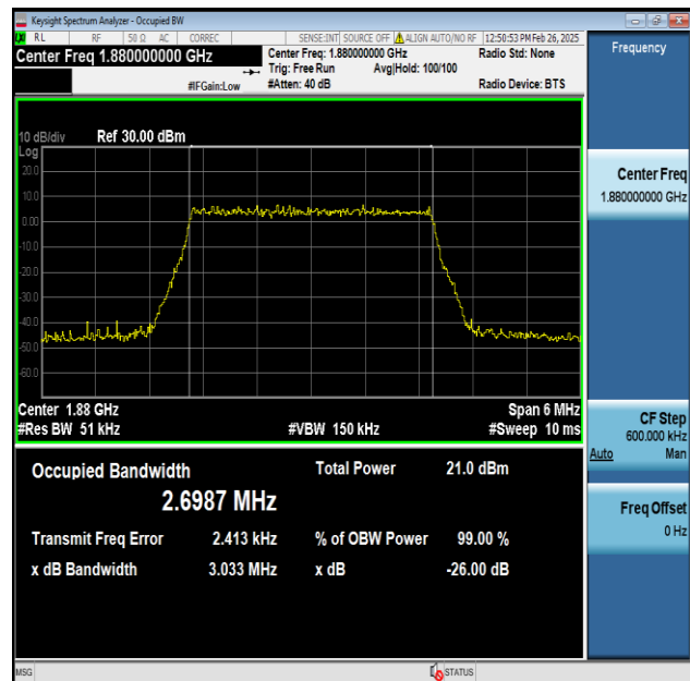
Band2-3MHz-256QAM-18900-15RB#0-PASS
