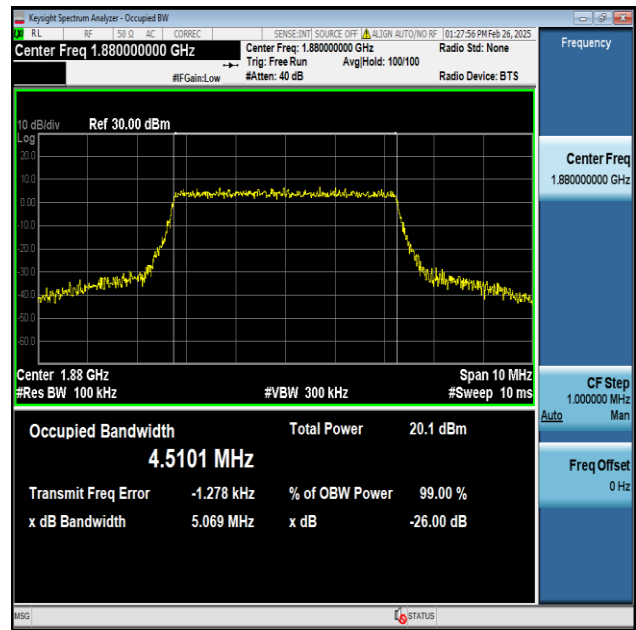
Band2-5MHz-16QAM-18900-25RB#0-PASS
