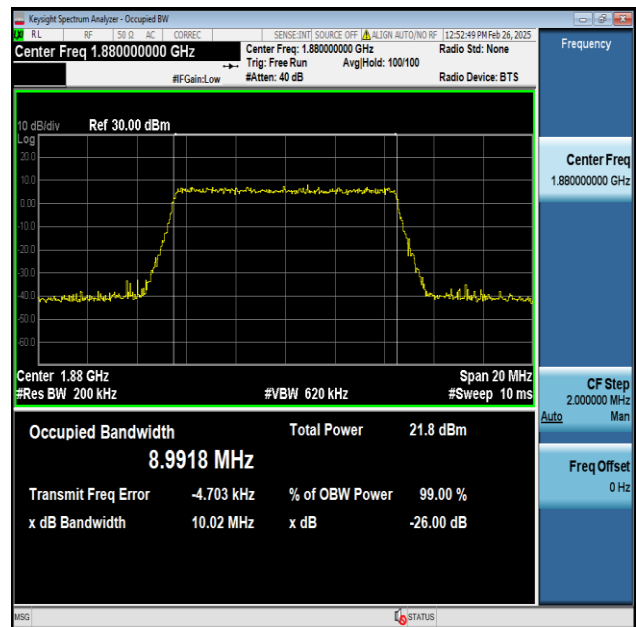
Band2-10MHz-256QAM-18900-50RB#0-PASS
