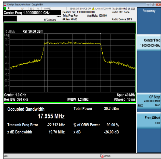
Band2-20MHz-16QAM-19100-100RB#0-PASS
