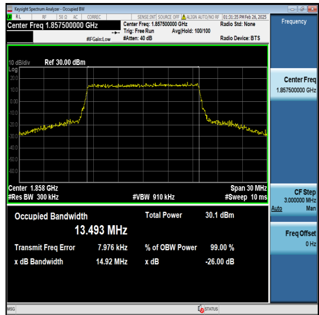
Band2-15MHz-16QAM-18675-75RB#0-PASS
