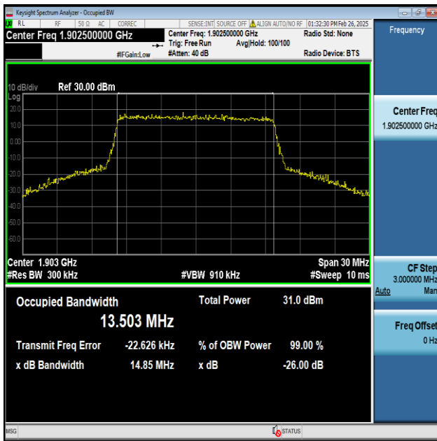
Band2-15MHz-QPSK-19125-75RB#0-PASS
