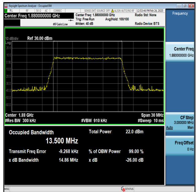
Band2-15MHz-256QAM-18900-75RB#0-PASS
