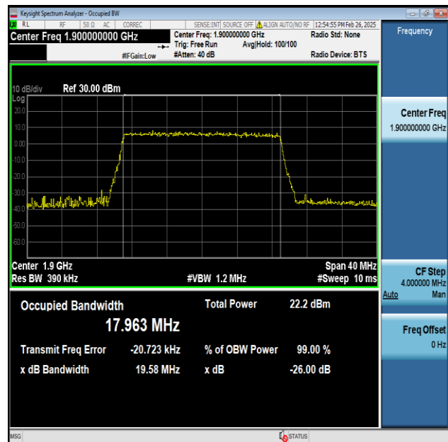
Band2-20MHz-256QAM-19100-100RB#0-PASS
