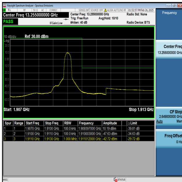
Band2-10MHz-QPSK-19150-1RB#49-PASS
