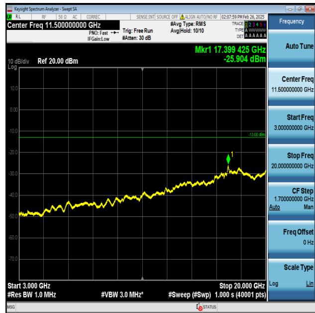
Band2-20MHz-QPSK-18900-1RB#0-3000~20000-PASS
