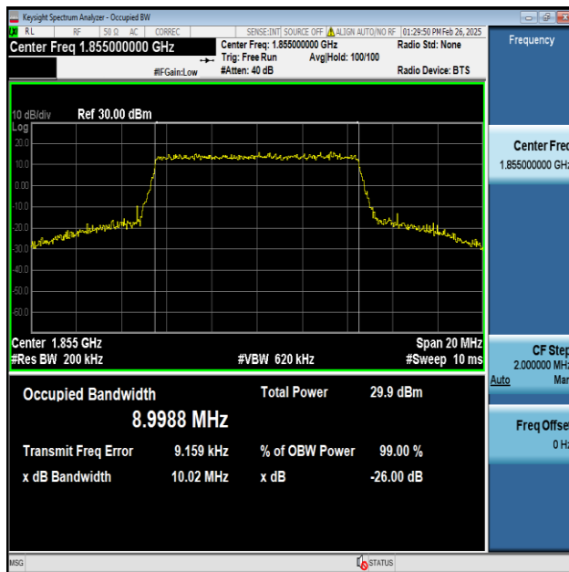
Band2-10MHz-64QAM-18650-50RB#0-PASS
