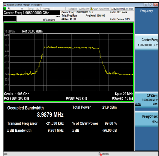
Band2-10MHz-256QAM-19150-50RB#0-PASS
