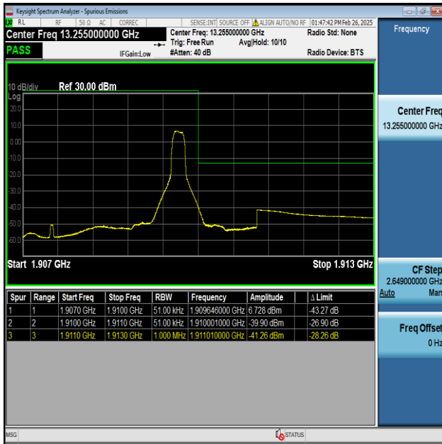
Band2-5MHz-QPSK-19175-1RB#24-PASS
