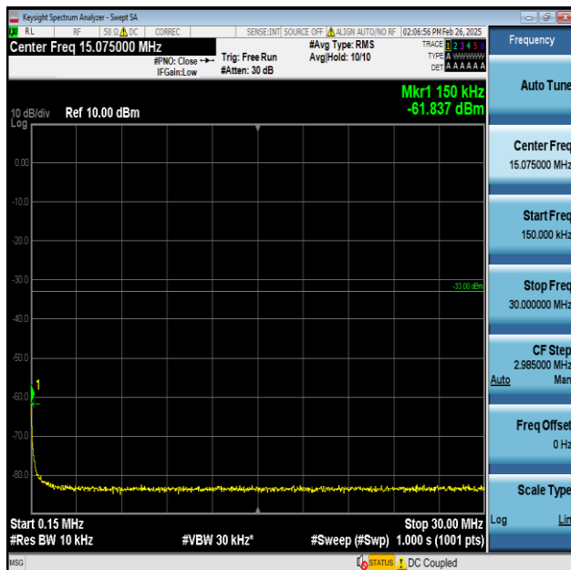
Band2-20MHz-QPSK-18900-1RB#0-0.15~30-PASS
