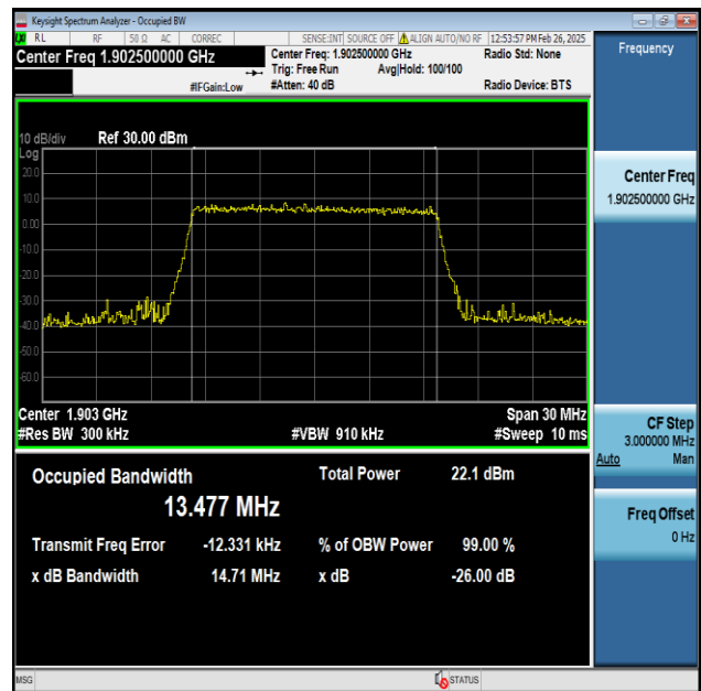
Band2-15MHz-256QAM-19125-75RB#0-PASS
