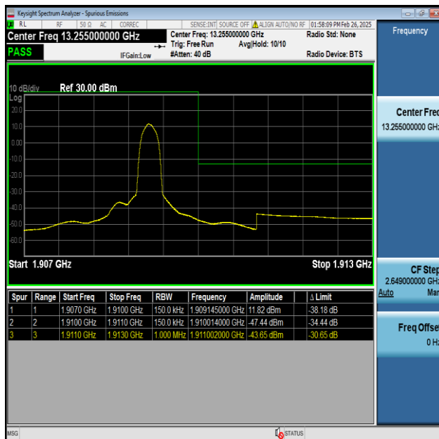
Band2-15MHz-QPSK-19125-1RB#74-PASS
