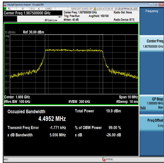
Band2-5MHz-16QAM-19175-25RB#0-PASS
