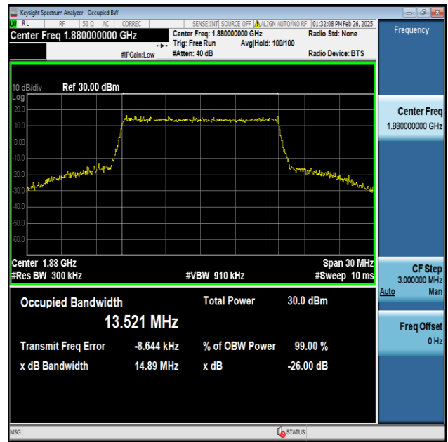
Band2-15MHz-16QAM-18900-75RB#0-PASS
