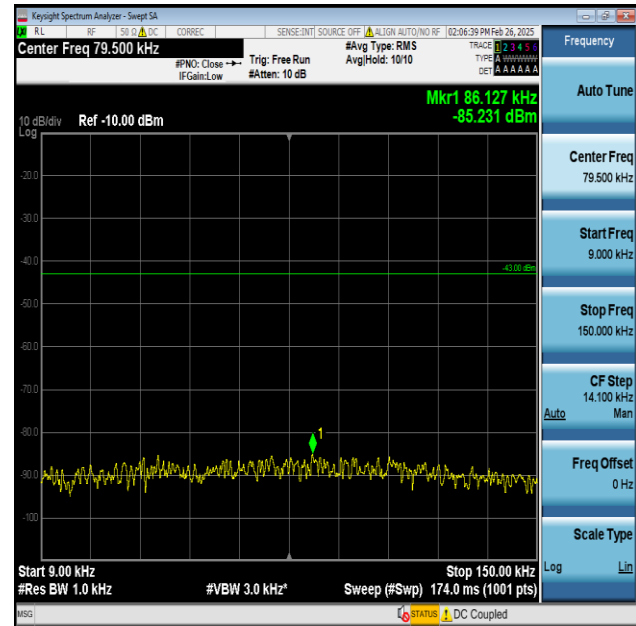
Band2-20MHz-QPSK-18900-1RB#0-0.009~0.15-PASS
