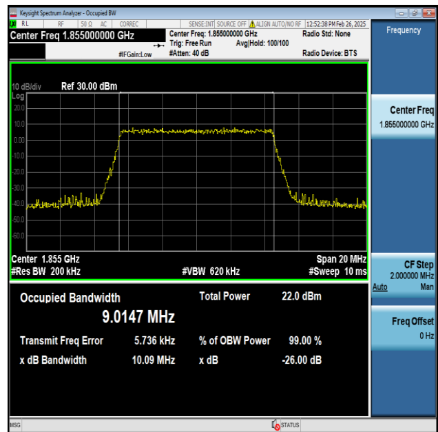
Band2-10MHz-256QAM-18650-50RB#0-PASS
