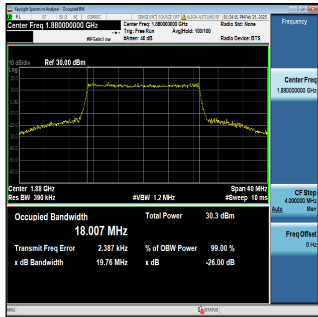
Band2-20MHz-16QAM-18900-100RB#0-PASS
