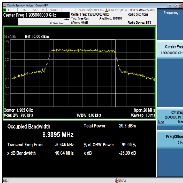
Band2-10MHz-64QAM-19150-50RB#0-PASS
