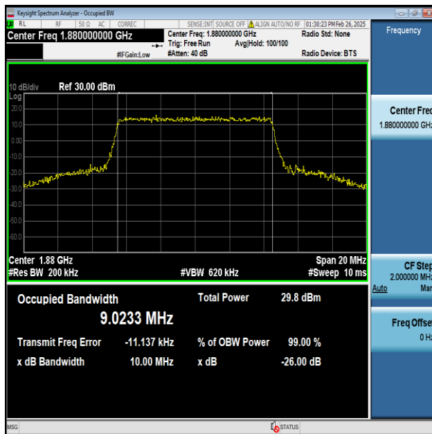
Band2-10MHz-64QAM-18900-50RB#0-PASS
