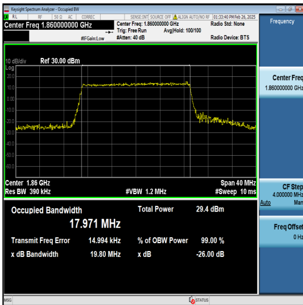
Band2-20MHz-64QAM-18700-100RB#0-PASS
