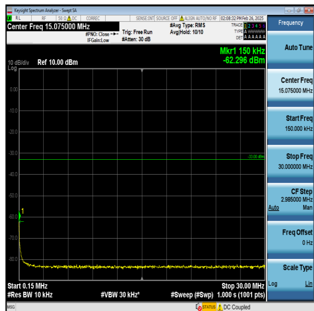
Band2-20MHz-QPSK-19100-1RB#0-0.15~30-PASS
