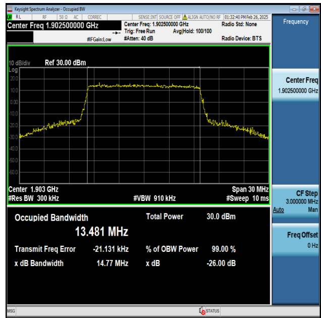
Band2-15MHz-16QAM-19125-75RB#0-PASS
