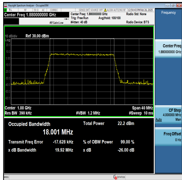
Band2-20MHz-256QAM-18900-100RB#0-PASS
