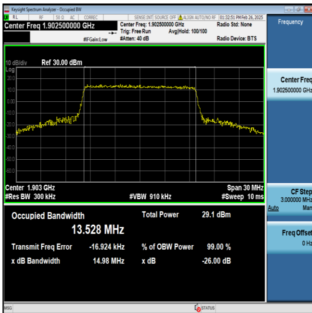
Band2-15MHz-64QAM-19125-75RB#0-PASS
