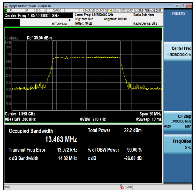
Band2-15MHz-256QAM-18675-75RB#0-PASS
