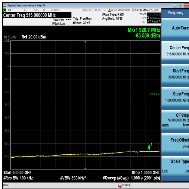
Band2-20MHz-QPSK-19100-1RB#0-30~1000-PASS
