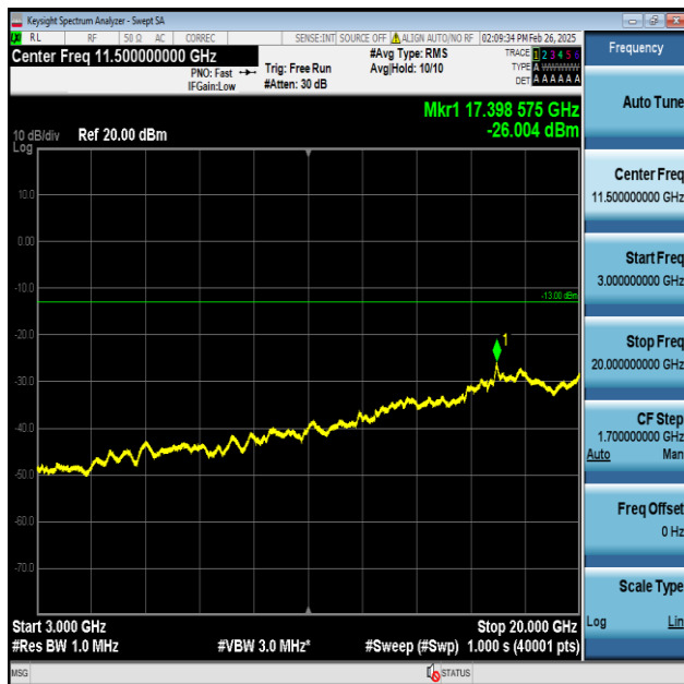
Band2-20MHz-QPSK-19100-1RB#0-3000~20000-PASS
