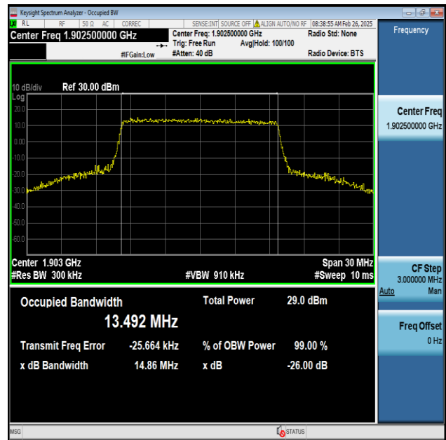
Band2-15MHz-16QAM-19125-75RB#0-PASS
