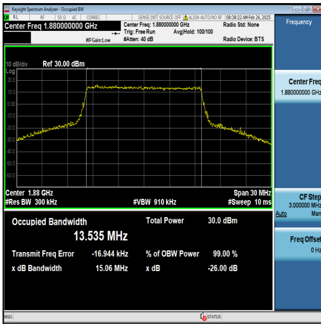
Band2-15MHz-QPSK-18900-75RB#0-PASS
