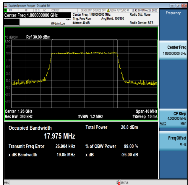
Band2-20MHz-256QAM-18700-100RB#0-PASS
