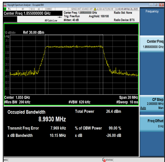
Band2-10MHz-256QAM-18650-50RB#0-PASS
