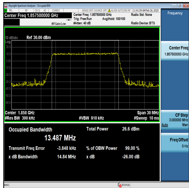
Band2-15MHz-256QAM-18675-75RB#0-PASS
