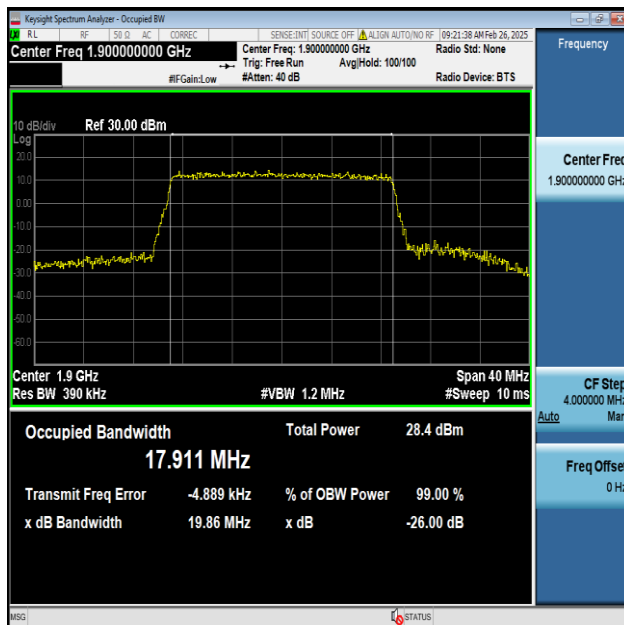
Band2-20MHz-64QAM-19100-100RB#0-PASS
