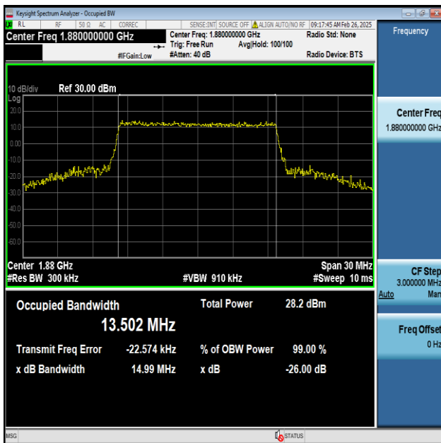
Band2-15MHz-64QAM-18900-75RB#0-PASS
