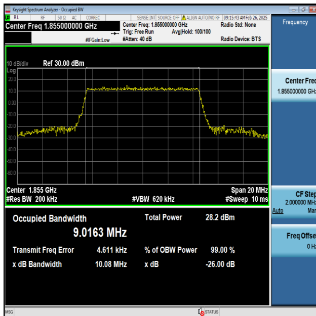
Band2-10MHz-64QAM-18650-50RB#0-PASS
