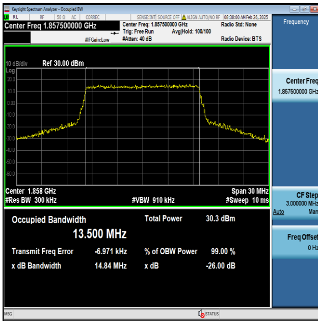
Band2-15MHz-QPSK-18675-75RB#0-PASS
