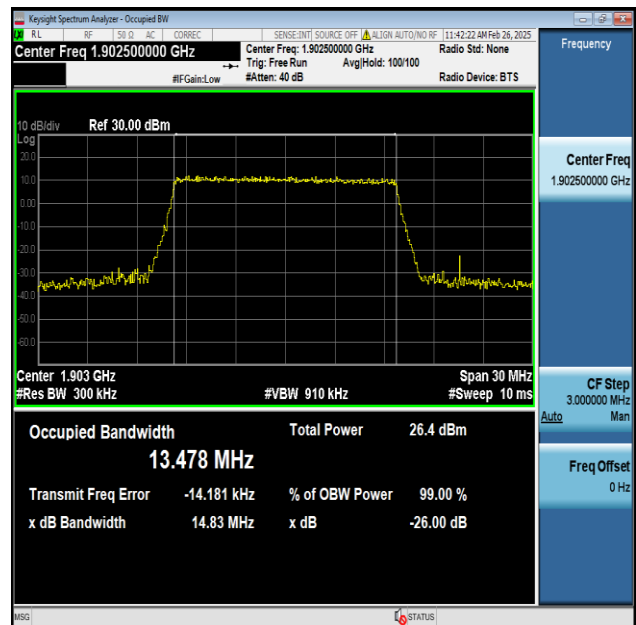
Band2-15MHz-256QAM-19125-75RB#0-PASS
