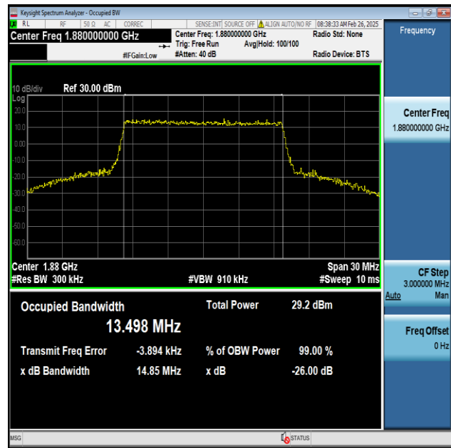
Band2-15MHz-16QAM-18900-75RB#0-PASS
