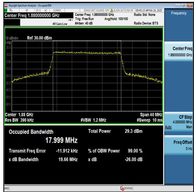
Band2-20MHz-16QAM-18900-100RB#0-PASS
