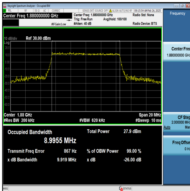
Band2-10MHz-64QAM-18900-50RB#0-PASS
