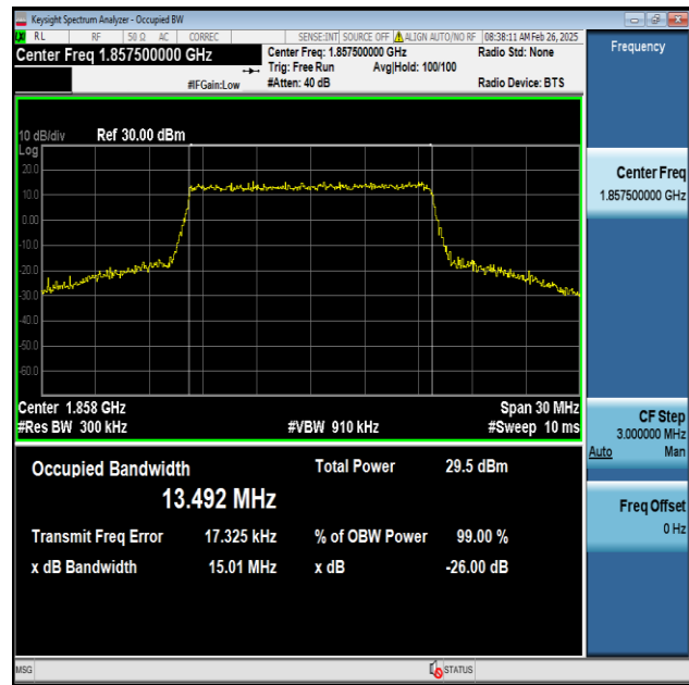
Band2-15MHz-16QAM-18675-75RB#0-PASS
