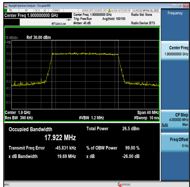
Band2-20MHz-256QAM-19100-100RB#0-PASS
