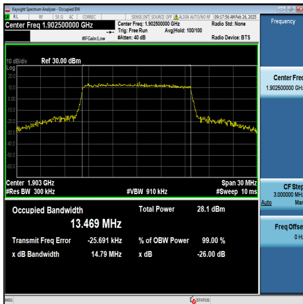
Band2-15MHz-64QAM-19125-75RB#0-PASS
