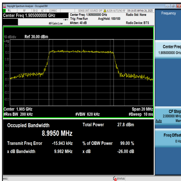
Band2-10MHz-64QAM-19150-50RB#0-PASS
