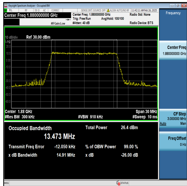
Band2-15MHz-256QAM-18900-75RB#0-PASS
