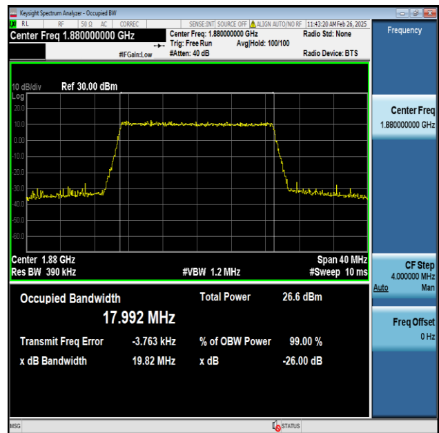
Band2-20MHz-256QAM-18900-100RB#0-PASS
