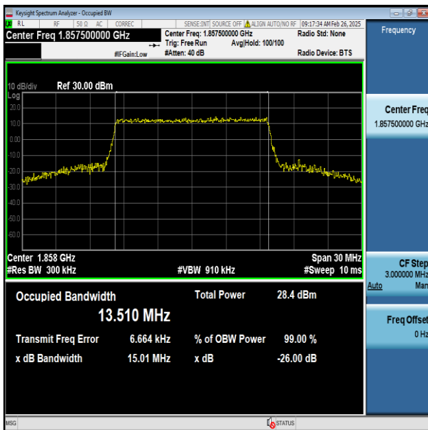
Band2-15MHz-64QAM-18675-75RB#0-PASS
