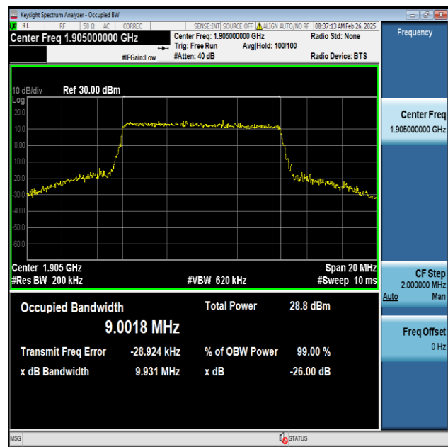
Band2-10MHz-16QAM-19150-50RB#0-PASS
