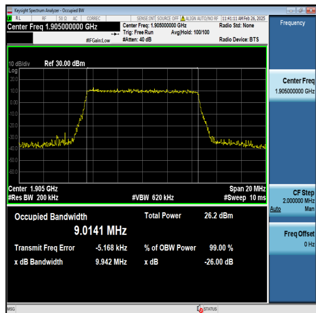
Band2-10MHz-256QAM-19150-50RB#0-PASS
