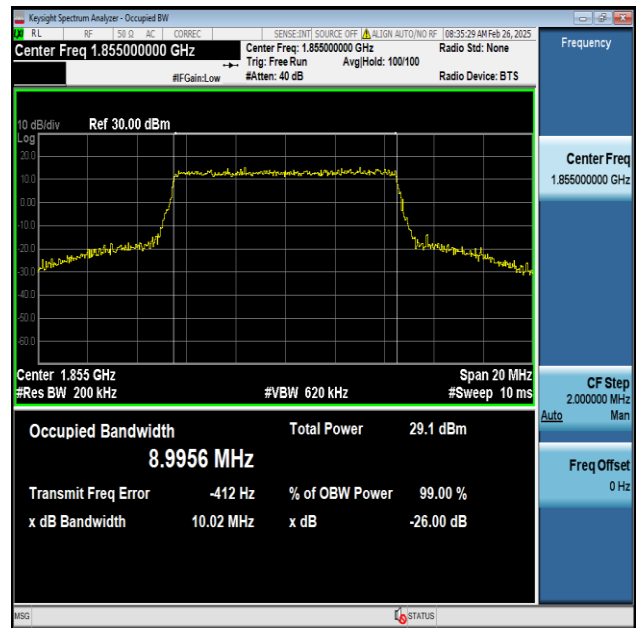
Band2-10MHz-16QAM-18650-50RB#0-PASS
