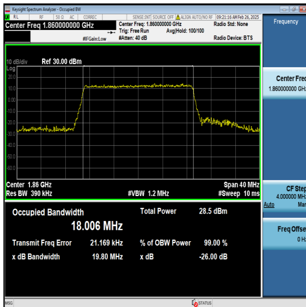
Band2-20MHz-64QAM-18700-100RB#0-PASS
