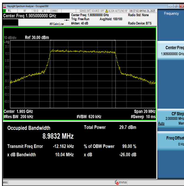
Band2-10MHz-QPSK-19150-50RB#0-PASS
