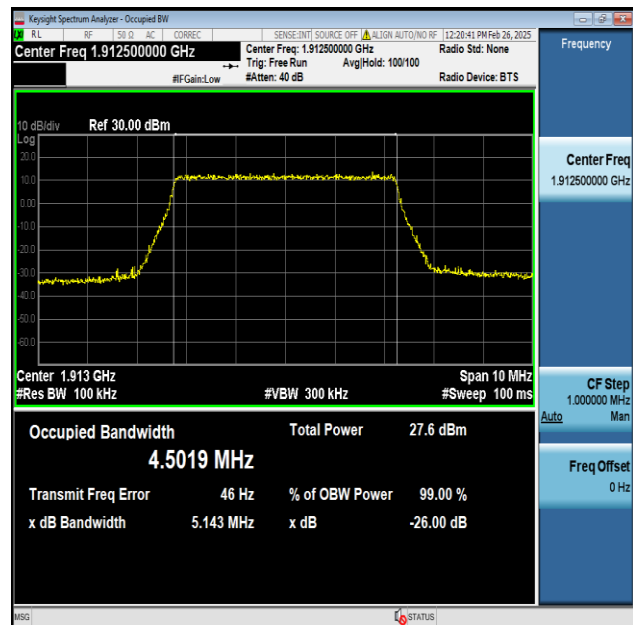
Band25-5MHz-256QAM-26665-25RB#0-PASS
