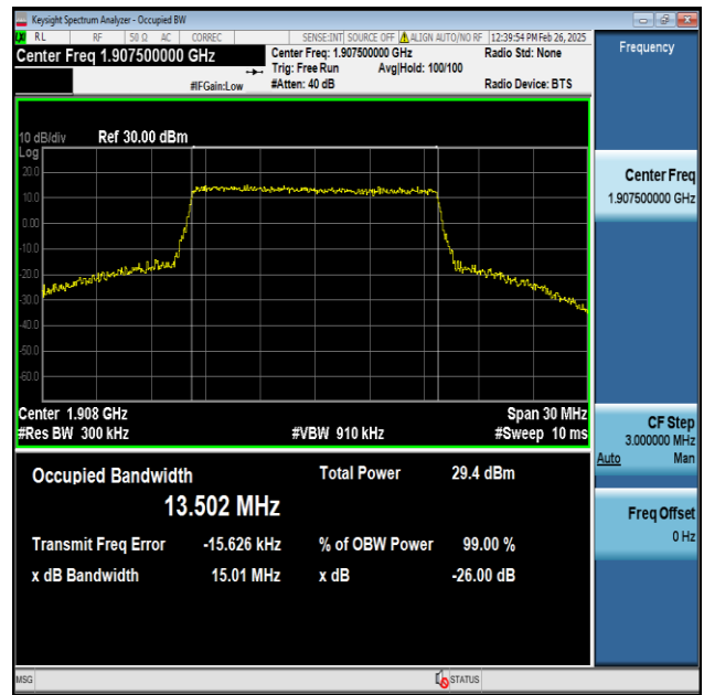
Band25-15MHz-16QAM-26615-75RB#0-PASS
