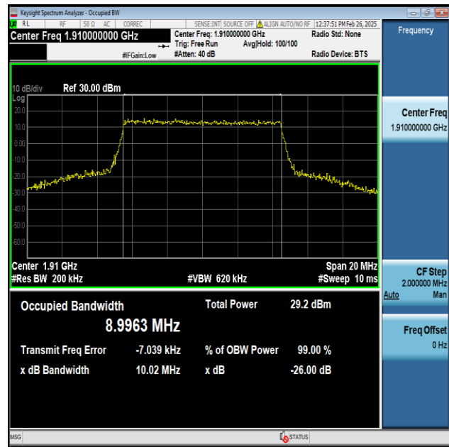
Band25-10MHz-16QAM-26640-50RB#0-PASS
