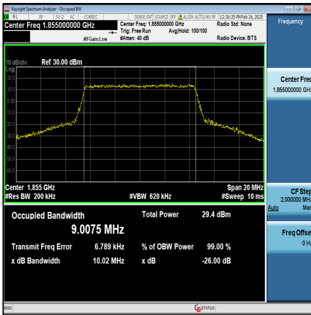
Band25-10MHz-QPSK-26090-50RB#0-PASS
