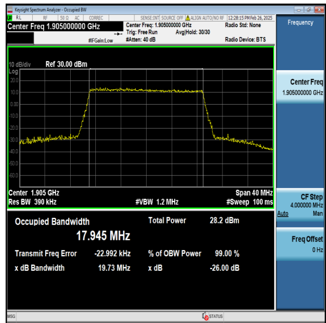
Band25-20MHz-256QAM-26590-100RB#0-PASS
