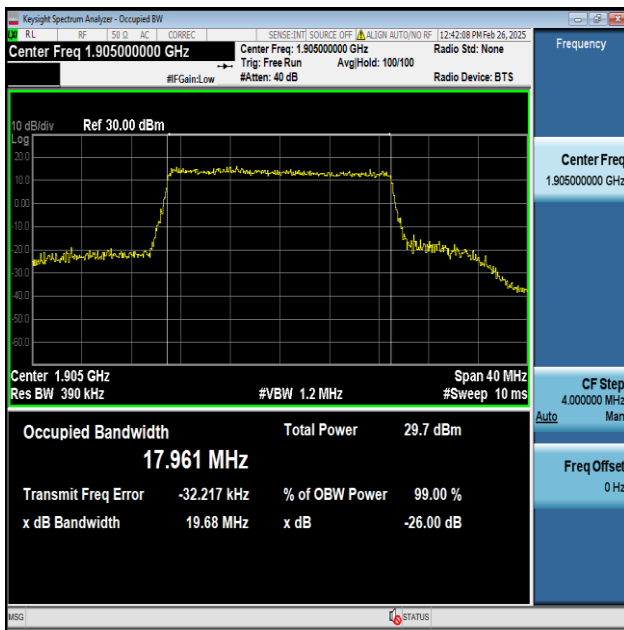
Band25-20MHz-64QAM-26590-100RB#0-PASS
