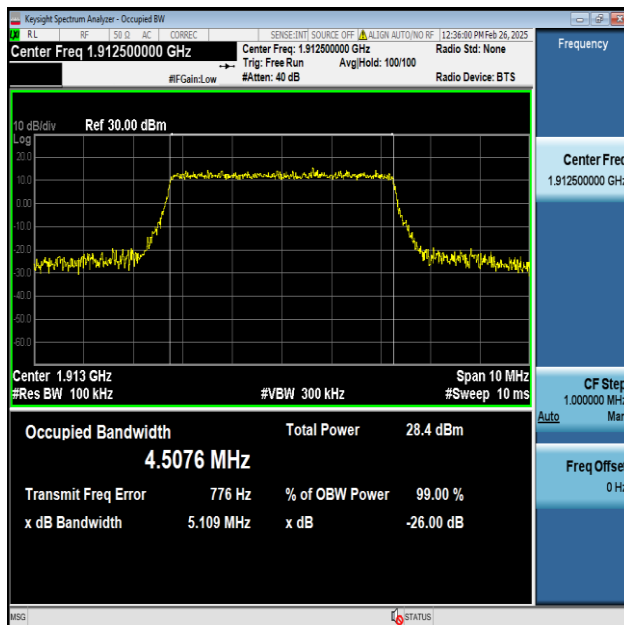
Band25-5MHz-64QAM-26665-25RB#0-PASS
