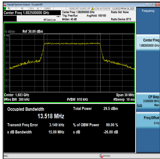
Band25-15MHz-16QAM-26365-75RB#0-PASS
