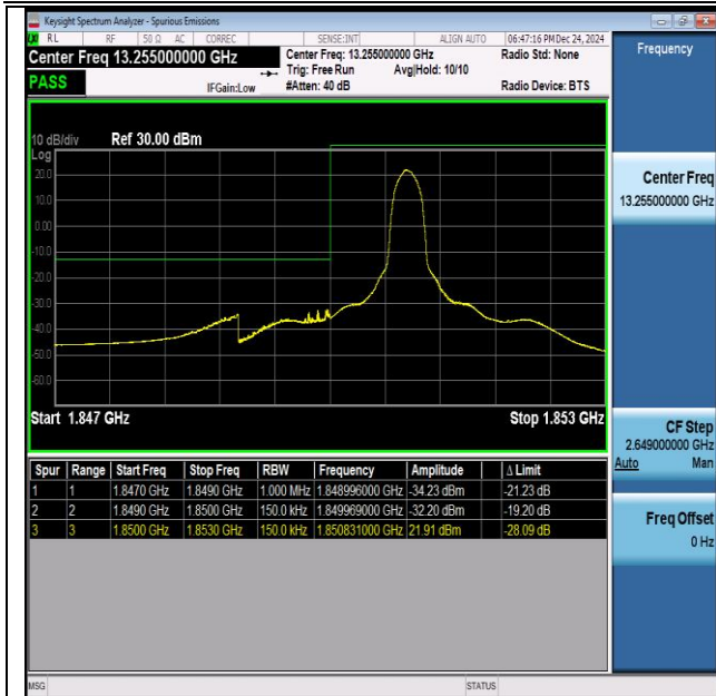
Band25-15MHz-QPSK-26115-1RB#0-PASS
