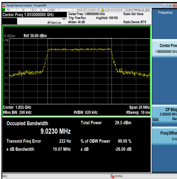
Band25-10MHz-64QAM-26090-50RB#0-PASS
