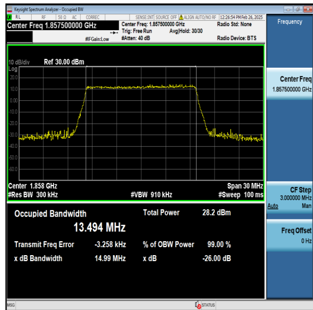
Band25-15MHz-256QAM-26115-75RB#0-PASS
