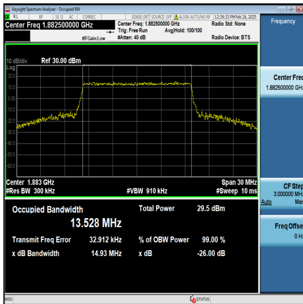
Band25-15MHz-64QAM-26365-75RB#0-PASS
