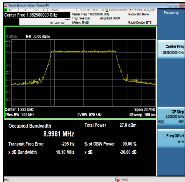
Band25-10MHz-256QAM-26365-50RB#0-PASS
