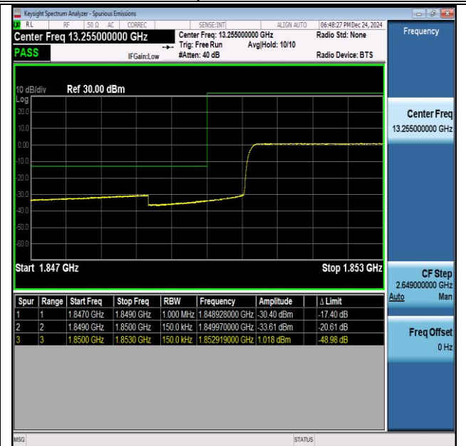
Band25-15MHz-QPSK-26115-75RB#0-PASS
