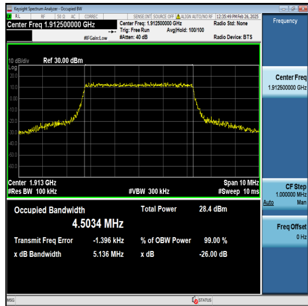
Band25-5MHz-16QAM-26665-25RB#0-PASS
