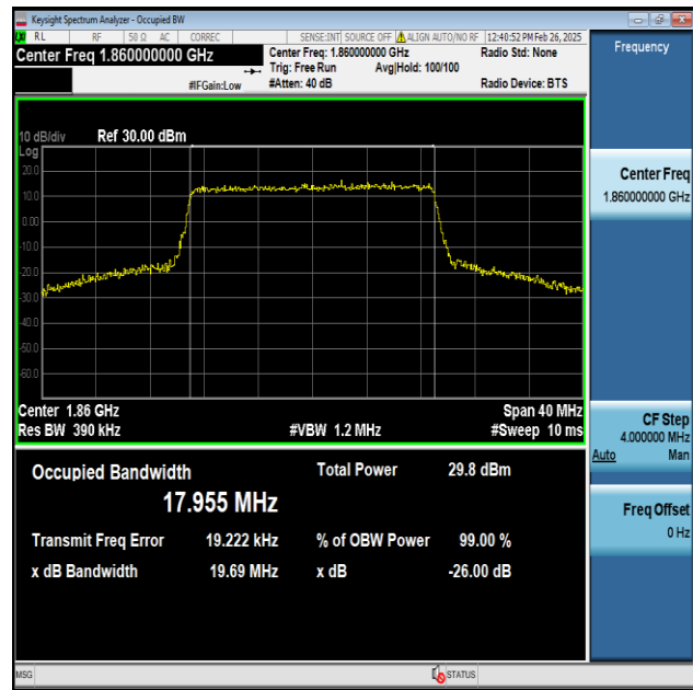
Band25-20MHz-16QAM-26140-100RB#0-PASS
