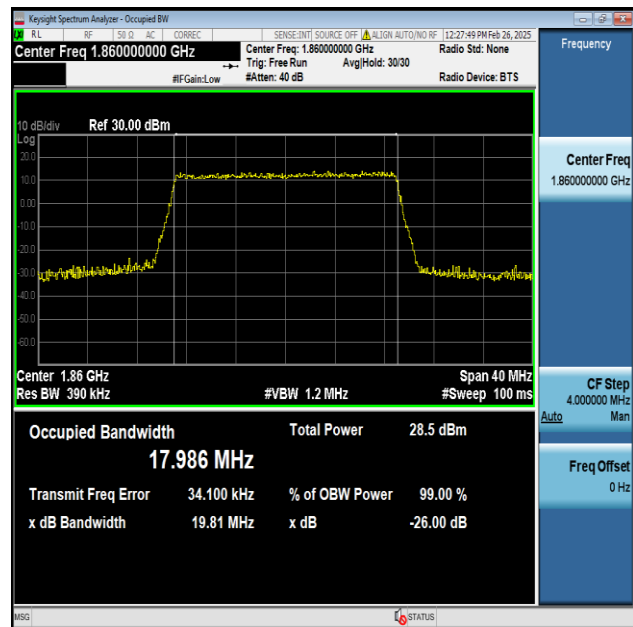
Band25-20MHz-256QAM-26140-100RB#0-PASS
