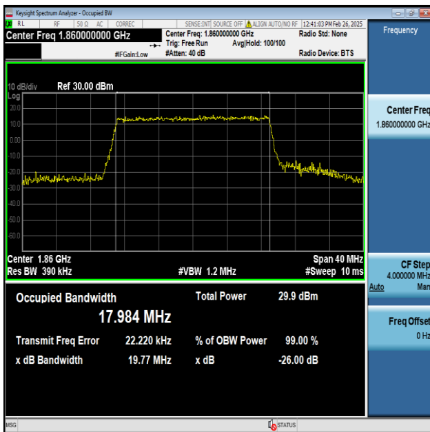
Band25-20MHz-64QAM-26140-100RB#0-PASS
