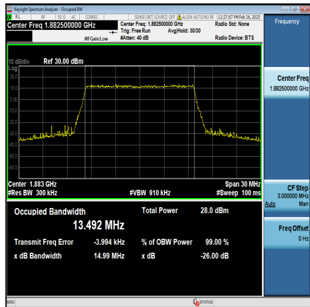
Band25-15MHz-256QAM-26365-75RB#0-PASS
