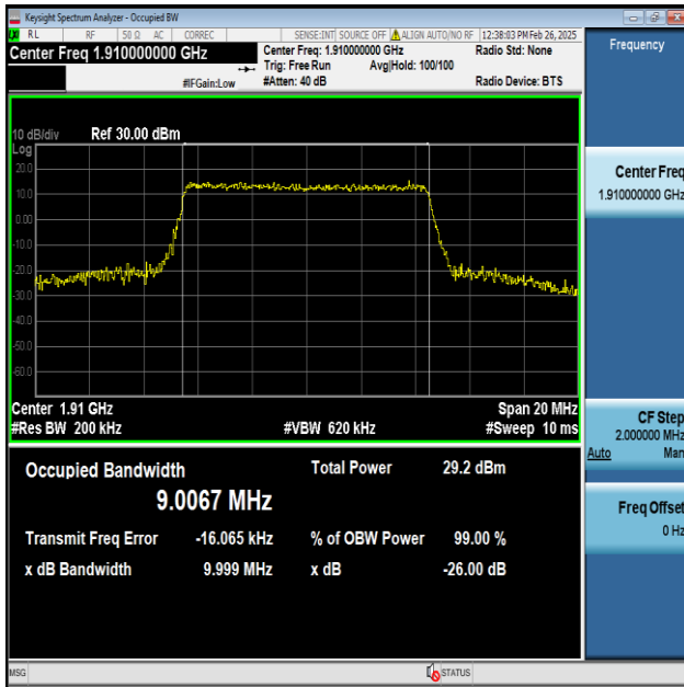
Band25-10MHz-64QAM-26640-50RB#0-PASS
