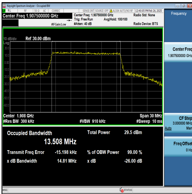
Band25-15MHz-64QAM-26615-75RB#0-PASS
