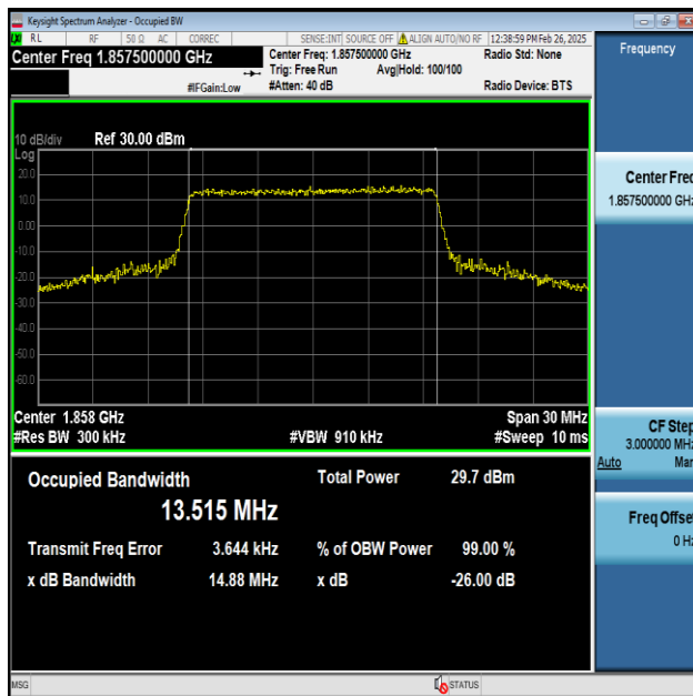
Band25-15MHz-64QAM-26115-75RB#0-PASS
