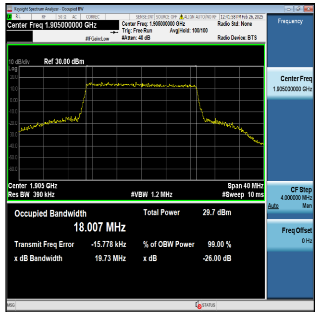
Band25-20MHz-16QAM-26590-100RB#0-PASS
