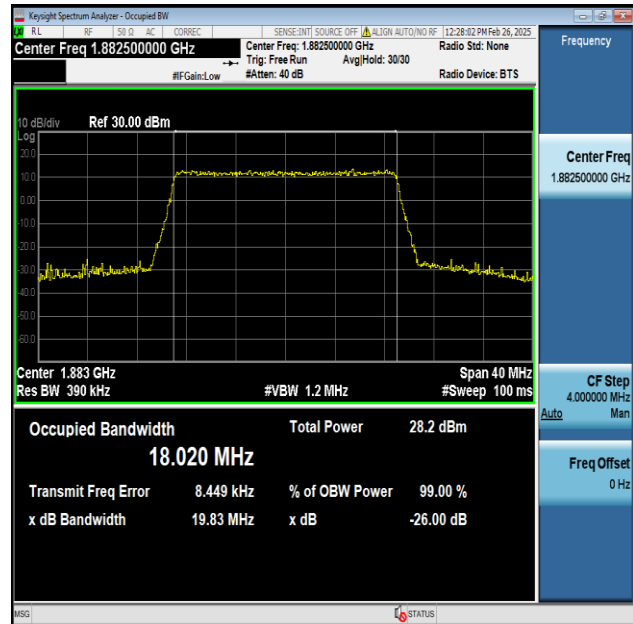
Band25-20MHz-256QAM-26365-100RB#0-PASS
