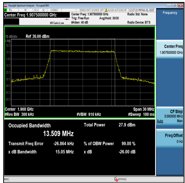
Band25-15MHz-256QAM-26615-75RB#0-PASS
