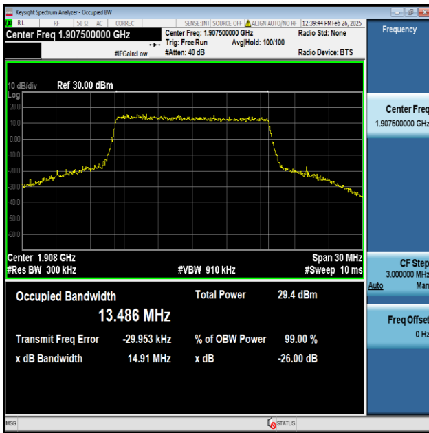
Band25-15MHz-QPSK-26615-75RB#0-PASS
