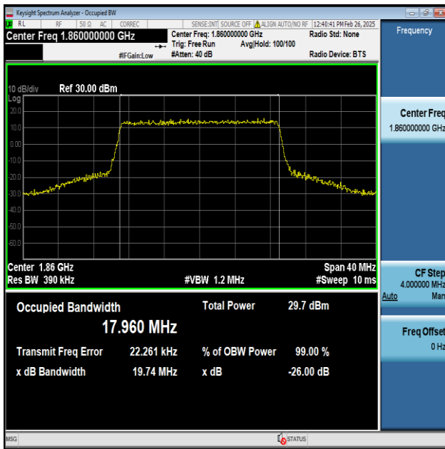
Band25-20MHz-QPSK-26140-100RB#0-PASS
