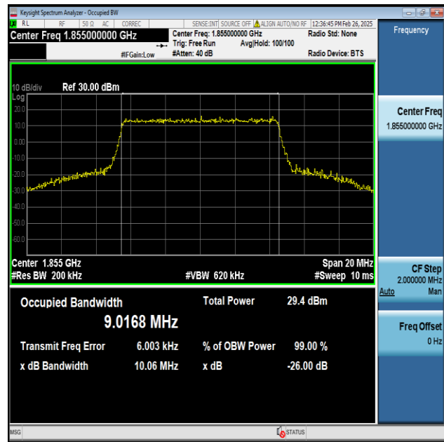
Band25-10MHz-16QAM-26090-50RB#0-PASS
