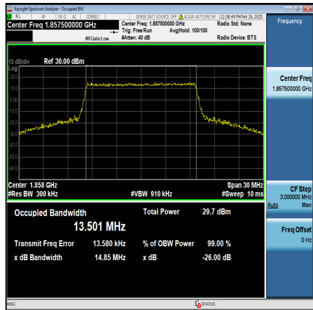
Band25-15MHz-16QAM-26115-75RB#0-PASS
