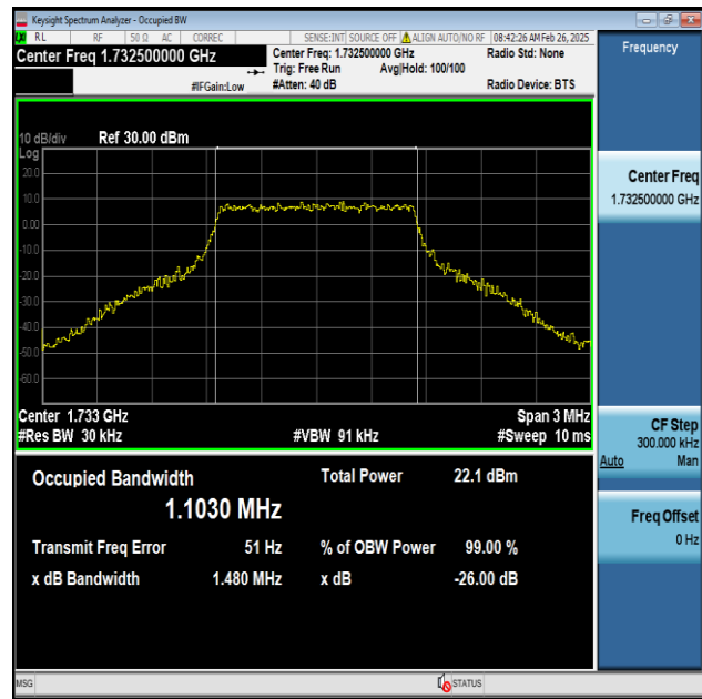
Band4-1.4MHz-16QAM-20175-6RB#0-PASS
