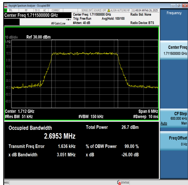
Band4-3MHz-256QAM-19965-15RB#0-PASS
