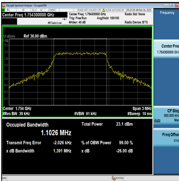
Band4-1.4MHz-64QAM-20393-6RB#0-PASS
