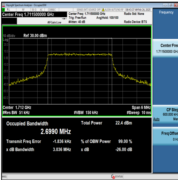
Band4-3MHz-QPSK-19965-15RB#0-PASS
