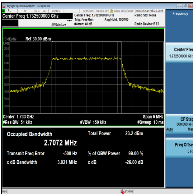
Band4-3MHz-64QAM-20175-15RB#0-PASS
