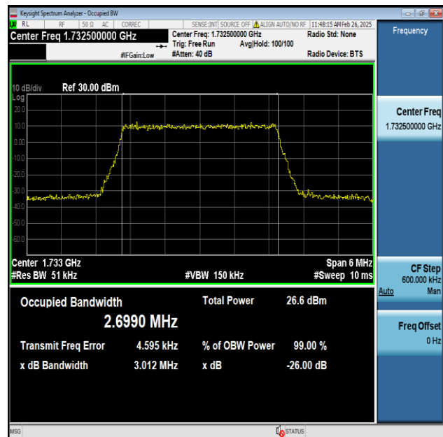
Band4-3MHz-256QAM-20175-15RB#0-PASS
