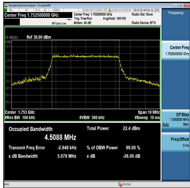
Band4-5MHz-16QAM-20375-25RB#0-PASS
