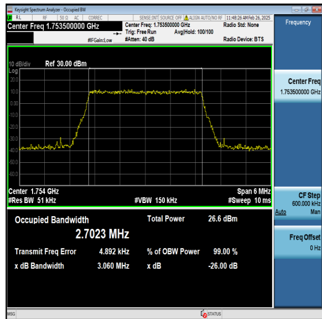
Band4-3MHz-256QAM-20385-15RB#0-PASS
