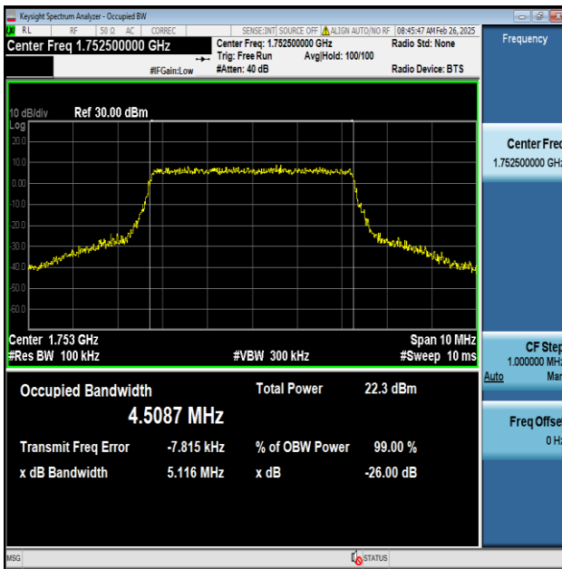
Band4-5MHz-QPSK-20375-25RB#0-PASS
