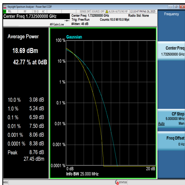
Band4-20MHz-256QAM-20175-100RB#0-PASS
