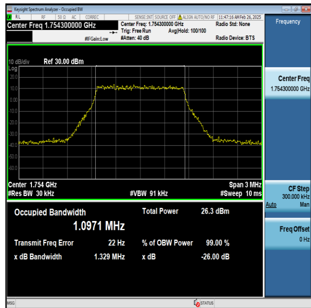
Band4-1.4MHz-256QAM-20393-6RB#0-PASS
