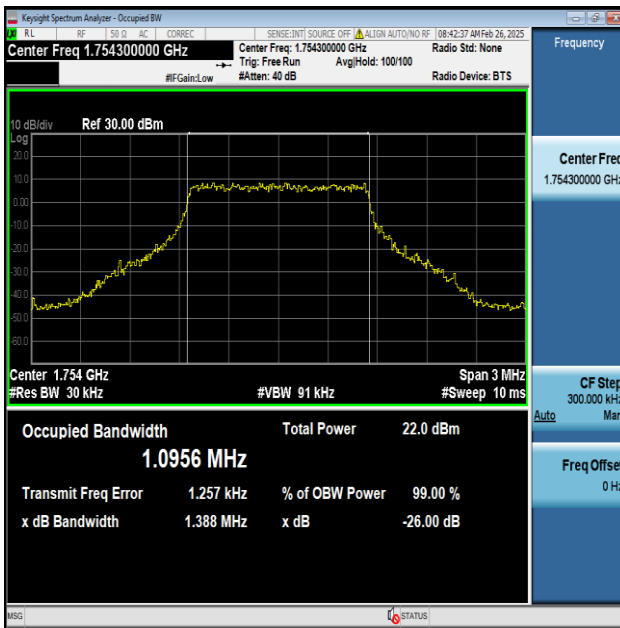
Band4-1.4MHz-QPSK-20393-6RB#0-PASS
