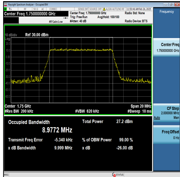
Band4-10MHz-256QAM-20350-50RB#0-PASS
