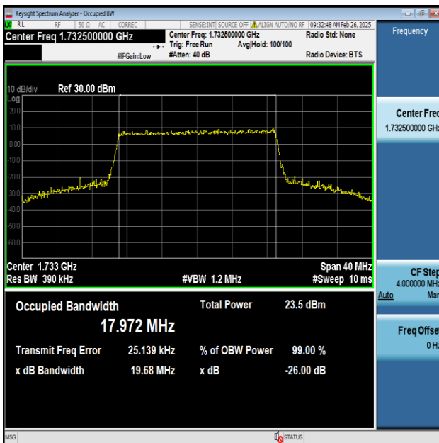
Band4-20MHz-64QAM-20175-100RB#0-PASS
