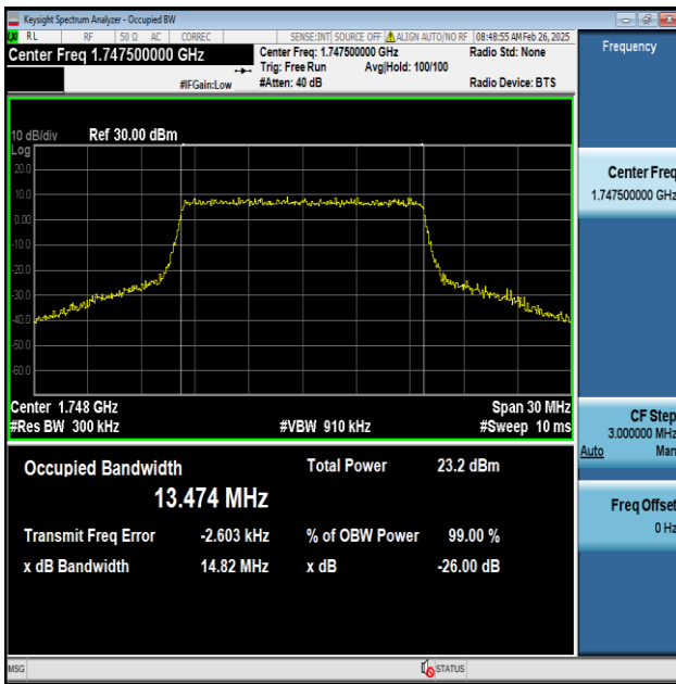
Band4-15MHz-QPSK-20325-75RB#0-PASS
