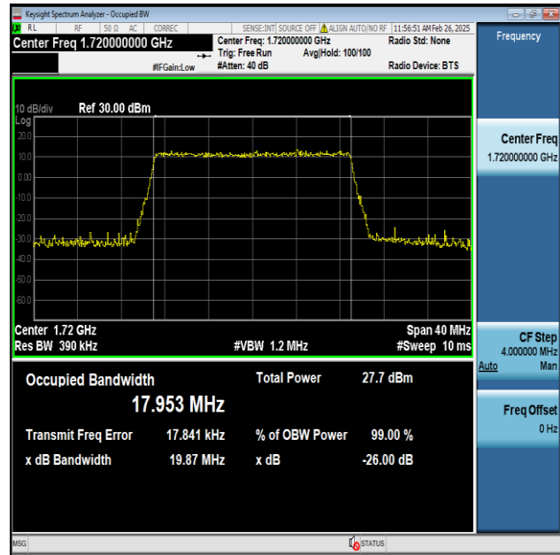
Band4-20MHz-256QAM-20050-100RB#0-PASS
