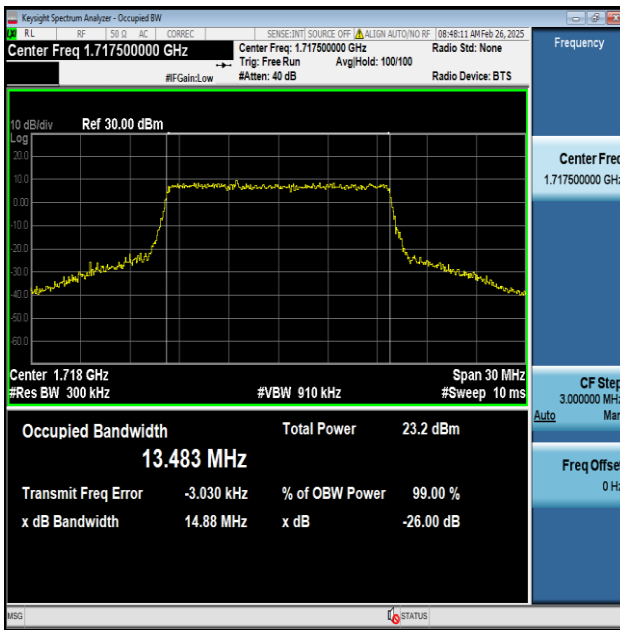
Band4-15MHz-QPSK-20025-75RB#0-PASS
