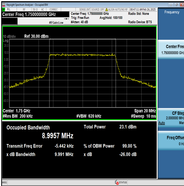
Band4-10MHz-QPSK-20350-50RB#0-PASS
