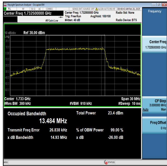
Band4-15MHz-16QAM-20175-75RB#0-PASS
