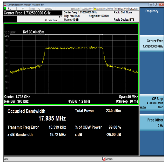
Band4-20MHz-16QAM-20175-100RB#0-PASS
