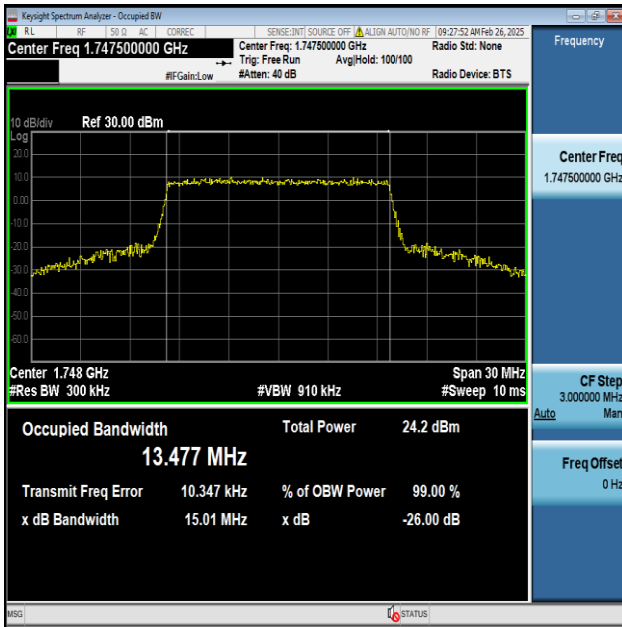
Band4-15MHz-64QAM-20325-75RB#0-PASS
