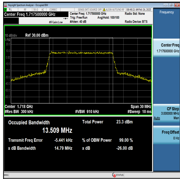
Band4-15MHz-16QAM-20025-75RB#0-PASS
