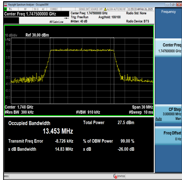
Band4-15MHz-256QAM-20325-75RB#0-PASS
