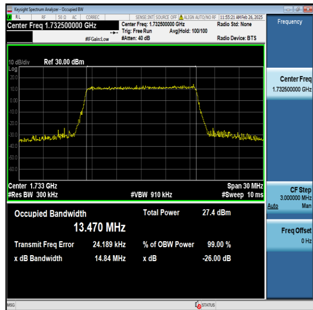
Band4-15MHz-256QAM-20175-75RB#0-PASS
