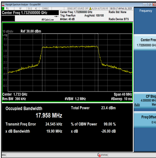
Band4-20MHz-QPSK-20175-100RB#0-PASS
