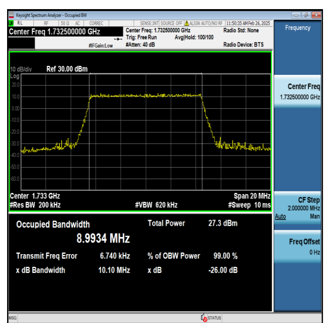
Band4-10MHz-256QAM-20175-50RB#0-PASS
