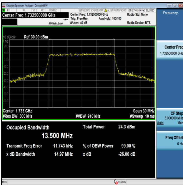
Band4-15MHz-64QAM-20175-75RB#0-PASS
