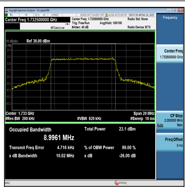
Band4-10MHz-16QAM-20175-50RB#0-PASS
