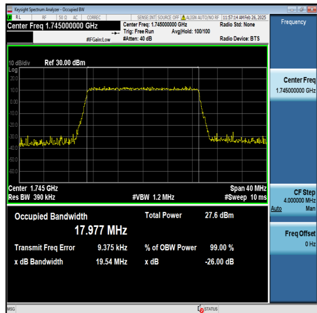
Band4-20MHz-256QAM-20300-100RB#0-PASS
