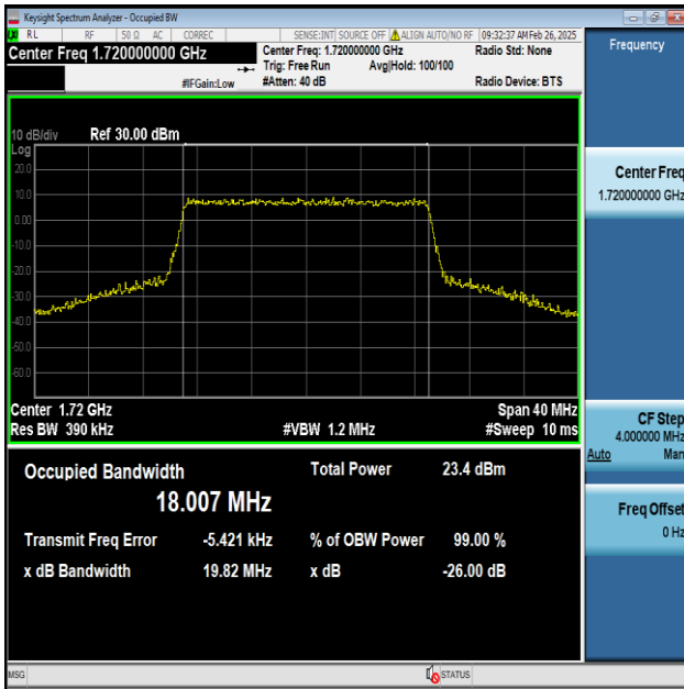
Band4-20MHz-64QAM-20050-100RB#0-PASS
