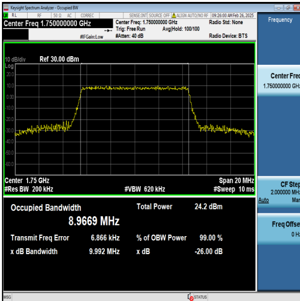
Band4-10MHz-64QAM-20350-50RB#0-PASS
