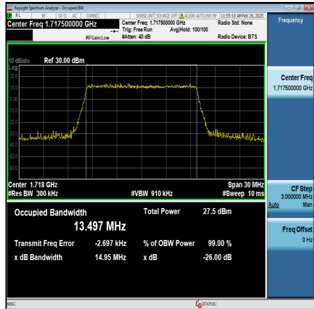
Band4-15MHz-256QAM-20025-75RB#0-PASS
