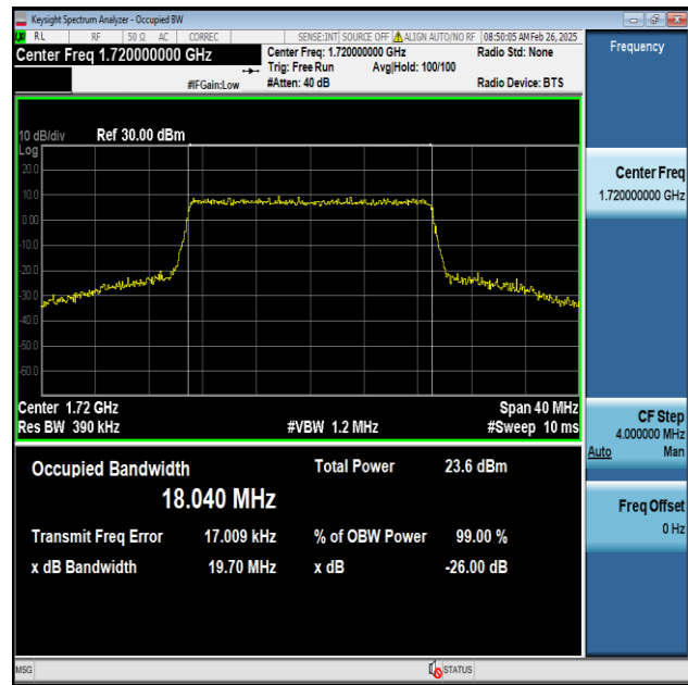
Band4-20MHz-16QAM-20050-100RB#0-PASS
