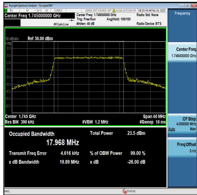
Band4-20MHz-16QAM-20300-100RB#0-PASS
