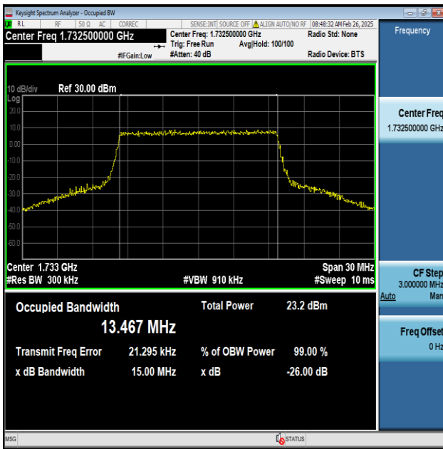
Band4-15MHz-QPSK-20175-75RB#0-PASS
