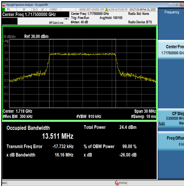
Band4-15MHz-64QAM-20025-75RB#0-PASS
