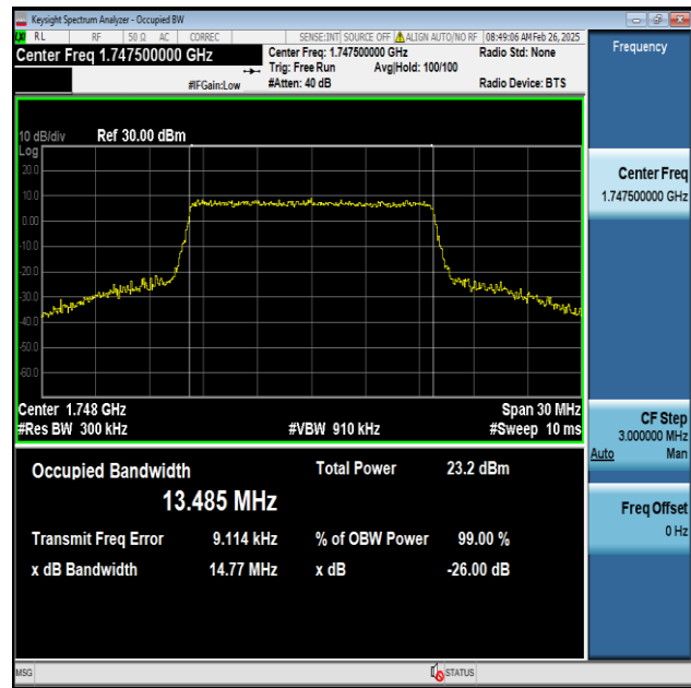
Band4-15MHz-16QAM-20325-75RB#0-PASS
