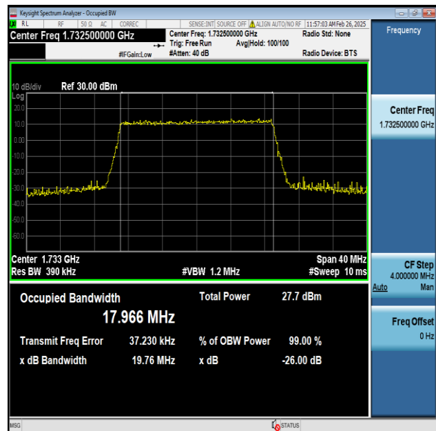
Band4-20MHz-256QAM-20175-100RB#0-PASS
