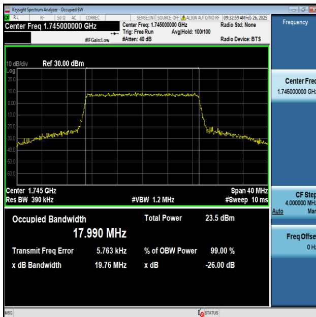
Band4-20MHz-64QAM-20300-100RB#0-PASS
