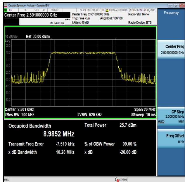
Band41-10MHz-256QAM-39700-50RB#0-PASS
