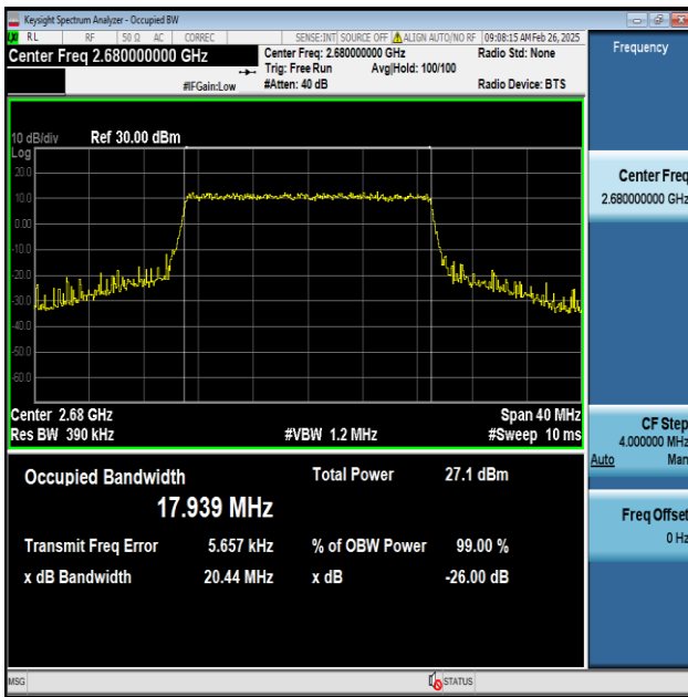
Band41-20MHz-QPSK-41490-100RB#0-PASS
