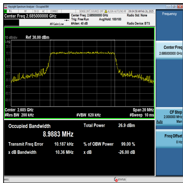
Band41-10MHz-16QAM-41540-50RB#0-PASS
