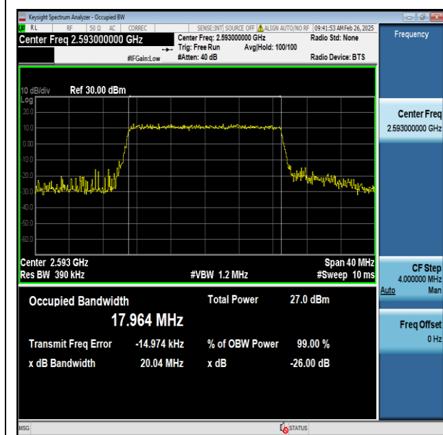
Band41-20MHz-64QAM-40620-100RB#0-PASS
