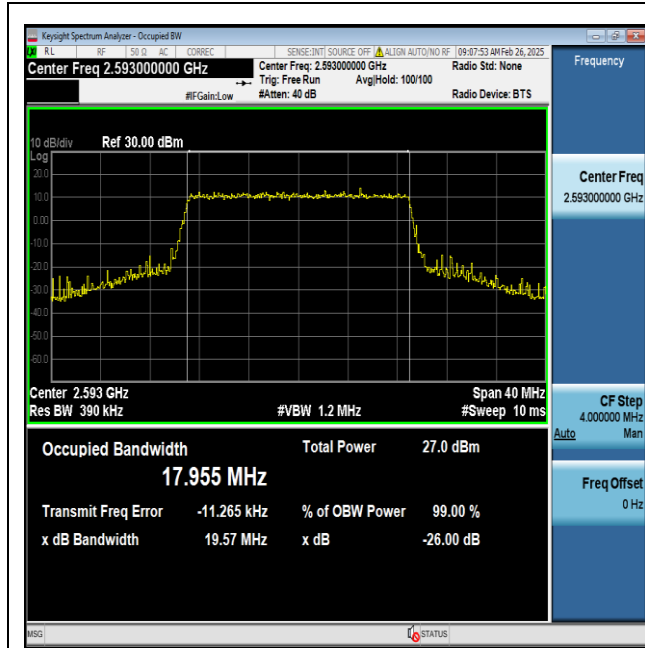
Band41-20MHz-QPSK-40620-100RB#0-PASS
