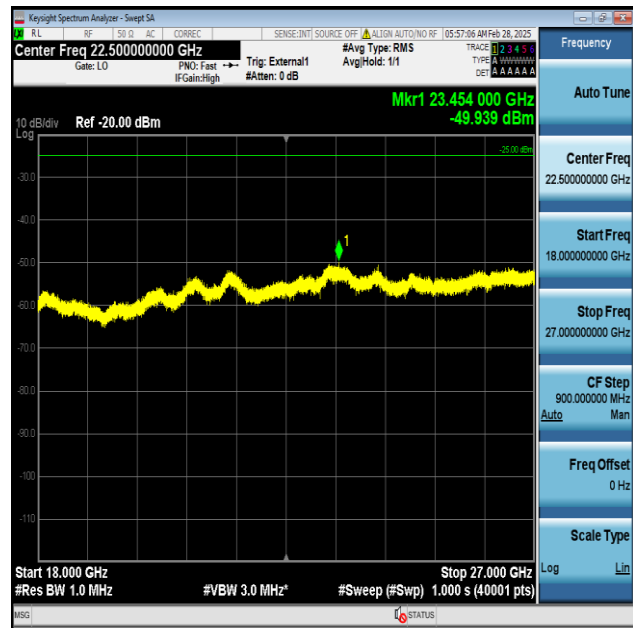
Band41-20MHz-QPSK-39750-1RB#0-18000~27000-PASS
