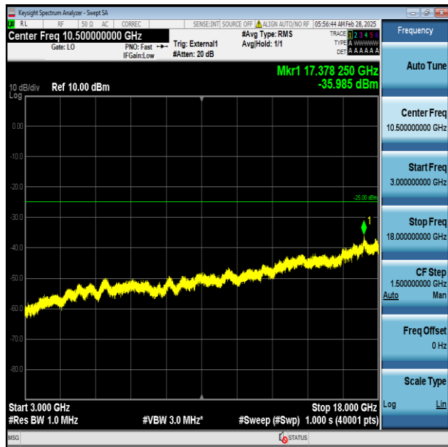
Band41-20MHz-QPSK-39750-1RB#0-3000~18000-PASS
