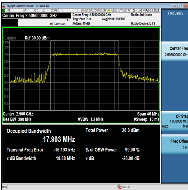
Band41-20MHz-64QAM-39750-100RB#0-PASS
