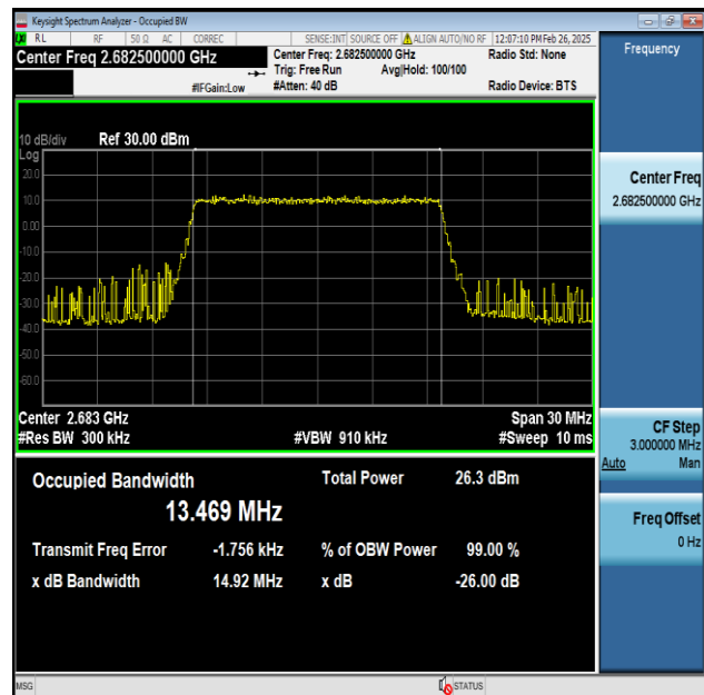
Band41-15MHz-256QAM-41515-75RB#0-PASS
