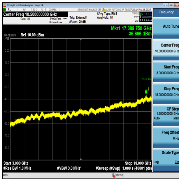
Band41-20MHz-QPSK-40620-1RB#0-3000~18000-PASS
