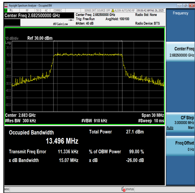
Band41-15MHz-16QAM-41515-75RB#0-PASS
