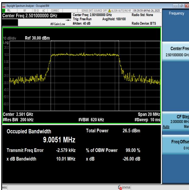
Band41-10MHz-64QAM-39700-50RB#0-PASS
