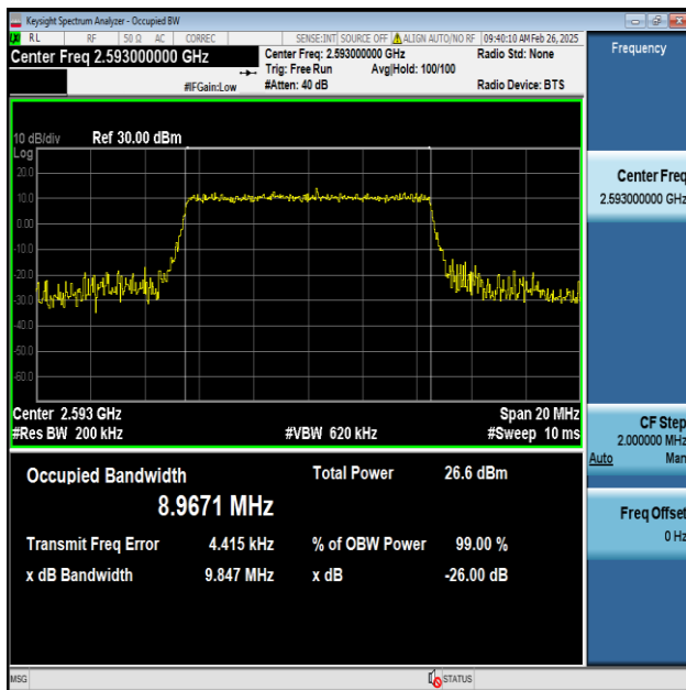
Band41-10MHz-64QAM-40620-50RB#0-PASS
