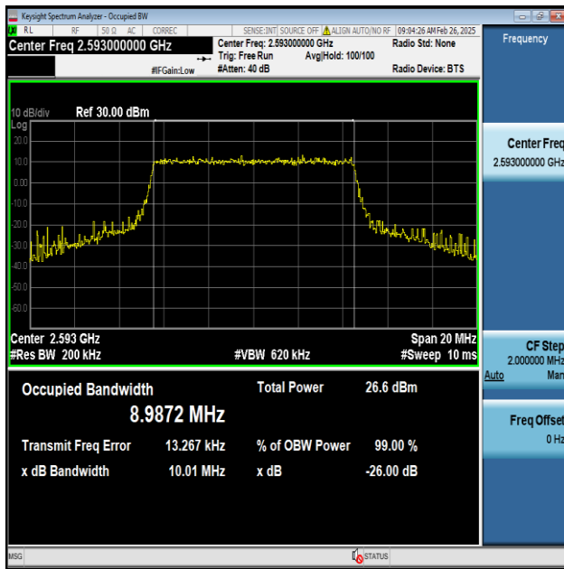
Band41-10MHz-QPSK-40620-50RB#0-PASS
