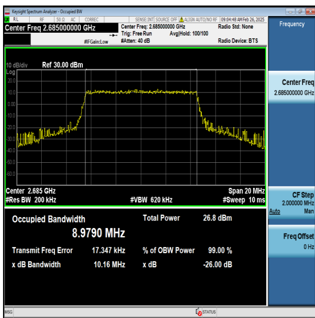
Band41-10MHz-QPSK-41540-50RB#0-PASS
