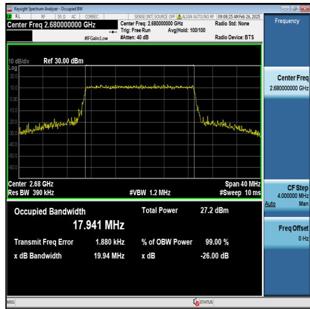
Band41-20MHz-16QAM-41490-100RB#0-PASS
