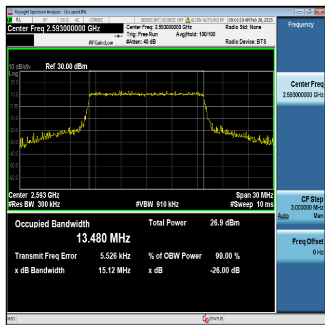
Band41-15MHz-16QAM-40620-75RB#0-PASS
