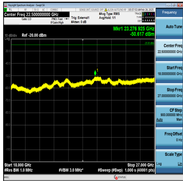
Band41-20MHz-QPSK-40620-1RB#0-18000~27000-PASS
