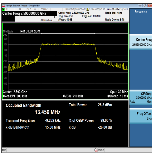
Band41-15MHz-QPSK-40620-75RB#0-PASS
