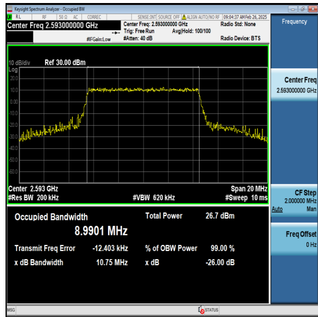
Band41-10MHz-16QAM-40620-50RB#0-PASS
