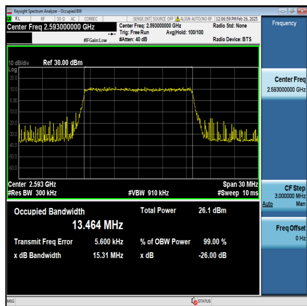
Band41-15MHz-256QAM-40620-75RB#0-PASS
