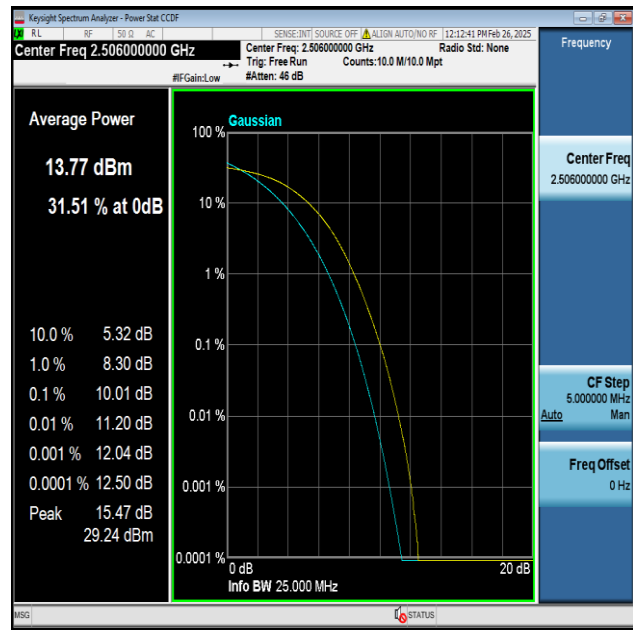
Band41-20MHz-256QAM-39750-100RB#0-PASS
