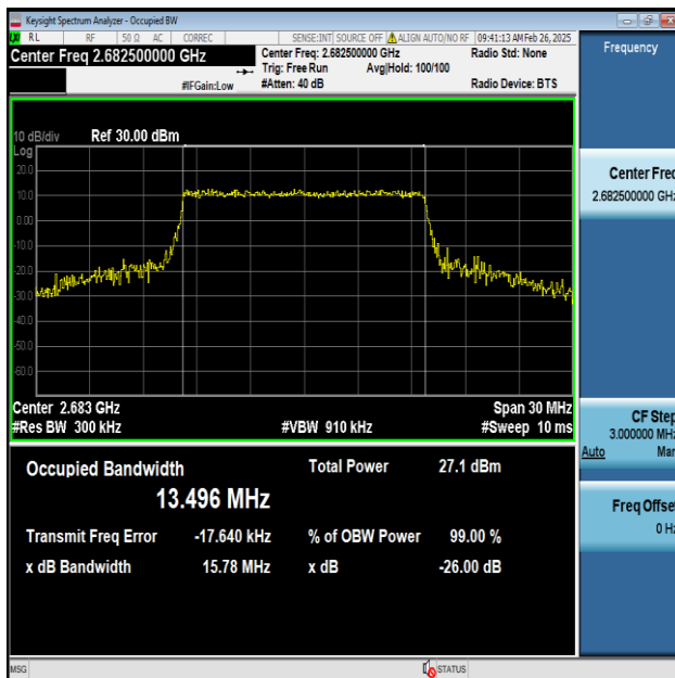
Band41-15MHz-64QAM-41515-75RB#0-PASS
