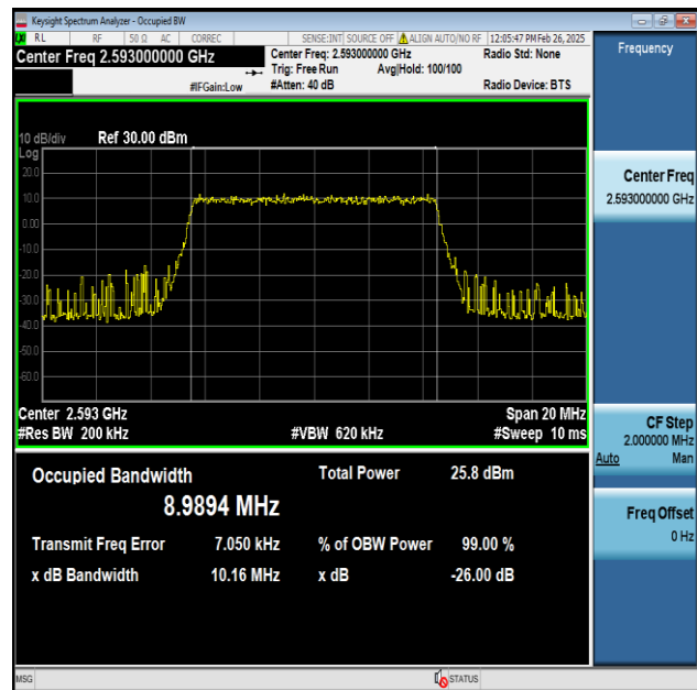
Band41-10MHz-256QAM-40620-50RB#0-PASS
