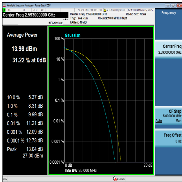
Band41-20MHz-256QAM-40620-100RB#0-PASS
