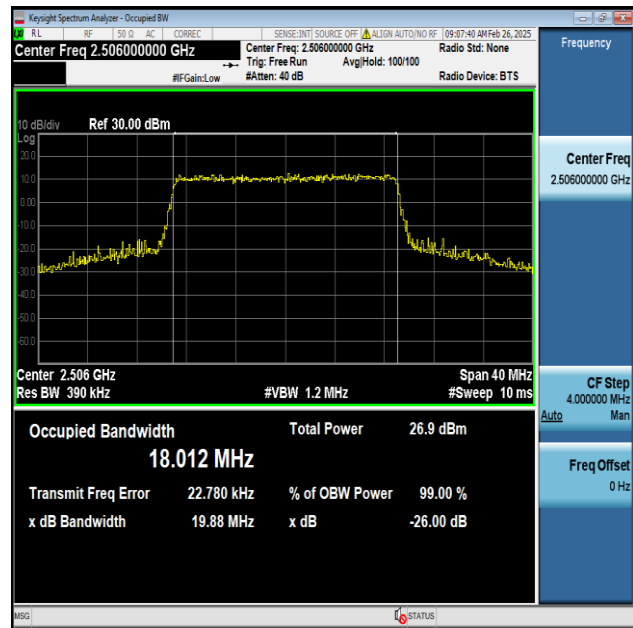
Band41-20MHz-16QAM-39750-100RB#0-PASS
