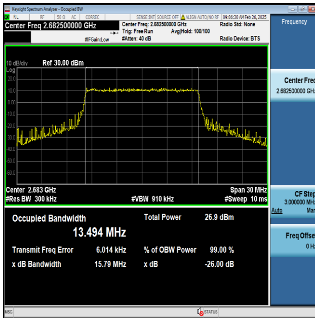
Band41-15MHz-QPSK-41515-75RB#0-PASS
