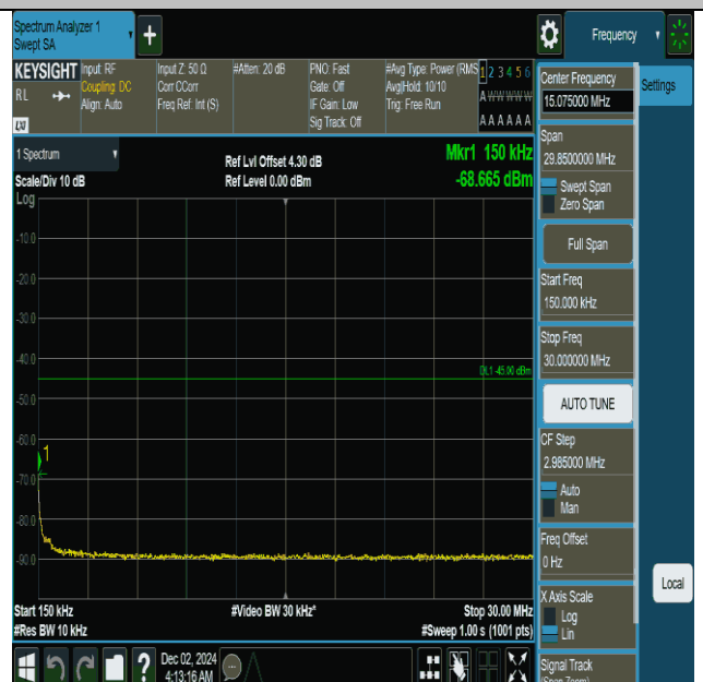
Band41-20MHz-QPSK-41490-1RB#0-0.15~30-PASS
