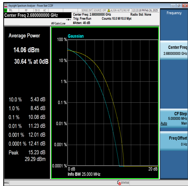
Band41-20MHz-256QAM-41490-100RB#0-PASS
