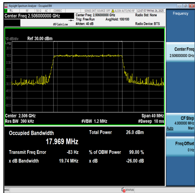
Band41-20MHz-256QAM-39750-100RB#0-PASS
