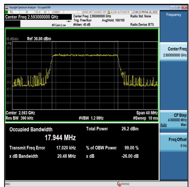
Band41-20MHz-256QAM-40620-100RB#0-PASS
