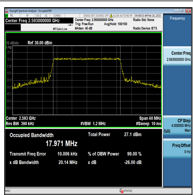
Band41-20MHz-16QAM-40620-100RB#0-PASS
