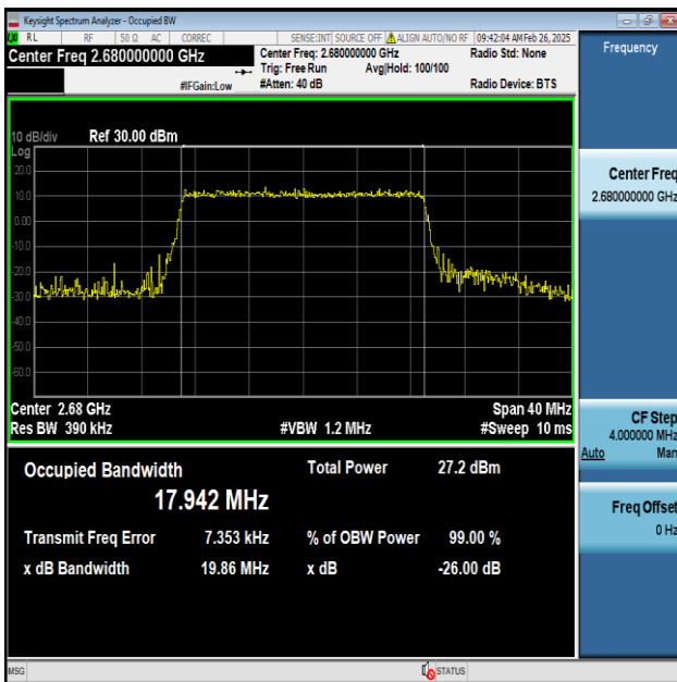
Band41-20MHz-64QAM-41490-100RB#0-PASS
