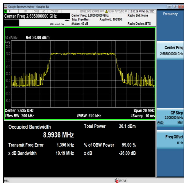
Band41-10MHz-256QAM-41540-50RB#0-PASS
