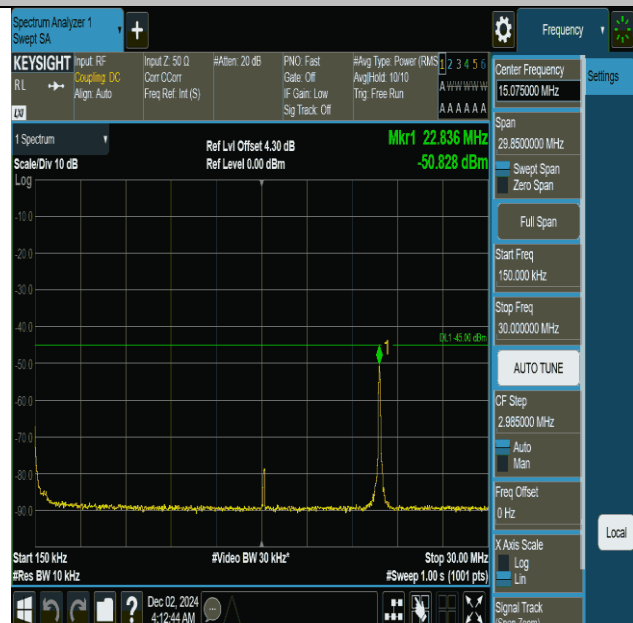
Band41-20MHz-QPSK-40620-1RB#0-0.15~30-PASS
