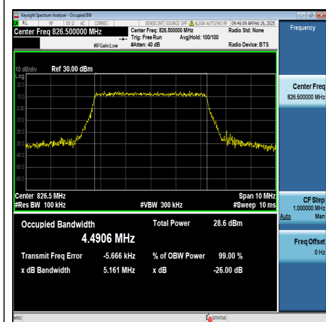
Band5-5MHz-64QAM-20425-25RB#0-PASS
