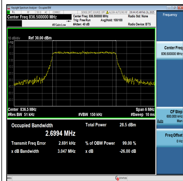
Band5-3MHz-64QAM-20525-15RB#0-PASS
