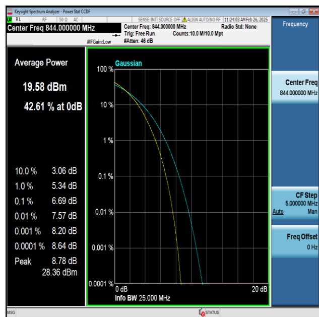
Band5-10MHz-256QAM-20600-50RB#0-PASS
