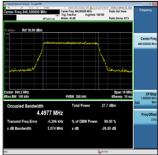
Band5-5MHz-256QAM-20625-25RB#0-PASS
