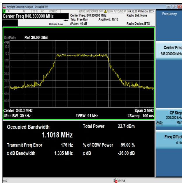
Band5-1.4MHz-64QAM-20643-6RB#0-PASS
