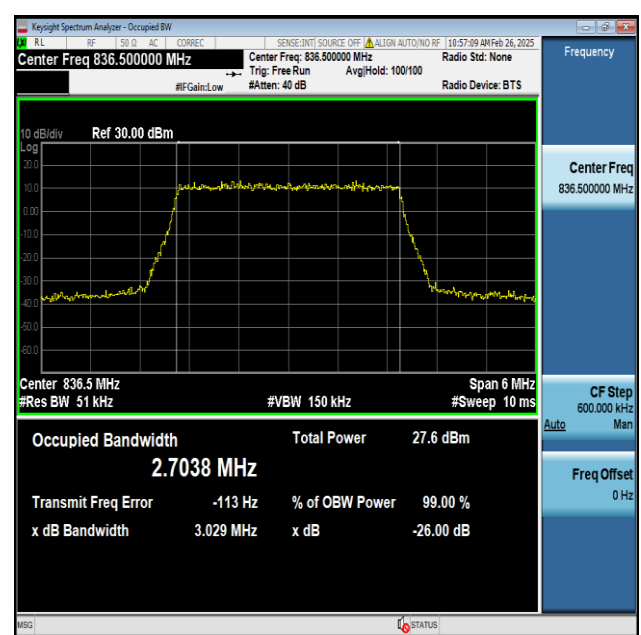
Band5-3MHz-256QAM-20525-15RB#0-PASS
