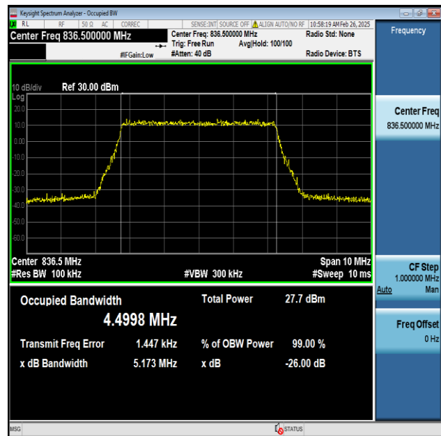
Band5-5MHz-256QAM-20525-25RB#0-PASS
