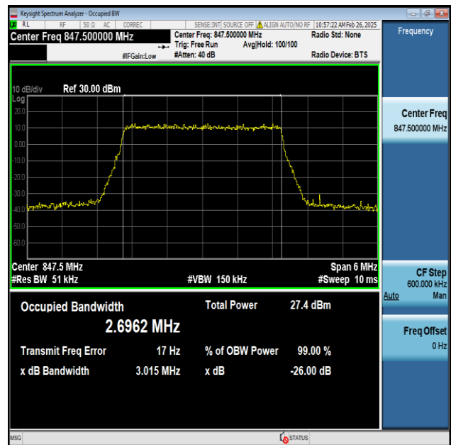
Band5-3MHz-256QAM-20635-15RB#0-PASS
