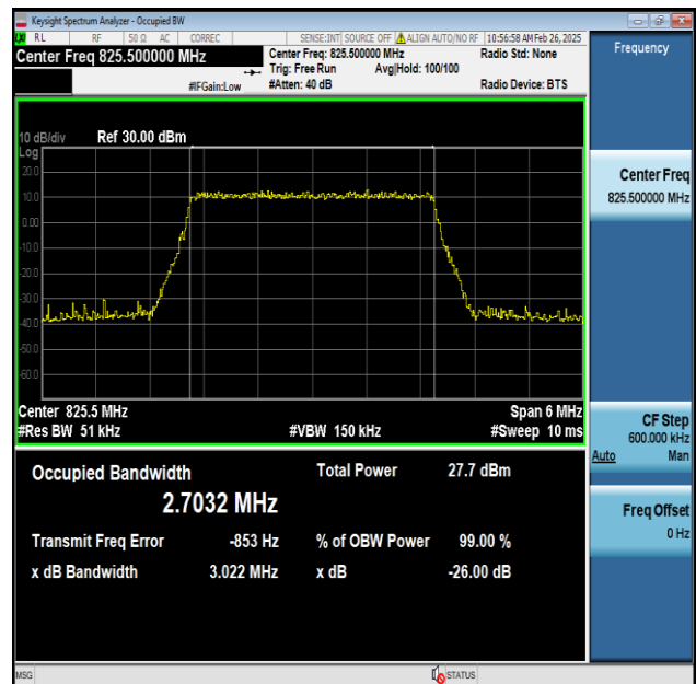
Band5-3MHz-256QAM-20415-15RB#0-PASS
