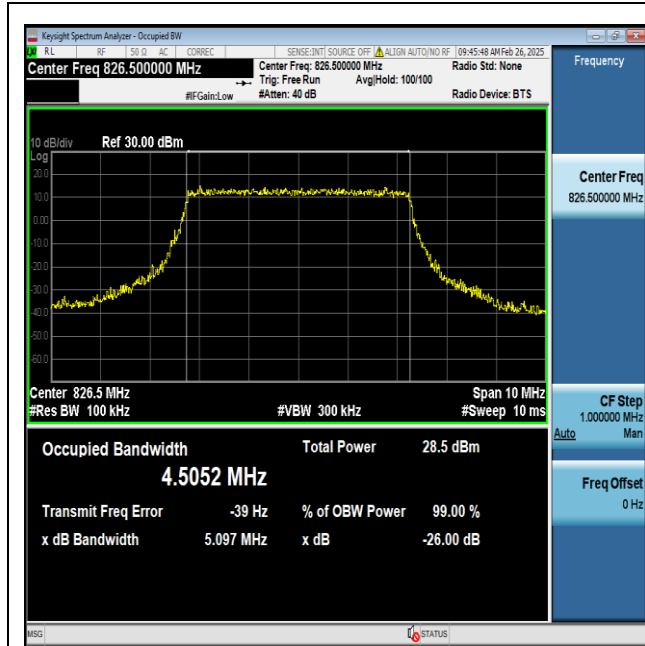
Band5-5MHz-QPSK-20425-25RB#0-PASS
