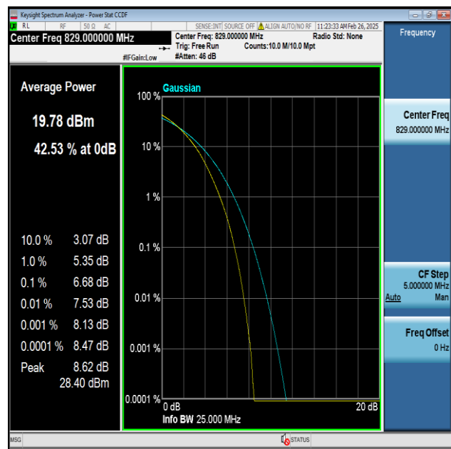
Band5-10MHz-256QAM-20450-50RB#0-PASS
