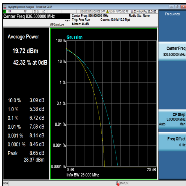
Band5-10MHz-256QAM-20525-50RB#0-PASS
