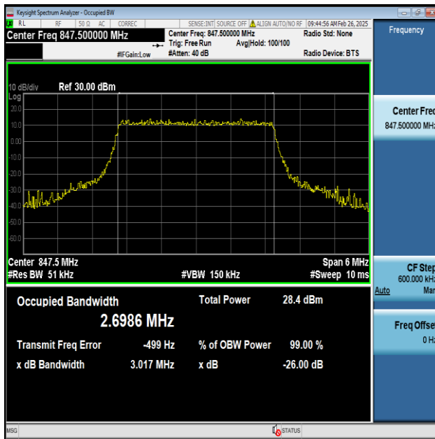
Band5-3MHz-QPSK-20635-15RB#0-PASS
