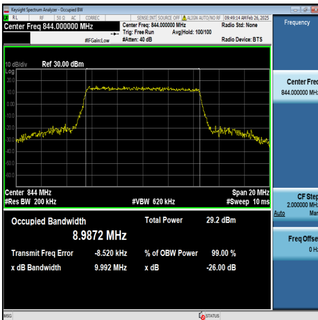
Band5-10MHz-64QAM-20600-50RB#0-PASS
