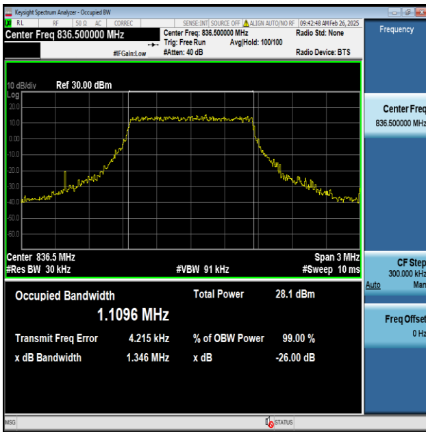
Band5-1.4MHz-QPSK-20525-6RB#0-PASS
