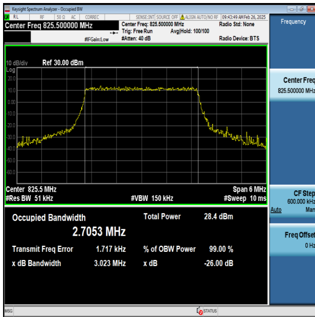
Band5-3MHz-QPSK-20415-15RB#0-PASS
