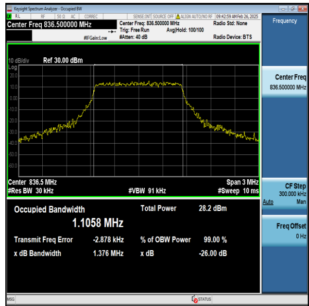
Band5-1.4MHz-16QAM-20525-6RB#0-PASS
