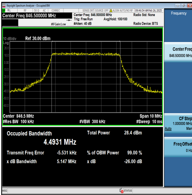
Band5-5MHz-QPSK-20625-25RB#0-PASS
