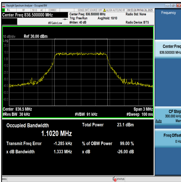
Band5-1.4MHz-64QAM-20525-6RB#0-PASS
