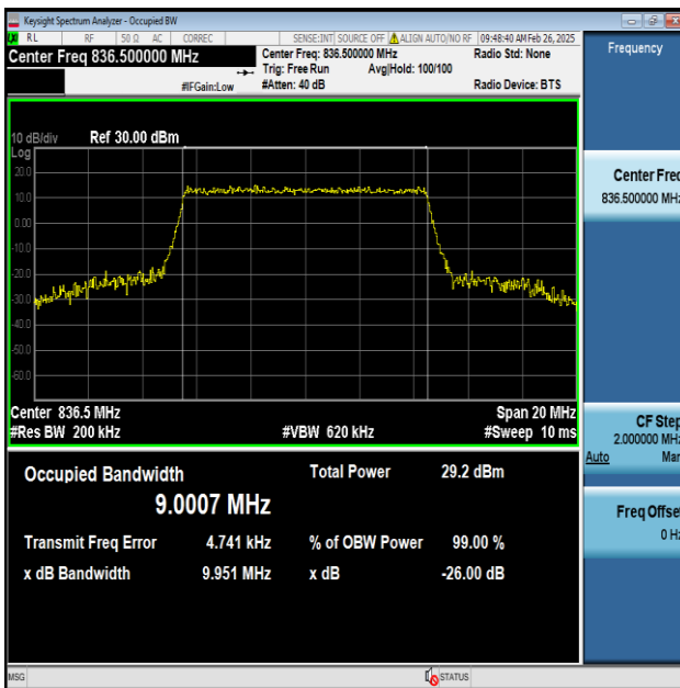
Band5-10MHz-64QAM-20525-50RB#0-PASS
