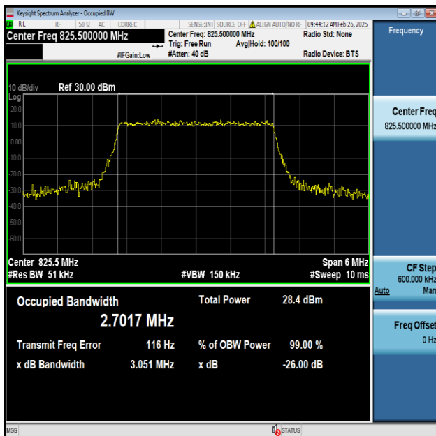
Band5-3MHz-64QAM-20415-15RB#0-PASS
