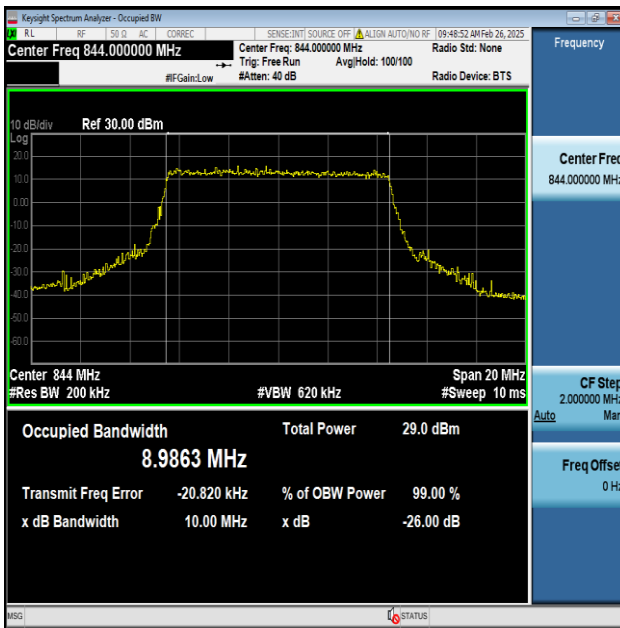
Band5-10MHz-QPSK-20600-50RB#0-PASS
