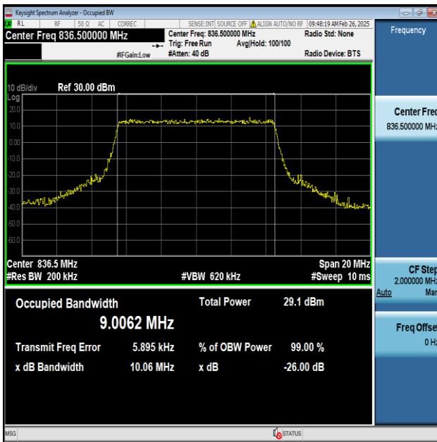
Band5-10MHz-QPSK-20525-50RB#0-PASS
