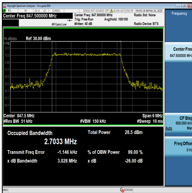
Band5-3MHz-64QAM-20635-15RB#0-PASS
