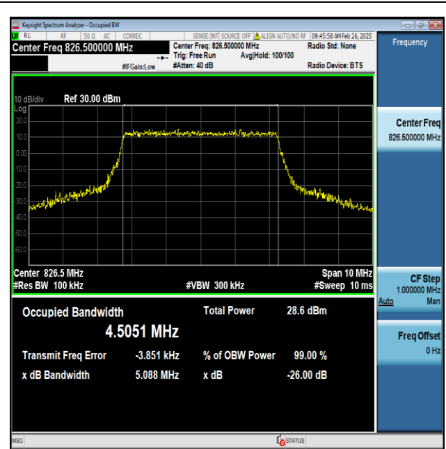
Band5-5MHz-16QAM-20425-25RB#0-PASS
