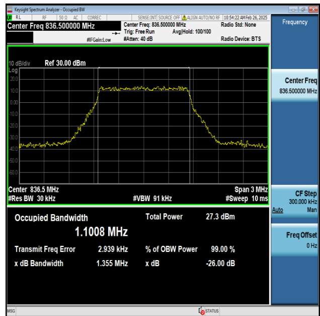
Band5-1.4MHz-256QAM-20525-6RB#0-PASS
