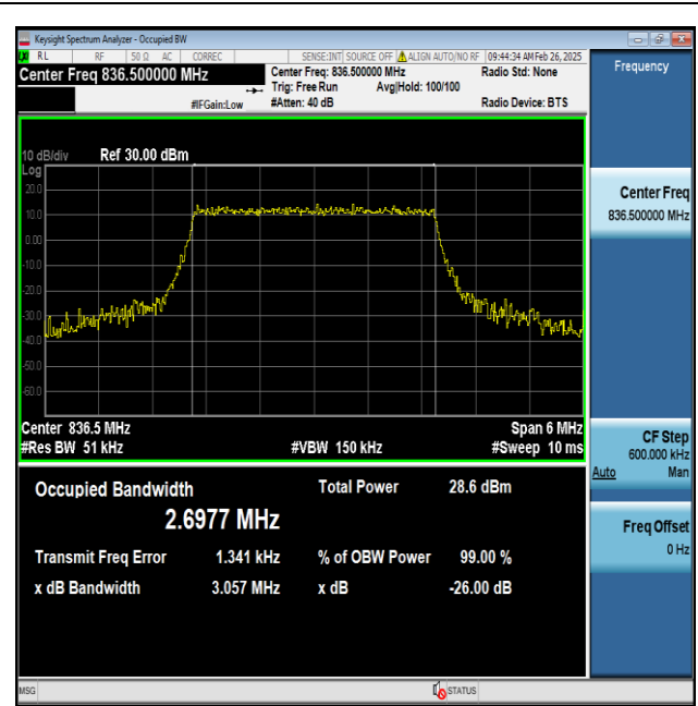
Band5-3MHz-16QAM-20525-15RB#0-PASS
