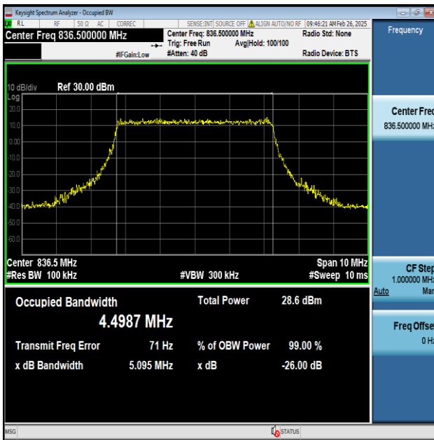
Band5-5MHz-QPSK-20525-25RB#0-PASS
