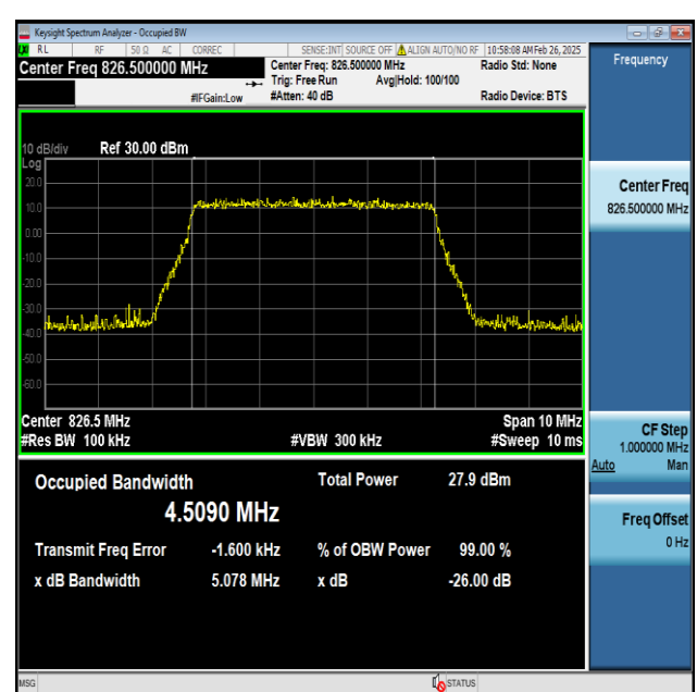
Band5-5MHz-256QAM-20425-25RB#0-PASS
