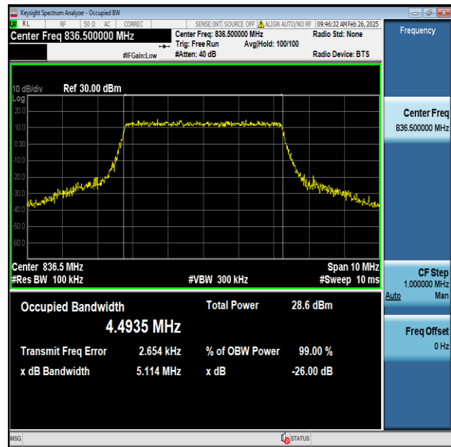
Band5-5MHz-16QAM-20525-25RB#0-PASS
