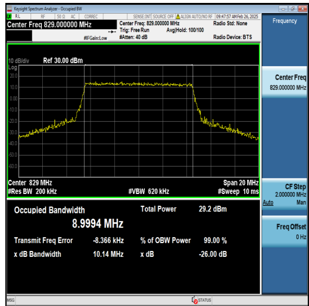
Band5-10MHz-16QAM-20450-50RB#0-PASS
