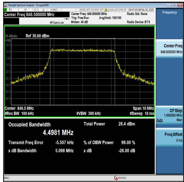
Band5-5MHz-16QAM-20625-25RB#0-PASS
