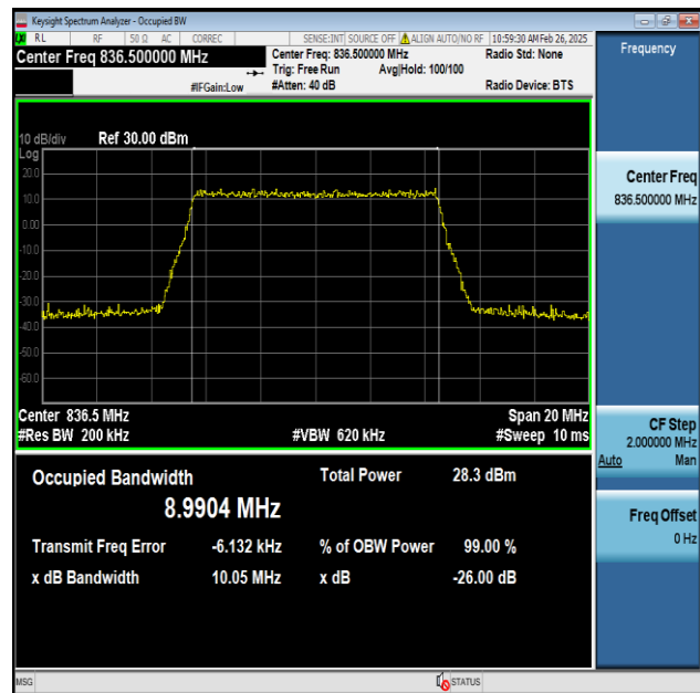
Band5-10MHz-256QAM-20525-50RB#0-PASS
