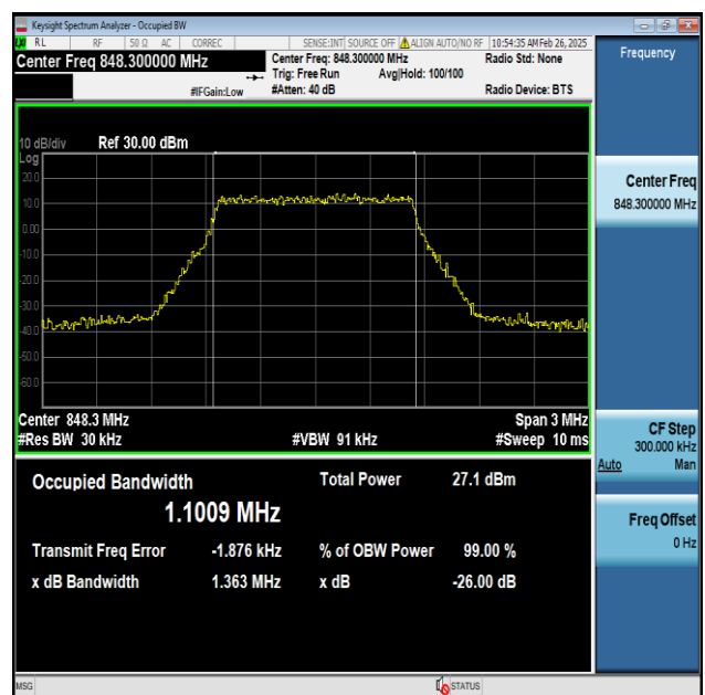
Band5-1.4MHz-256QAM-20643-6RB#0-PASS
