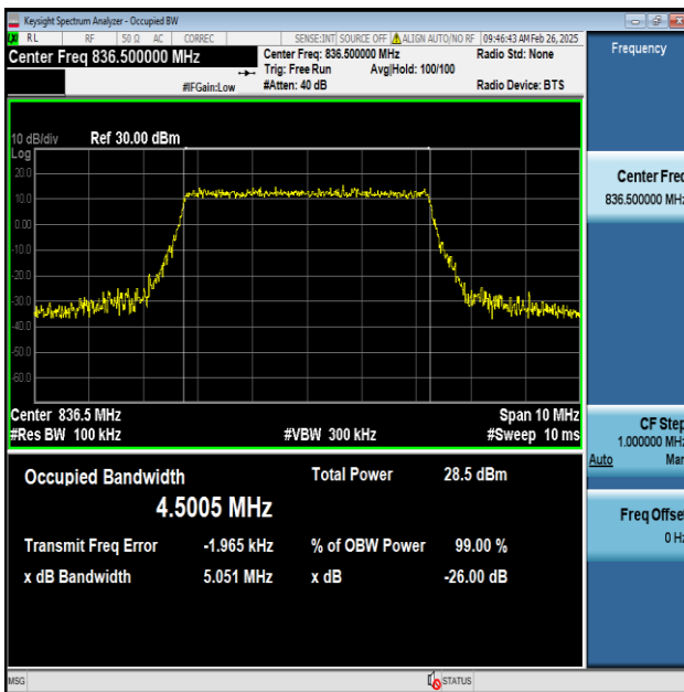
Band5-5MHz-64QAM-20525-25RB#0-PASS
