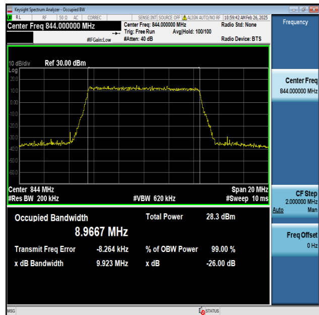
Band5-10MHz-256QAM-20600-50RB#0-PASS
