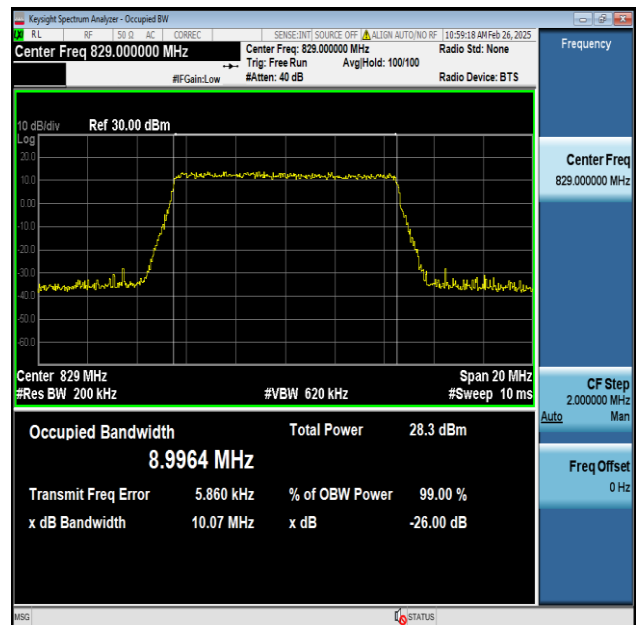
Band5-10MHz-256QAM-20450-50RB#0-PASS
