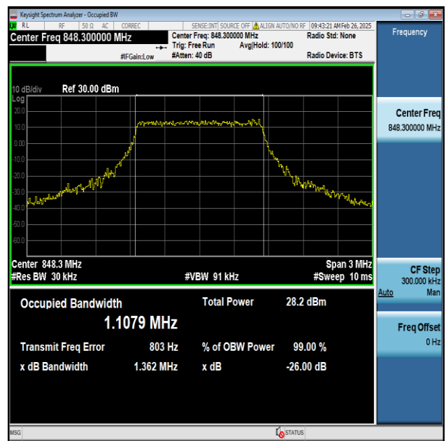
Band5-1.4MHz-16QAM-20643-6RB#0-PASS
