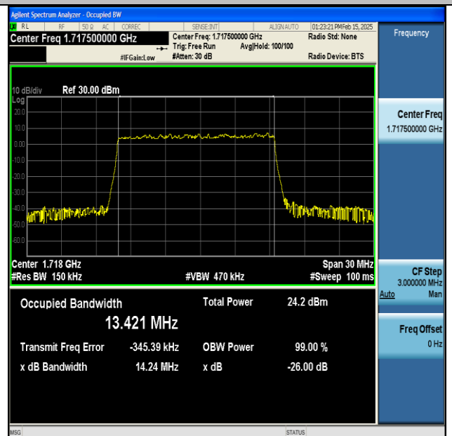
NTNV-DC_13A_n66A-PC3-15-5+15-M+L-QPSK-IDLE- DFT-QPSK-Outer_Full-Ant1-PASS
