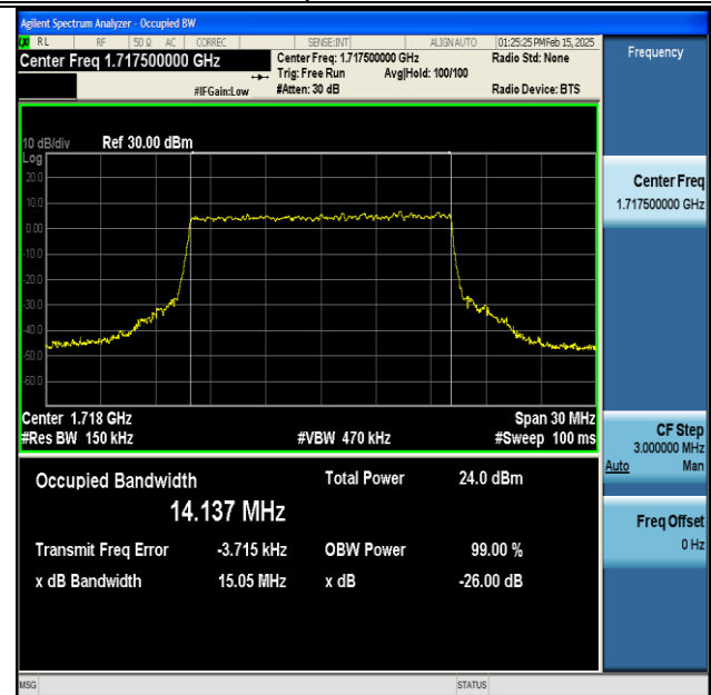
NTNV-DC_13A_n66A-PC3-15-5+15-M+L-QPSK-IDLE-CP-64QAM-Outet_Full-Ant1-PASS
