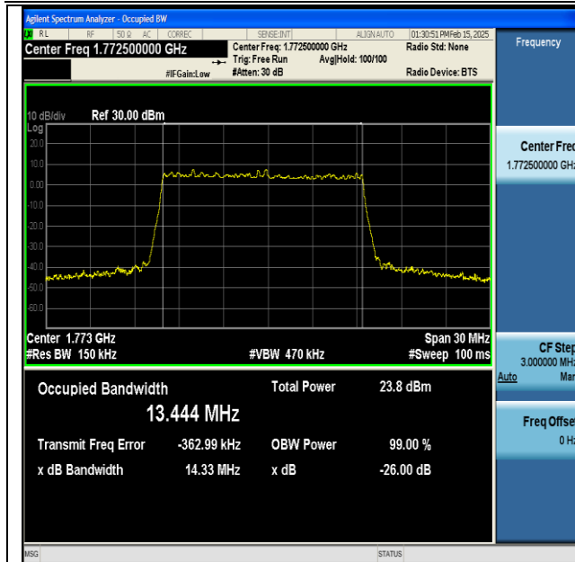
NTNV-DC_13A_n66A-PC3-15-5+15-M+H-QPSK-IDLE-DFT-256QAM-Outer_Full-Ant1-PASS
