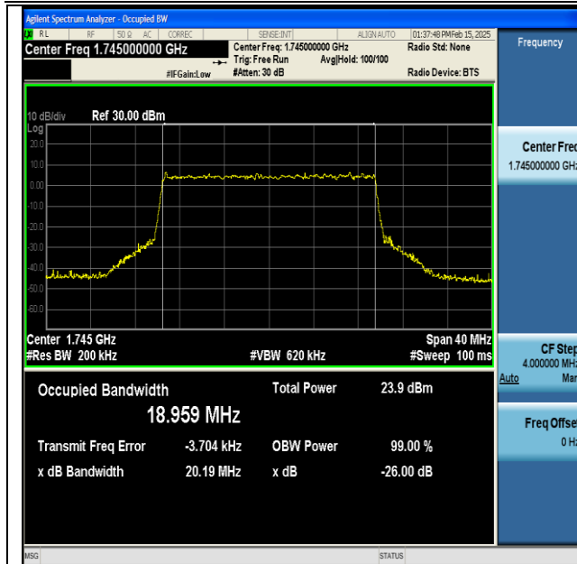
NTNV-DC_13A_n66A-PC3-15-5+20-M+M-QPSK-IDLE-CP-16QAM-Outer_Full-Ant1-PASS
