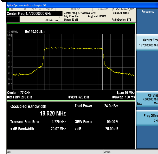
NTNV-DC_13A_n66A-PC3-15-5+20-M+H-QPSK-IDLE-CP-QPSK-Outer_Full-Ant1-PASS
