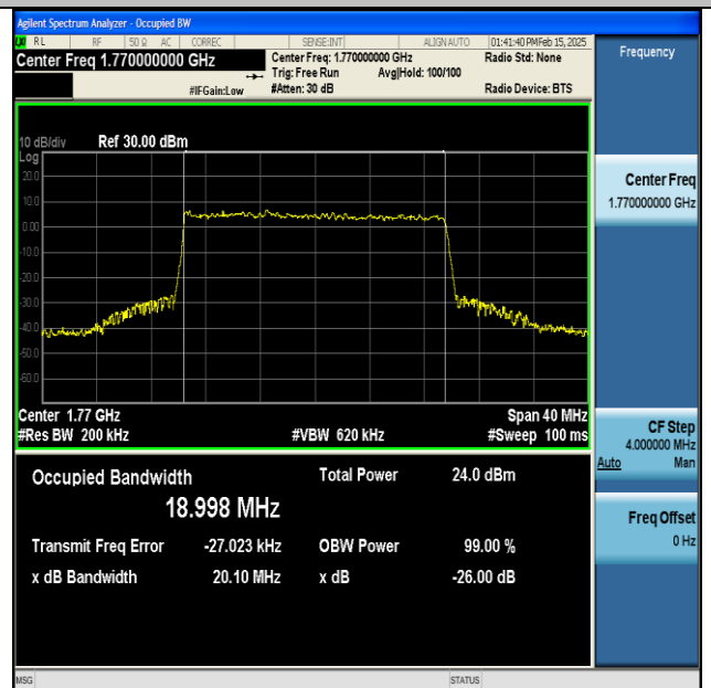
NTNV-DC_13A_n66A-PC3-15-5+20-M+H-QPSK-IDLE-CP-256QAM-Outer_Full-Ant1-PASS
