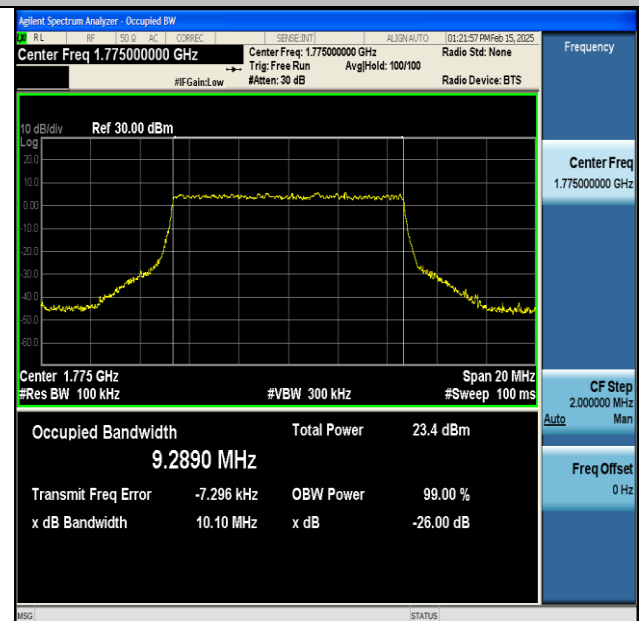
NTNV-DC_13A_n66A-PC3-15-5+10-M+H-QPSK-IDLE- CP-16QAM-Outer_Full-Ant1-PASS
