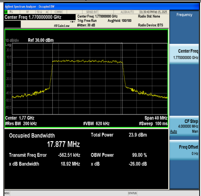
NTNV-DC_13A_n66A-PC3-15-5+20-M+H-QPSK-IDLE- DFT-16QAM-Outer_Full-Ant1-PASS
