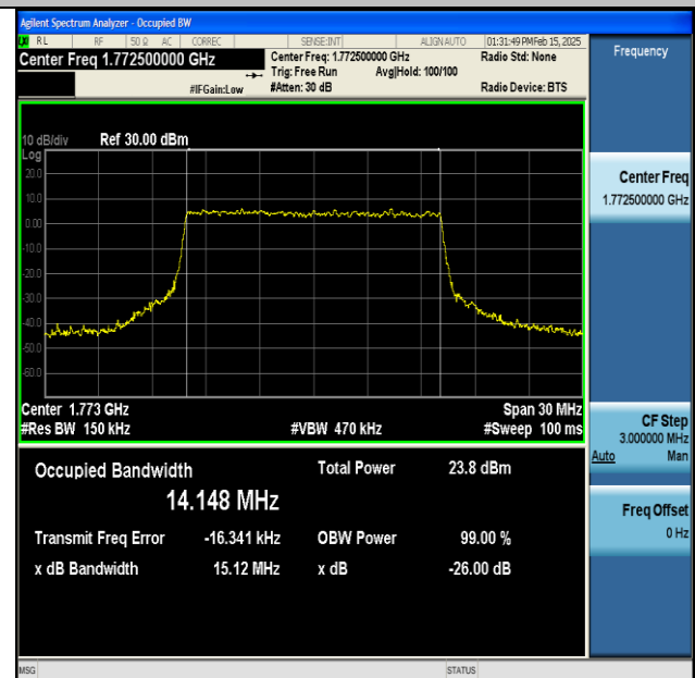
NTNV-DC_13A_n66A-PC3-15-5+15-M+H-QPSK-IDLE-CP-64QAM-Outer_Full-Ant1-PASS
