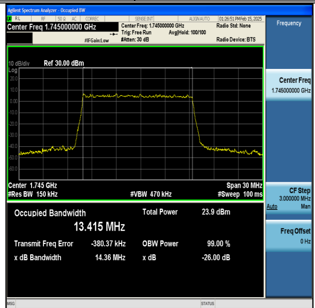
NTNV-DC_13A_n66A-PC3-15-5+15-M+M-QPSK-IDLE- DFT-16QAM-Outer_Full-Ant1-PASS
