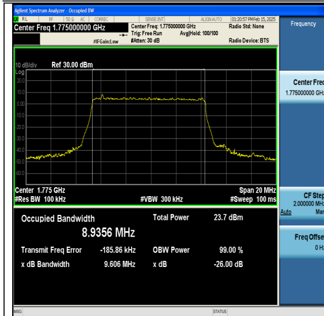
NTNV-DC_13A_n66A-PC3-15-5+10-M+H-QPSK-IDLE- DFT-64QAM-Outer_Full-Ant1-PASS
