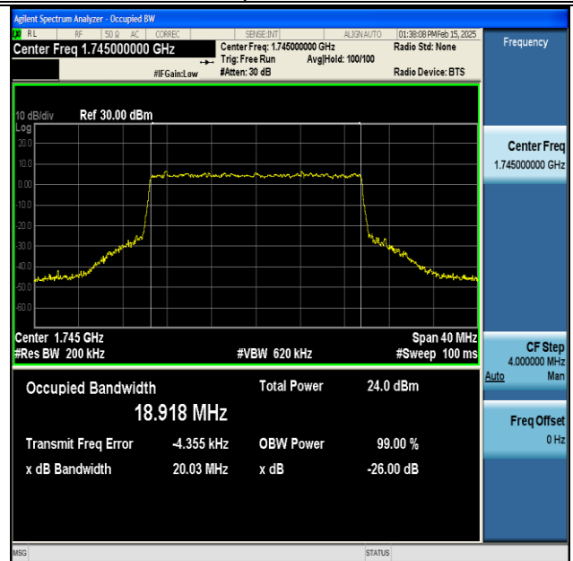
NTNV-DC_13A_n66A-PC3-15-5+20-M+M-QPSK-IDLE-CP-64QAM-Outer_Full-Ant1-PASS
