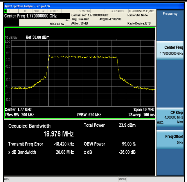
NTNV-DC_13A_n66A-PC3-15-5+20-M+H-QPSK-IDLE-CP-16QAM-Outer_Full-Ant1-PASS
