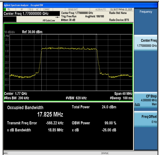
NTNV-DC_13A_n66A-PC3-15-5+20-M+H-QPSK-IDLE-DFT-BPSK-Outer_Full-Ant1-PASS
