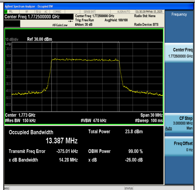
NTNV-DC_13A_n66A-PC3-15-5+15-M+H-QPSK-IDLE- DFT-64QAM-Outer_Full-Ant1-PASS
