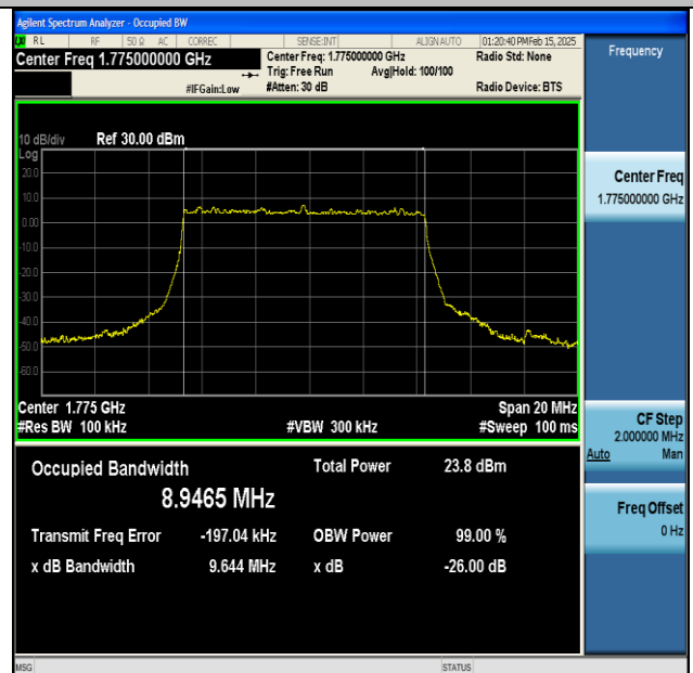
NTNV-DC_13A_n66A-PC3-15-5+10-M+H-QPSK-IDLE- DFT-16QAM-Outer_Full-Ant1-PASS
