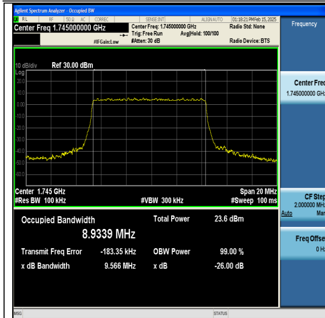
NTNV-DC_13A_n66A-PC3-15-5+10-M+M-QPSK-IDLE- DFT-256QAM-Outer_Full-Ant1-PASS
