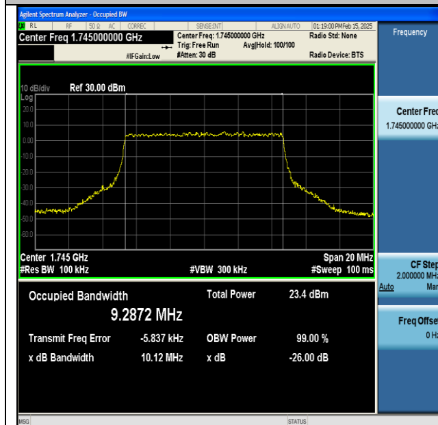
NTNV-DC_13A_n66A-PC3-15-5+10-M+M-QPSK-IDLE- CP-16QAM-Outer_Full-Ant1-PASS
