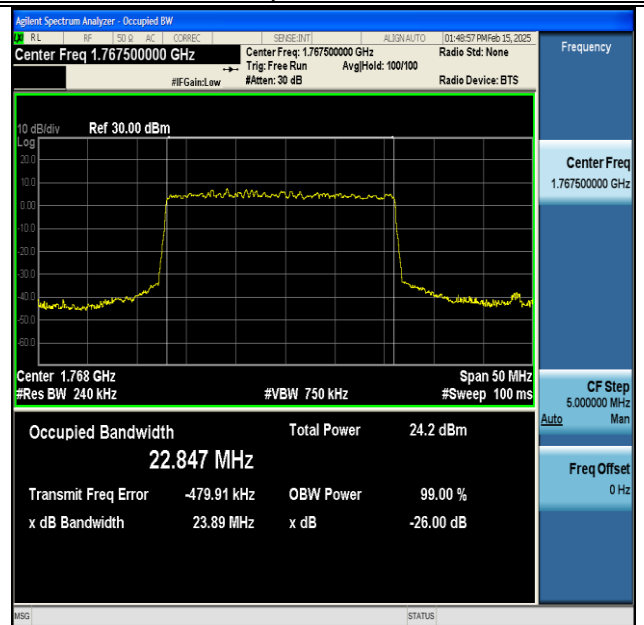
NTNV-DC_13A_n66A-PC3-15-5+25-M+H-QPSK-IDLE- DFT-64QAM-Outer_Full-Ant1-PASS
