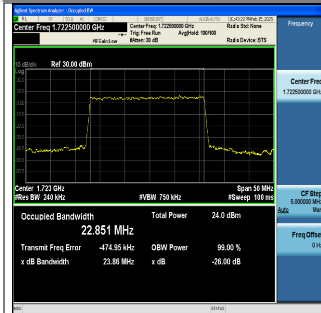
NTNV-DC_13A_n66A-PC3-15-5+25-M+L-QPSK-IDLE-DFT-256QAM-Outter_Full-Ant1-PASS
