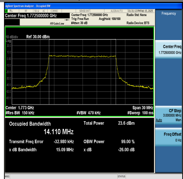
NTNV-DC_13A_n66A-PC3-15-5+15-M+H-QPSK-IDLE-CP-QPSK-Outer_Full-Ant1-PASS
