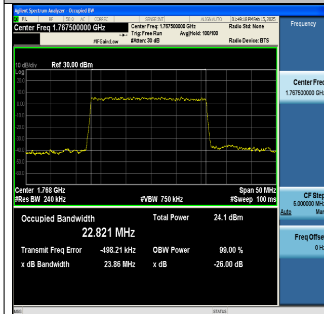
NTNV-DC_13A_n66A-PC3-15-5+25-M+H-QPSK-IDLE- DFT-256QAM-Outer_Full-Ant1-PASS
