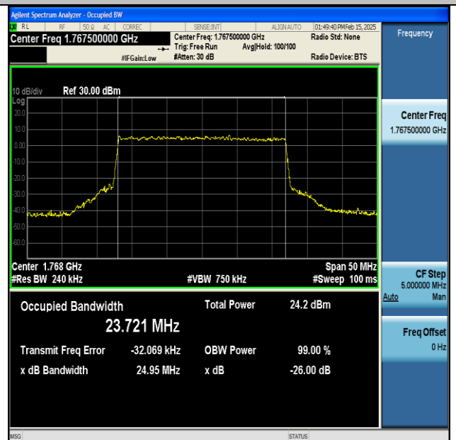
NTNV-DC_13A_n66A-PC3-15-5+25-M+H-QPSK-IDLE- CP-QPSK-Outer_Full-Ant1-PASS
