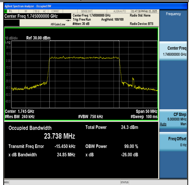
NTNV-DC_13A_n66A-PC3-15-5+25-M+M-QPSK-IDLE-CP-256QAM-Outer_Full-Ant1-PASS
