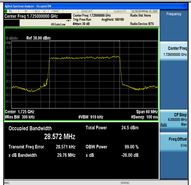
NTNV-DC_13A_n66A-PC3-15-5+30-M+L-QPSK-IDLE- DFT-BPSK-Outer_Full-Ant1-PASS
