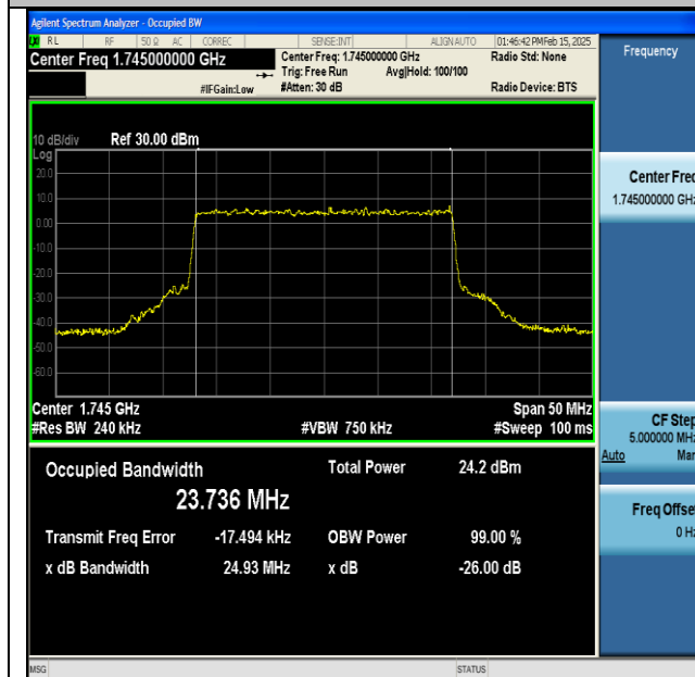
NTNV-DC_13A_n66A-PC3-15-5+25-M+M-QPSK-IDLE- CP-QPSK-Outer_Full-Ant1-PASS
