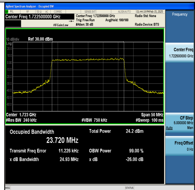
NTNV-DC_13A_n66A-PC3-15-5+25-M+L-QPSK-IDLE-CP-64QAM-Outter_Full-Ant1-PASS
