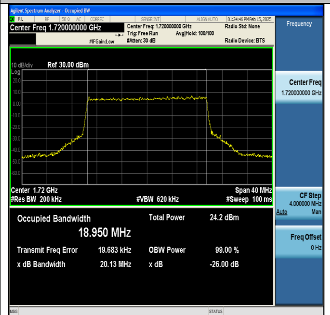
NTNV-DC_13A_n66A-PC3-15-5+20-M+L-QPSK-IDLE-CP-16QAM-Outer_Full-Ant1-PASS
