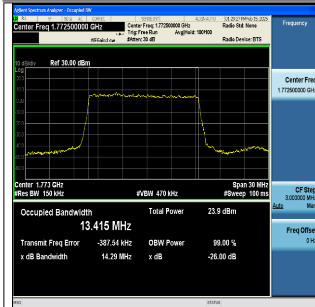
NTNV-DC_13A_n66A-PC3-15-5+15-M+H-QPSK-IDLE- DFT-BPSK-Outer_Full-Ant1-PASS
