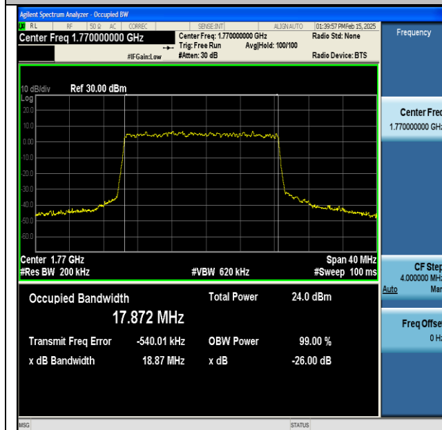
NTNV-DC_13A_n66A-PC3-15-5+20-M+H-QPSK-IDLE- DFT-64QAM-Outer_Full-Ant1-PASS
