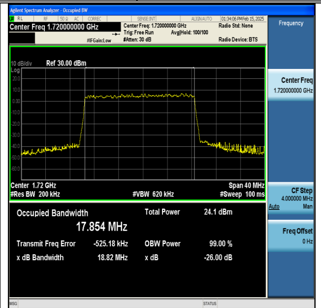
NTNV-DC_13A_n66A-PC3-15-5+20-M+L-QPSK-IDLE-DFT-256QAM-Outer_Full-Ant1-PASS
