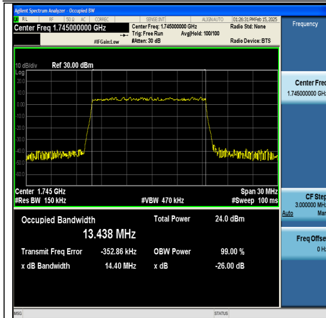
NTNV-DC_13A_n66A-PC3-15-5+15-M+M-QPSK-IDLE- DFT-QPSK-Outer_Full-Ant1-PASS
