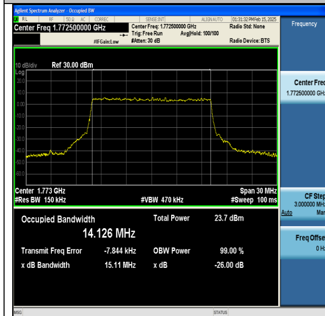
NTNV-DC_13A_n66A-PC3-15-5+15-M+H-QPSK-IDLE-CP-16QAM-Outer_Full-Ant1-PASS
