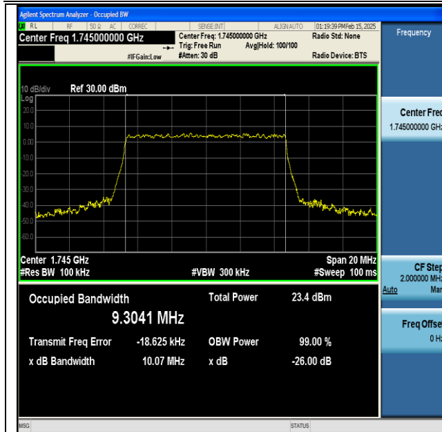
NTNV-DC_13A_n66A-PC3-15-5+10-M+M-QPSK-IDLE- CP-256QAM-Outer_Full-Ant1-PASS
