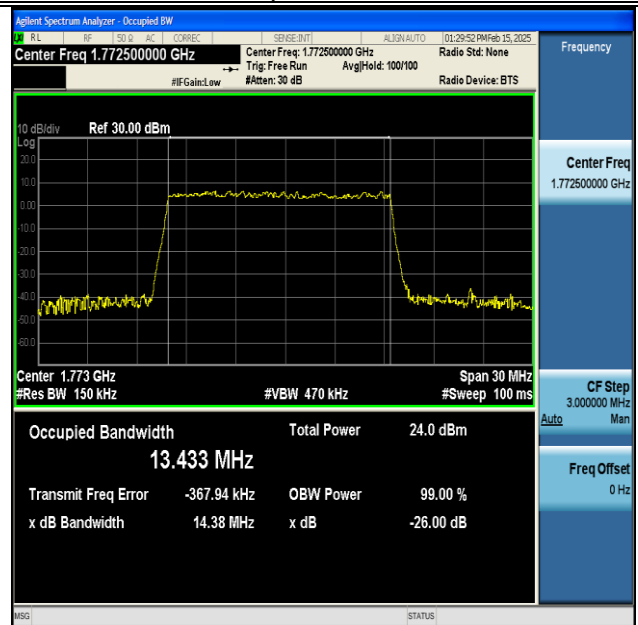
NTNV-DC_13A_n66A-PC3-15-5+15-M+H-QPSK-IDLE- DFT-QPSK-Outer_Full-Ant1-PASS
