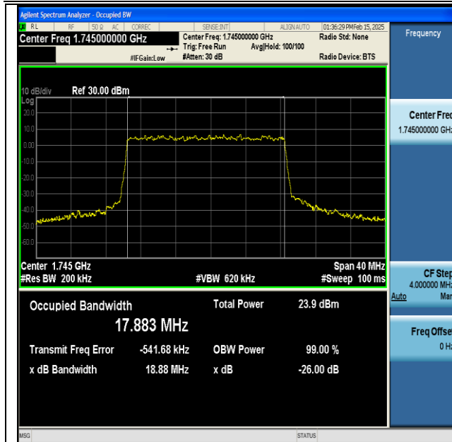
NTNV-DC_13A_n66A-PC3-15-5+20-M+M-QPSK-IDLE- DFT-16QAM-Outer_Full-Ant1-PASS
