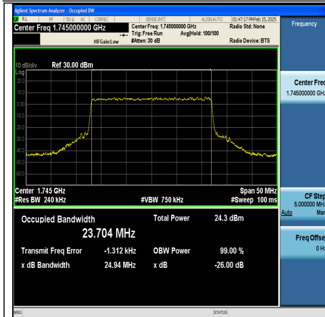
NTNV-DC_13A_n66A-PC3-15-5+25-M+M-QPSK-IDLE-CP-64QAM-Outer_Full-Ant1-PASS
