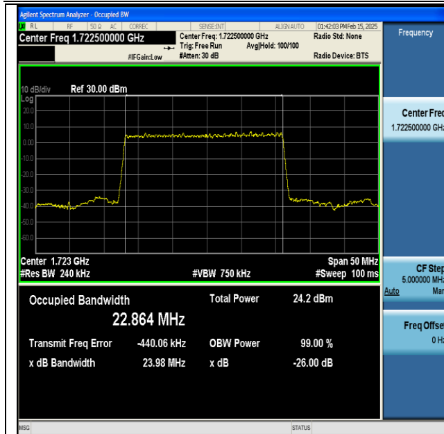
NTNV-DC_13A_n66A-PC3-15-5+25-M+L-QPSK-IDLE- DFT-BPSK-Outer_Full-Ant1-PASS
