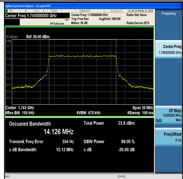
NTNV-DC_13A_n66A-PC3-15-5+15-M+M-QPSK-IDLE-CP-16QAM-Outer_Full-Ant1-PASS
