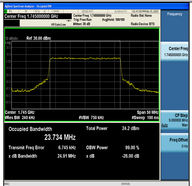
NTNV-DC_13A_n66A-PC3-15-5+25-M+M-QPSK-IDLE- CP-16QAM-Outer_Full-Ant1-PASS
