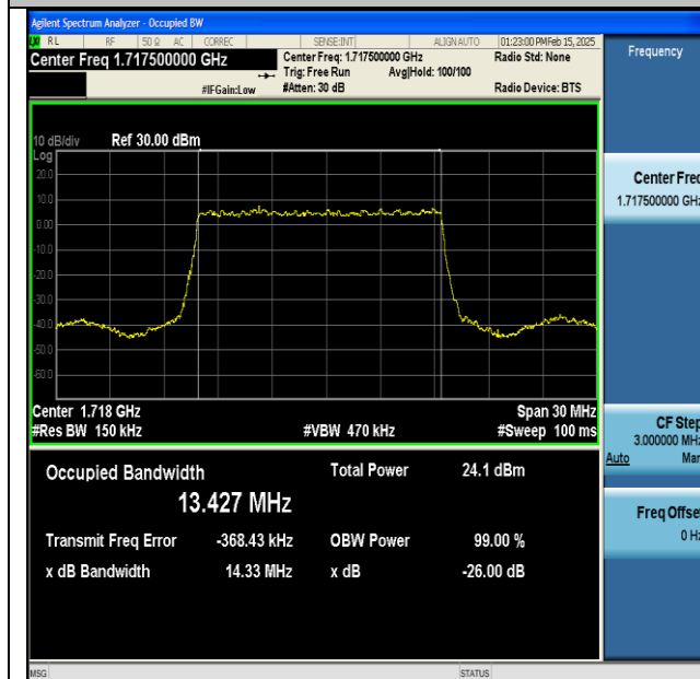
NTNV-DC_13A_n66A-PC3-15-5+15-M+L-QPSK-IDLE- DFT-BPSK-Outer_Full-Ant1-PASS
