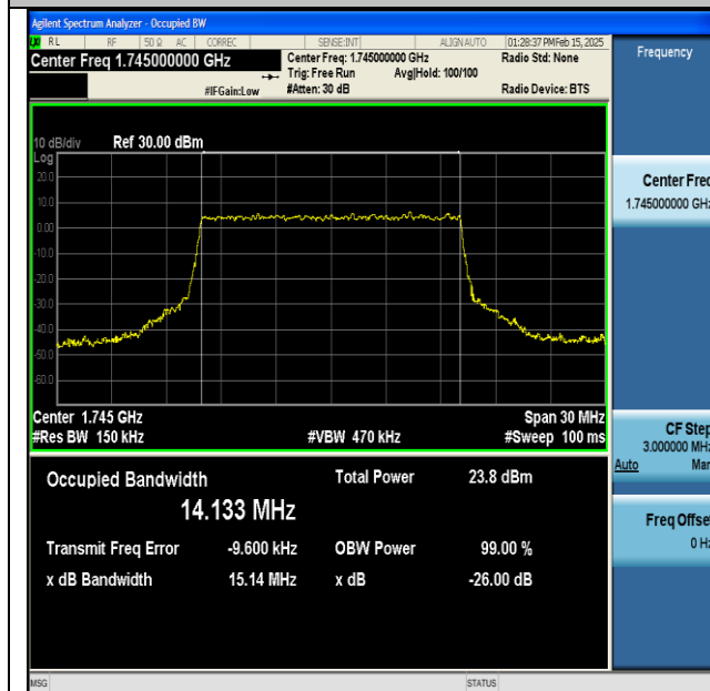
NTNV-DC_13A_n66A-PC3-15-5+15-M+M-QPSK-IDLE-CP-64QAM-Outer_Full-Ant1-PASS
