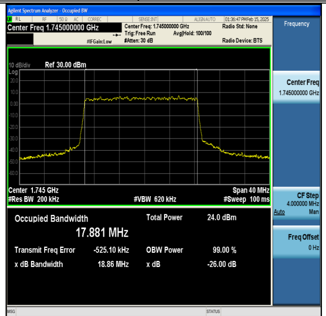
NTNV-DC_13A_n66A-PC3-15-5+20-M+M-QPSK-IDLE- DFT-64QAM-Outer_Full-Ant1-PASS
