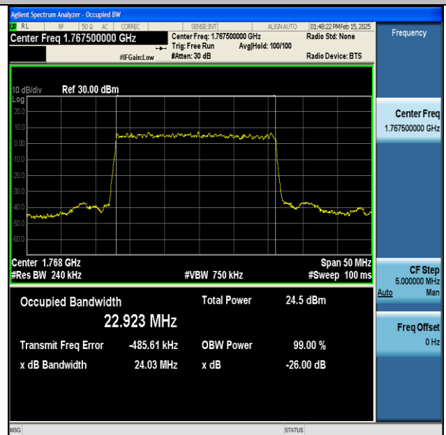
NTNV-DC_13A_n66A-PC3-15-5+25-M+H-QPSK-IDLE-DFT-QPSK-Outer_Full-Ant1-PASS
