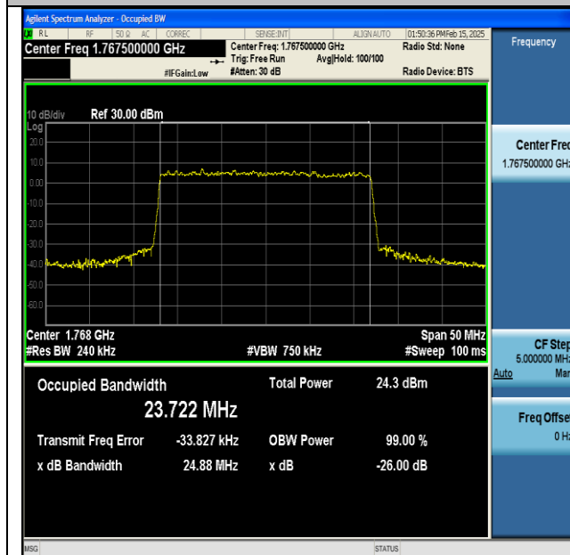
NTNV-DC_13A_n66A-PC3-15-5+25-M+H-QPSK-IDLE- CP-256QAM-Outer_Full-Ant1-PASS
