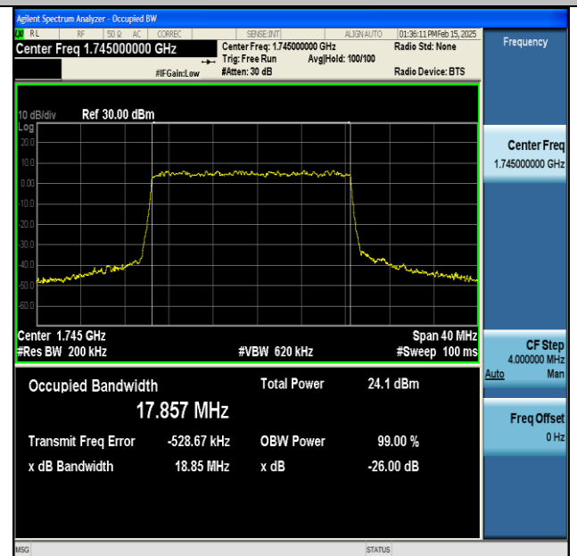
NTNV-DC_13A_n66A-PC3-15-5+20-M+M-QPSK-IDLE-DFT-QPSK-Outet_Full-Ant1-PASS
