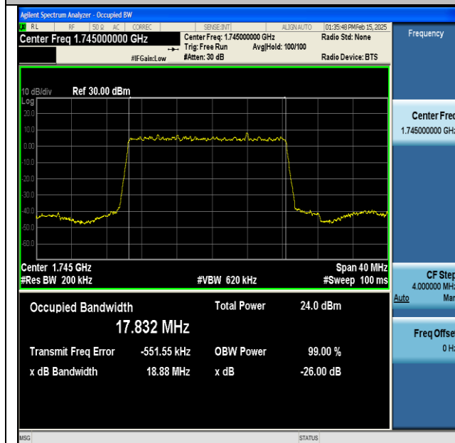
NTNV-DC_13A_n66A-PC3-15-5+20-M+M-QPSK-IDLE-DFT-BPSK-Outet_Full-Ant1-PASS
