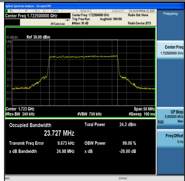
NTNV-DC_13A_n66A-PC3-15-5+25-M+L-QPSK-IDLE-CP-QPSK-Outter_Full-Ant1-PASS
