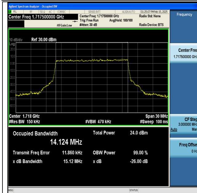
NTNV-DC_13A_n66A-PC3-15-5+15-M+L-QPSK-IDLE-CP-16QAM-Outet_Full-Ant1-PASS
