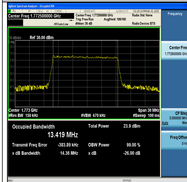
NTNV-DC_13A_n66A-PC3-15-5+15-M+H-QPSK-IDLE- DFT-16QAM-Outer_Full-Ant1-PASS
