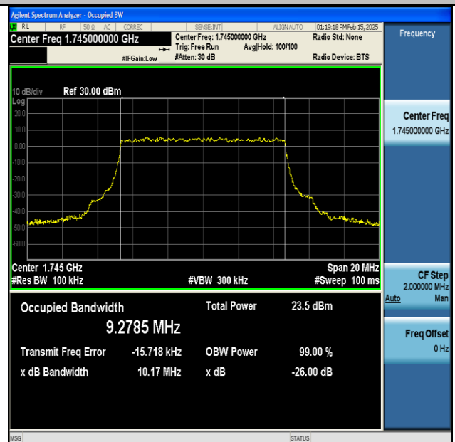
NTNV-DC_13A_n66A-PC3-15-5+10-M+M-QPSK-IDLE- CP-64QAM-Outer_Full-Ant1-PASS
