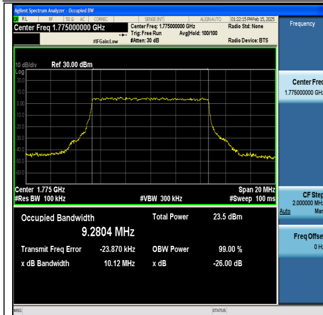
NTNV-DC_13A_n66A-PC3-15-5+10-M+H-QPSK-IDLE- CP-64QAM-Outer_Full-Ant1-PASS
