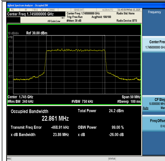
NTNV-DC_13A_n66A-PC3-15-5+25-M+M-QPSK-IDLE- DFT-64QAM-Outer_Full-Ant1-PASS
