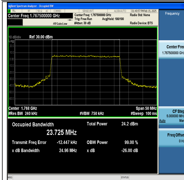
NTNV-DC_13A_n66A-PC3-15-5+25-M+H-QPSK-IDLE- CP-16QAM-Outer_Full-Ant1-PASS
