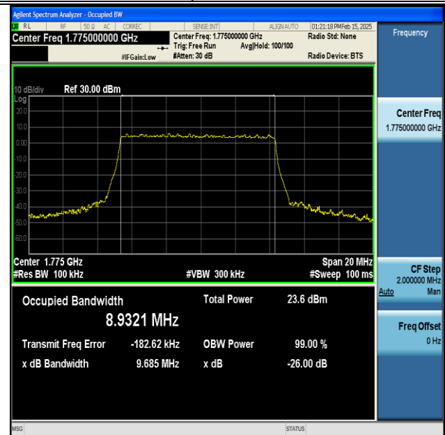
NTNV-DC_13A_n66A-PC3-15-5+10-M+H-QPSK-IDLE- DFT-256QAM-Outer_Full-Ant1-PASS
