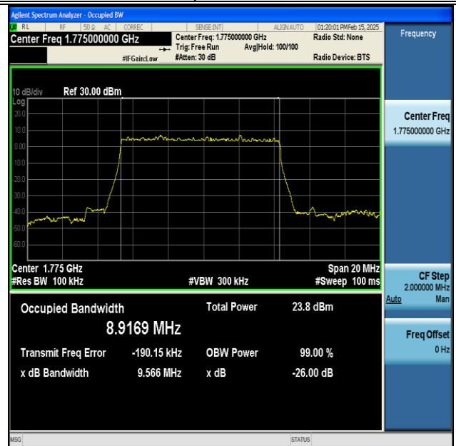
NTNV-DC_13A_n66A-PC3-15-5+10-M+H-QPSK-IDLE- DFT-BPSK-Outer_Full-Ant1-PASS
