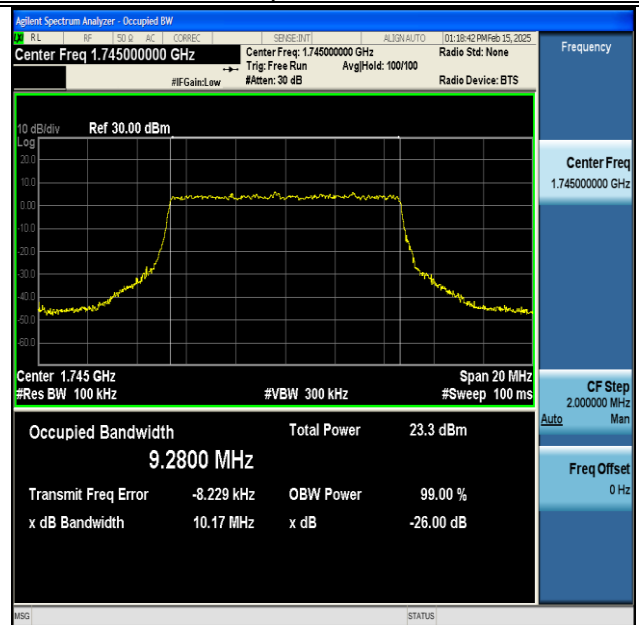
NTNV-DC_13A_n66A-PC3-15-5+10-M+M-QPSK-IDLE- CP-QPSK-Outer_Full-Ant1-PASS
