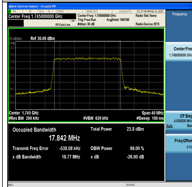
NTNV-DC_13A_n66A-PC3-15-5+20-M+M-QPSK-IDLE- DFT-256QAM-Outer_Full-Ant1-PASS
