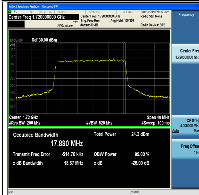
NTNV-DC_13A_n66A-PC3-15-5+20-M+L-QPSK-IDLE-DFT-64QAM-Outer_Full-Ant1-PASS
