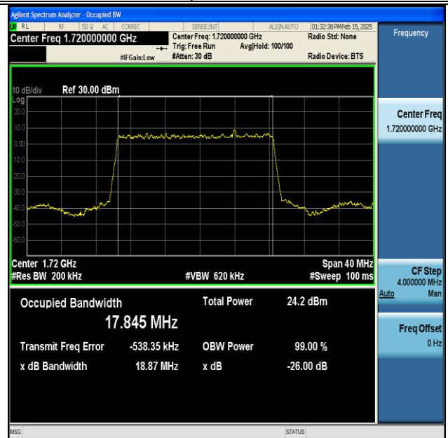
NTNV-DC_13A_n66A-PC3-15-5+20-M+L-QPSK-IDLE-DFT-BPSK-Outer_Full-Ant1-PASS
