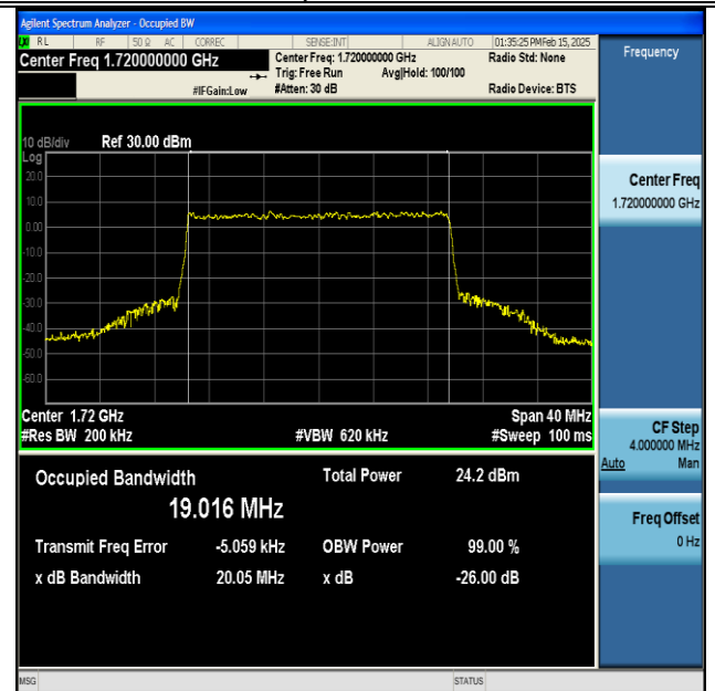
NTNV-DC_13A_n66A-PC3-15-5+20-M+L-QPSK-IDLE-CP-256QAM-Outet_Full-Ant1-PASS
