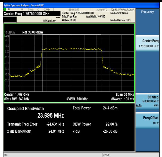
NTNV-DC_13A_n66A-PC3-15-5+25-M+H-QPSK-IDLE- CP-64QAM-Outer_Full-Ant1-PASS
