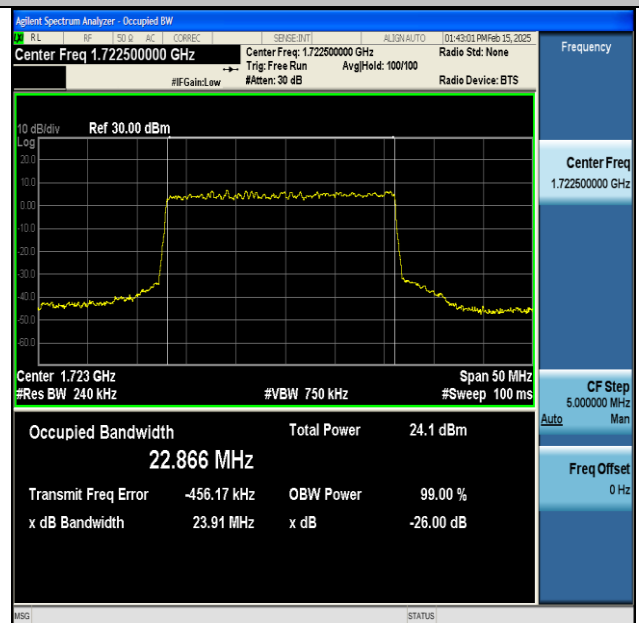
NTNV-DC_13A_n66A-PC3-15-5+25-M+L-QPSK-IDLE- DFT-64QAM-Outer_Full-Ant1-PASS
