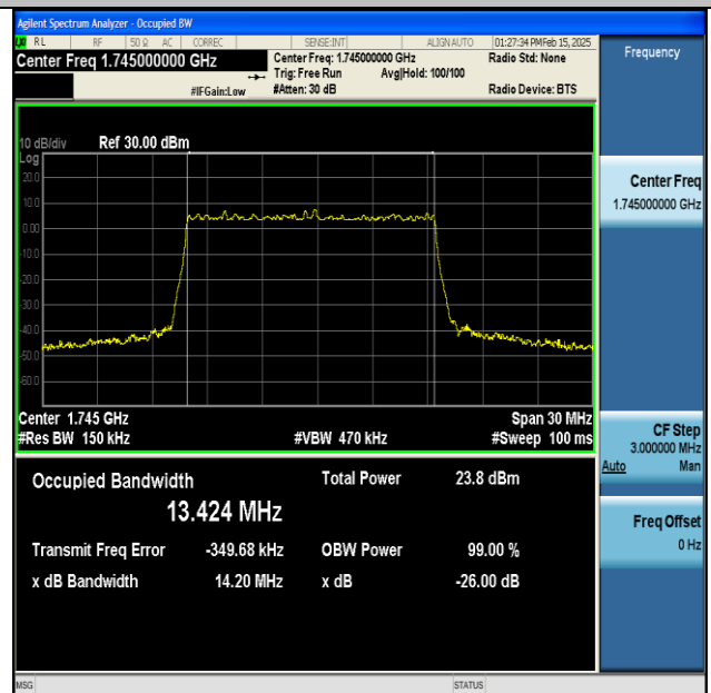
NTNV-DC_13A_n66A-PC3-15-5+15-M+M-QPSK-IDLE- DFT-256QAM-Outer_Full-Ant1-PASS
