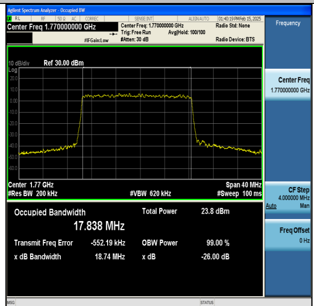
NTNV-DC_13A_n66A-PC3-15-5+20-M+H-QPSK-IDLE- DFT-256QAM-Outer_Full-Ant1-PASS
