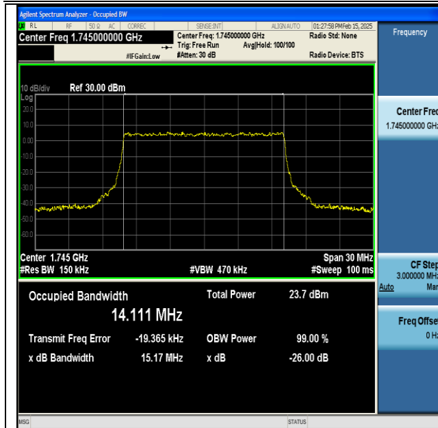
NTNV-DC_13A_n66A-PC3-15-5+15-M+M-QPSK-IDLE-CP-QPSK-Outer_Full-Ant1-PASS
