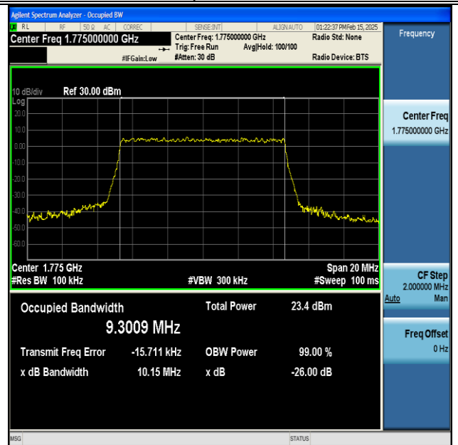
NTNV-DC_13A_n66A-PC3-15-5+10-M+H-QPSK-IDLE- CP-256QAM-Outer_Full-Ant1-PASS
