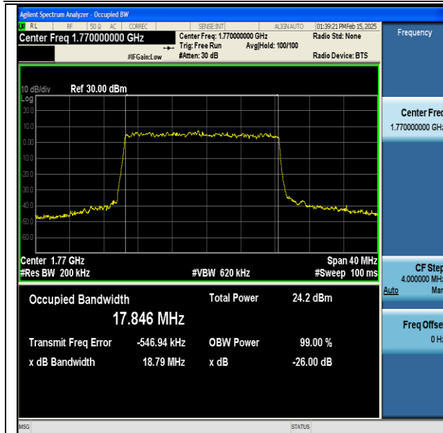
NTNV-DC_13A_n66A-PC3-15-5+20-M+H-QPSK-IDLE- DFT-QPSK-Outer_Full-Ant1-PASS
