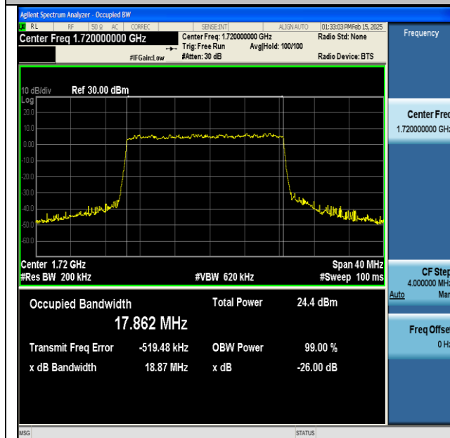
NTNV-DC_13A_n66A-PC3-15-5+20-M+L-QPSK-IDLE-DFT-QPSK-Outer_Full-Ant1-PASS
