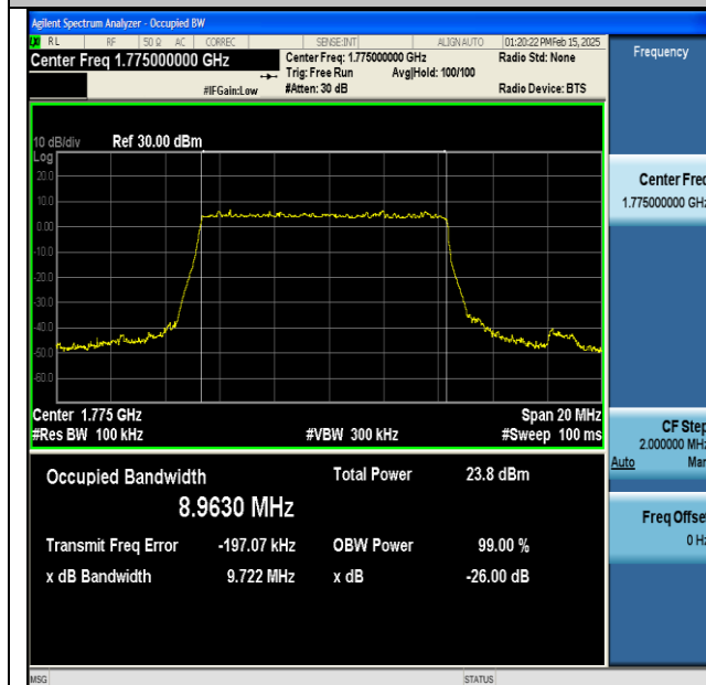
NTNV-DC_13A_n66A-PC3-15-5+10-M+H-QPSK-IDLE- DFT-QPSK-Outer_Full-Ant1-PASS
