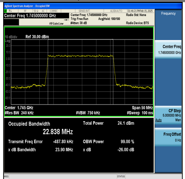
NTNV-DC_13A_n66A-PC3-15-5+25-M+M-QPSK-IDLE- DFT-256QAM-Outer_Full-Ant1-PASS
