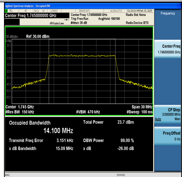
NTNV-DC_13A_n66A-PC3-15-5+15-M+M-QPSK-IDLE-CP-256QAM-Outer_Full-Ant1-PASS
