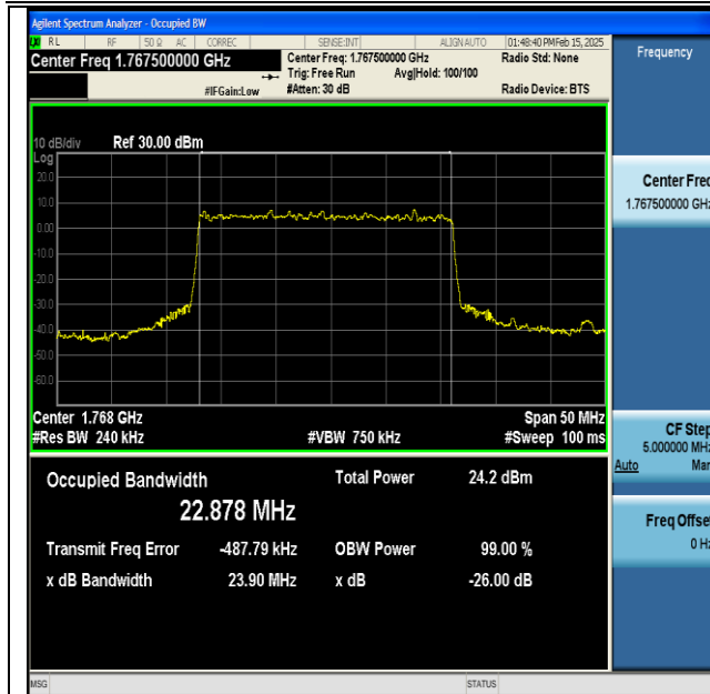
NTNV-DC_13A_n66A-PC3-15-5+25-M+H-QPSK-IDLE- DFT-16QAM-Outer_Full-Ant1-PASS
