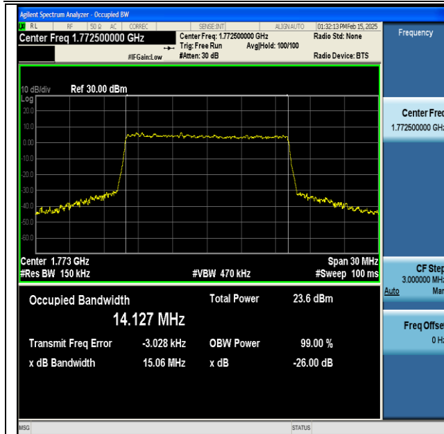
NTNV-DC_13A_n66A-PC3-15-5+15-M+H-QPSK-IDLE-CP-256QAM-Outer_Full-Ant1-PASS
