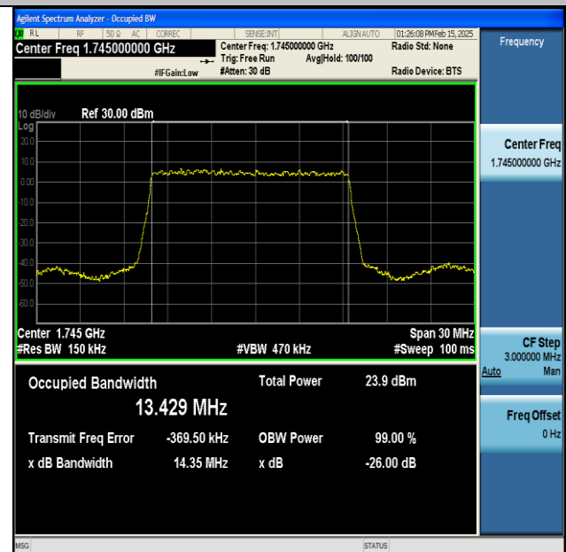
NTNV-DC_13A_n66A-PC3-15-5+15-M+M-QPSK-IDLE-DFT-BPSK-Outet_Full-Ant1-PASS
