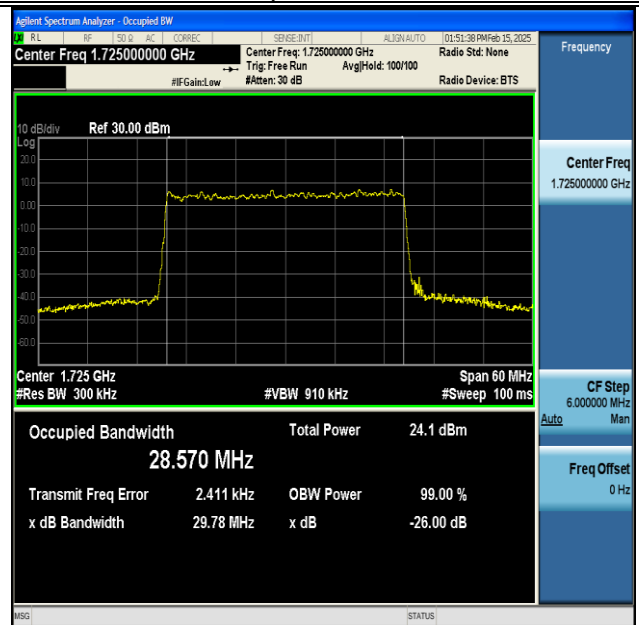
NTNV-DC_13A_n66A-PC3-15-5+30-M+L-QPSK-IDLE- DFT-16QAM-Outer_Full-Ant1-PASS
