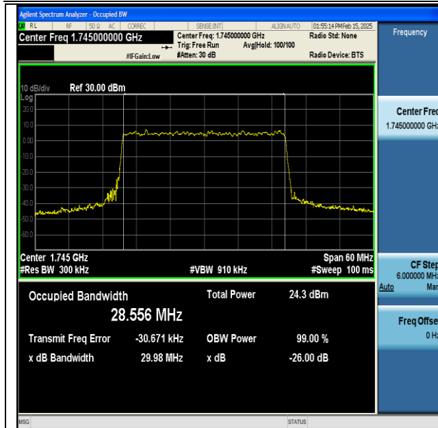
NTNV-DC_13A_n66A-PC3-15-5+30-M+M-QPSK-IDLE-DFT-256QAM-Outet_Full-Ant1-PASS
