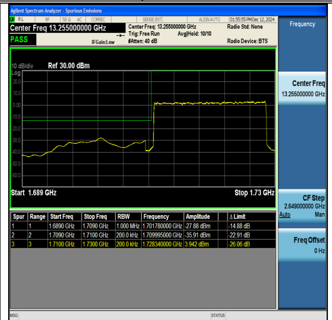
NTNV-DC_13A_n66A-PC3-15-5+20-M+L-QPSK-IDLE- DFT-BPSK-Outer_Full-PASS
