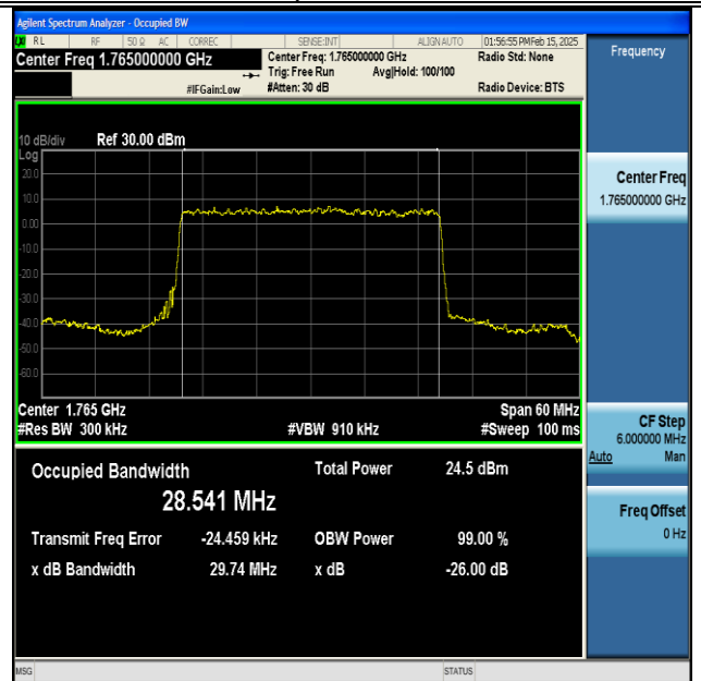
NTNV-DC_13A_n66A-PC3-15-5+30-M+H-QPSK-IDLE-DFT-BPSK-Outer_Full-Ant1-PASS
