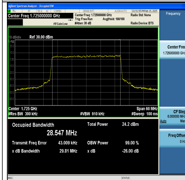
NTNV-DC_13A_n66A-PC3-15-5+30-M+L-QPSK-IDLE- DFT-64QAM-Outer_Full-Ant1-PASS
