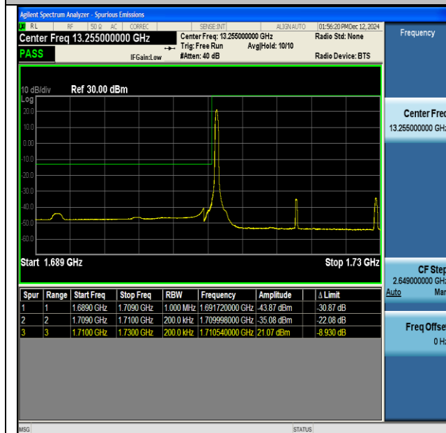
NTNV-DC_13A_n66A-PC3-15-5+20-M+L-QPSK-IDLE-CP- QPSK-Edge_1RB_Left-PASS
