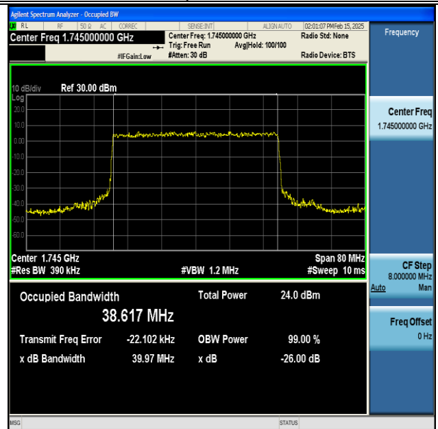
NTNV-DC_13A_n66A-PC3-15-5+40-M+M-QPSK-IDLE- DFT-16QAM-Outer_Full-Ant1-PASS
