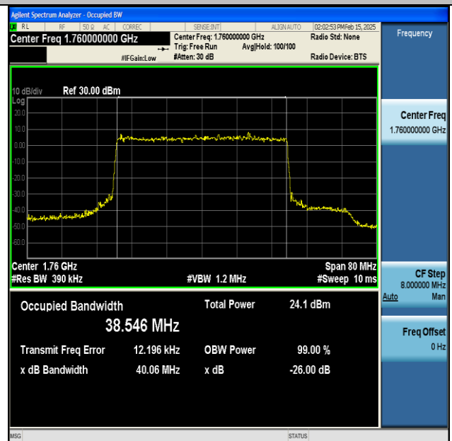
NTNV-DC_13A_n66A-PC3-15-5+40-M+H-QPSK-IDLE- DFT-64QAM-Outer_Full-Ant1-PASS
