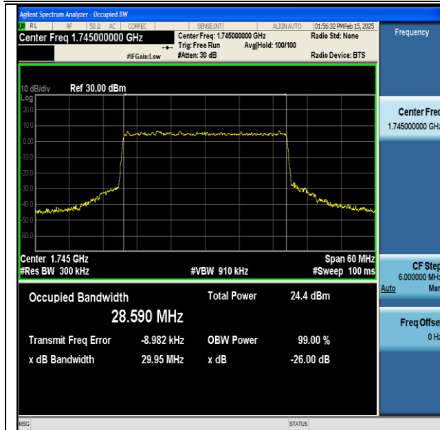
NTNV-DC_13A_n66A-PC3-15-5+30-M+M-QPSK-IDLE-CP-256QAM-Outer_Full-Ant1-PASS
