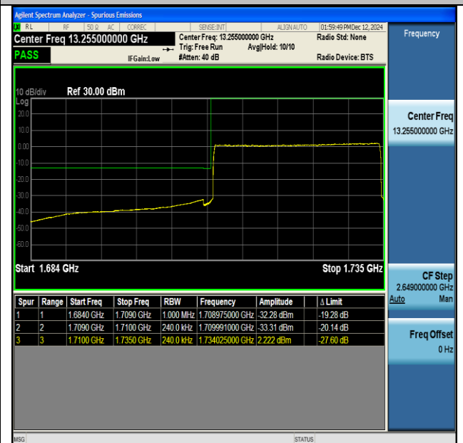
NTNV-DC_13A_n66A-PC3-15-5+25-M+L-QPSK-IDLE-CP- QPSK-Outer_Full-PASS
