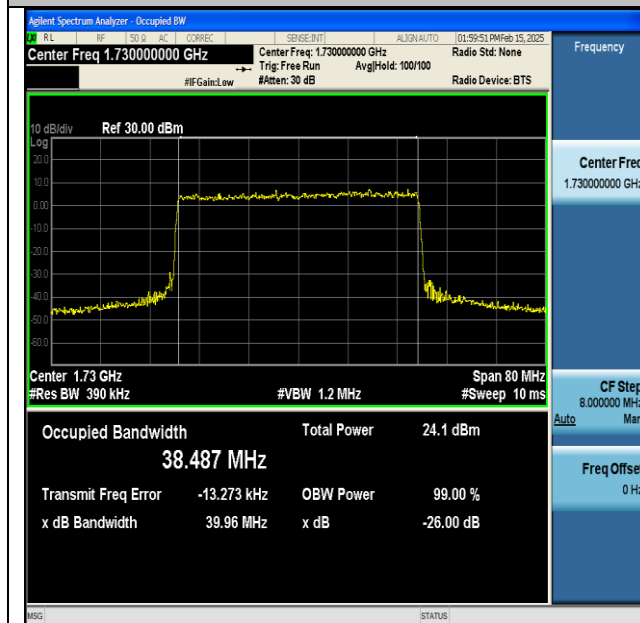
NTNV-DC_13A_n66A-PC3-15-5+40-M+L-QPSK-IDLE- DFT-256QAM-Outer_Full-Ant1-PASS
