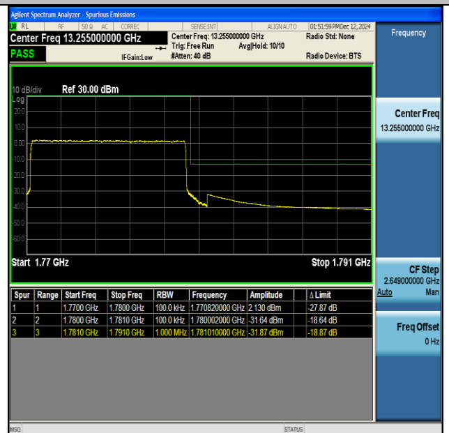
NTNV-DC_13A_n66A-PC3-15-5+10-M+H-QPSK-IDLE- CP-QPSK-Outer_Full-PASS
