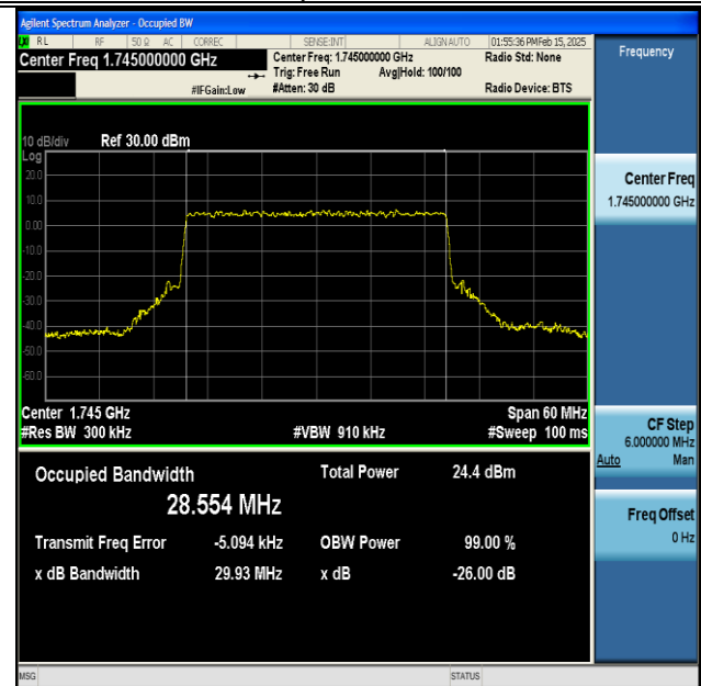
NTNV-DC_13A_n66A-PC3-15-5+30-M+M-QPSK-IDLE-CP-QPSK-Outet_Full-Ant1-PASS
