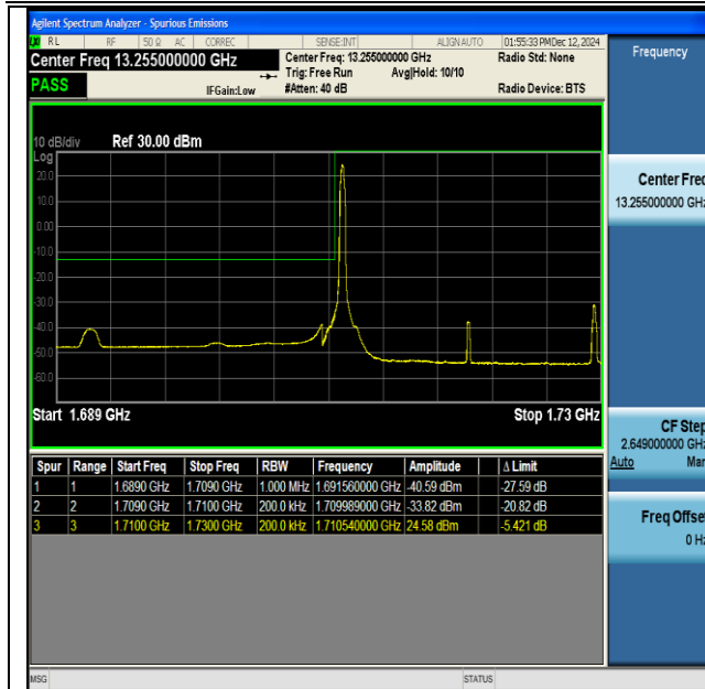
NTNV-DC_13A_n66A-PC3-15-5+20-M+L-QPSK-IDLE- DFT-BPSK-Edge_1RB_Left-PASS
