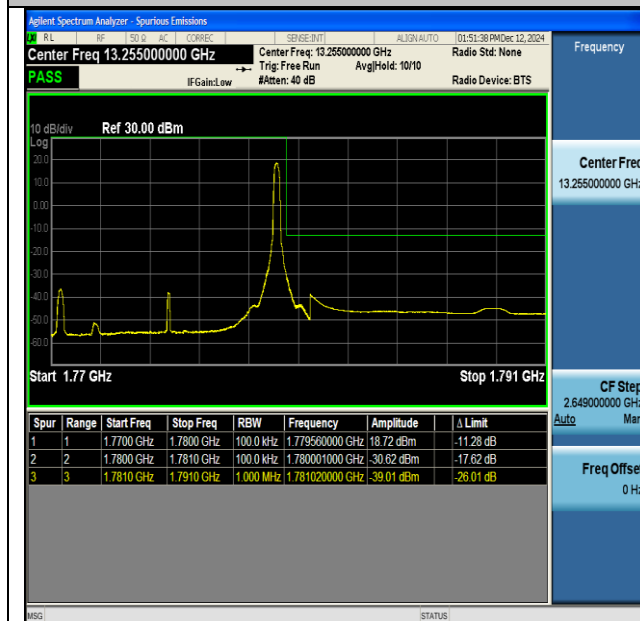
NTNV-DC_13A_n66A-PC3-15-5+10-M+H-QPSK-IDLE- CP-QPSK-Edge_1RB_Right-PASS
