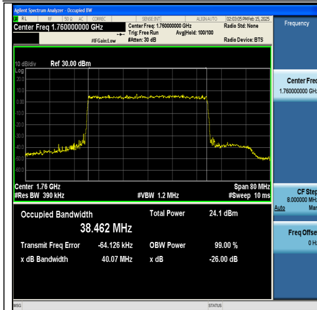
NTNV-DC_13A_n66A-PC3-15-5+40-M+H-QPSK-IDLE- DFT-256QAM-Outer_Full-Ant1-PASS
