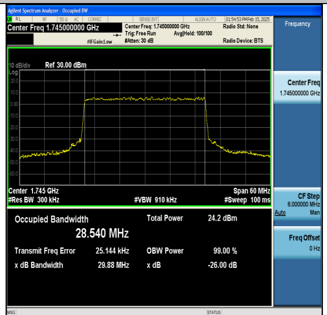
NTNV-DC_13A_n66A-PC3-15-5+30-M+M-QPSK-IDLE- DFT-64QAM-Outer_Full-Ant1-PASS
