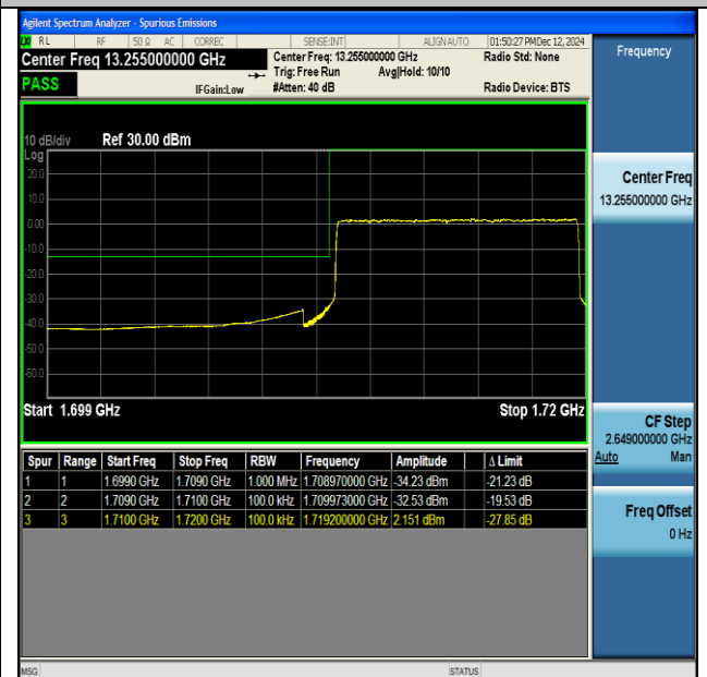
NTNV-DC_13A_n66A-PC3-15-5+10-M+L-QPSK-IDLE-CP- QPSK-Outer_Full-PASS
