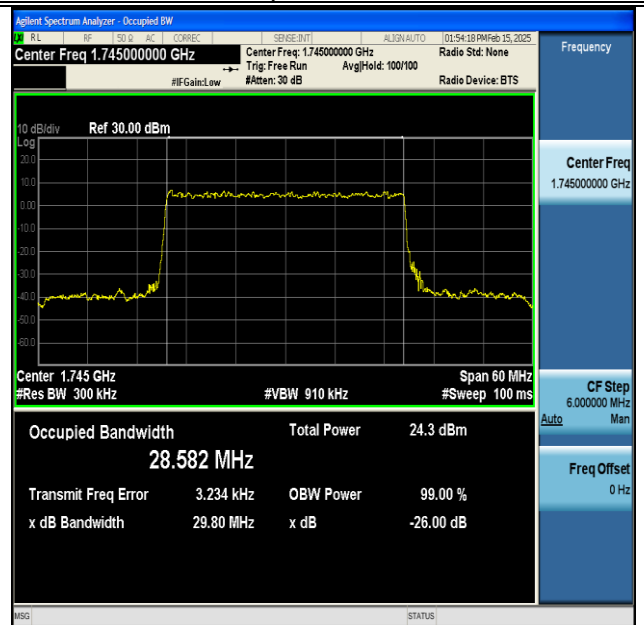
NTNV-DC_13A_n66A-PC3-15-5+30-M+M-QPSK-IDLE- DFT-QPSK-Outer_Full-Ant1-PASS
