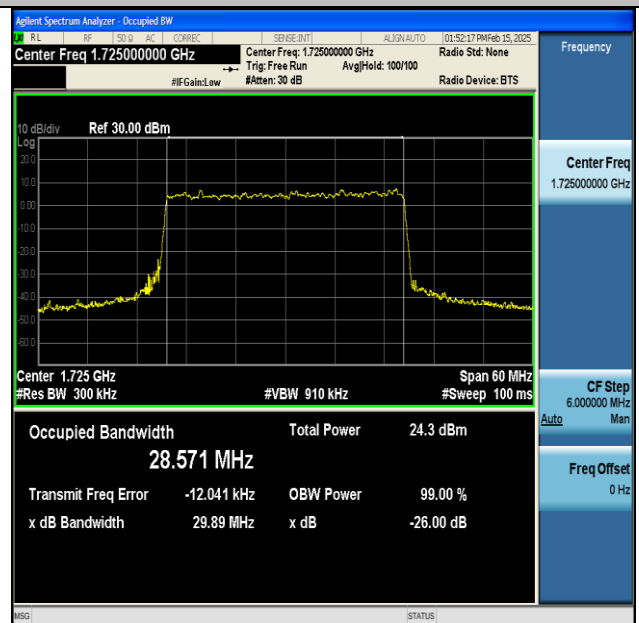
NTNV-DC_13A_n66A-PC3-15-5+30-M+L-QPSK-IDLE- DFT-256QAM-Outer_Full-Ant1-PASS
