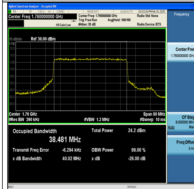
NTNV-DC_13A_n66A-PC3-15-5+40-M+H-QPSK-IDLE- CP-16QAM-Outer_Full-Ant1-PASS
