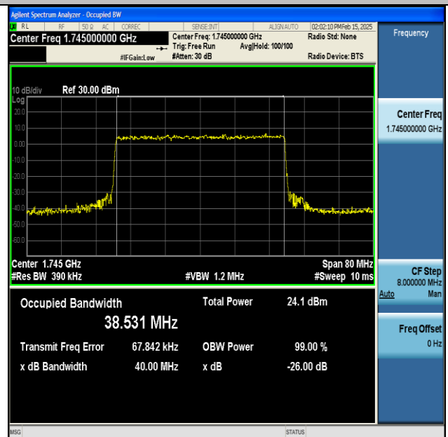
NTNV-DC_13A_n66A-PC3-15-5+40-M+M-QPSK-IDLE-CP-256QAM-Outer_Full-Ant1-PASS
