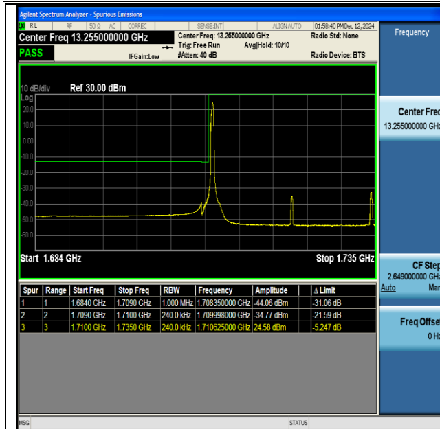
NTNV-DC_13A_n66A-PC3-15-5+25-M+L-QPSK-IDLE- DFT-BPSK-Edge_1RB_Left-PASS
