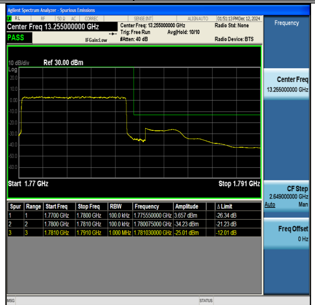
NTNV-DC_13A_n66A-PC3-15-5+10-M+H-QPSK-IDLE- DFT-BPSK-Outer_Full-PASS
