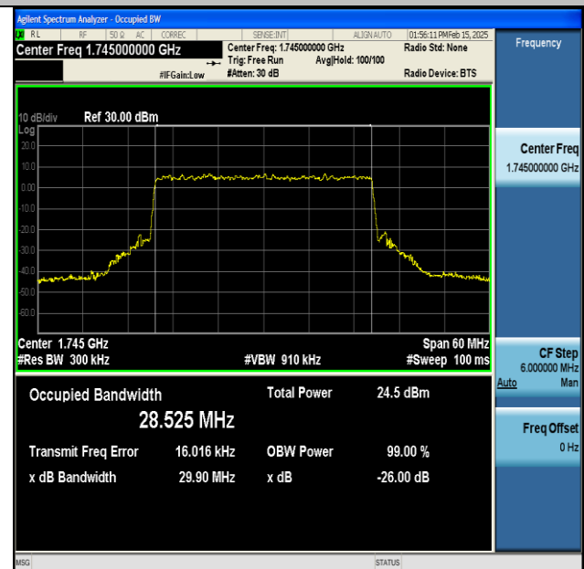
NTNV-DC_13A_n66A-PC3-15-5+30-M+M-QPSK-IDLE-CP-64QAM-Outet_Full-Ant1-PASS
