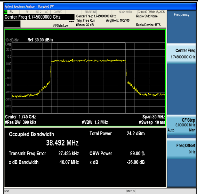
NTNV-DC_13A_n66A-PC3-15-5+40-M+M-QPSK-IDLE-CP-16QAM-Outer_Full-Ant1-PASS
