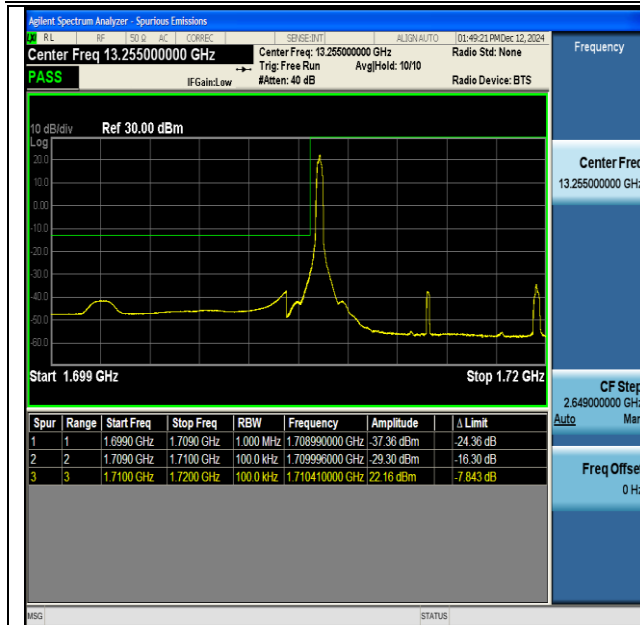
NTNV-DC_13A_n66A-PC3-15-5+10-M+L-QPSK-IDLE- DFT-BPSK-Edge_1RB_Left-PASS
