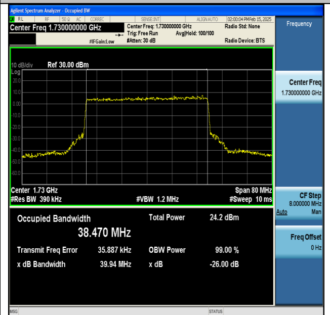
NTNV-DC_13A_n66A-PC3-15-5+40-M+L-QPSK-IDLE-CP- QPSK-Outer_Full-Ant1-PASS
