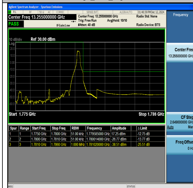
NTNV-DC_13A_n66A-PC3-15-5+5-M+H-QPSK-IDLE-CP- QPSK-Edge_1RB_Right-PASS
