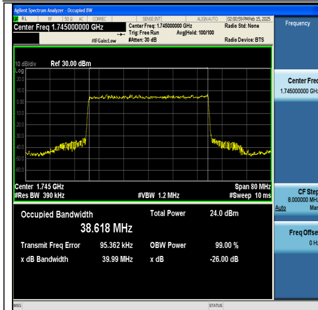
NTNV-DC_13A_n66A-PC3-15-5+40-M+M-QPSK-IDLE- DFT-QPSK-Outer_Full-Ant1-PASS
