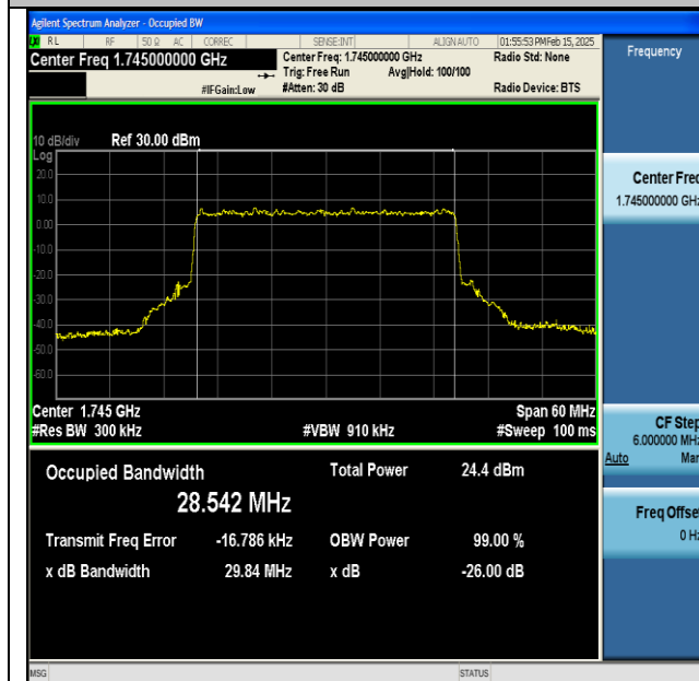
NTNV-DC_13A_n66A-PC3-15-5+30-M+M-QPSK-IDLE-CP-16QAM-Outet_Full-Ant1-PASS
