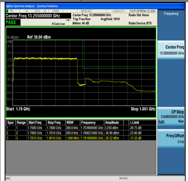
NTNV-DC_13A_n66A-PC3-15-5+20-M+H-QPSK-IDLE- DFT-BPSK-Outer_Full-PASS
