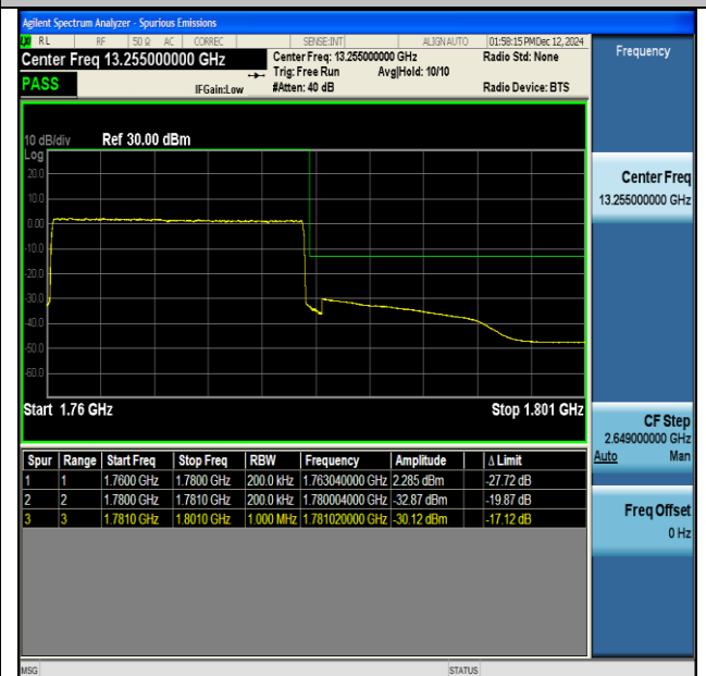
NTNV-DC_13A_n66A-PC3-15-5+20-M+H-QPSK-IDLE- CP-QPSK-Outer_Full-PASS
