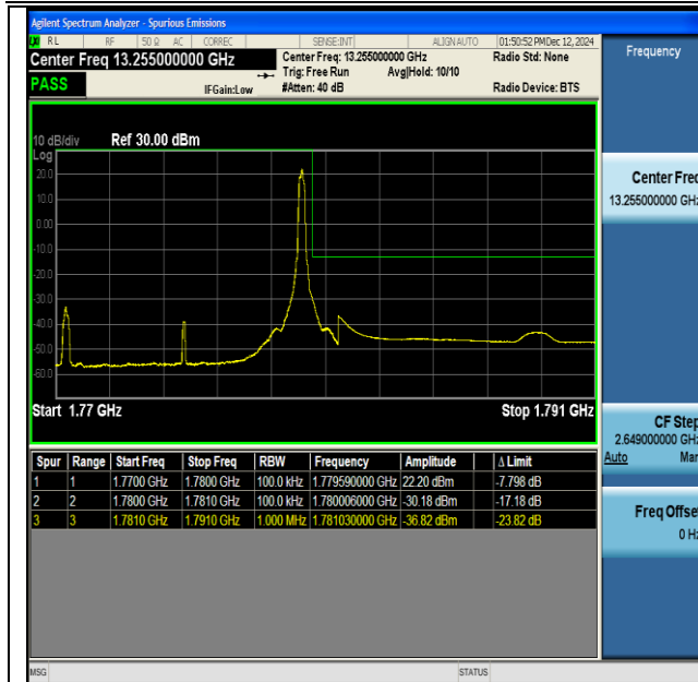
NTNV-DC_13A_n66A-PC3-15-5+10-M+H-QPSK-IDLE- DFT-BPSK-Edge_1RB_Right-PASS
