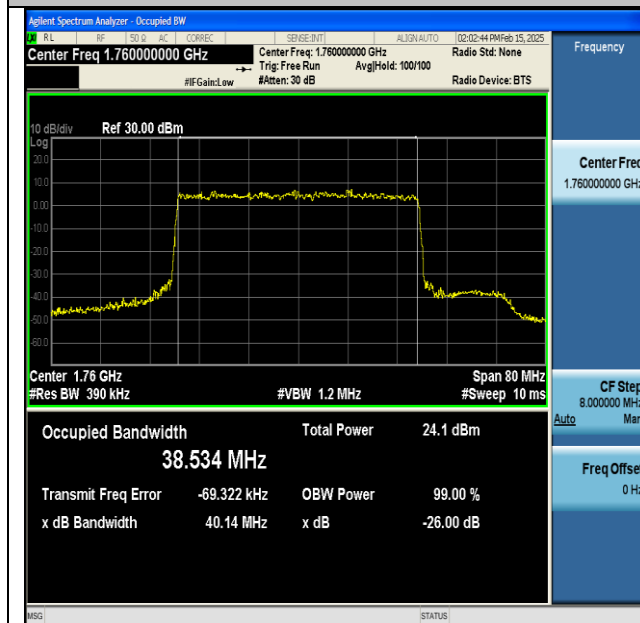
NTNV-DC_13A_n66A-PC3-15-5+40-M+H-QPSK-IDLE- DFT-16QAM-Outer_Full-Ant1-PASS
