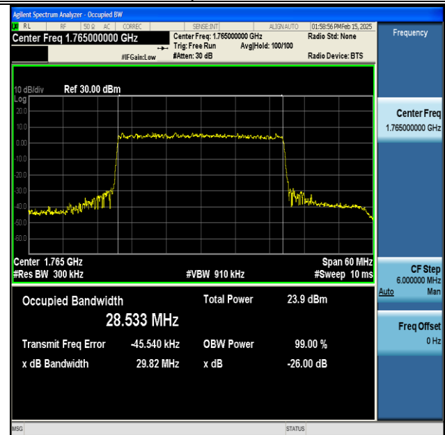
NTNV-DC_13A_n66A-PC3-15-5+30-M+H-QPSK-IDLE-CP-256QAM-Outet_Full-Ant1-PASS
