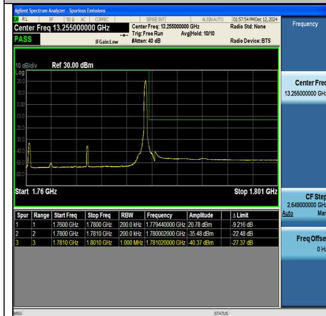
NTNV-DC_13A_n66A-PC3-15-5+20-M+H-QPSK-IDLE- CP-QPSK-Edge_1RB_Right-PASS
