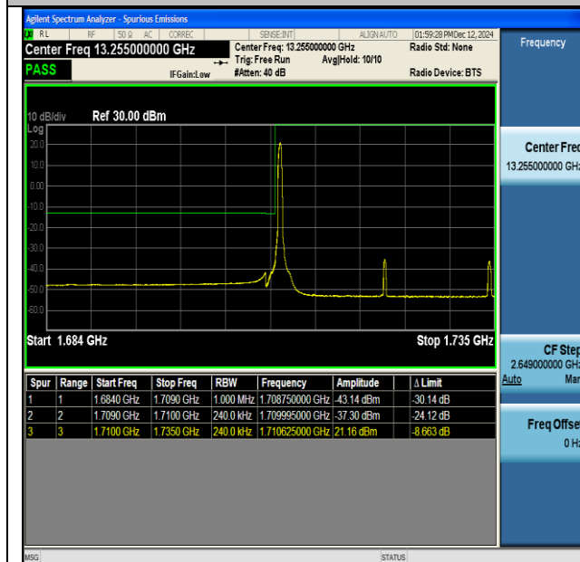
NTNV-DC_13A_n66A-PC3-15-5+25-M+L-QPSK-IDLE-CP- QPSK-Edge_1RB_Left-PASS
