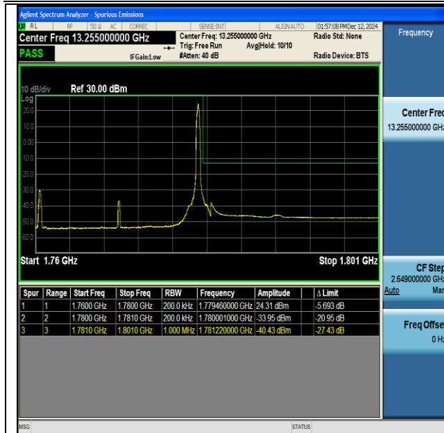
NTNV-DC_13A_n66A-PC3-15-5+20-M+H-QPSK-IDLE- DFT-BPSK-Edge_1RB_Right-PASS
