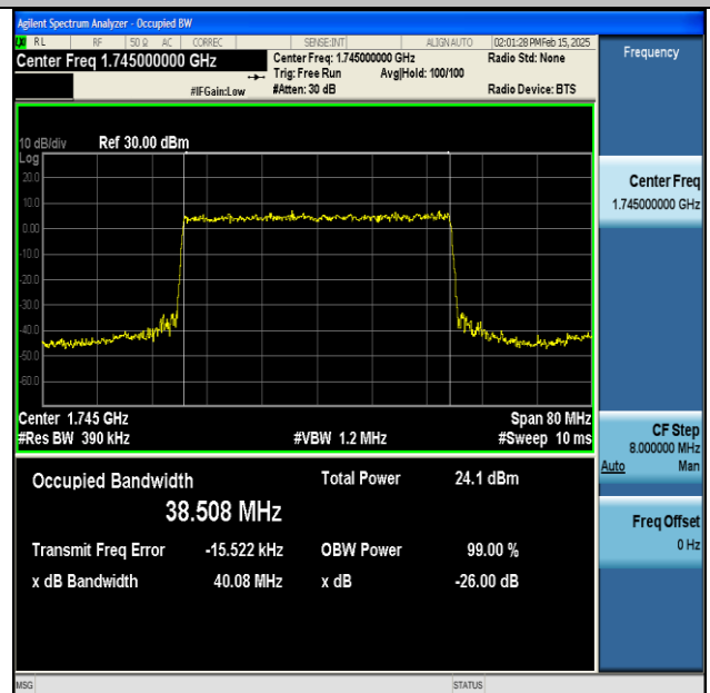
NTNV-DC_13A_n66A-PC3-15-5+40-M+M-QPSK-IDLE- DFT-256QAM-Outer_Full-Ant1-PASS
