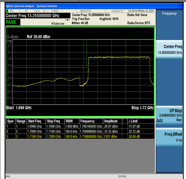
NTNV-DC_13A_n66A-PC3-15-5+10-M+L-QPSK-IDLE- DFT-BPSK-Outer_Full-PASS
