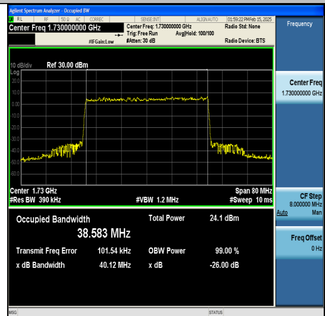
NTNV-DC_13A_n66A-PC3-15-5+40-M+L-QPSK-IDLE-DFT-QPSK-Outet_Full-Ant1-PASS
