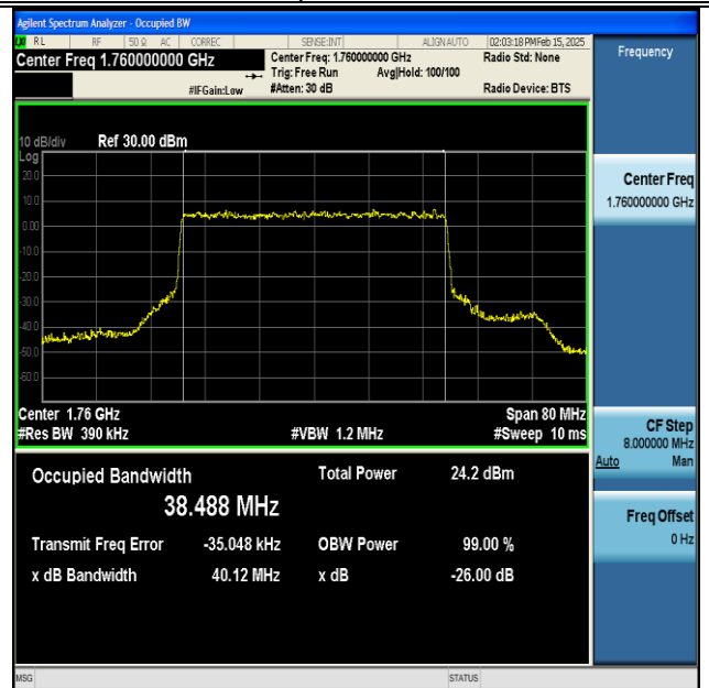
NTNV-DC_13A_n66A-PC3-15-5+40-M+H-QPSK-IDLE- CP-QPSK-Outer_Full-Ant1-PASS
