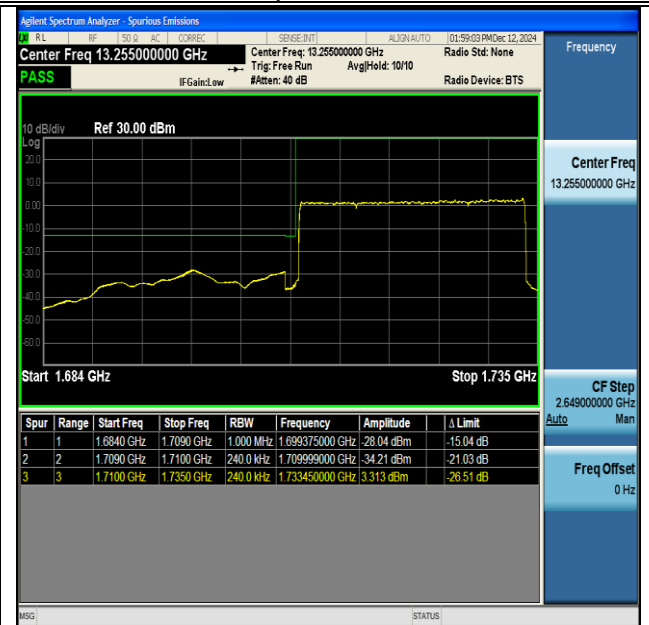
NTNV-DC_13A_n66A-PC3-15-5+25-M+L-QPSK-IDLE- DFT-BPSK-Outer_Full-PASS
