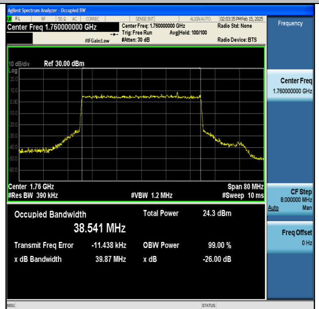
NTNV-DC_13A_n66A-PC3-15-5+40-M+H-QPSK-IDLE- CP-64QAM-Outer_Full-Ant1-PASS
