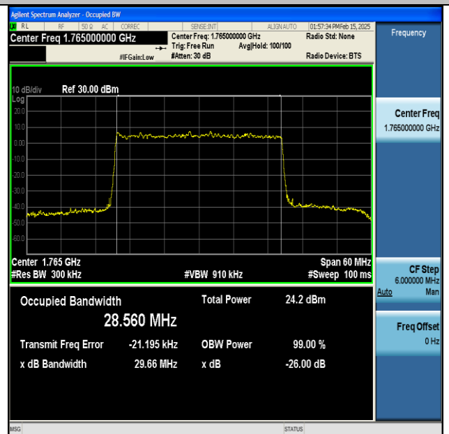
NTNV-DC_13A_n66A-PC3-15-5+30-M+H-QPSK-IDLE-DFT-16QAM-Outer_Full-Ant1-PASS
