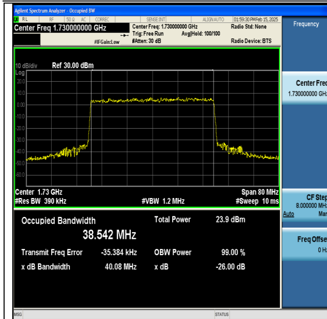
NTNV-DC_13A_n66A-PC3-15-5+40-M+L-QPSK-IDLE- DFT-16QAM-Outer_Full-Ant1-PASS
