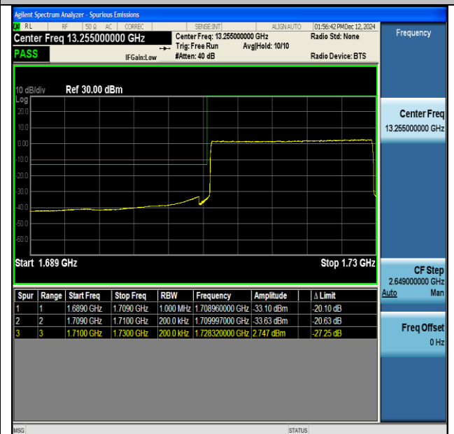
NTNV-DC_13A_n66A-PC3-15-5+20-M+L-QPSK-IDLE-CP- QPSK-Outer_Full-PASS
