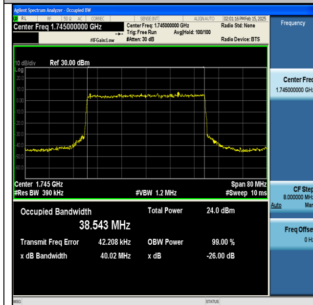
NTNV-DC_13A_n66A-PC3-15-5+40-M+M-QPSK-IDLE- DFT-64QAM-Outer_Full-Ant1-PASS
