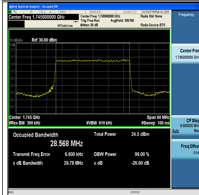
NTNV-DC_13A_n66A-PC3-15-5+30-M+M-QPSK-IDLE- DFT-BPSK-Outer_Full-Ant1-PASS
