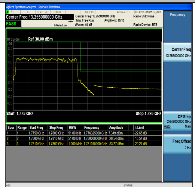
NTNV-DC_13A_n66A-PC3-15-5+5-M+H-QPSK-IDLE-CP- QPSK-Outer_Full-PASS
