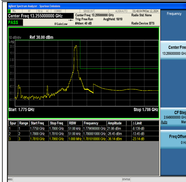
NTNV-DC_13A_n66A-PC3-15-5+5-M+H-QPSK-IDLE-DFT- BPSK-Edge_1RB_Right-PASS
