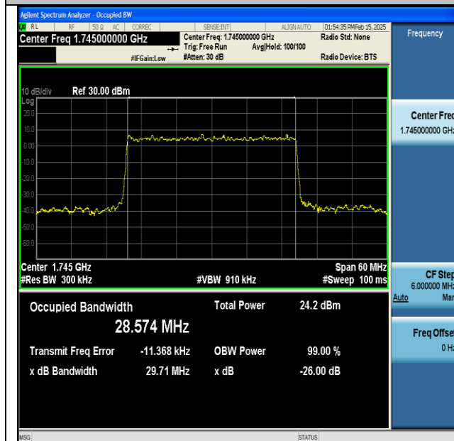
NTNV-DC_13A_n66A-PC3-15-5+30-M+M-QPSK-IDLE- DFT-16QAM-Outer_Full-Ant1-PASS
