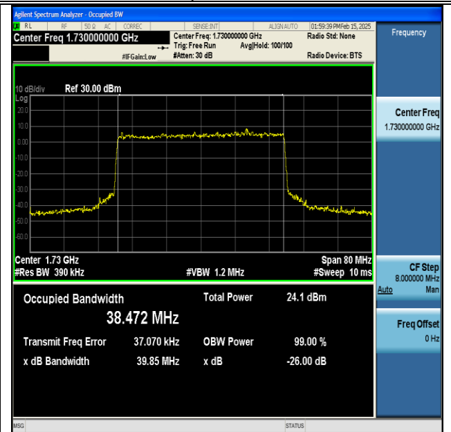
NTNV-DC_13A_n66A-PC3-15-5+40-M+L-QPSK-IDLE- DFT-64QAM-Outer_Full-Ant1-PASS
