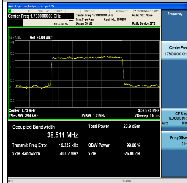
NTNV-DC_13A_n66A-PC3-15-5+40-M+L-QPSK-IDLE-DFT-BPSK-Outet_Full-Ant1-PASS
