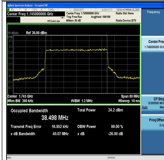
NTNV-DC_13A_n66A-PC3-15-5+40-M+M-QPSK-IDLE-CP-QPSK-Outer_Full-Ant1-PASS
