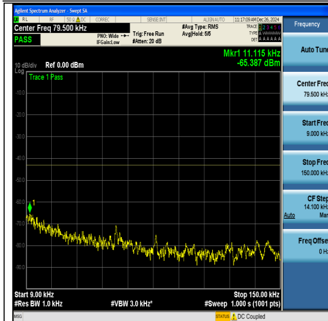
NTNV-DC_13A_n66A-PC3-15-5+40-M+M-QPSK-IDLE- DFT-BPSK-Inner_1RB_Left-0.009-0.15-PASS
