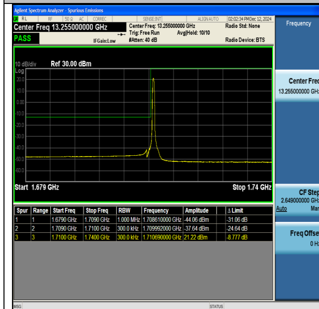
NTNV-DC_13A_n66A-PC3-15-5+30-M+L-QPSK-IDLE-CP- QPSK-Edge_1RB_Left-PASS
