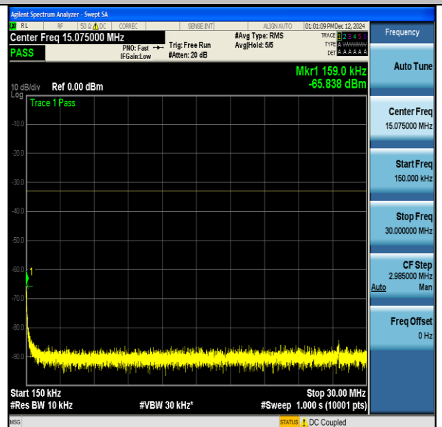
NTNV-DC_13A_n66A-PC3-15-5+40-M+M-QPSK-IDLE- CP-QPSK-Inner_1RB_Left-0.15-30-PASS
