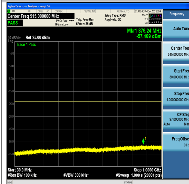
NTNV-DC_13A_n66A-PC3-15-5+40-M+H-QPSK-IDLE- DFT-BPSK-Inner_1RB_Left-30-1000-PASS
