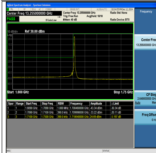
NTNV-DC_13A_n66A-PC3-15-5+40-M+L-QPSK-IDLE-DFT-BPSK-Edge_1RB_Left-PASS
