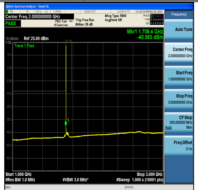
NTNV-DC_13A_n66A-PC3-15-5+40-M+L-QPSK-IDLE-CP- QPSK-Inner_1RB_Left-1000-3000-PASS
