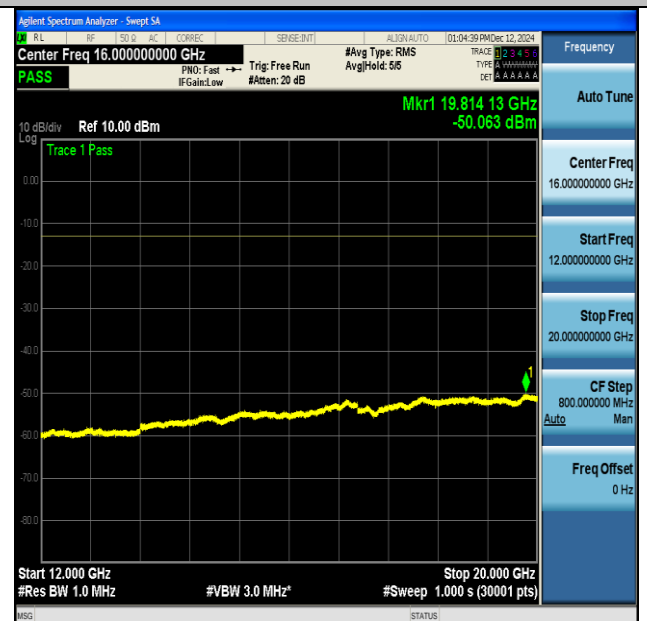
NTNV-DC_13A_n66A-PC3-15-5+40-M+H-QPSK-IDLE- CP-QPSK-Inner_1RB_Left-12000-20000-PASS
