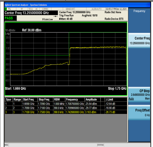
NTNV-DC_13A_n66A-PC3-15-5+40-M+L-QPSK-IDLE-DFT-BPSK-Outer_Full-PASS
