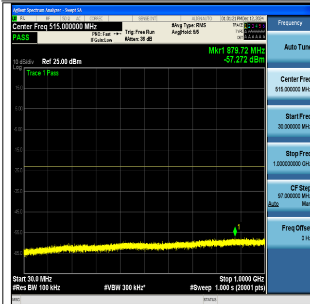
NTNV-DC_13A_n66A-PC3-15-5+40-M+M-QPSK-IDLE- CP-QPSK-Inner_1RB_Left-30-1000-PASS
