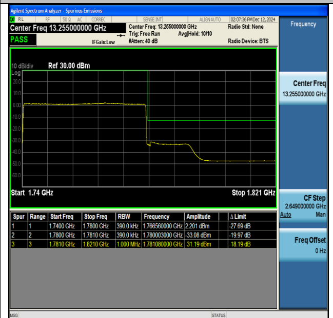
NTNV-DC_13A_n66A-PC3-15-5+40-M+H-QPSK-IDLE- CP-QPSK-Outer_Full-PASS
