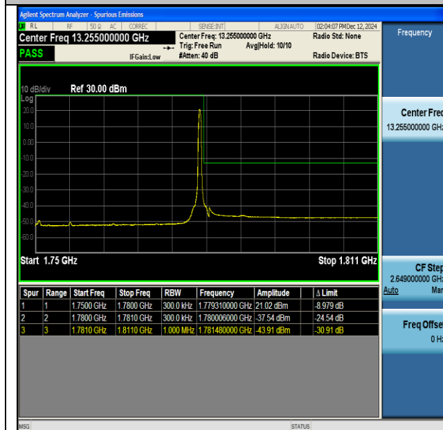
NTNV-DC_13A_n66A-PC3-15-5+30-M+H-QPSK-IDLE- CP-QPSK-Edge_1RB_Right-PASS
