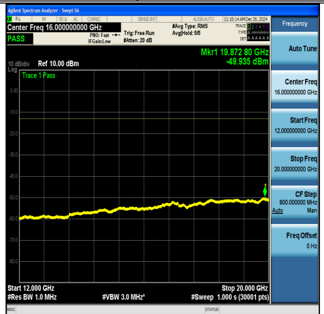
NTNV-DC_13A_n66A-PC3-15-5+40-M+M-QPSK-IDLE- DFT-BPSK-Inner_1RB_Left-12000-20000-PASS
