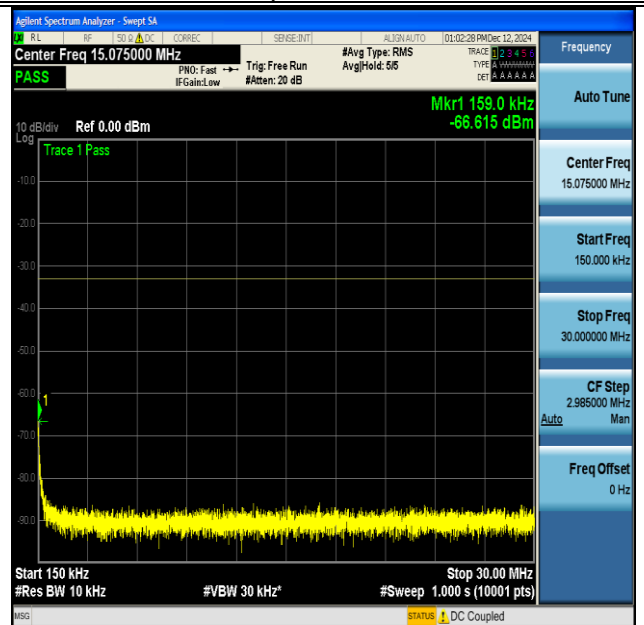
NTNV-DC_13A_n66A-PC3-15-5+40-M+H-QPSK-IDLE- DFT-BPSK-Inner_1RB_Left-0.15-30-PASS
