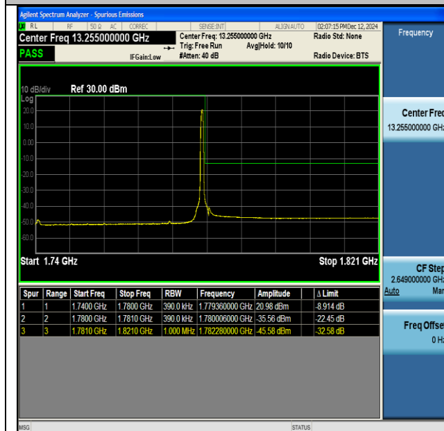
NTNV-DC_13A_n66A-PC3-15-5+40-M+H-QPSK-IDLE- CP-QPSK-Edge_1RB_Right-PASS
