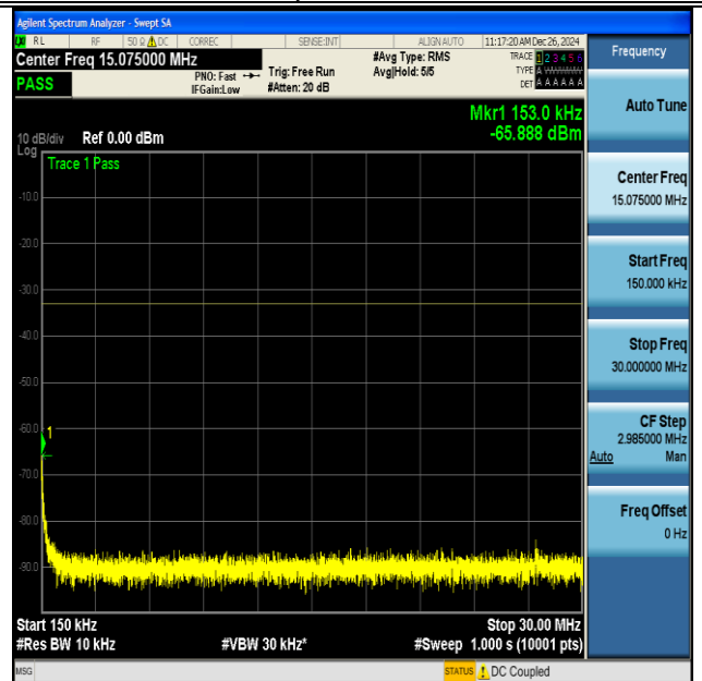
NTNV-DC_13A_n66A-PC3-15-5+40-M+M-QPSK-IDLE- DFT-BPSK-Inner_1RB_Left-0.15-30-PASS
