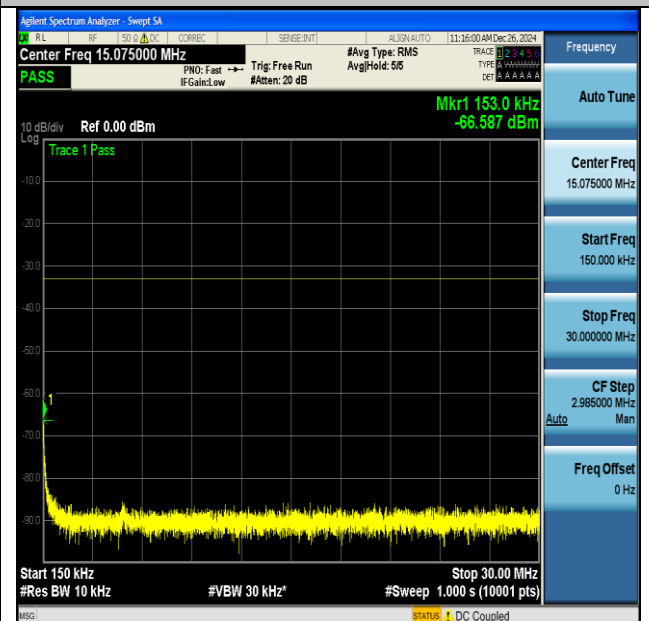
NTNV-DC_13A_n66A-PC3-15-5+40-M+L-QPSK-IDLE-CP-QPSK-Inner_1RB_Left-0.15-30-PASS
