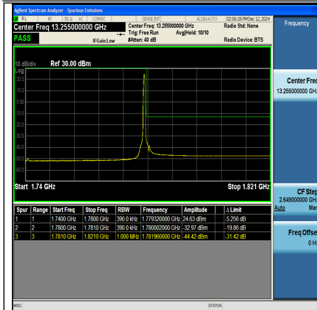
NTNV-DC_13A_n66A-PC3-15-5+40-M+H-QPSK-IDLE- DFT-BPSK-Edge_1RB_Right-PASS
