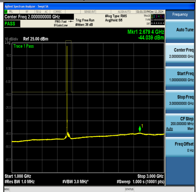
NTNV-DC_13A_n66A-PC3-15-5+40-M+M-QPSK-IDLE- CP-QPSK-Inner_1RB_Left-1000-3000-PASS
