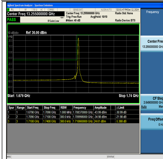
NTNV-DC_13A_n66A-PC3-15-5+30-M+L-QPSK-IDLE- DFT-BPSK-Edge_1RB_Left-PASS
