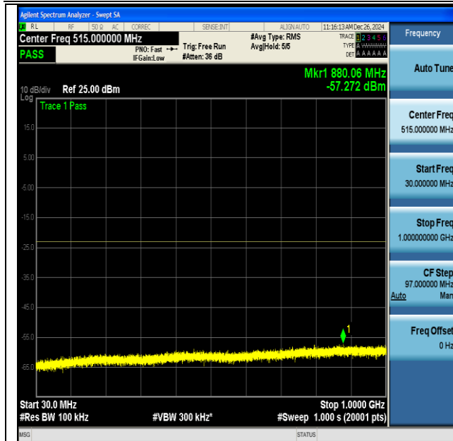
NTNV-DC_13A_n66A-PC3-15-5+40-M+L-QPSK-IDLE-CP- QPSK-Inner_1RB_Left-30-1000-PASS
