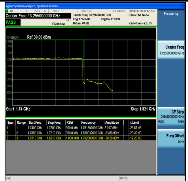
NTNV-DC_13A_n66A-PC3-15-5+40-M+H-QPSK-IDLE- DFT-BPSK-Outer_Full-PASS
