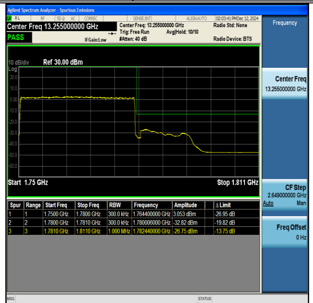
NTNV-DC_13A_n66A-PC3-15-5+30-M+H-QPSK-IDLE- DFT-BPSK-Outer_Full-PASS
