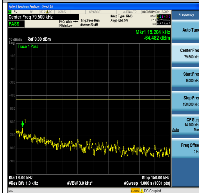
NTNV-DC_13A_n66A-PC3-15-5+40-M+M-QPSK-IDLE- CP-QPSK-Inner_1RB_Left-0.009-0.15-PASS
