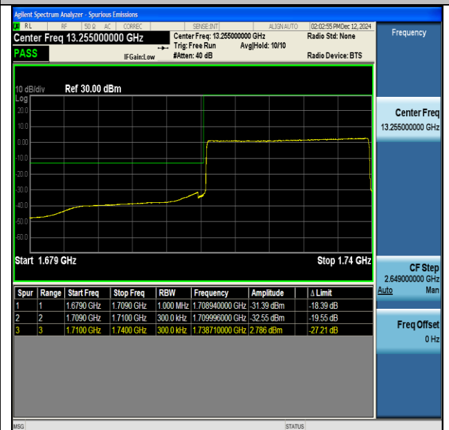
NTNV-DC_13A_n66A-PC3-15-5+30-M+L-QPSK-IDLE-CP- QPSK-Outer_Full-PASS
