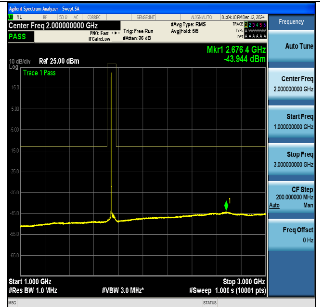
NTNV-DC_13A_n66A-PC3-15-5+40-M+H-QPSK-IDLE- CP-QPSK-Inner_1RB_Left-1000-3000-PASS
