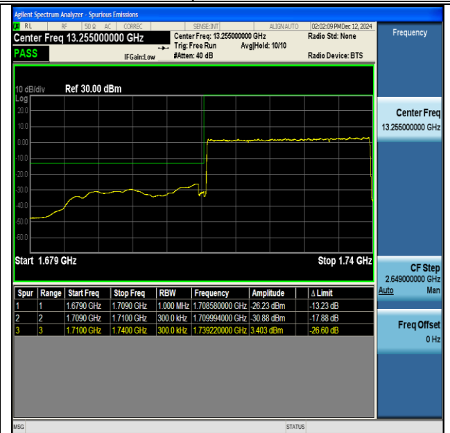
NTNV-DC_13A_n66A-PC3-15-5+30-M+L-QPSK-IDLE- DFT-BPSK-Outer_Full-PASS
