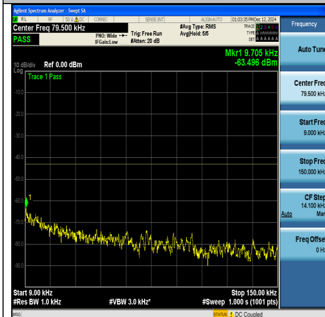
NTNV-DC_13A_n66A-PC3-15-5+40-M+H-QPSK-IDLE- CP-QPSK-Inner_1RB_Left-0.009-0.15-PASS
