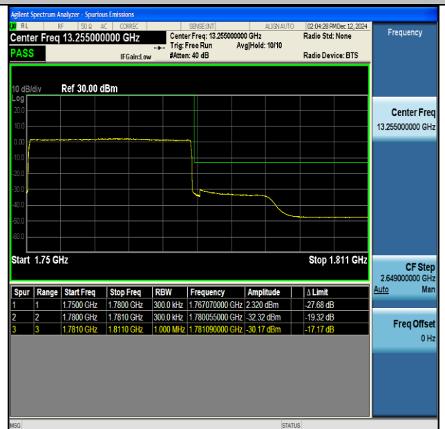
NTNV-DC_13A_n66A-PC3-15-5+30-M+H-QPSK-IDLE- CP-QPSK-Outer_Full-PASS
