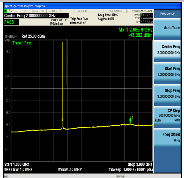
NTNV-DC_13A_n66A-PC3-15-5+40-M+M-QPSK-IDLE- DFT-BPSK-Inner_1RB_Left-1000-3000-PASS
