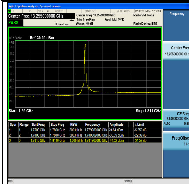
NTNV-DC_13A_n66A-PC3-15-5+30-M+H-QPSK-IDLE- DFT-BPSK-Edge_1RB_Right-PASS
