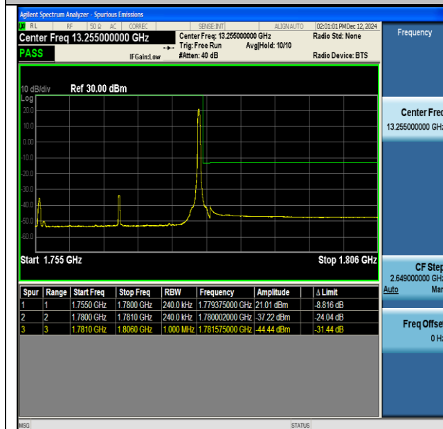
NTNV-DC_13A_n66A-PC3-15-5+25-M+H-QPSK-IDLE- CP-QPSK-Edge_1RB_Right-PASS
