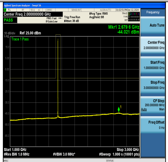
NTNV-DC_13A_n66A-PC3-15-5+40-M+H-QPSK-IDLE- DFT-BPSK-Inner_1RB_Left-1000-3000-PASS
