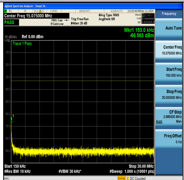
NTNV-DC_13A_n66A-PC3-15-5+40-M+H-QPSK-IDLE- CP-QPSK-Inner_1RB_Left-0.15-30-PASS
