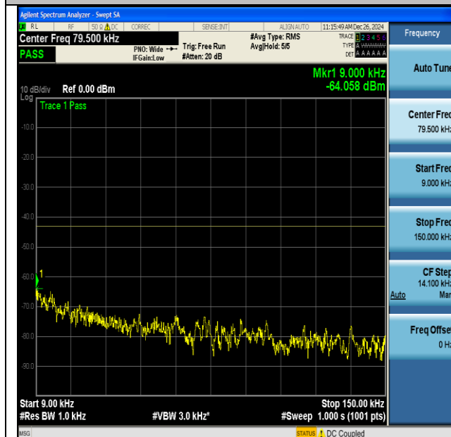
NTNV-DC_13A_n66A-PC3-15-5+40-M+L-QPSK-IDLE-CP-QPSK-Inner_1RB_Left-0.009-0.15-PASS
