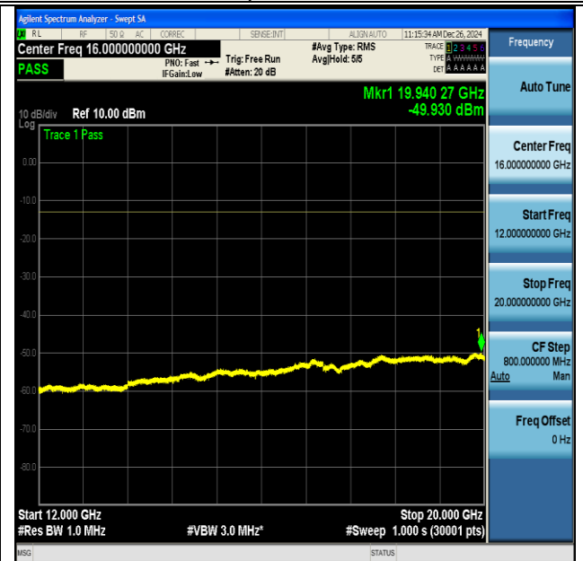
NTNV-DC_13A_n66A-PC3-15-5+40-M+L-QPSK-IDLE-DFT-BPSK-Inner_1RB_Left-12000-20000-PASS
