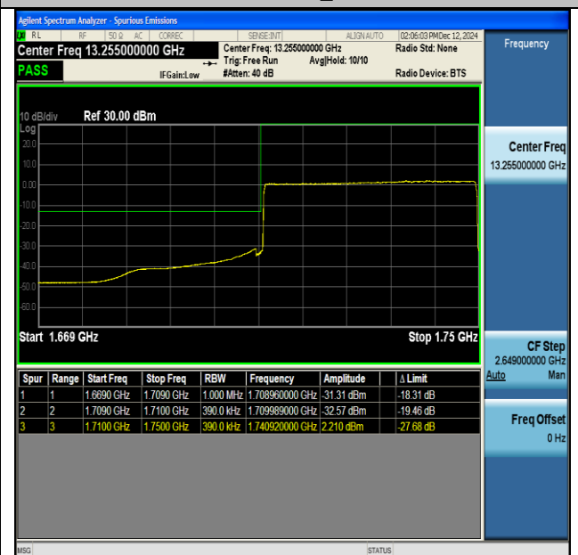
NTNV-DC_13A_n66A-PC3-15-5+40-M+L-QPSK-IDLE-CP-QPSK-Outer_Full-PASS
