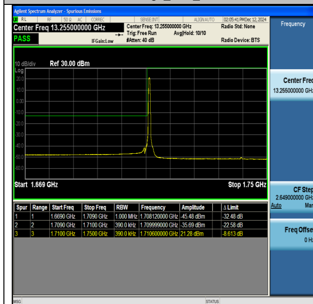
NTNV-DC_13A_n66A-PC3-15-5+40-M+L-QPSK-IDLE-CP-QPSK-Edge_1RB_Left-PASS
