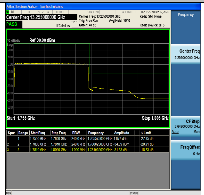
NTNV-DC_13A_n66A-PC3-15-5+25-M+H-QPSK-IDLE- CP-QPSK-Outer_Full-PASS
