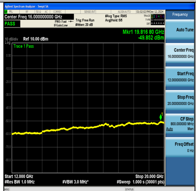
NTNV-DC_13A_n66A-PC3-15-5+40-M+M-QPSK-IDLE- CP-QPSK-Inner_1RB_Left-12000-20000-PASS
