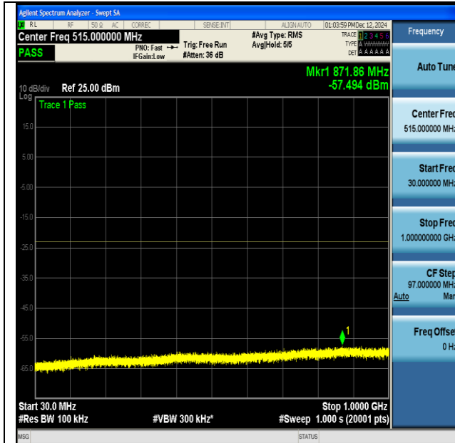
NTNV-DC_13A_n66A-PC3-15-5+40-M+H-QPSK-IDLE- CP-QPSK-Inner_1RB_Left-30-1000-PASS
