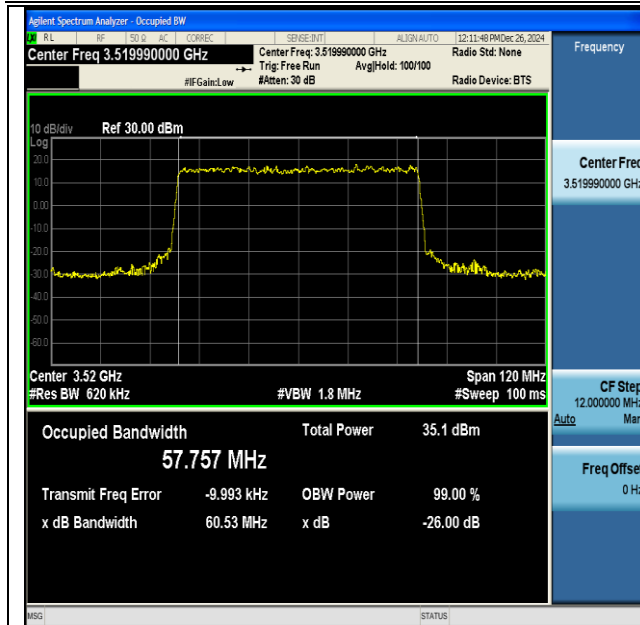
NTNV-DC_41A_n77A(3450-3550)-PC3-30-5+60-M+H- QPSK-IDLE-DFT-QPSK-Outer_Full-Ant1-PASS
