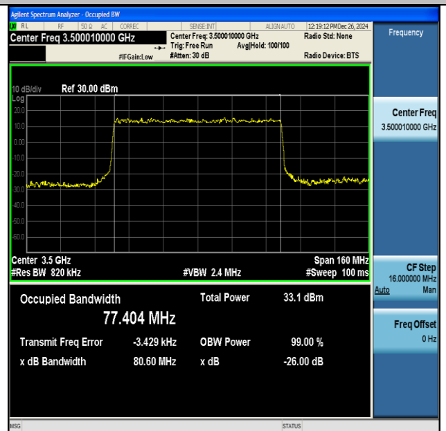
NTNV-DC_41A_n77A(3450-3550)-PC3-30-5+80-M+M- QPSK-IDLE-CP-16QAM-Outer_Full-Ant1-PASS
