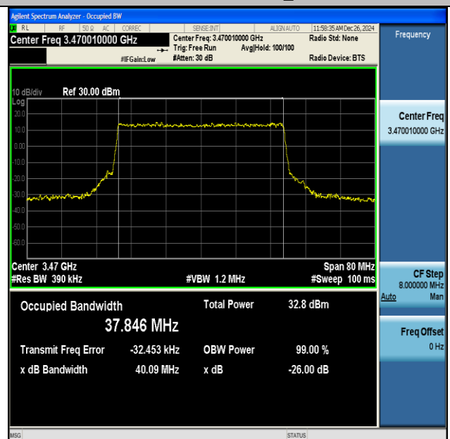
NTNV-DC_41A_n77A(3450-3550)-PC3-30-5+40-M+L- QPSK-IDLE-CP-QPSK-Outer_Full-Ant1-PASS
