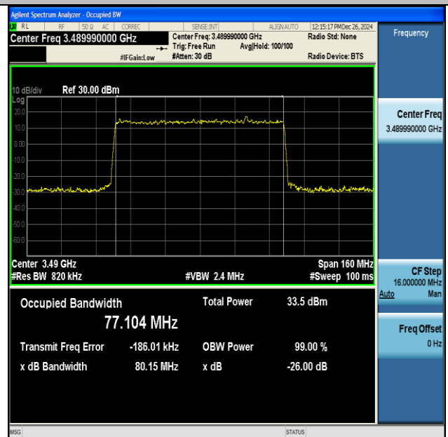
NTNV-DC_41A_n77A(3450-3550)-PC3-30-5+80-M+L-QPSK-IDLE-DFT-64QAM-Outer_Full-Ant1-PASS
