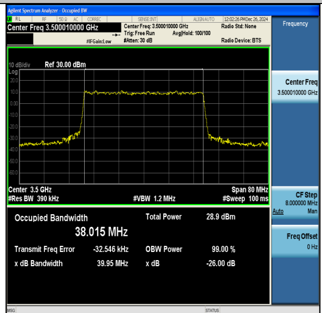
NTNV-DC_41A_n77A(3450-3550)-PC3-30-5+40-M+M- QPSK-IDLE-CP-256QAM-Outer_Full-Ant1-PASS
