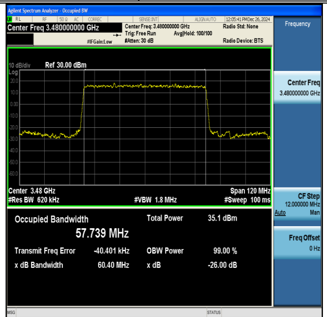
NTNV-DC_41A_n77A(3450-3550)-PC3-30-5+60-M+L- QPSK-IDLE-DFT-BPSK-Outer_Full-Ant1-PASS
