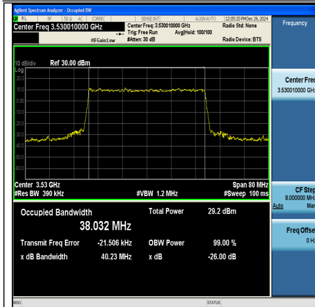
NTNV-DC_41A_n77A(3450-3550)-PC3-30-5+40-M+H- QPSK-IDLE-CP-256QAM-Outer_Full-Ant1-PASS
