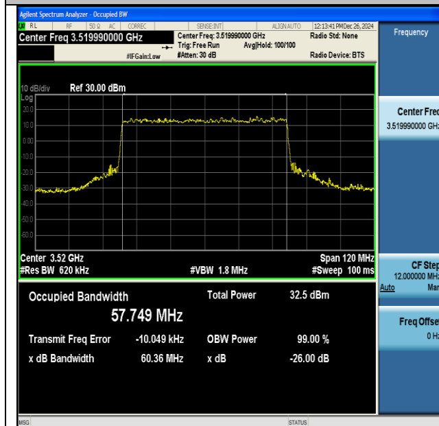
NTNV-DC_41A_n77A(3450-3550)-PC3-30-5+60-M+H- QPSK-IDLE-CP-64QAM-Outer_Full-Ant1-PASS
