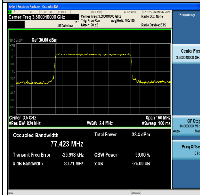
NTNV-DC_41A_n77A(3450-3550)-PC3-30-5+80-M+M- QPSK-IDLE-CP-QPSK-Outer_Full-Ant1-PASS
