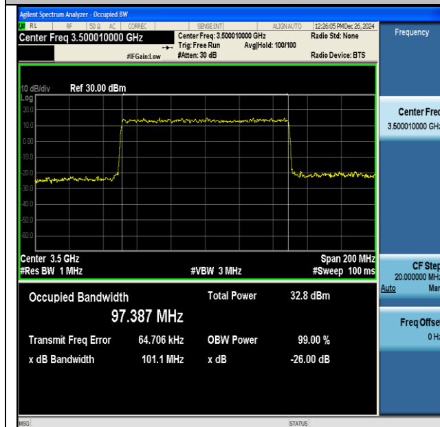
NTNV-DC_41A_n77A(3450-3550)-PC3-30-5+100-M+L- QPSK-IDLE-CP-64QAM-Outer_Full-Ant1-PASS
