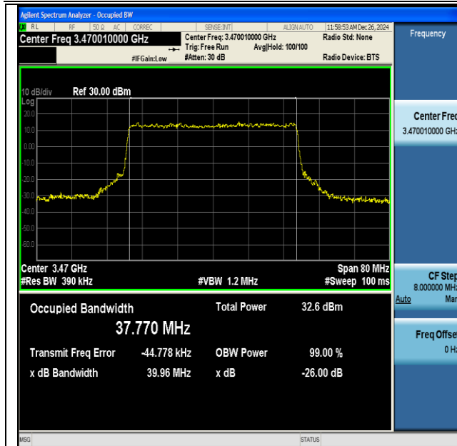
NTNV-DC_41A_n77A(3450-3550)-PC3-30-5+40-M+L- QPSK-IDLE-CP-16QAM-Outer_Full-Ant1-PASS
