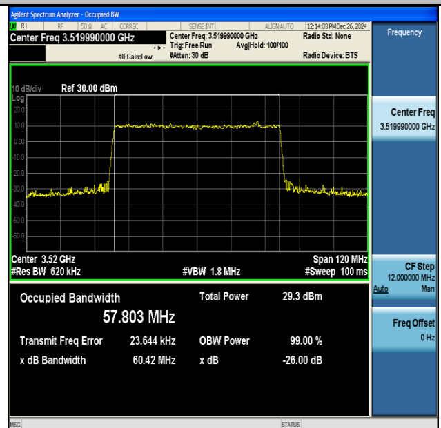
NTNV-DC_41A_n77A(3450-3550)-PC3-30-5+60-M+H- QPSK-IDLE-CP-256QAM-Outer_Full-Ant1-PASS
