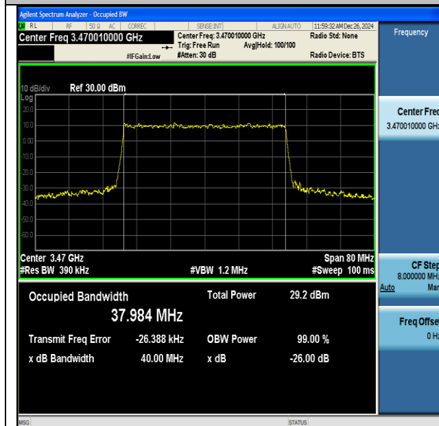
NTNV-DC_41A_n77A(3450-3550)-PC3-30-5+40-M+L- QPSK-IDLE-CP-256QAM-Outer_Full-Ant1-PASS
