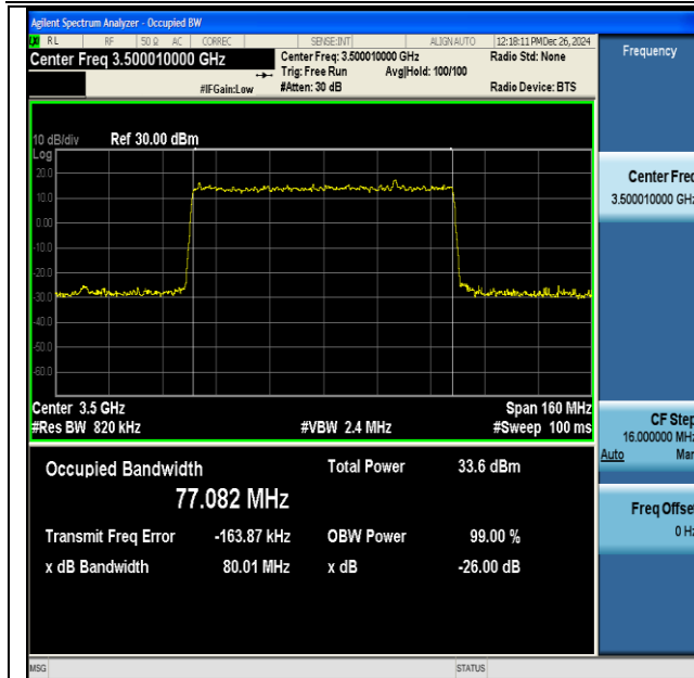
NTNV-DC_41A_n77A(3450-3550)-PC3-30-5+80-M+M- QPSK-IDLE-DFT-64QAM-Outer_Full-Ant1-PASS
