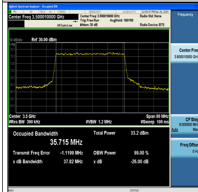
NTNV-DC_41A_n77A(3450-3550)-PC3-30-5+40-M+M- QPSK-IDLE-DFT-64QAM-Outer_Full-Ant1-PASS
