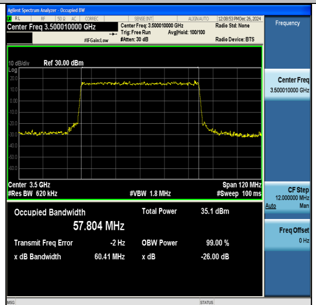
NTNV-DC_41A_n77A(3450-3550)-PC3-30-5+60-M+M- QPSK-IDLE-DFT-QPSK-Outer_Full-Ant1-PASS
