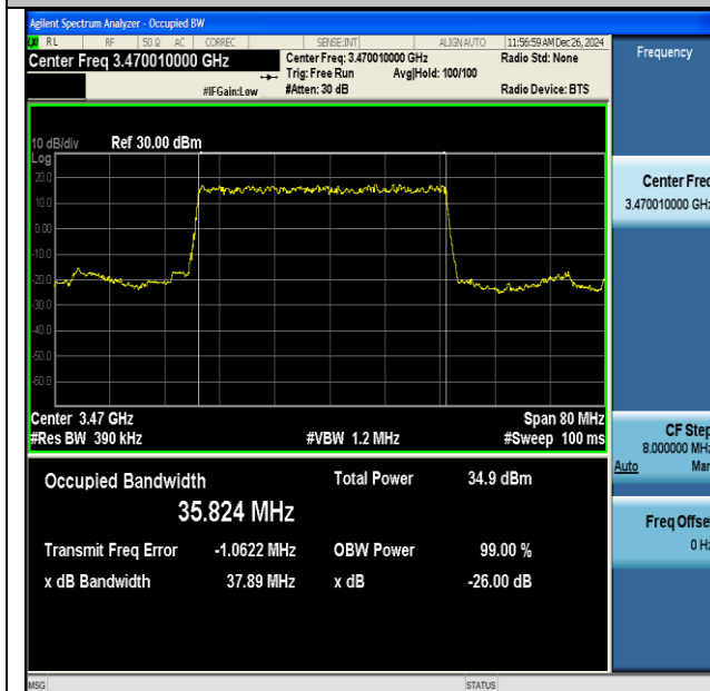
NTNV-DC_41A_n77A(3450-3550)-PC3-30-5+40-M+L- QPSK-IDLE-DFT-BPSK-Outer_Full-Ant1-PASS
