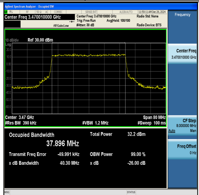
NTNV-DC_41A_n77A(3450-3550)-PC3-30-5+40-M+L- QPSK-IDLE-CP-64QAM-Outer_Full-Ant1-PASS
