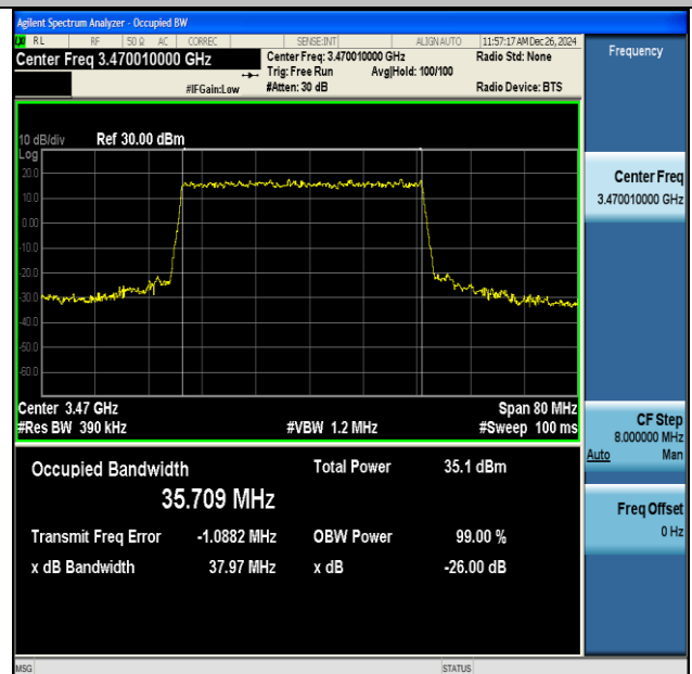
NTNV-DC_41A_n77A(3450-3550)-PC3-30-5+40-M+L- QPSK-IDLE-DFT-QPSK-Outer_Full-Ant1-PASS
