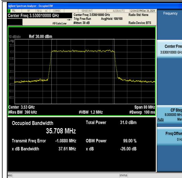
NTNV-DC_41A_n77A(3450-3550)-PC3-30-5+40-M+H- QPSK-IDLE-DFT-256QAM-Outer_Full-Ant1-PASS
