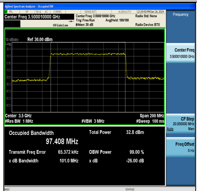
NTNV-DC_41A_n77A(3450-3550)-PC3-30-5+100-M+M- QPSK-IDLE-CP-64QAM-Outer_Full-Ant1-PASS
