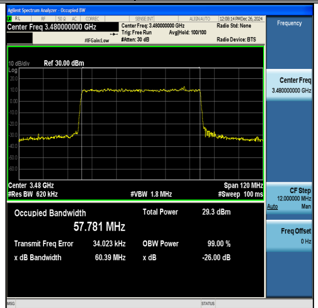
NTNV-DC_41A_n77A(3450-3550)-PC3-30-5+60-M+L- QPSK-IDLE-CP-256QAM-Outer_Full-Ant1-PASS
