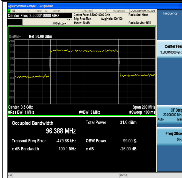
NTNV-DC_41A_n77A(3450-3550)-PC3-30-5+100-M+M- QPSK-IDLE-DFT-256QAM-Outer_Full-Ant1-PASS
