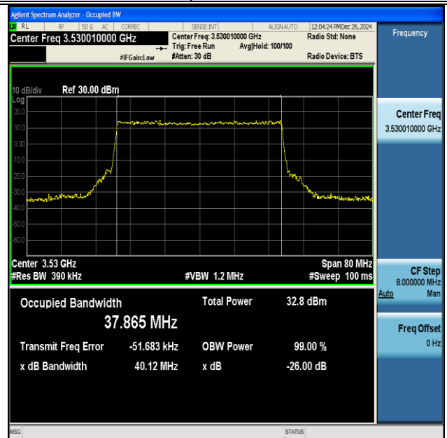
NTNV-DC_41A_n77A(3450-3550)-PC3-30-5+40-M+H- QPSK-IDLE-CP-QPSK-Outer_Full-Ant1-PASS
