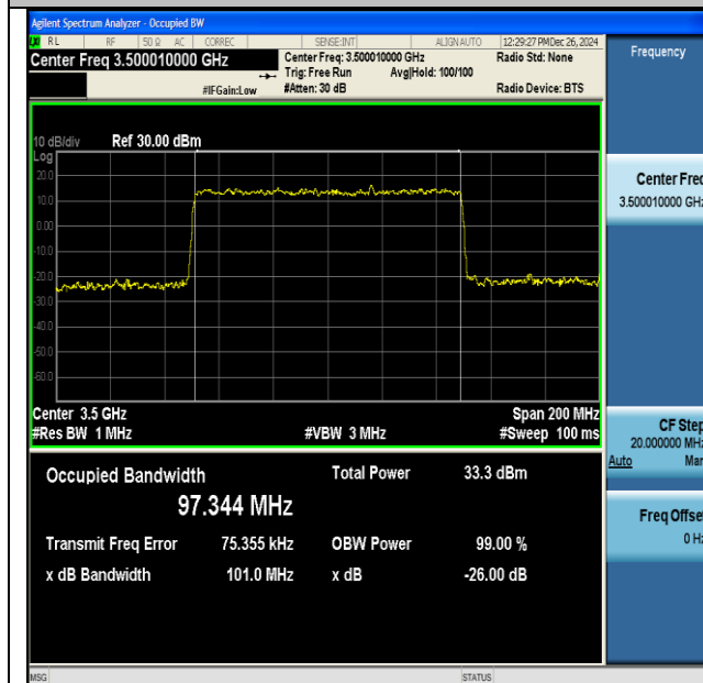
NTNV-DC_41A_n77A(3450-3550)-PC3-30-5+100-M+M- QPSK-IDLE-CP-16QAM-Outer_Full-Ant1-PASS
