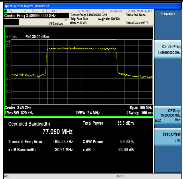
NTNV-DC_41A_n77A(3450-3550)-PC3-30-5+80-M+L-QPSK-IDLE-DFT-QPSK-Outer_Full-Ant1-PASS
