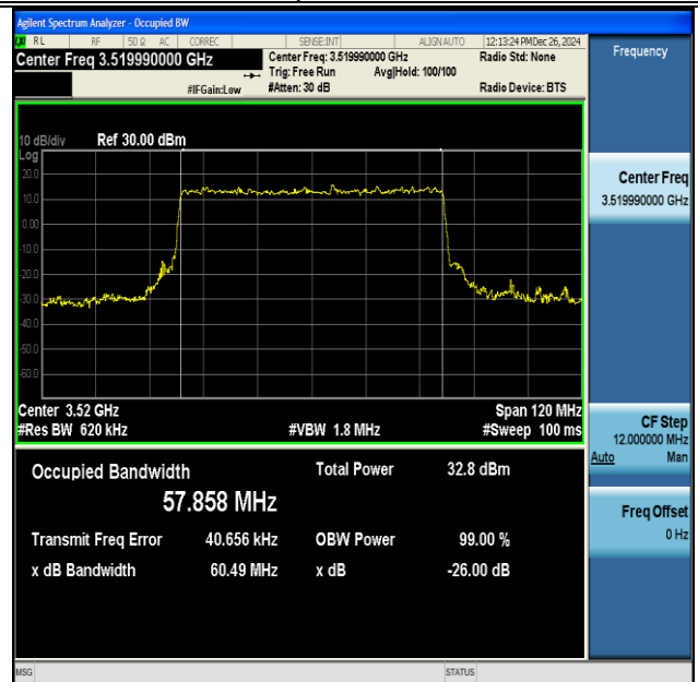
NTNV-DC_41A_n77A(3450-3550)-PC3-30-5+60-M+H- QPSK-IDLE-CP-16QAM-Outer_Full-Ant1-PASS
