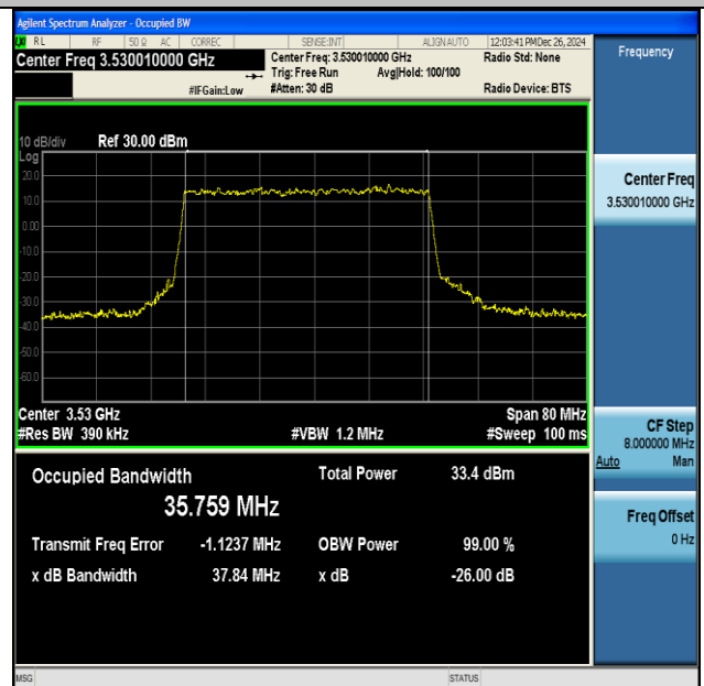
NTNV-DC_41A_n77A(3450-3550)-PC3-30-5+40-M+H- QPSK-IDLE-DFT-64QAM-Outer_Full-Ant1-PASS
