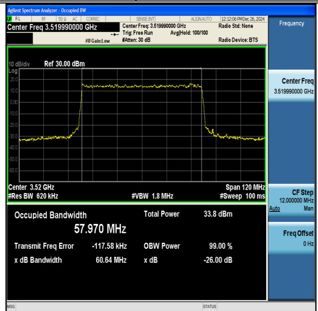
NTNV-DC_41A_n77A(3450-3550)-PC3-30-5+60-M+H- QPSK-IDLE-DFT-16QAM-Outer_Full-Ant1-PASS
