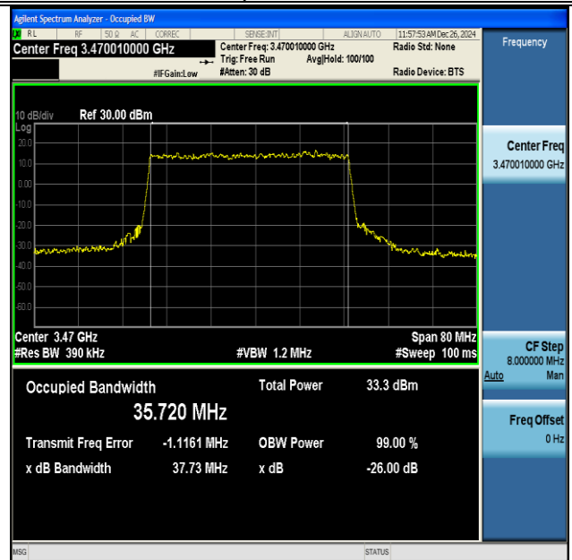
NTNV-DC_41A_n77A(3450-3550)-PC3-30-5+40-M+L- QPSK-IDLE-DFT-64QAM-Outer_Full-Ant1-PASS
