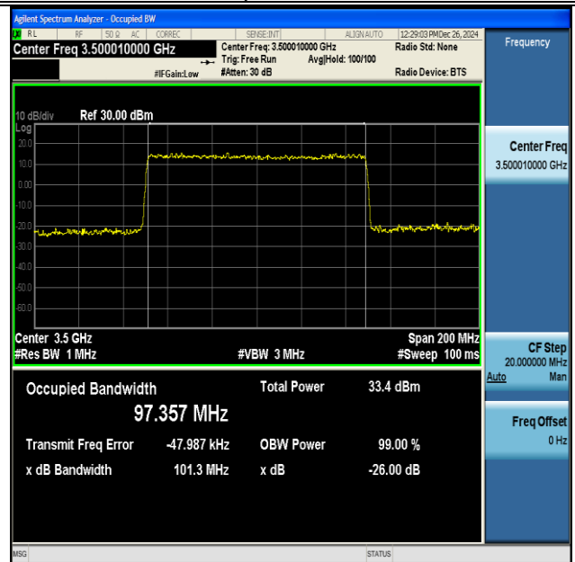
NTNV-DC_41A_n77A(3450-3550)-PC3-30-5+100-M+M- QPSK-IDLE-CP-QPSK-Outer_Full-Ant1-PASS
