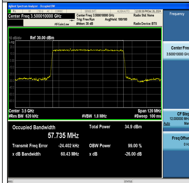
NTNV-DC_41A_n77A(3450-3550)-PC3-30-5+60-M+M- QPSK-IDLE-DFT-BPSK-Outer_Full-Ant1-PASS
