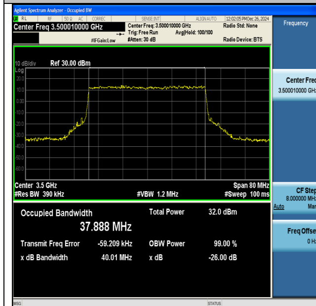
NTNV-DC_41A_n77A(3450-3550)-PC3-30-5+40-M+M- QPSK-IDLE-CP-64QAM-Outer_Full-Ant1-PASS
