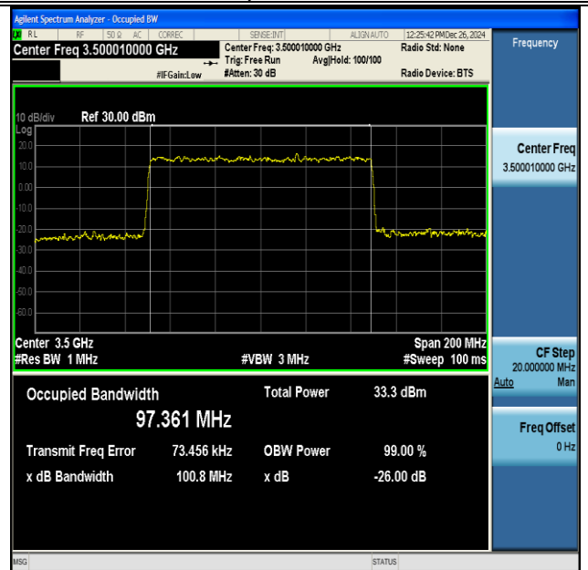
NTNV-DC_41A_n77A(3450-3550)-PC3-30-5+100-M+L- QPSK-IDLE-CP-16QAM-Outer_Full-Ant1-PASS
