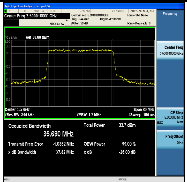
NTNV-DC_41A_n77A(3450-3550)-PC3-30-5+40-M+M- QPSK-IDLE-DFT-16QAM-Outer_Full-Ant1-PASS
