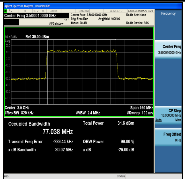
NTNV-DC_41A_n77A(3450-3550)-PC3-30-5+80-M+M- QPSK-IDLE-DFT-256QAM-Outer_Full-Ant1-PASS
