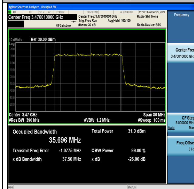
NTNV-DC_41A_n77A(3450-3550)-PC3-30-5+40-M+L- QPSK-IDLE-DFT-256QAM-Outer_Full-Ant1-PASS
