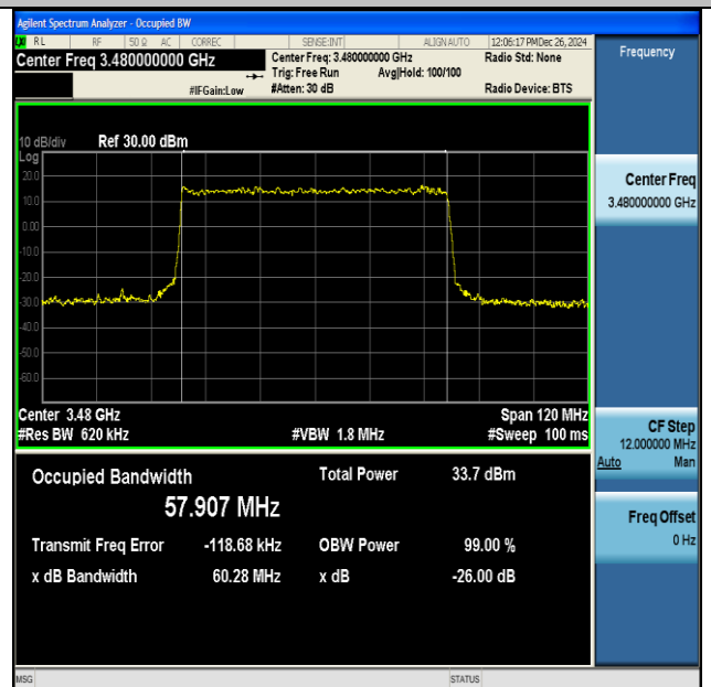
NTNV-DC_41A_n77A(3450-3550)-PC3-30-5+60-M+L- QPSK-IDLE-DFT-16QAM-Outer_Full-Ant1-PASS
