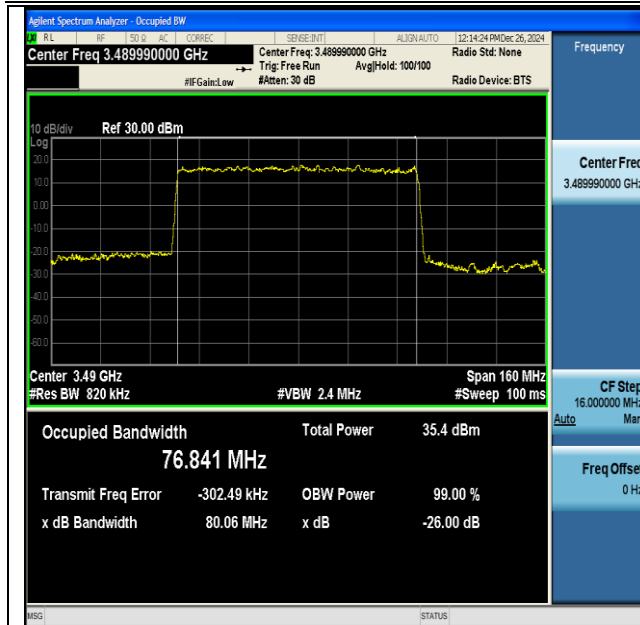
NTNV-DC_41A_n77A(3450-3550)-PC3-30-5+80-M+L-QPSK-IDLE-DFT-BPSK-Outer_Full-Ant1-PASS
