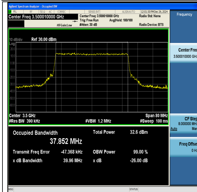
NTNV-DC_41A_n77A(3450-3550)-PC3-30-5+40-M+M- QPSK-IDLE-CP-QPSK-Outer_Full-Ant1-PASS
