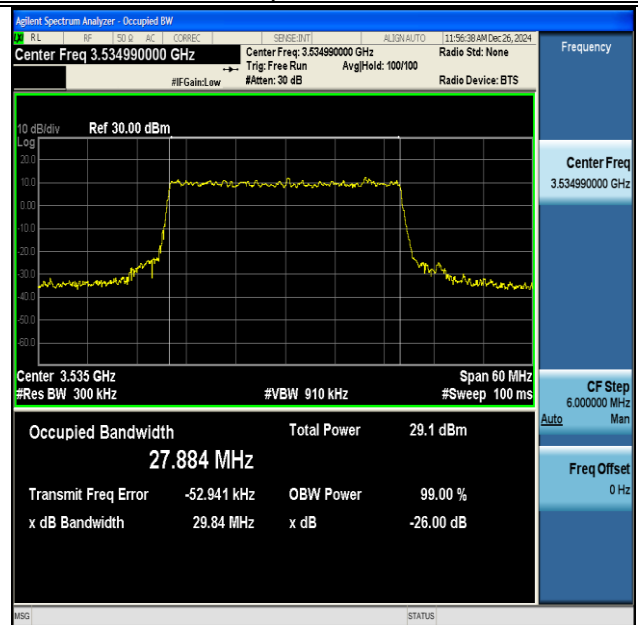
NTNV-DC_41A_n77A(3450-3550)-PC3-30-5+30-M+H- QPSK-IDLE-CP-256QAM-Outer_Full-Ant1-PASS
