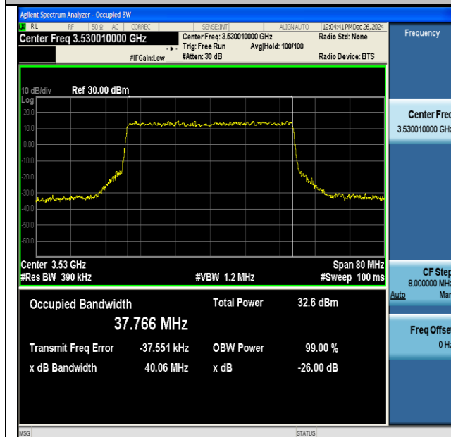
NTNV-DC_41A_n77A(3450-3550)-PC3-30-5+40-M+H- QPSK-IDLE-CP-16QAM-Outer_Full-Ant1-PASS
