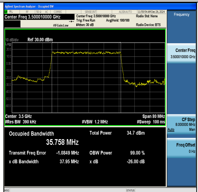
NTNV-DC_41A_n77A(3450-3550)-PC3-30-5+40-M+M- QPSK-IDLE-DFT-BPSK-Outer_Full-Ant1-PASS
