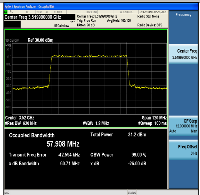
NTNV-DC_41A_n77A(3450-3550)-PC3-30-5+60-M+H- QPSK-IDLE-DFT-256QAM-Outer_Full-Ant1-PASS
