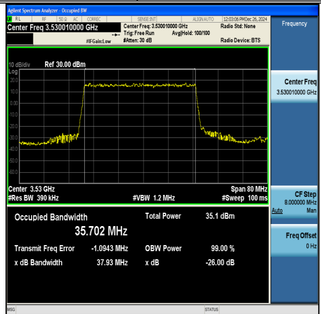
NTNV-DC_41A_n77A(3450-3550)-PC3-30-5+40-M+H- QPSK-IDLE-DFT-QPSK-Outer_Full-Ant1-PASS
