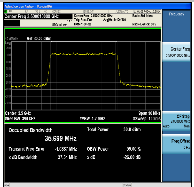
NTNV-DC_41A_n77A(3450-3550)-PC3-30-5+40-M+M- QPSK-IDLE-DFT-256QAM-Outer_Full-Ant1-PASS
