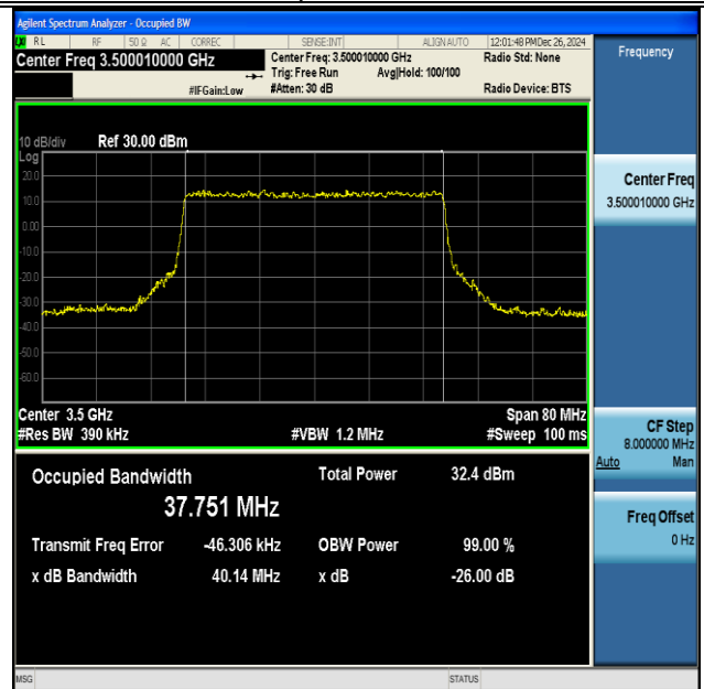
NTNV-DC_41A_n77A(3450-3550)-PC3-30-5+40-M+M- QPSK-IDLE-CP-16QAM-Outer_Full-Ant1-PASS
