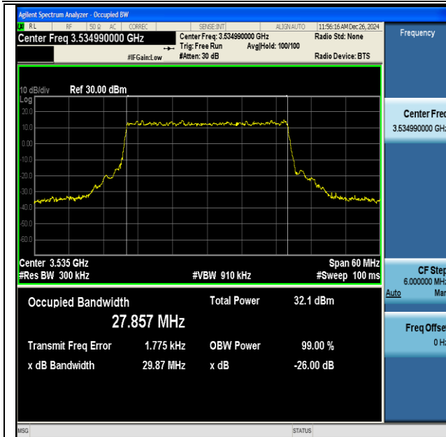
NTNV-DC_41A_n77A(3450-3550)-PC3-30-5+30-M+H- QPSK-IDLE-CP-64QAM-Outer_Full-Ant1-PASS
