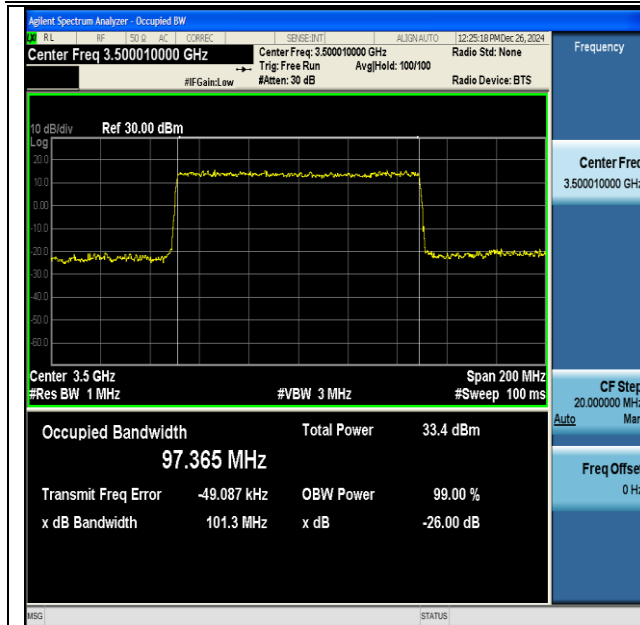
NTNV-DC_41A_n77A(3450-3550)-PC3-30-5+100-M+L- QPSK-IDLE-CP-QPSK-Outer_Full-Ant1-PASS
