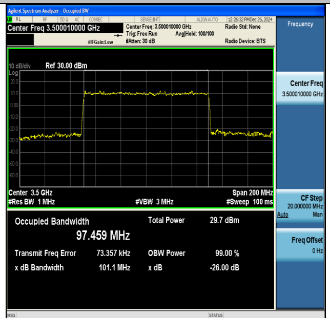
NTNV-DC_41A_n77A(3450-3550)-PC3-30-5+100-M+L- QPSK-IDLE-CP-256QAM-Outer_Full-Ant1-PASS
