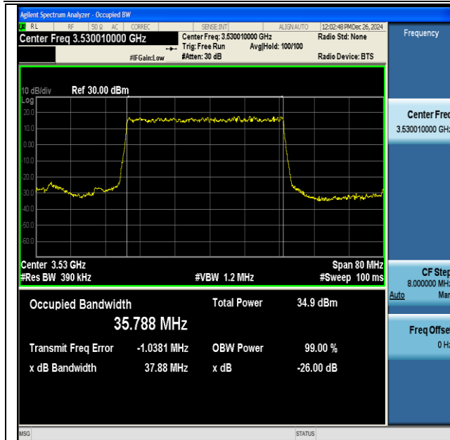
NTNV-DC_41A_n77A(3450-3550)-PC3-30-5+40-M+H- QPSK-IDLE-DFT-BPSK-Outer_Full-Ant1-PASS
