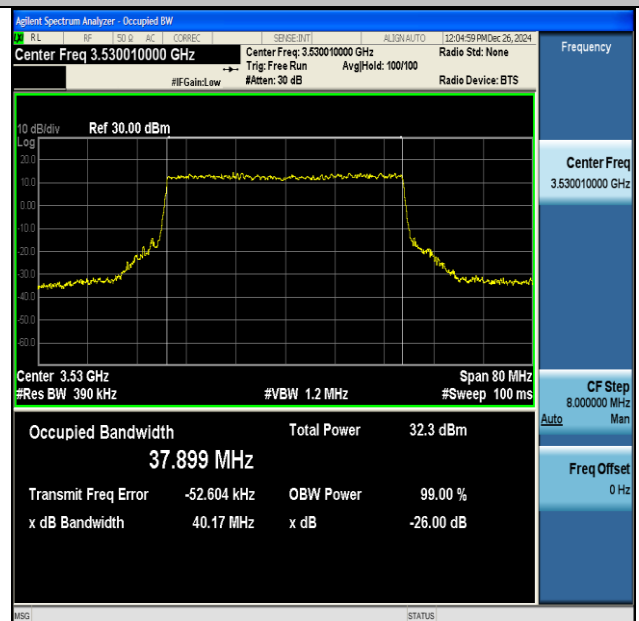
NTNV-DC_41A_n77A(3450-3550)-PC3-30-5+40-M+H- QPSK-IDLE-CP-64QAM-Outer_Full-Ant1-PASS
