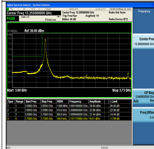
NTNV-DC_41A_n77A(3700-3980)-PC3-30-5+30-M+L- QPSK-IDLE-CP-QPSK-Edge_1RB_Left-PASS
