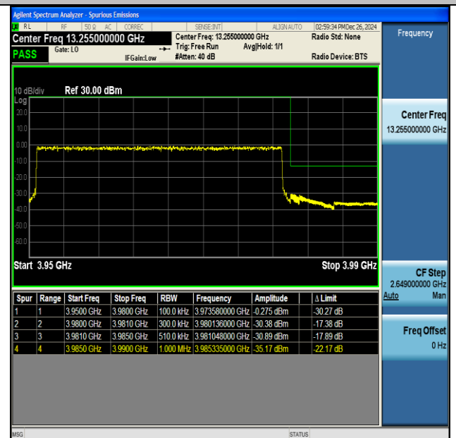
NTNV-DC_41A_n77A(3700-3980)-PC3-30-5+30-M+H- QPSK-IDLE-CP-QPSK-Outer_Full-PASS
