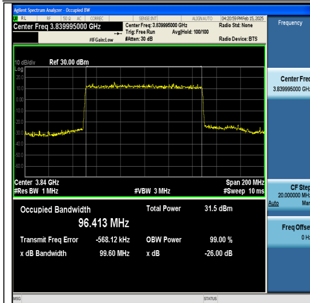
NTNV-DC_41A_n77A(3700-3980)-PC3-30-5+100-M+M-QPSK-IDLE-DFT-BPSK-Outer_Full-Ant1-PASS
