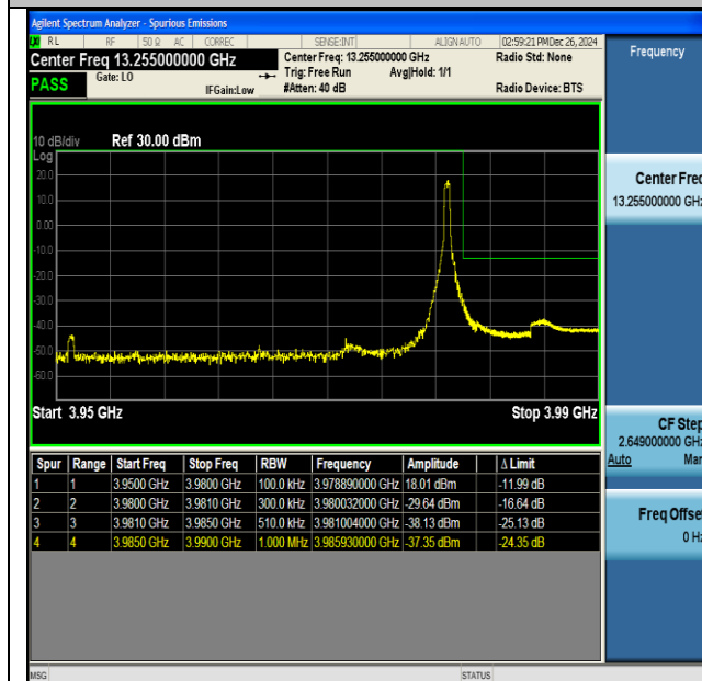
NTNV-DC_41A_n77A(3700-3980)-PC3-30-5+30-M+H- QPSK-IDLE-CP-QPSK-Edge_1RB_Right-PASS
