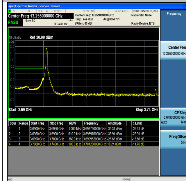
NTNV-DC_41A_n77A(3700-3980)-PC3-30-5+40-M+L- QPSK-IDLE-CP-QPSK-Edge_1RB_Left-PASS
