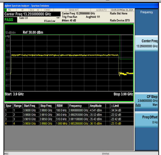
NTNV-DC_41A_n77A(3700-3980)-PC3-30-5+80-M+H- QPSK-IDLE-CP-QPSK-Outer_Full-PASS
