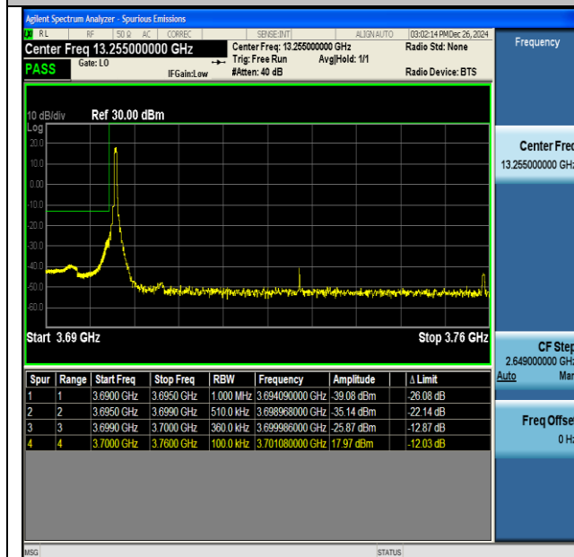
NTNV-DC_41A_n77A(3700-3980)-PC3-30-5+60-M+L- QPSK-IDLE-CP-QPSK-Edge_1RB_Left-PASS
