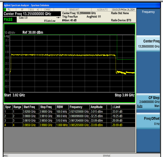
NTNV-DC_41A_n77A(3700-3980)-PC3-30-5+60-M+H- QPSK-IDLE-CP-QPSK-Outer_Full-PASS
