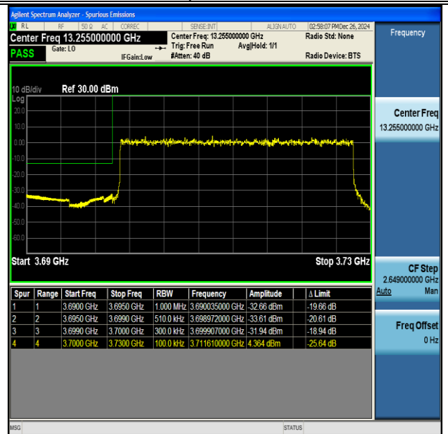
NTNV-DC_41A_n77A(3700-3980)-PC3-30-5+30-M+L- QPSK-IDLE-DFT-BPSK-Outer_Full-PASS
