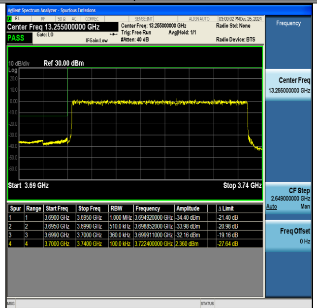
NTNV-DC_41A_n77A(3700-3980)-PC3-30-5+40-M+L- QPSK-IDLE-DFT-BPSK-Outer_Full-PASS
