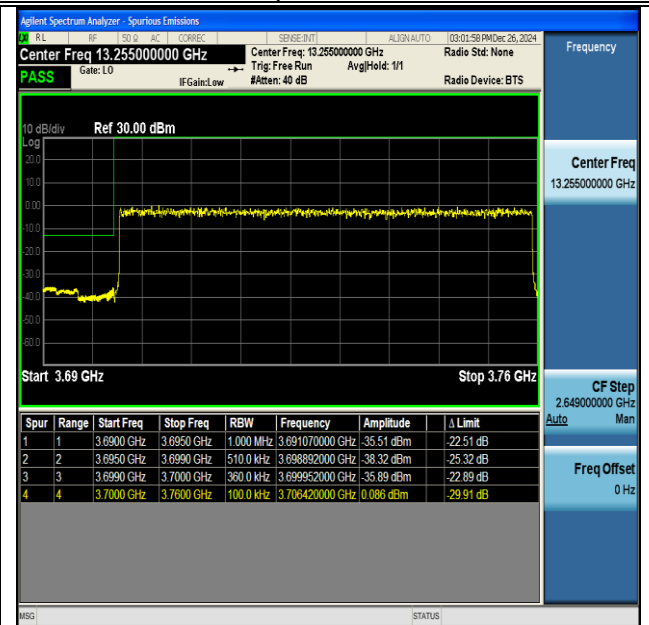
NTNV-DC_41A_n77A(3700-3980)-PC3-30-5+60-M+L- QPSK-IDLE-DFT-BPSK-Outer_Full-PASS
