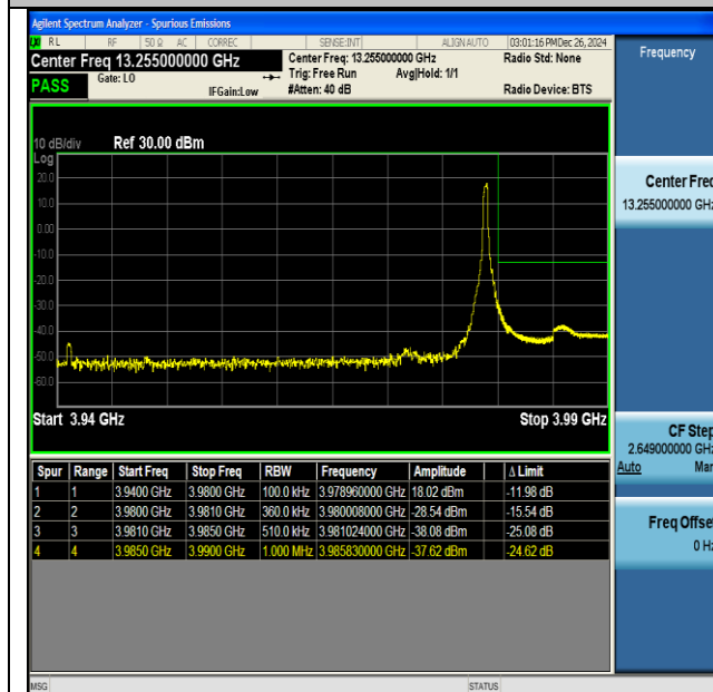
NTNV-DC_41A_n77A(3700-3980)-PC3-30-5+40-M+H- QPSK-IDLE-CP-QPSK-Edge_1RB_Right-PASS
