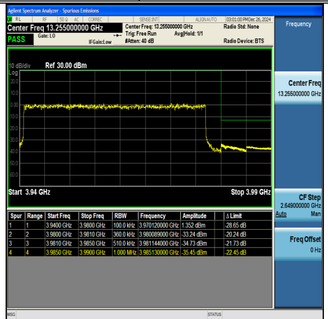
NTNV-DC_41A_n77A(3700-3980)-PC3-30-5+40-M+H- QPSK-IDLE-DFT-BPSK-Outer_Full-PASS
