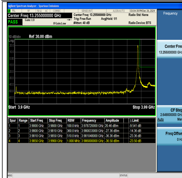
NTNV-DC_41A_n77A(3700-3980)-PC3-30-5+80-M+H- QPSK-IDLE-DFT-BPSK-Edge_1RB_Right-PASS
