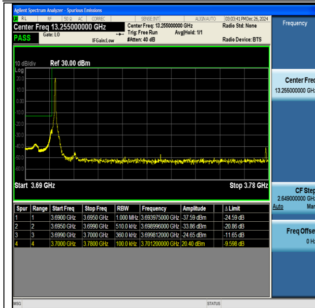
NTNV-DC_41A_n77A(3700-3980)-PC3-30-5+80-M+L- QPSK-IDLE-DFT-BPSK-Edge_1RB_Left-PASS
