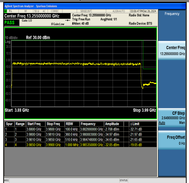
NTNV-DC_41A_n77A(3700-3980)-PC3-30-5+100-M+H- QPSK-IDLE-DFT-BPSK-Outer_Full-PASS
