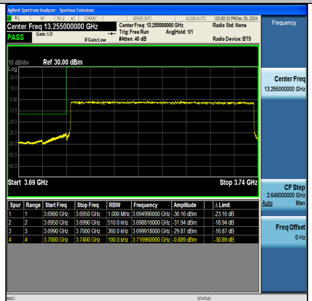
NTNV-DC_41A_n77A(3700-3980)-PC3-30-5+40-M+L- QPSK-IDLE-CP-QPSK-Outer_Full-PASS
