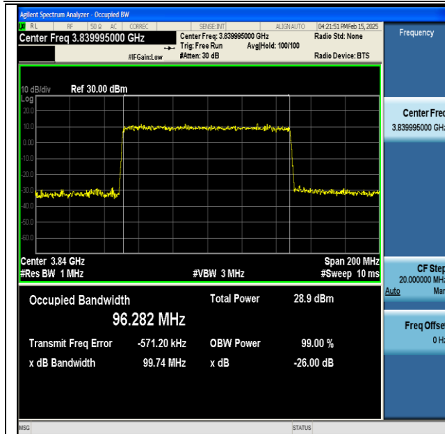
NTNV-DC_41A_n77A(3700-3980)-PC3-30-5+100-M+M-QPSK-IDLE-DFT-256QAM-Outer_Full-Ant1-PASS
