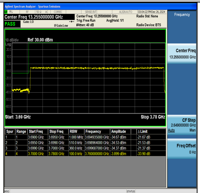
NTNV-DC_41A_n77A(3700-3980)-PC3-30-5+80-M+L- QPSK-IDLE-CP-QPSK-Outer_Full-PASS
