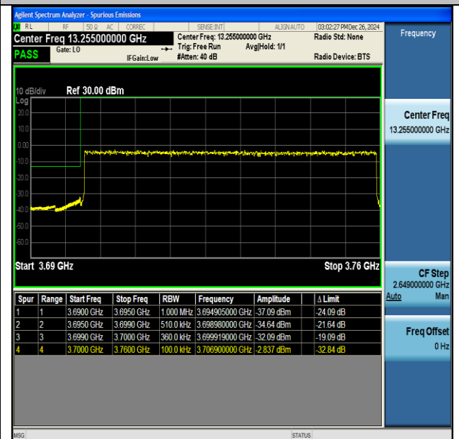
NTNV-DC_41A_n77A(3700-3980)-PC3-30-5+60-M+L- QPSK-IDLE-CP-QPSK-Outer_Full-PASS
