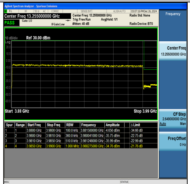
NTNV-DC_41A_n77A(3700-3980)-PC3-30-5+100-M+H- QPSK-IDLE-CP-QPSK-Outer_Full-PASS
