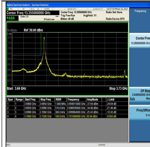
NTNV-DC_41A_n77A(3700-3980)-PC3-30-5+30-M+L- QPSK-IDLE-DFT-BPSK-Edge_1RB_Left-PASS
