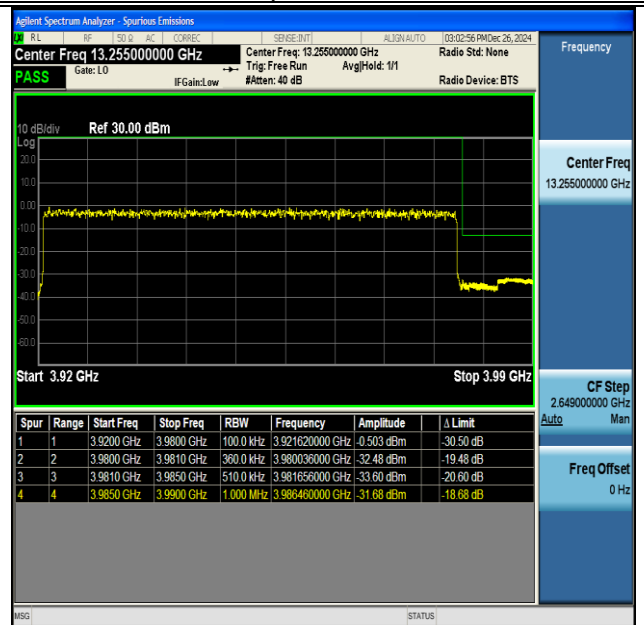
NTNV-DC_41A_n77A(3700-3980)-PC3-30-5+60-M+H- QPSK-IDLE-DFT-BPSK-Outer_Full-PASS
