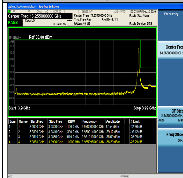
NTNV-DC_41A_n77A(3700-3980)-PC3-30-5+80-M+H- QPSK-IDLE-CP-QPSK-Edge_1RB_Right-PASS
