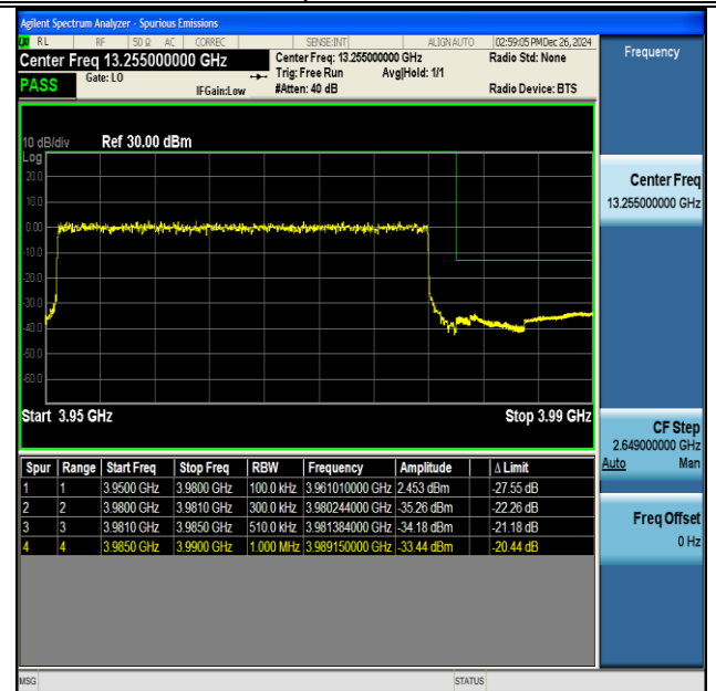
NTNV-DC_41A_n77A(3700-3980)-PC3-30-5+30-M+H- QPSK-IDLE-DFT-BPSK-Outer_Full-PASS
