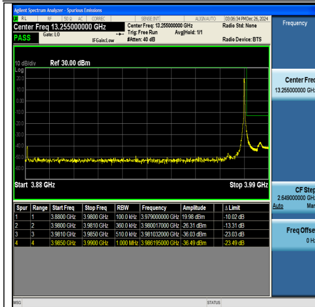
NTNV-DC_41A_n77A(3700-3980)-PC3-30-5+100-M+H- QPSK-IDLE-DFT-BPSK-Edge_1RB_Right-PASS
