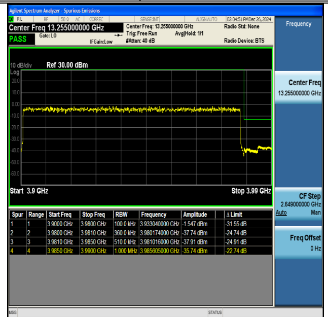
NTNV-DC_41A_n77A(3700-3980)-PC3-30-5+80-M+H- QPSK-IDLE-DFT-BPSK-Outer_Full-PASS
