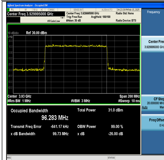
NTNV-DC_41A_n77A(3700-3980)-PC3-30-5+100-M+H- QPSK-IDLE-DFT-64QAM-Outer_Full-Ant1-PASS
