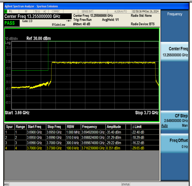
NTNV-DC_41A_n77A(3700-3980)-PC3-30-5+30-M+L- QPSK-IDLE-CP-QPSK-Outer_Full-PASS
