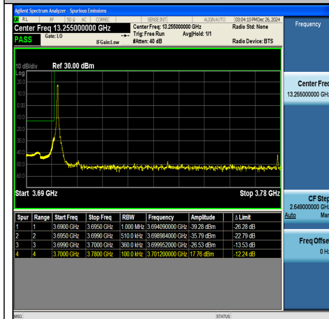
NTNV-DC_41A_n77A(3700-3980)-PC3-30-5+80-M+L- QPSK-IDLE-CP-QPSK-Edge_1RB_Left-PASS
