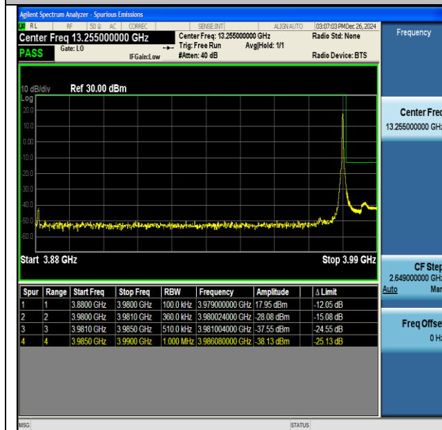
NTNV-DC_41A_n77A(3700-3980)-PC3-30-5+100-M+H- QPSK-IDLE-CP-QPSK-Edge_1RB_Right-PASS
