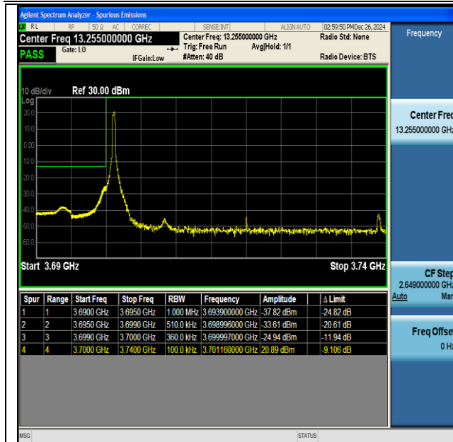
NTNV-DC_41A_n77A(3700-3980)-PC3-30-5+40-M+L- QPSK-IDLE-DFT-BPSK-Edge_1RB_Left-PASS
