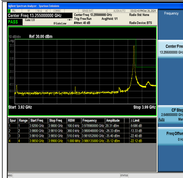
NTNV-DC_41A_n77A(3700-3980)-PC3-30-5+60-M+H- QPSK-IDLE-DFT-BPSK-Edge_1RB_Right-PASS
