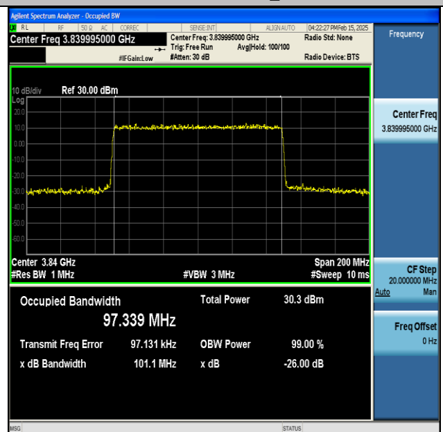
NTNV-DC_41A_n77A(3700-3980)-PC3-30-5+100-M+M-QPSK-IDLE-CP-64QAM-Outer_Full-Ant1-PASS
