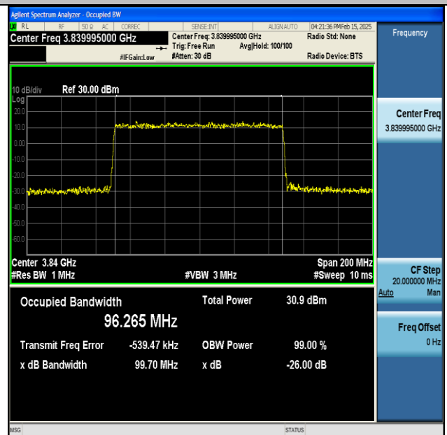
NTNV-DC_41A_n77A(3700-3980)-PC3-30-5+100-M+M-QPSK-IDLE-DFT-64QAM-Outer_Full-Ant1-PASS
