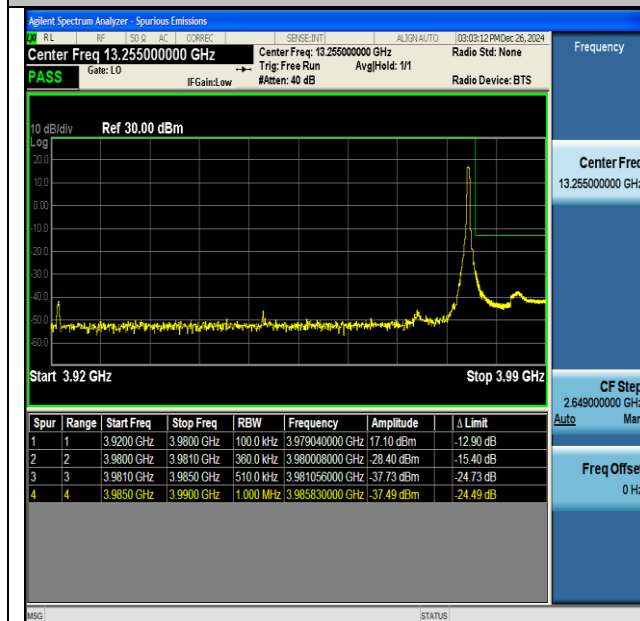
NTNV-DC_41A_n77A(3700-3980)-PC3-30-5+60-M+H- QPSK-IDLE-CP-QPSK-Edge_1RB_Right-PASS
