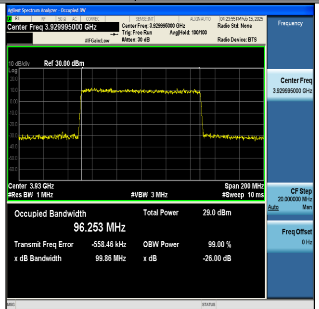
NTNV-DC_41A_n77A(3700-3980)-PC3-30-5+100-M+H- QPSK-IDLE-DFT-256QAM-Outer_Full-Ant1-PASS
