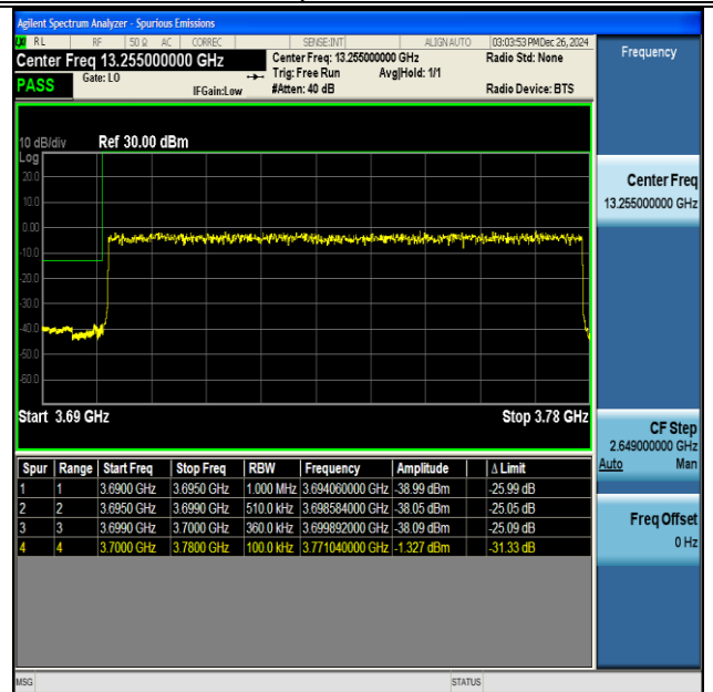
NTNV-DC_41A_n77A(3700-3980)-PC3-30-5+80-M+L- QPSK-IDLE-DFT-BPSK-Outer_Full-PASS
