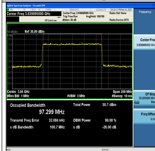
NTNV-DC_41A_n77A(3700-3980)-PC3-30-5+100-M+M-QPSK-IDLE-CP-16QAM-Outer_Full-Ant1-PASS
