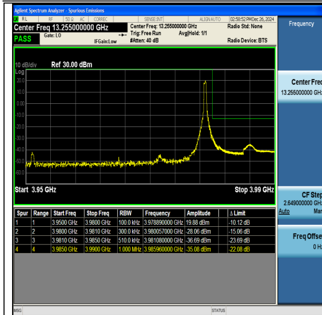
NTNV-DC_41A_n77A(3700-3980)-PC3-30-5+30-M+H- QPSK-IDLE-DFT-BPSK-Edge_1RB_Right-PASS
