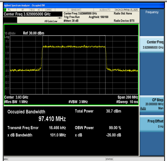
NTNV-DC_41A_n77A(3700-3980)-PC3-30-5+100-M+H- QPSK-IDLE-CP-16QAM-Outer_Full-Ant1-PASS
