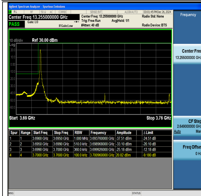
NTNV-DC_41A_n77A(3700-3980)-PC3-30-5+60-M+L- QPSK-IDLE-DFT-BPSK-Edge_1RB_Left-PASS
