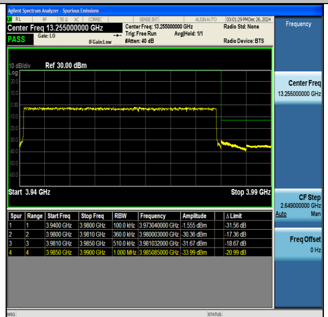
NTNV-DC_41A_n77A(3700-3980)-PC3-30-5+40-M+H- QPSK-IDLE-CP-QPSK-Outer_Full-PASS
