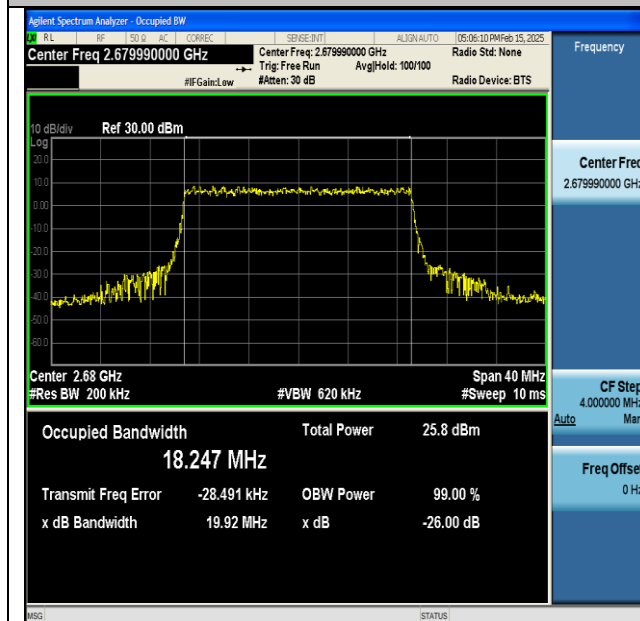
NTNV-DC_66A_n41A-PC3-30-5+20-M+H-QPSK-IDLE- CP-256QAM-Outer_Full-Ant1-PASS
