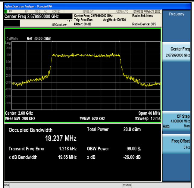
NTNV-DC_66A_n41A-PC3-30-5+20-M+H-QPSK-IDLE- CP-64QAM-Outer_Full-Ant1-PASS
