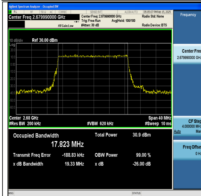
NTNV-DC_66A_n41A-PC3-30-5+20-M+H-QPSK-IDLE-DFT-16QAM-Outet_Full-Ant1-PASS
