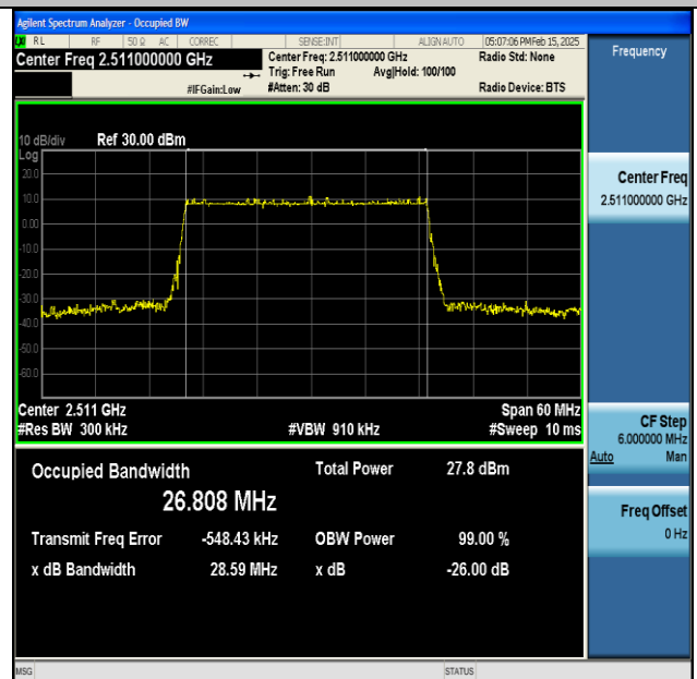
NTNV-DC_66A_n41A-PC3-30-5+30-M+L-QPSK-IDLE- DFT-256QAM-Outer_Full-Ant1-PASS
