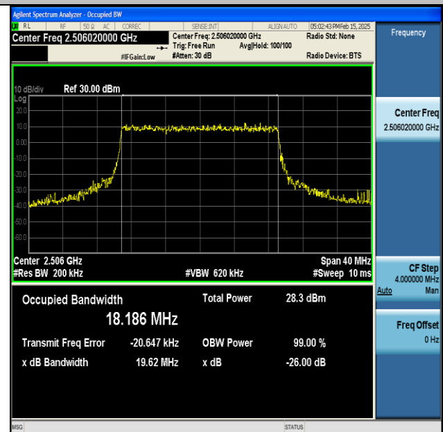
NTNV-DC_66A_n41A-PC3-30-5+20-M+L-QPSK-IDLE-CP-64QAM-Outter_Full-Ant1-PASS
