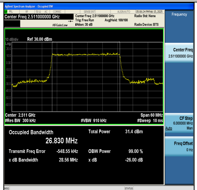
NTNV-DC_66A_n41A-PC3-30-5+30-M+L-QPSK-IDLE- DFT-BPSK-Outer_Full-Ant1-PASS
