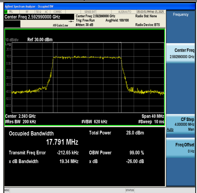
NTNV-DC_66A_n41A-PC3-30-5+20-M+M-QPSK-IDLE- DFT-256QAM-Outer_Full-Ant1-PASS
