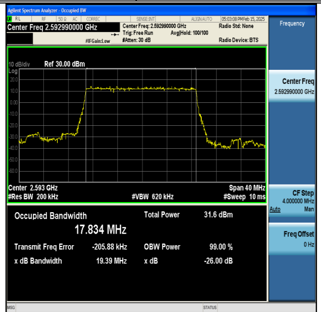
NTNV-DC_66A_n41A-PC3-30-5+20-M+M-QPSK-IDLE- DFT-BPSK-Outer_Full-Ant1-PASS
