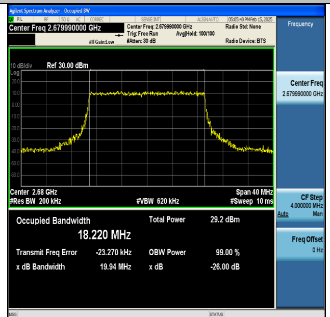
NTNV-DC_66A_n41A-PC3-30-5+20-M+H-QPSK-IDLE-CP-QPSK-Outet_Full-Ant1-PASS
