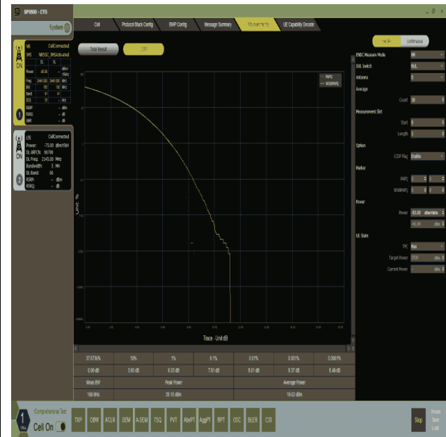
NTVN-DC_66A_N41A-PC3-15-5+100-M+H-QPSK-IDLE-CP-256QAM-Outer_Full-PASS
