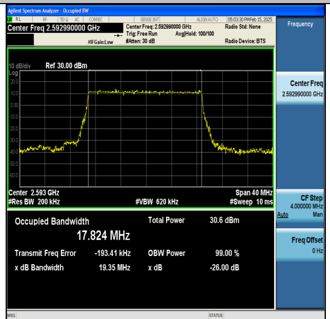
NTNV-DC_66A_n41A-PC3-30-5+20-M+M-QPSK-IDLE- DFT-16QAM-Outer_Full-Ant1-PASS
