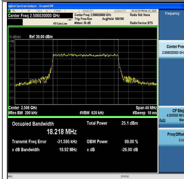
NTNV-DC_66A_n41A-PC3-30-5+20-M+L-QPSK-IDLE-CP- 256QAM-Outer_Full-Ant1-PASS
