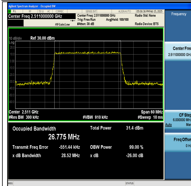
NTNV-DC_66A_n41A-PC3-30-5+30-M+L-QPSK-IDLE- DFT-QPSK-Outer_Full-Ant1-PASS
