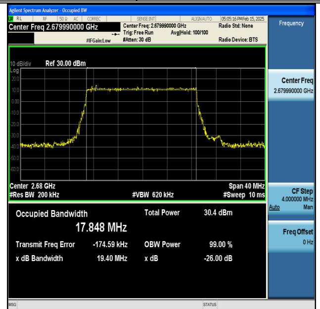
NTNV-DC_66A_n41A-PC3-30-5+20-M+H-QPSK-IDLE-DFT-64QAM-Outet_Full-Ant1-PASS
