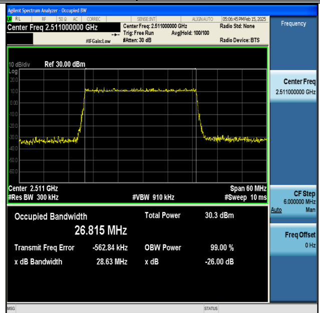
NTNV-DC_66A_n41A-PC3-30-5+30-M+L-QPSK-IDLE- DFT-16QAM-Outer_Full-Ant1-PASS
