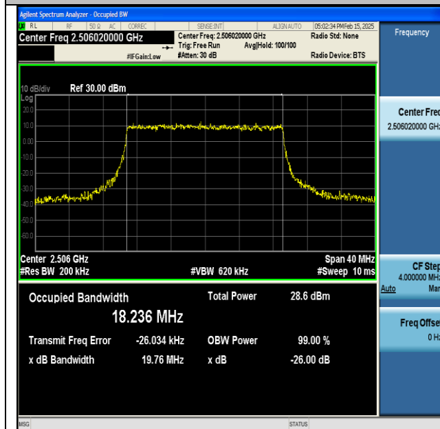
NTNV-DC_66A_n41A-PC3-30-5+20-M+L-QPSK-IDLE-CP-16QAM-Outter_Full-Ant1-PASS
