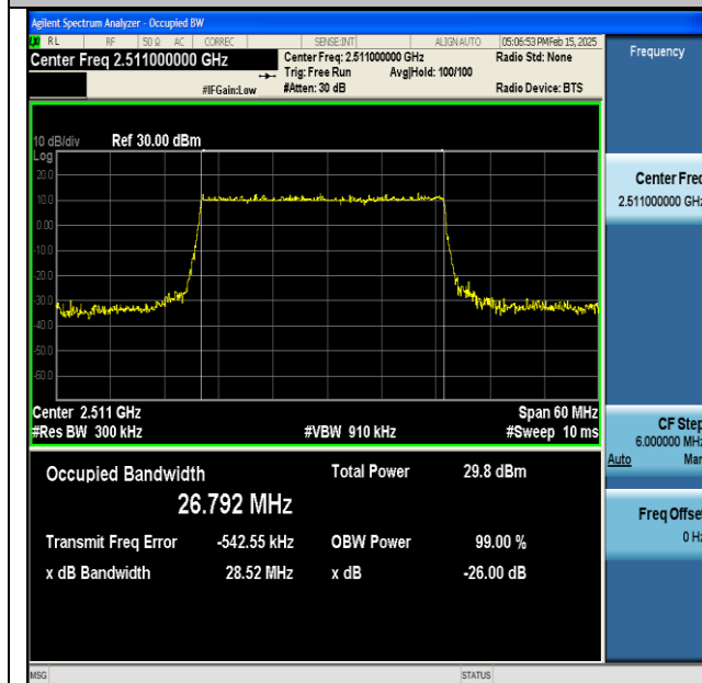
NTNV-DC_66A_n41A-PC3-30-5+30-M+L-QPSK-IDLE- DFT-64QAM-Outer_Full-Ant1-PASS
