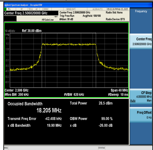
NTNV-DC_66A_n41A-PC3-30-5+20-M+L-QPSK-IDLE-CP-QPSK-Outter_Full-Ant1-PASS
