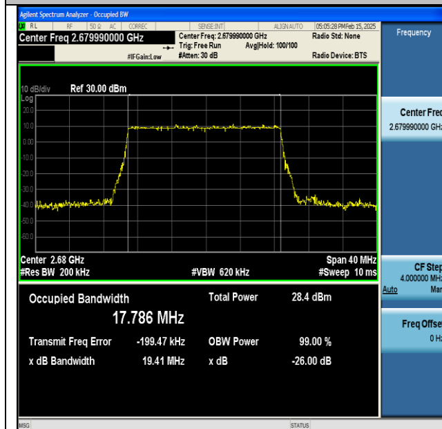
NTNV-DC_66A_n41A-PC3-30-5+20-M+H-QPSK-IDLE-DFT-256QAM-Outet_Full-Ant1-PASS
