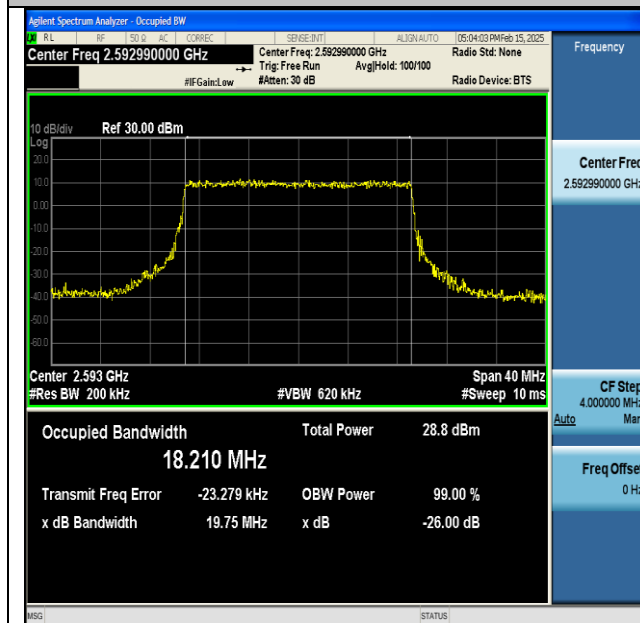
NTNV-DC_66A_n41A-PC3-30-5+20-M+M-QPSK-IDLE- CP-QPSK-Outer_Full-Ant1-PASS
