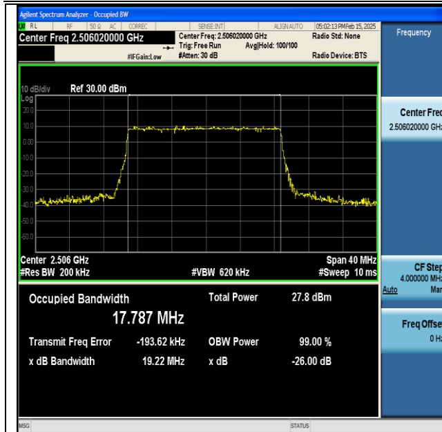
NTNV-DC_66A_n41A-PC3-30-5+20-M+L-QPSK-IDLE-DFT-256QAM-Outter_Full-Ant1-PASS
