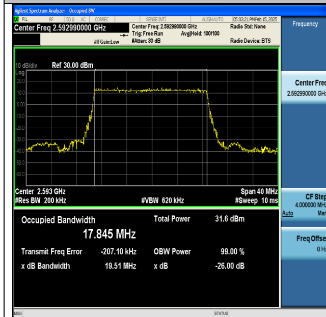
NTNV-DC_66A_n41A-PC3-30-5+20-M+M-QPSK-IDLE- DFT-QPSK-Outer_Full-Ant1-PASS
