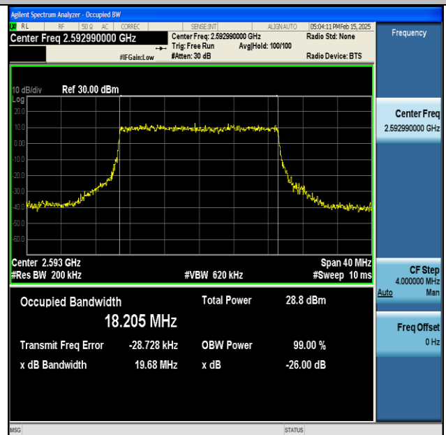
NTNV-DC_66A_n41A-PC3-30-5+20-M+M-QPSK-IDLE- CP-16QAM-Outer_Full-Ant1-PASS
