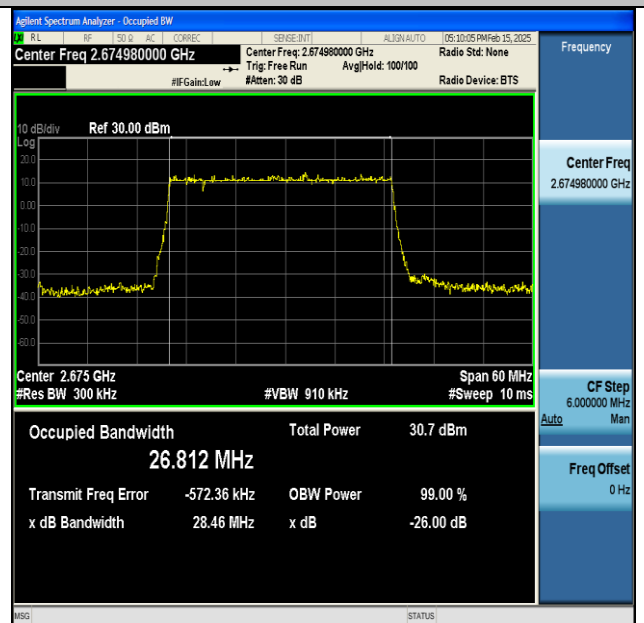
NTNV-DC_66A_n41A-PC3-30-5+30-M+H-QPSK-IDLE-DFT-16QAM-Outer_Full-Ant1-PASS
