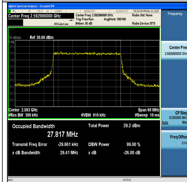
NTNV-DC_66A_n41A-PC3-30-5+30-M+M-QPSK-IDLE- CP-16QAM-Outer_Full-Ant1-PASS
