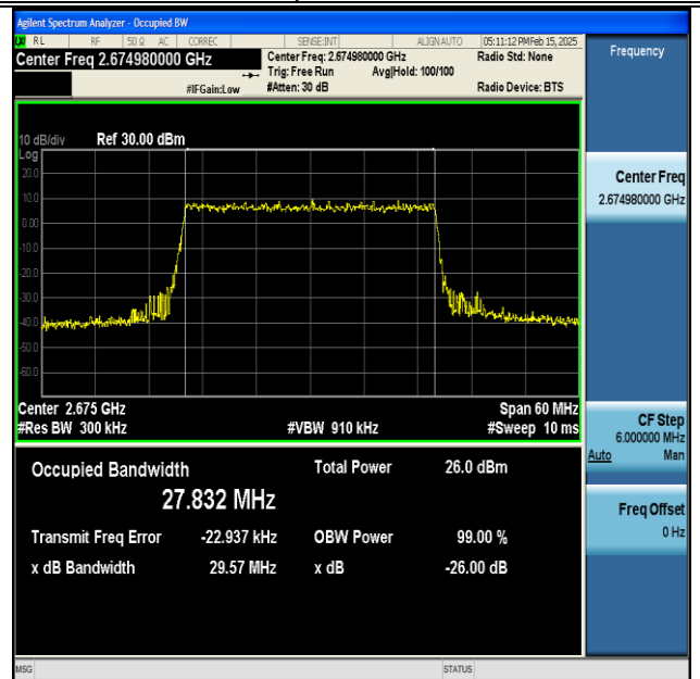
NTNV-DC_66A_n41A-PC3-30-5+30-M+H-QPSK-IDLE- CP-256QAM-Outer_Full-Ant1-PASS
