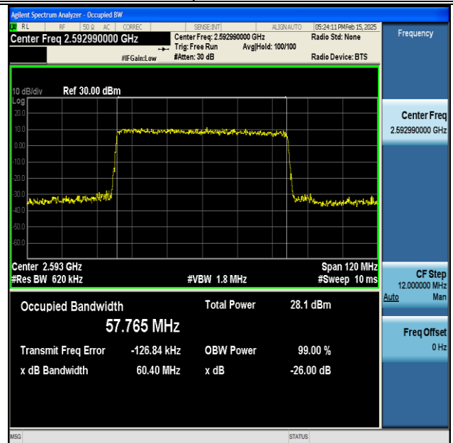
NTNV-DC_66A_n41A-PC3-30-5+60-M+M-QPSK-IDLE- DFT-256QAM-Outer_Full-Ant1-PASS
