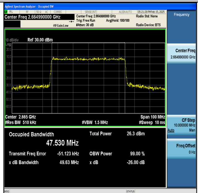
NTNV-DC_66A_n41A-PC3-30-5+50-M+H-QPSK-IDLE- CP-256QAM-Outer_Full-Ant1-PASS
