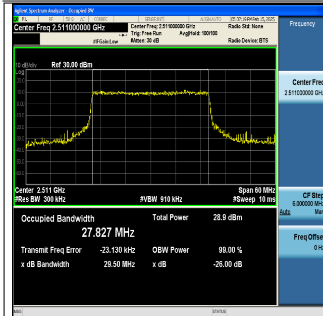
NTNV-DC_66A_n41A-PC3-30-5+30-M+L-QPSK-IDLE-CP-QPSK-Outer_Full-Ant1-PASS
