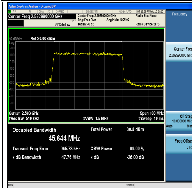
NTNV-DC_66A_n41A-PC3-30-5+50-M+M-QPSK-IDLE- DFT-16QAM-Outer_Full-Ant1-PASS
