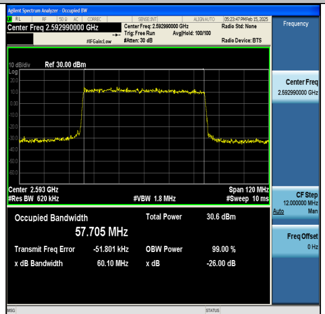
NTNV-DC_66A_n41A-PC3-30-5+60-M+M-QPSK-IDLE-DFT-16QAM-Outer_Full-Ant1-PASS
