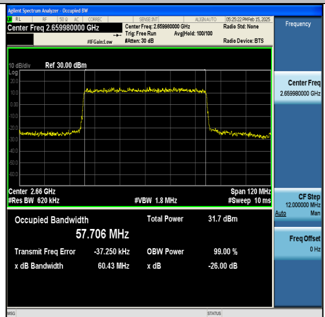
NTNV-DC_66A_n41A-PC3-30-5+60-M+H-QPSK-IDLE-DFT-QPSK-Outer_Full-Ant1-PASS
