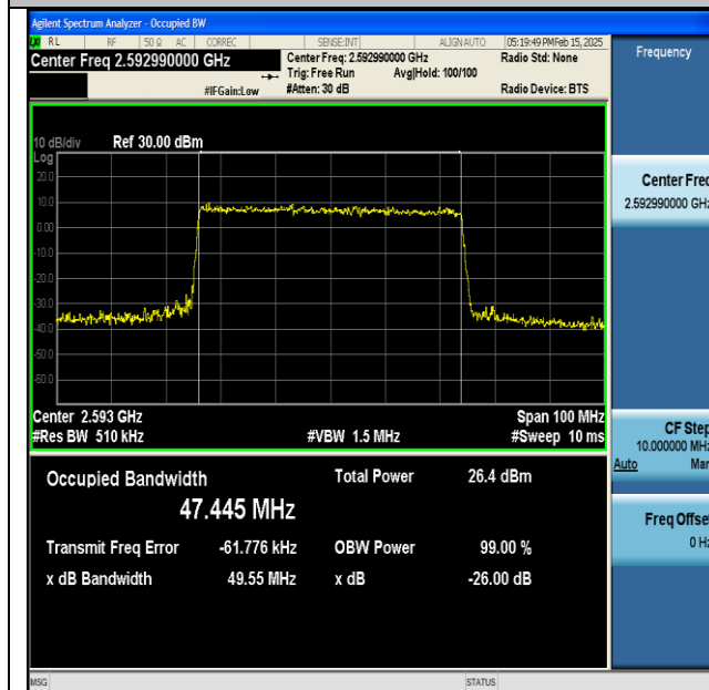
NTNV-DC_66A_n41A-PC3-30-5+50-M+M-QPSK-IDLE- CP-256QAM-Outer_Full-Ant1-PASS
