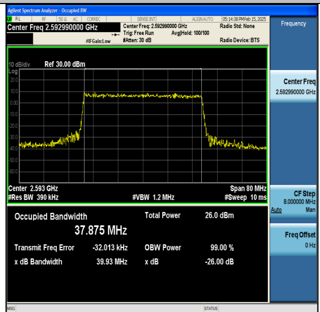
NTNV-DC_66A_n41A-PC3-30-5+40-M+M-QPSK-IDLE-CP-256QAM-Outer_Full-Ant1-PASS
