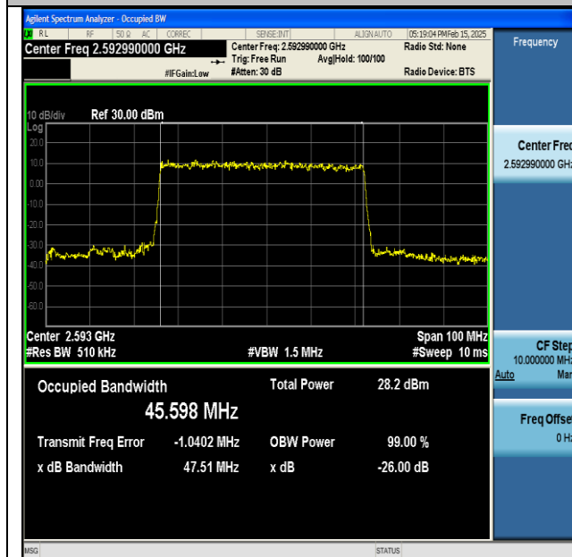
NTNV-DC_66A_n41A-PC3-30-5+50-M+M-QPSK-IDLE- DFT-256QAM-Outer_Full-Ant1-PASS
