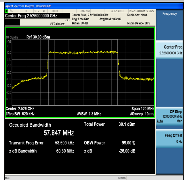
NTNV-DC_66A_n41A-PC3-30-5+60-M+L-QPSK-IDLE-DFT-64QAM-Outter_Full-Ant1-PASS
