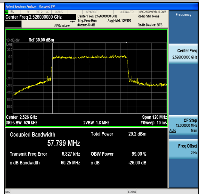
NTNV-DC_66A_n41A-PC3-30-5+60-M+L-QPSK-IDLE-CP-64QAM-Outter_Full-Ant1-PASS
