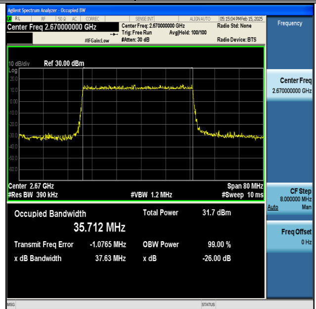
NTNV-DC_66A_n41A-PC3-30-5+40-M+H-QPSK-IDLE- DFT-QPSK-Outer_Full-Ant1-PASS
