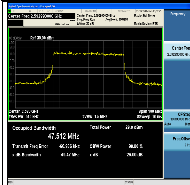
NTNV-DC_66A_n41A-PC3-30-5+50-M+M-QPSK-IDLE- CP-16QAM-Outer_Full-Ant1-PASS
