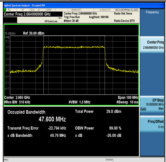
NTNV-DC_66A_n41A-PC3-30-5+50-M+H-QPSK-IDLE- CP-16QAM-Outer_Full-Ant1-PASS
