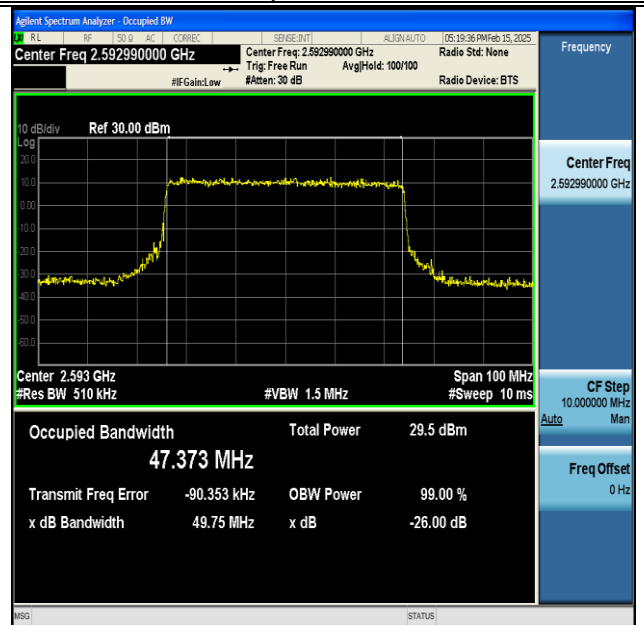
NTNV-DC_66A_n41A-PC3-30-5+50-M+M-QPSK-IDLE- CP-64QAM-Outer_Full-Ant1-PASS
