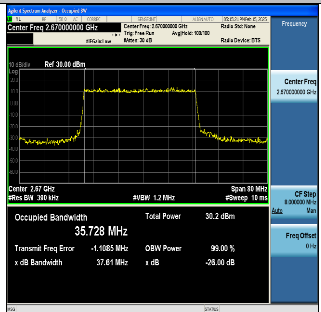
NTNV-DC_66A_n41A-PC3-30-5+40-M+H-QPSK-IDLE- DFT-64QAM-Outer_Full-Ant1-PASS
