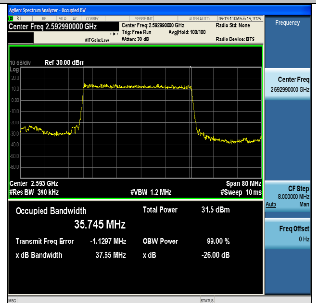
NTNV-DC_66A_n41A-PC3-30-5+40-M+M-QPSK-IDLE-DFT-BPSK-Outet_Full-Ant1-PASS
