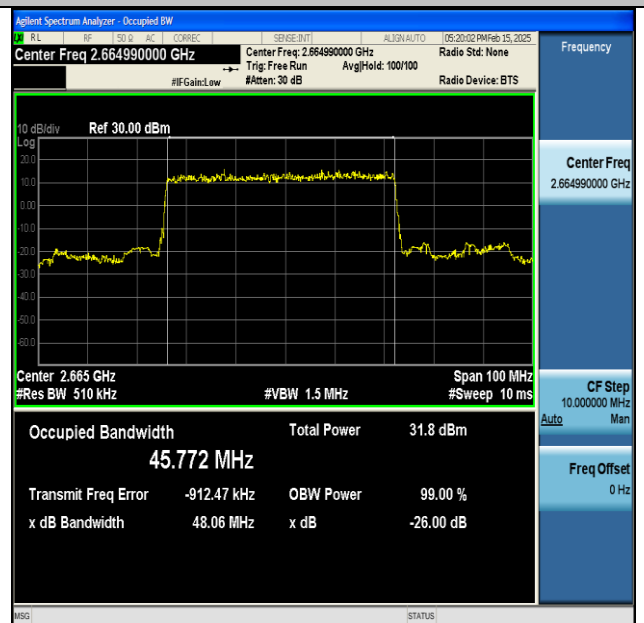
NTNV-DC_66A_n41A-PC3-30-5+50-M+H-QPSK-IDLE- DFT-BPSK-Outer_Full-Ant1-PASS
