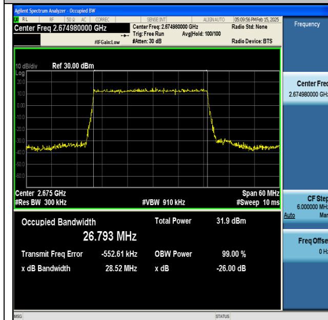
NTNV-DC_66A_n41A-PC3-30-5+30-M+H-QPSK-IDLE-DFT-QPSK-Outer_Full-Ant1-PASS
