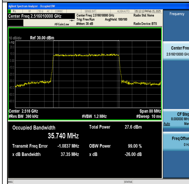
NTNV-DC_66A_n41A-PC3-30-5+40-M+L-QPSK-IDLE- DFT-256QAM-Outer_Full-Ant1-PASS
