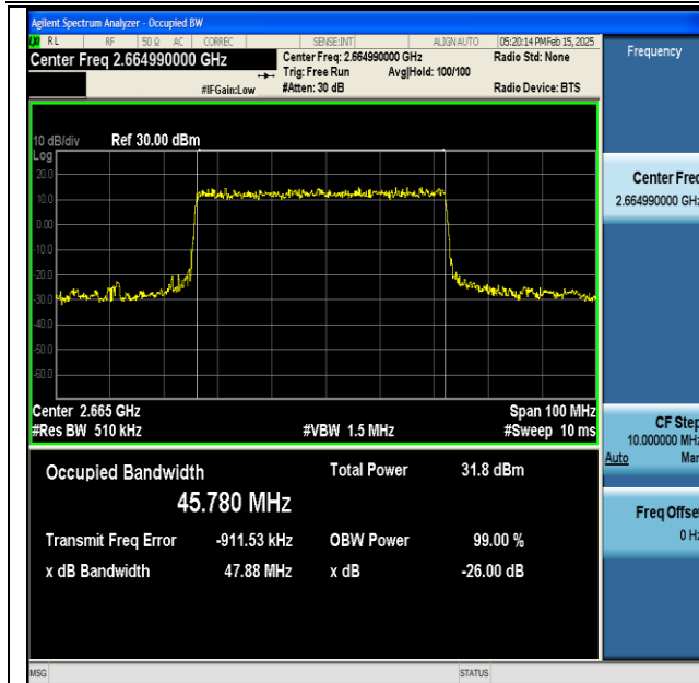
NTNV-DC_66A_n41A-PC3-30-5+50-M+H-QPSK-IDLE-DFT-QPSK-Outet_Full-Ant1-PASS
