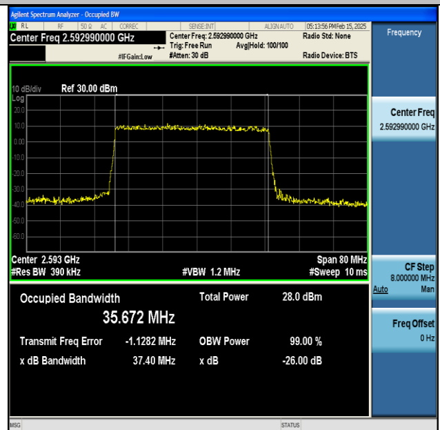
NTNV-DC_66A_n41A-PC3-30-5+40-M+M-QPSK-IDLE- DFT-256QAM-Outer_Full-Ant1-PASS
