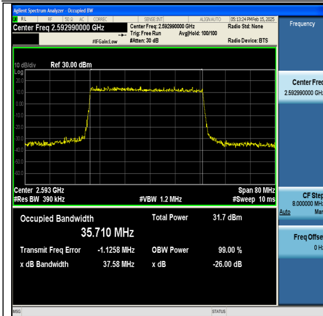
NTNV-DC_66A_n41A-PC3-30-5+40-M+M-QPSK-IDLE- DFT-QPSK-Outer_Full-Ant1-PASS
