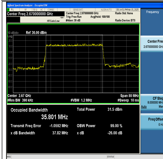
NTNV-DC_66A_n41A-PC3-30-5+40-M+H-QPSK-IDLE- DFT-BPSK-Outer_Full-Ant1-PASS
