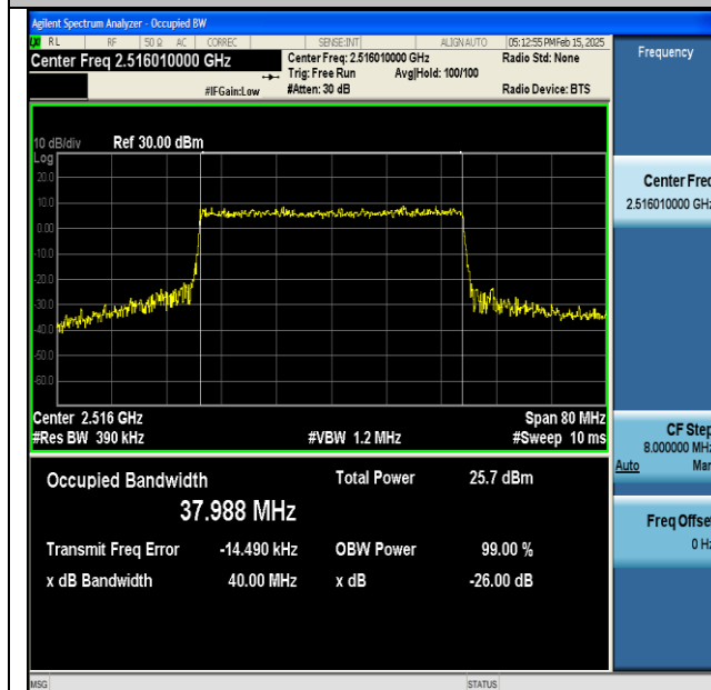
NTNV-DC_66A_n41A-PC3-30-5+40-M+L-QPSK-IDLE-CP-256QAM-Outet_Full-Ant1-PASS
