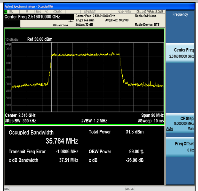
NTNV-DC_66A_n41A-PC3-30-5+40-M+L-QPSK-IDLE- DFT-QPSK-Outer_Full-Ant1-PASS
