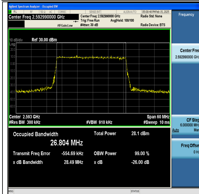
NTNV-DC_66A_n41A-PC3-30-5+30-M+M-QPSK-IDLE- DFT-256QAM-Outer_Full-Ant1-PASS
