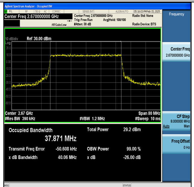
NTNV-DC_66A_n41A-PC3-30-5+40-M+H-QPSK-IDLE- CP-64QAM-Outer_Full-Ant1-PASS
