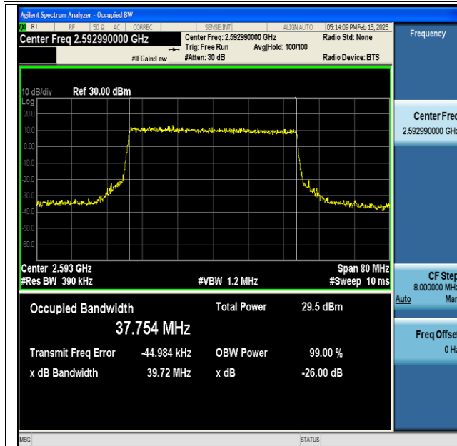
NTNV-DC_66A_n41A-PC3-30-5+40-M+M-QPSK-IDLE-CP-QPSK-Outer_Full-Ant1-PASS
