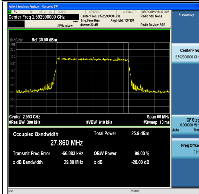
NTNV-DC_66A_n41A-PC3-30-5+30-M+M-QPSK-IDLE-CP-256QAM-Outer_Full-Ant1-PASS
