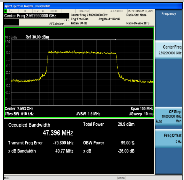
NTNV-DC_66A_n41A-PC3-30-5+50-M+M-QPSK-IDLE- CP-QPSK-Outer_Full-Ant1-PASS
