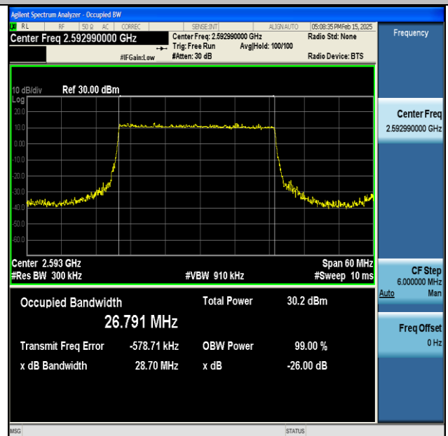
NTNV-DC_66A_n41A-PC3-30-5+30-M+M-QPSK-IDLE- DFT-64QAM-Outer_Full-Ant1-PASS
