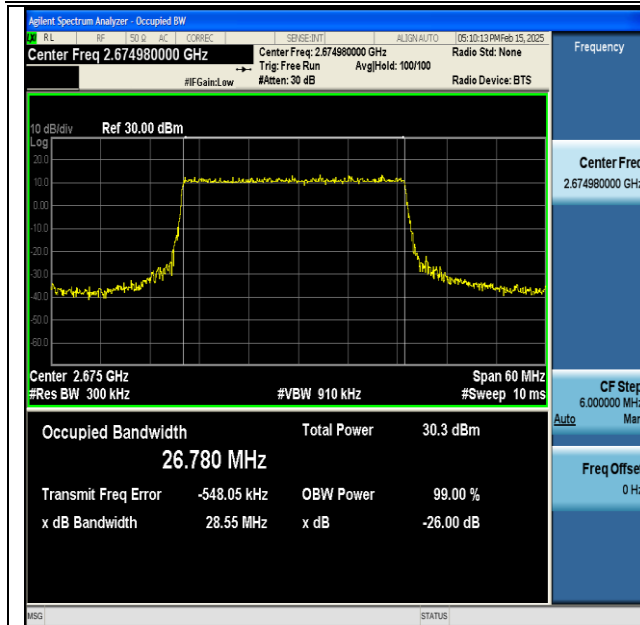
NTNV-DC_66A_n41A-PC3-30-5+30-M+H-QPSK-IDLE- DFT-64QAM-Outer_Full-Ant1-PASS
