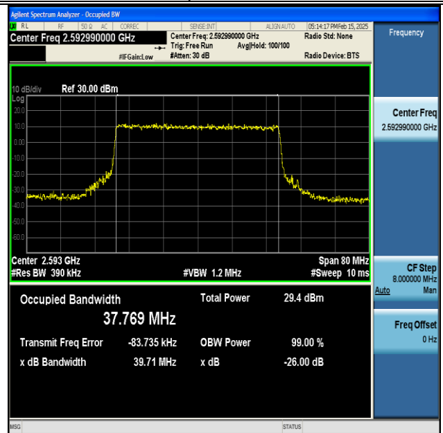
NTNV-DC_66A_n41A-PC3-30-5+40-M+M-QPSK-IDLE-CP-16QAM-Outer_Full-Ant1-PASS
