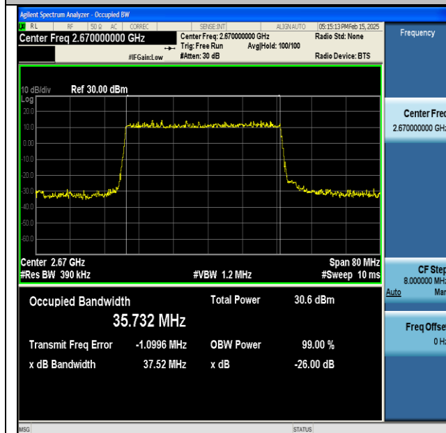
NTNV-DC_66A_n41A-PC3-30-5+40-M+H-QPSK-IDLE- DFT-16QAM-Outer_Full-Ant1-PASS
