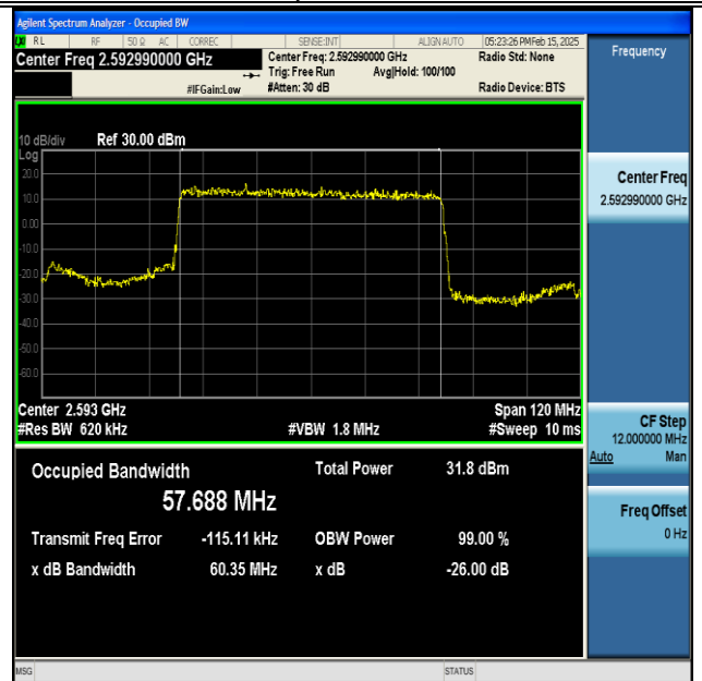
NTNV-DC_66A_n41A-PC3-30-5+60-M+M-QPSK-IDLE-DFT-BPSK-Outer_Full-Ant1-PASS
