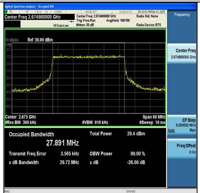
NTNV-DC_66A_n41A-PC3-30-5+30-M+H-QPSK-IDLE- CP-16QAM-Outer_Full-Ant1-PASS
