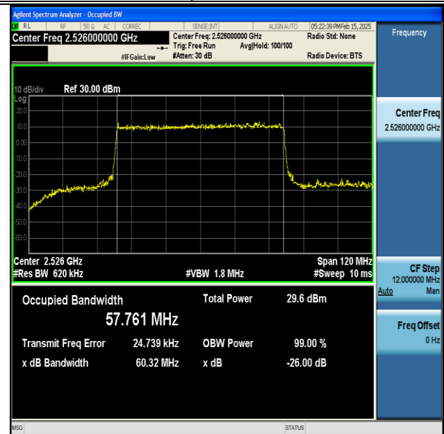
NTNV-DC_66A_n41A-PC3-30-5+60-M+L-QPSK-IDLE-CP-QPSK-Outter_Full-Ant1-PASS
