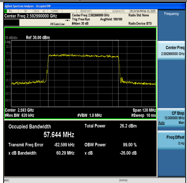
NTNV-DC_66A_n41A-PC3-30-5+60-M+M-QPSK-IDLE-CP-256QAM-Outer_Full-Ant1-PASS
