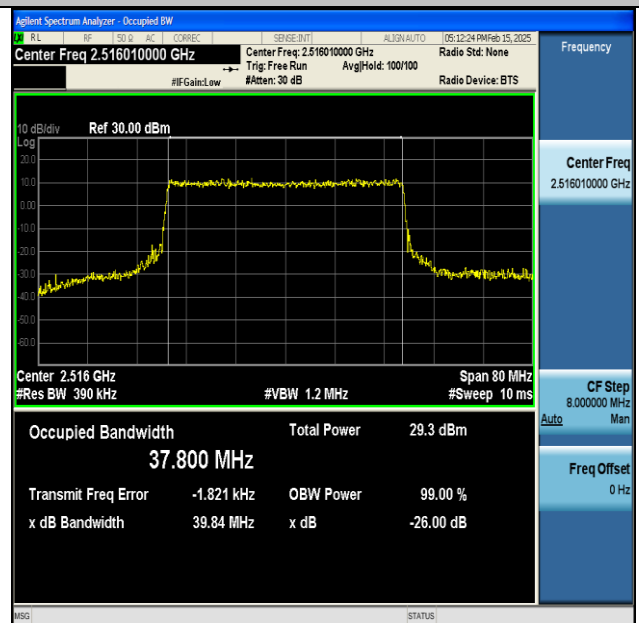
NTNV-DC_66A_n41A-PC3-30-5+40-M+L-QPSK-IDLE-CP- QPSK-Outer_Full-Ant1-PASS
