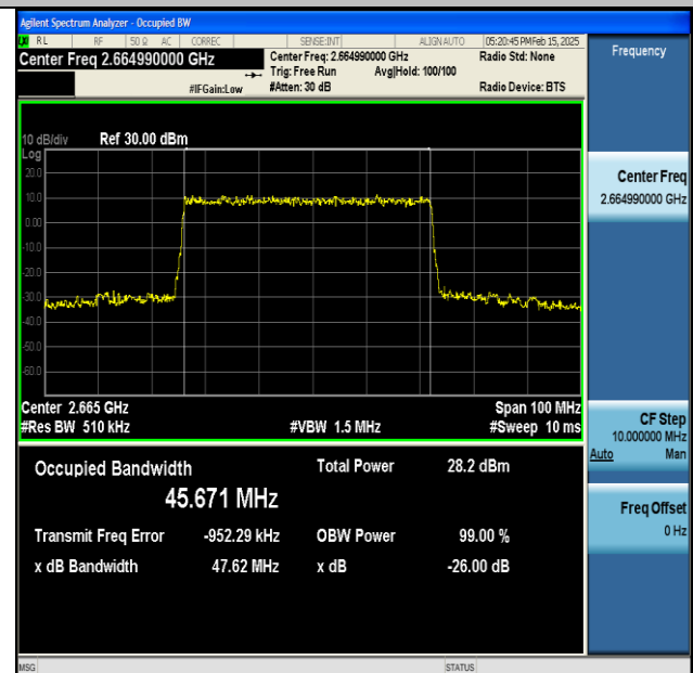
NTNV-DC_66A_n41A-PC3-30-5+50-M+H-QPSK-IDLE-DFT-256QAM-Outet_Full-Ant1-PASS
