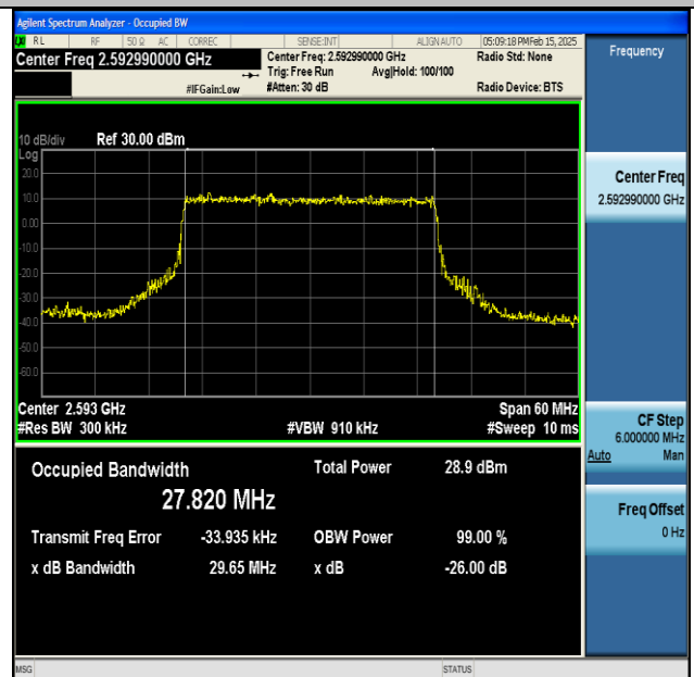
NTNV-DC_66A_n41A-PC3-30-5+30-M+M-QPSK-IDLE- CP-64QAM-Outer_Full-Ant1-PASS
