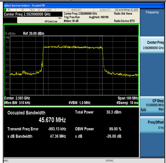
NTNV-DC_66A_n41A-PC3-30-5+50-M+M-QPSK-IDLE- DFT-64QAM-Outer_Full-Ant1-PASS
