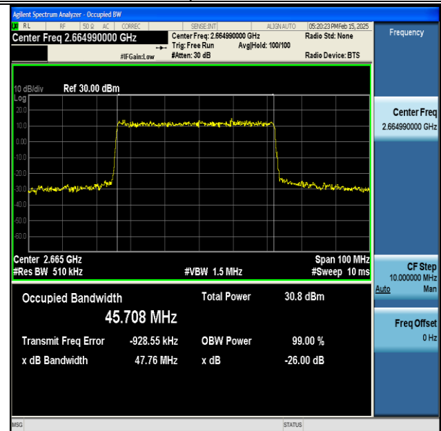
NTNV-DC_66A_n41A-PC3-30-5+50-M+H-QPSK-IDLE-DFT-16QAM-Outet_Full-Ant1-PASS
