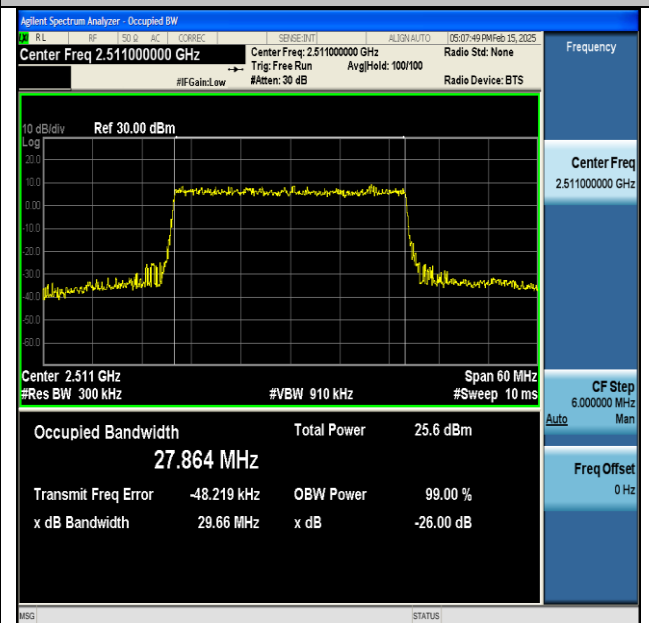
NTNV-DC_66A_n41A-PC3-30-5+30-M+L-QPSK-IDLE-CP-256QAM-Outer_Full-Ant1-PASS
