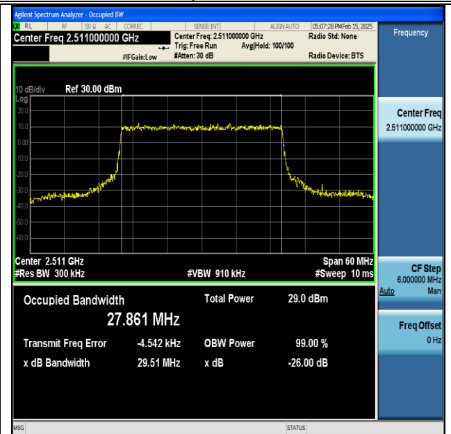
NTNV-DC_66A_n41A-PC3-30-5+30-M+L-QPSK-IDLE-CP-16QAM-Outer_Full-Ant1-PASS
