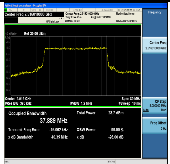
NTNV-DC_66A_n41A-PC3-30-5+40-M+L-QPSK-IDLE-CP-64QAM-Outet_Full-Ant1-PASS
