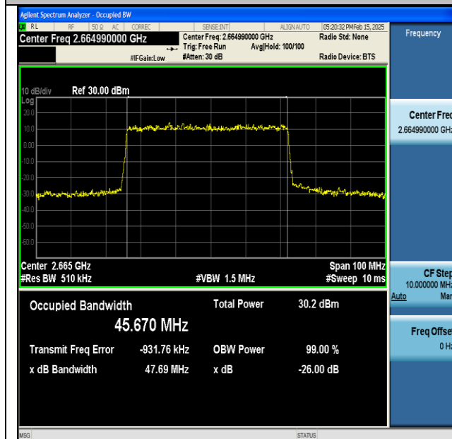
NTNV-DC_66A_n41A-PC3-30-5+50-M+H-QPSK-IDLE-DFT-64QAM-Outet_Full-Ant1-PASS
