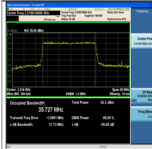
NTNV-DC_66A_n41A-PC3-30-5+40-M+L-QPSK-IDLE- DFT-16QAM-Outer_Full-Ant1-PASS
