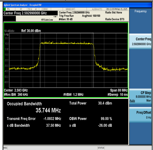
NTNV-DC_66A_n41A-PC3-30-5+40-M+M-QPSK-IDLE- DFT-16QAM-Outer_Full-Ant1-PASS
