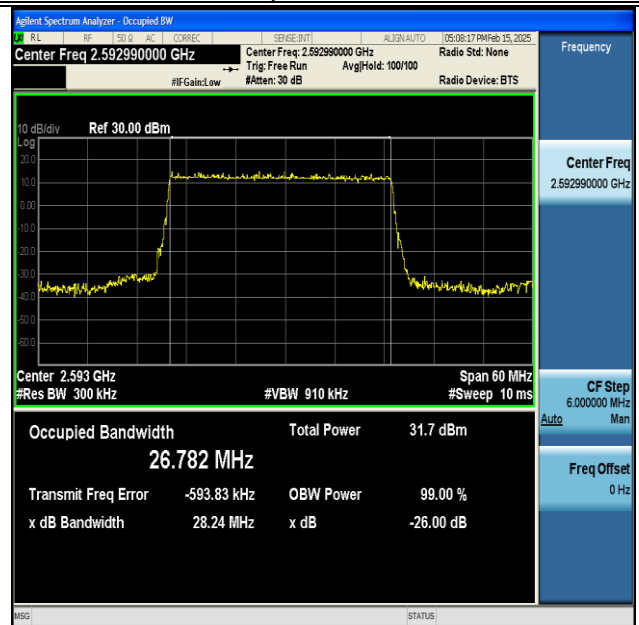
NTNV-DC_66A_n41A-PC3-30-5+30-M+M-QPSK-IDLE- DFT-QPSK-Outer_Full-Ant1-PASS
