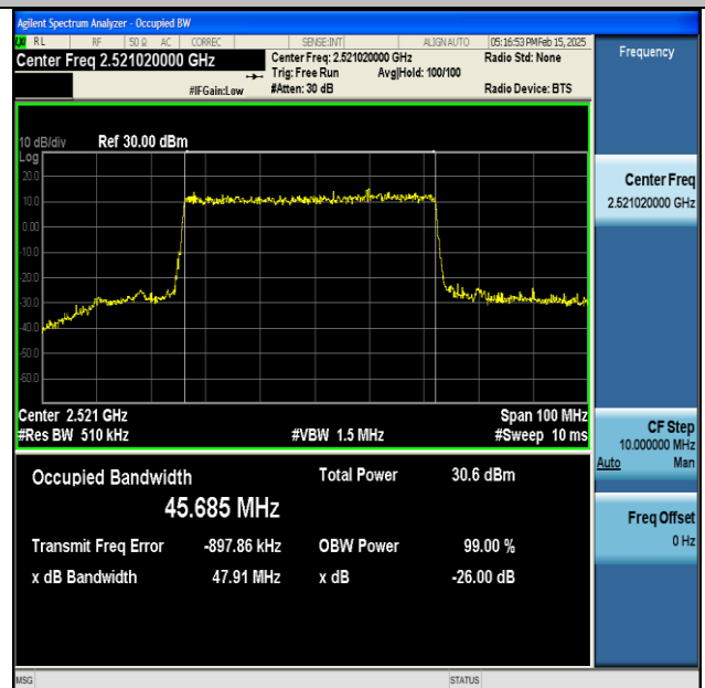
NTNV-DC_66A_n41A-PC3-30-5+50-M+L-QPSK-IDLE- DFT-16QAM-Outer_Full-Ant1-PASS
