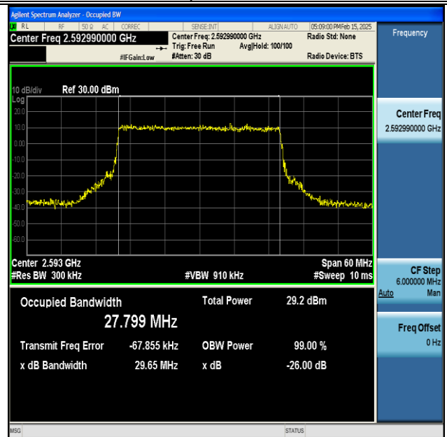
NTNV-DC_66A_n41A-PC3-30-5+30-M+M-QPSK-IDLE- CP-QPSK-Outer_Full-Ant1-PASS
