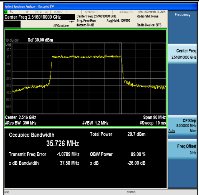
NTNV-DC_66A_n41A-PC3-30-5+40-M+L-QPSK-IDLE- DFT-64QAM-Outer_Full-Ant1-PASS
