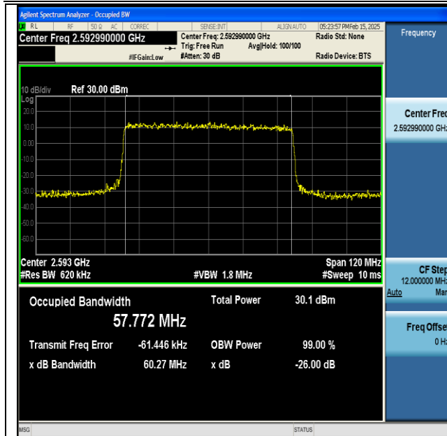
NTNV-DC_66A_n41A-PC3-30-5+60-M+M-QPSK-IDLE- DFT-64QAM-Outer_Full-Ant1-PASS
