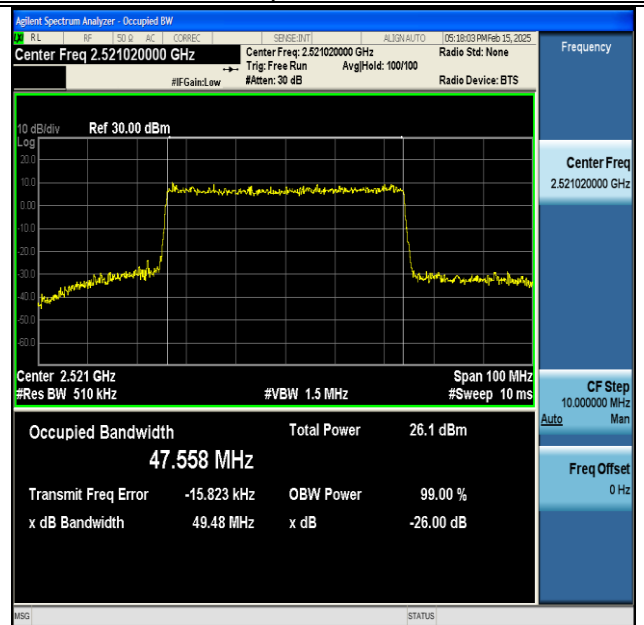
NTNV-DC_66A_n41A-PC3-30-5+50-M+L-QPSK-IDLE-CP-256QAM-Outet_Full-Ant1-PASS
