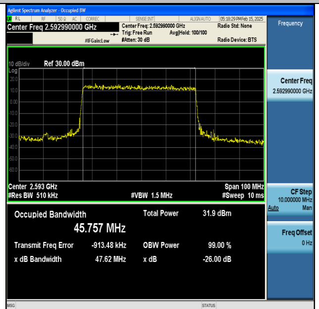
NTNV-DC_66A_n41A-PC3-30-5+50-M+M-QPSK-IDLE-DFT-QPSK-Outet_Full-Ant1-PASS
