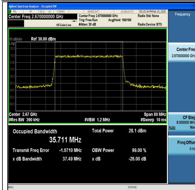
NTNV-DC_66A_n41A-PC3-30-5+40-M+H-QPSK-IDLE- DFT-256QAM-Outer_Full-Ant1-PASS
