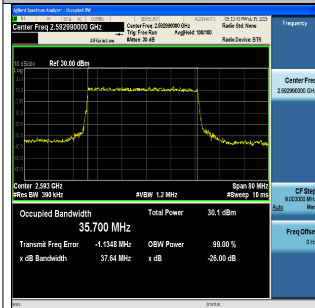
NTNV-DC_66A_n41A-PC3-30-5+40-M+M-QPSK-IDLE- DFT-64QAM-Outer_Full-Ant1-PASS
