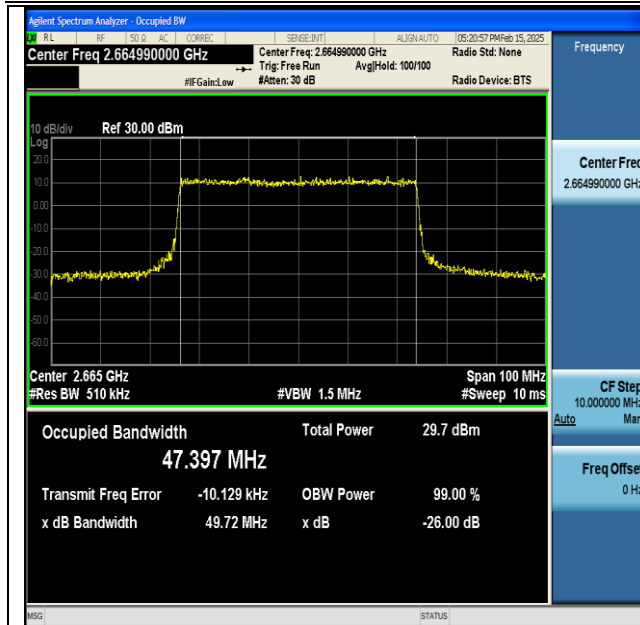
NTNV-DC_66A_n41A-PC3-30-5+50-M+H-QPSK-IDLE- CP-QPSK-Outer_Full-Ant1-PASS
