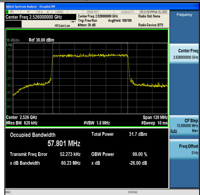
NTNV-DC_66A_n41A-PC3-30-5+60-M+L-QPSK-IDLE-DFT-QPSK-Outter_Full-Ant1-PASS
