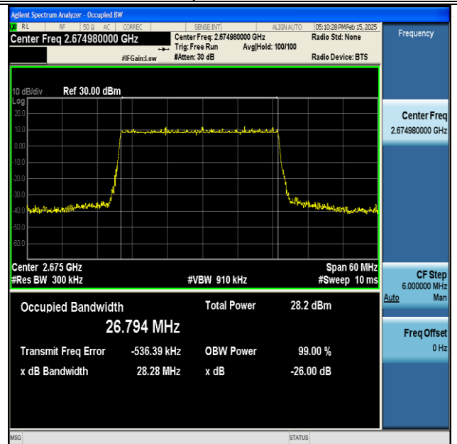
NTNV-DC_66A_n41A-PC3-30-5+30-M+H-QPSK-IDLE- DFT-256QAM-Outer_Full-Ant1-PASS
