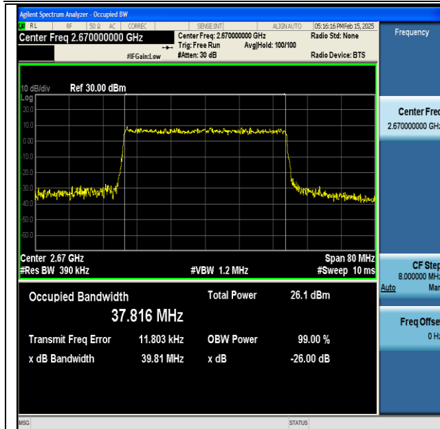
NTNV-DC_66A_n41A-PC3-30-5+40-M+H-QPSK-IDLE- CP-256QAM-Outer_Full-Ant1-PASS
