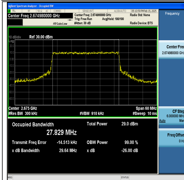
NTNV-DC_66A_n41A-PC3-30-5+30-M+H-QPSK-IDLE- CP-64QAM-Outer_Full-Ant1-PASS
