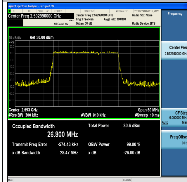
NTNV-DC_66A_n41A-PC3-30-5+30-M+M-QPSK-IDLE- DFT-16QAM-Outer_Full-Ant1-PASS
