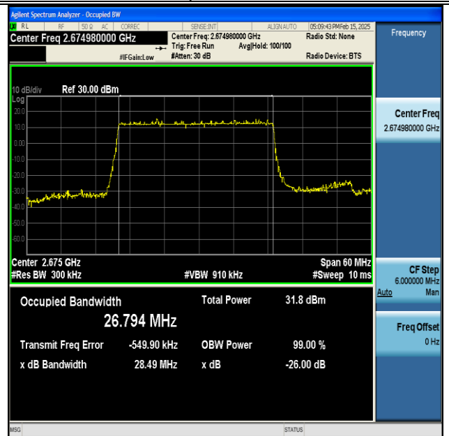
NTNV-DC_66A_n41A-PC3-30-5+30-M+H-QPSK-IDLE-DFT-BPSK-Outer_Full-Ant1-PASS
