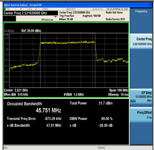
NTNV-DC_66A_n41A-PC3-30-5+50-M+L-QPSK-IDLE- DFT-BPSK-Outer_Full-Ant1-PASS
