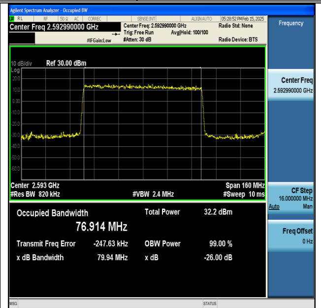
NTNV-DC_66A_n41A-PC3-30-5+80-M+M-QPSK-IDLE-DFT-QPSK-Outer_Full-Ant1-PASS
