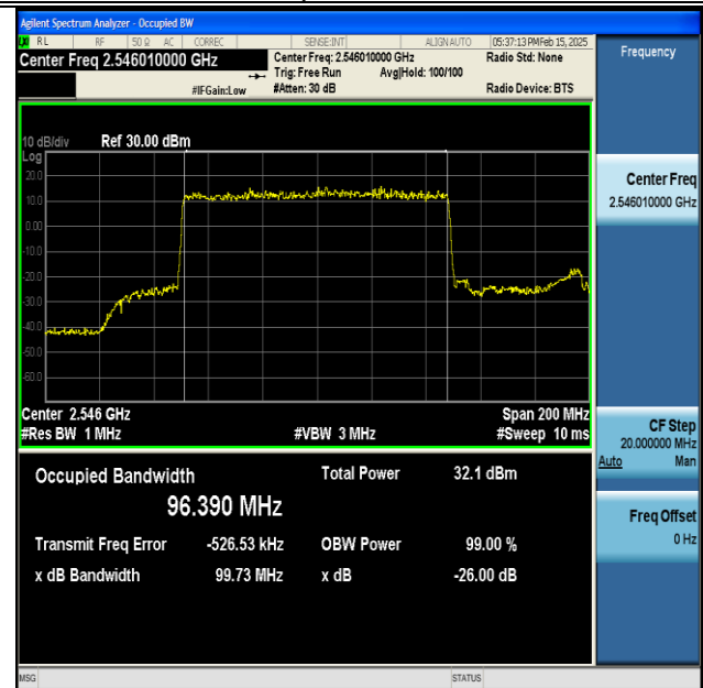
NTNV-DC_66A_n41A-PC3-30-5+100-M+L-QPSK-IDLE-DFT-BPSK-Outer_Full-Ant1-PASS
