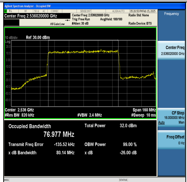
NTNV-DC_66A_n41A-PC3-30-5+80-M+L-QPSK-IDLE- DFT-BPSK-Outer_Full-Ant1-PASS
