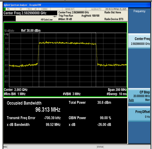
NTNV-DC_66A_n41A-PC3-30-5+100-M+M-QPSK-IDLE-DFT-64QAM-Outter_Full-Ant1-PASS
