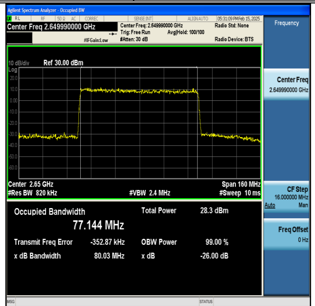
NTNV-DC_66A_n41A-PC3-30-5+80-M+H-QPSK-IDLE- DFT-256QAM-Outer_Full-Ant1-PASS
