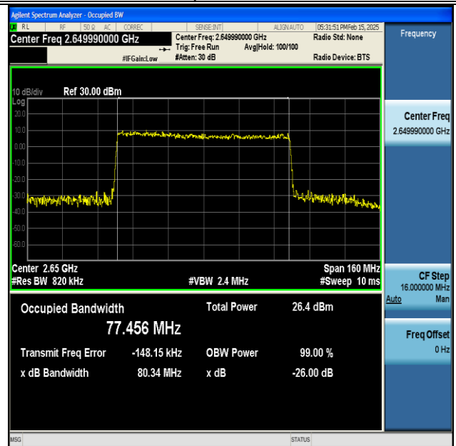
NTNV-DC_66A_n41A-PC3-30-5+80-M+H-QPSK-IDLE- CP-256QAM-Outer_Full-Ant1-PASS
