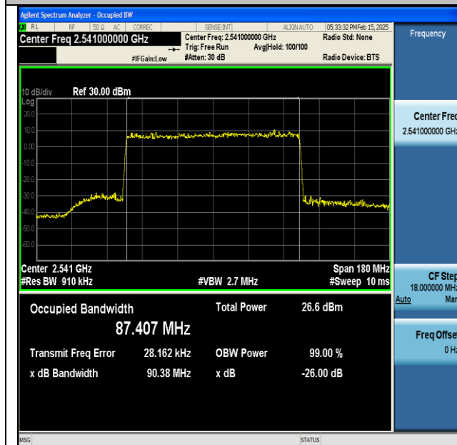
NTNV-DC_66A_n41A-PC3-30-5+90-M+L-QPSK-IDLE-CP-256QAM-Outet_Full-Ant1-PASS
