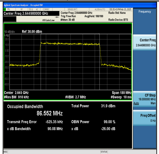
NTNV-DC_66A_n41A-PC3-30-5+90-M+H-QPSK-IDLE- DFT-QPSK-Outer_Full-Ant1-PASS
