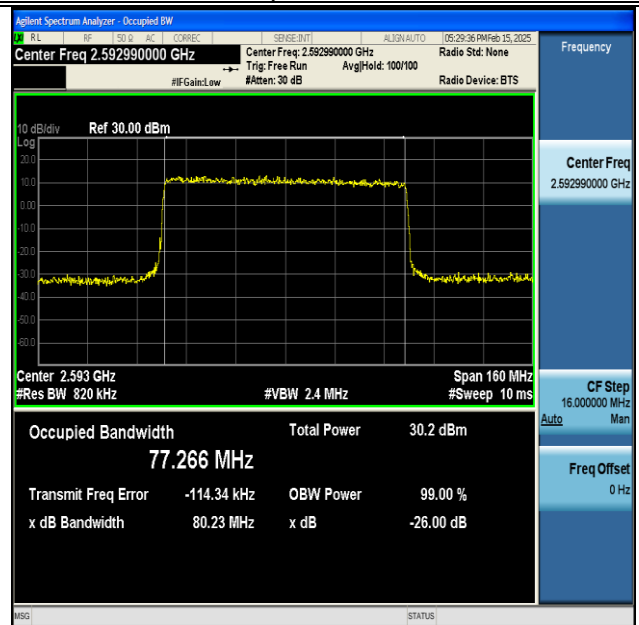
NTNV-DC_66A_n41A-PC3-30-5+80-M+M-QPSK-IDLE- CP-QPSK-Outer_Full-Ant1-PASS
