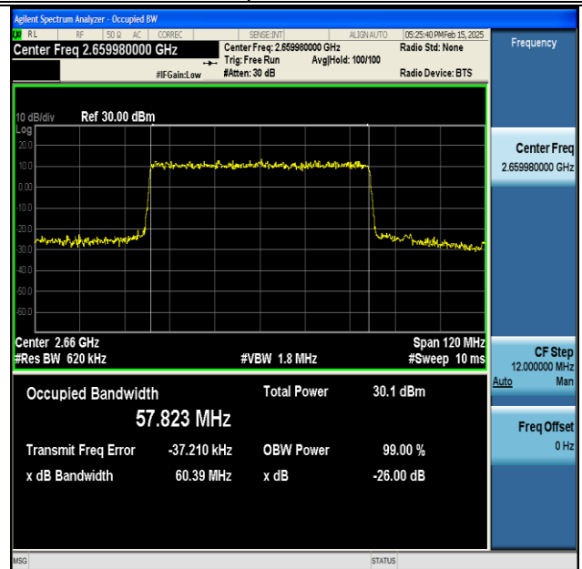
NTNV-DC_66A_n41A-PC3-30-5+60-M+H-QPSK-IDLE- DFT-64QAM-Outer_Full-Ant1-PASS
