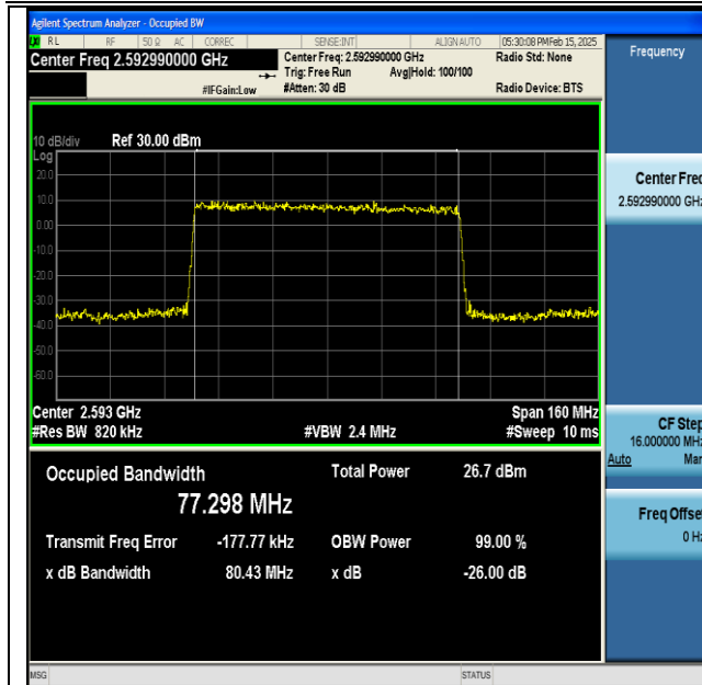
NTNV-DC_66A_n41A-PC3-30-5+80-M+M-QPSK-IDLE- CP-256QAM-Outer_Full-Ant1-PASS
