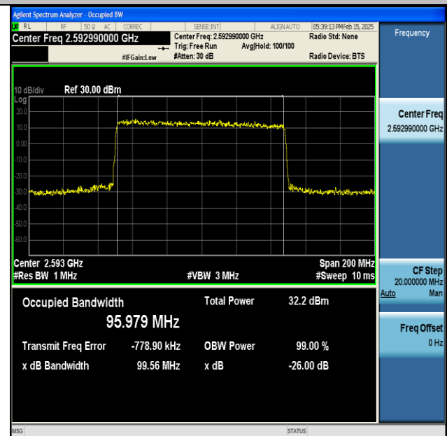
NTNV-DC_66A_n41A-PC3-30-5+100-M+M-QPSK-IDLE-DFT-QPSK-Outer_Full-Ant1-PASS
