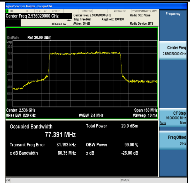
NTNV-DC_66A_n41A-PC3-30-5+80-M+L-QPSK-IDLE-CP-16QAM-Outer_Full-Ant1-PASS
