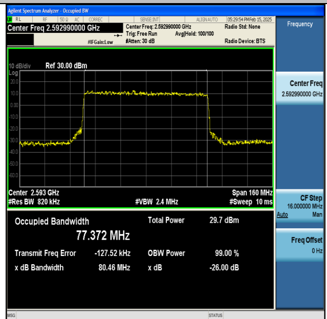
NTNV-DC_66A_n41A-PC3-30-5+80-M+M-QPSK-IDLE- CP-64QAM-Outer_Full-Ant1-PASS
