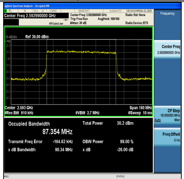
NTNV-DC_66A_n41A-PC3-30-5+90-M+M-QPSK-IDLE-CP-16QAM-Outer_Full-Ant1-PASS
