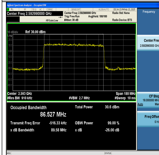
NTNV-DC_66A_n41A-PC3-30-5+90-M+M-QPSK-IDLE- DFT-64QAM-Outer_Full-Ant1-PASS
