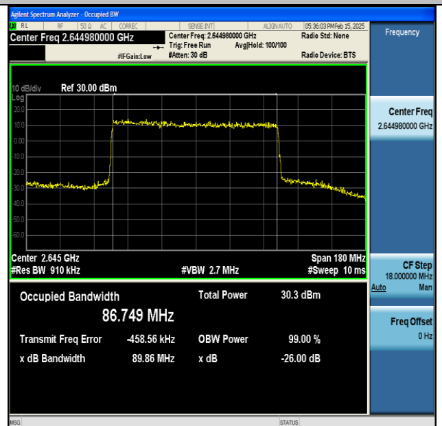
NTNV-DC_66A_n41A-PC3-30-5+90-M+H-QPSK-IDLE- DFT-64QAM-Outer_Full-Ant1-PASS
