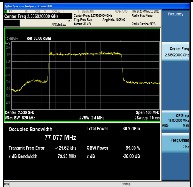
NTNV-DC_66A_n41A-PC3-30-5+80-M+L-QPSK-IDLE- DFT-16QAM-Outer_Full-Ant1-PASS
