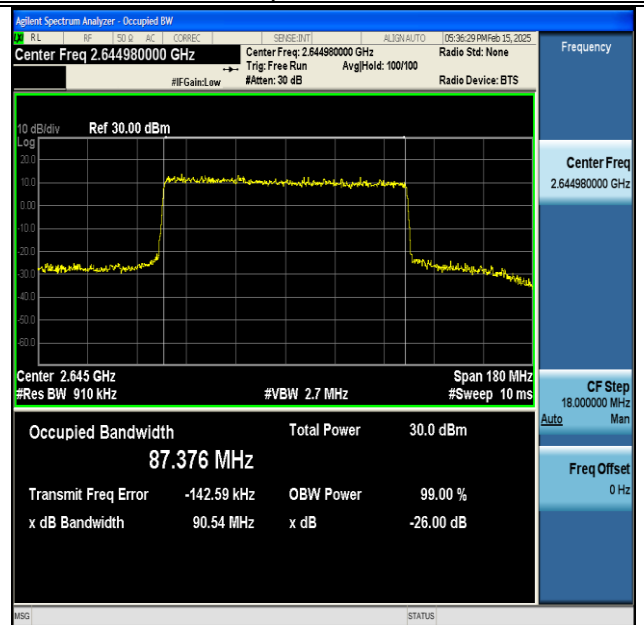
NTNV-DC_66A_n41A-PC3-30-5+90-M+H-QPSK-IDLE- CP-QPSK-Outer_Full-Ant1-PASS
