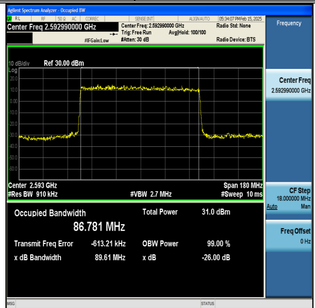
NTNV-DC_66A_n41A-PC3-30-5+90-M+M-QPSK-IDLE- DFT-16QAM-Outer_Full-Ant1-PASS
