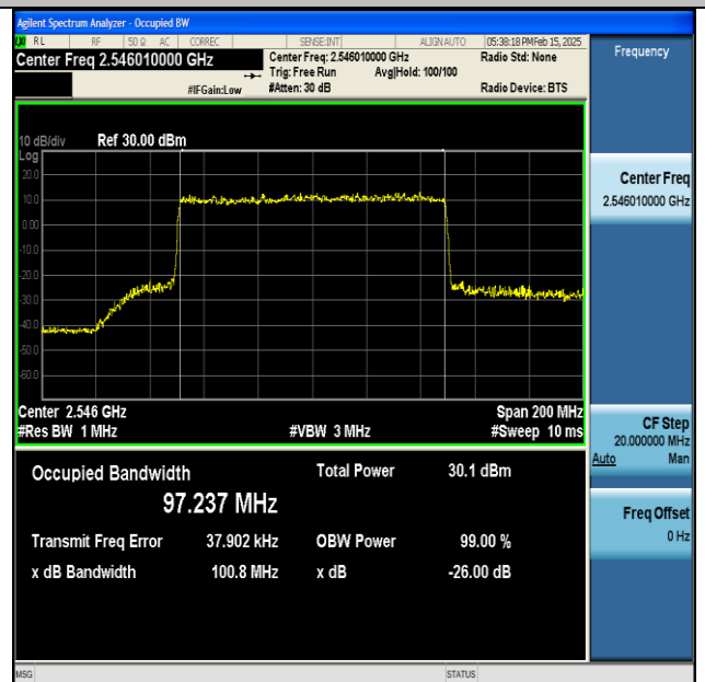
NTNV-DC_66A_n41A-PC3-30-5+100-M+L-QPSK-IDLE- CP-16QAM-Outer_Full-Ant1-PASS
