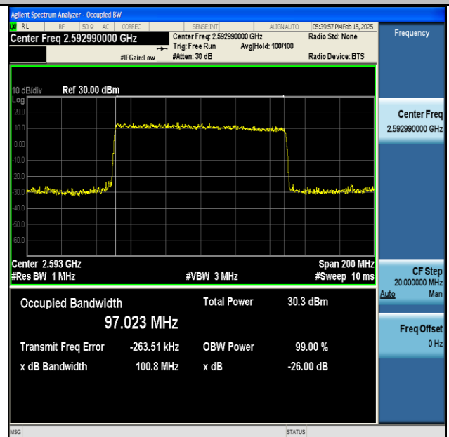
NTNV-DC_66A_n41A-PC3-30-5+100-M+M-QPSK-IDLE-CP-QPSK-Outter_Full-Ant1-PASS
