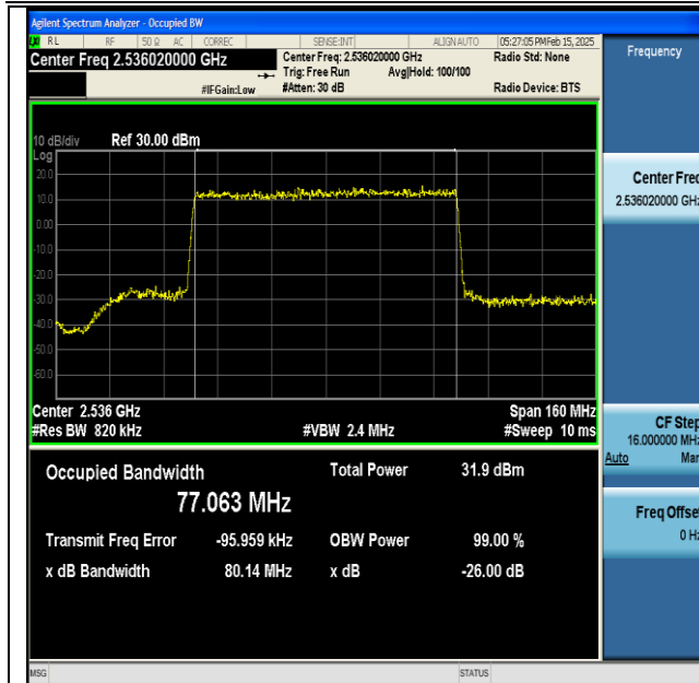
NTNV-DC_66A_n41A-PC3-30-5+80-M+L-QPSK-IDLE- DFT-QPSK-Outer_Full-Ant1-PASS
