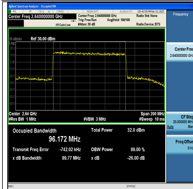
NTNV-DC_66A_n41A-PC3-30-5+100-M+H-QPSK-IDLE-DFT-QPSK-Outer_Full-Ant1-PASS
