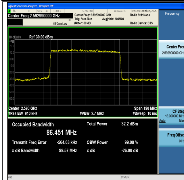
NTNV-DC_66A_n41A-PC3-30-5+90-M+M-QPSK-IDLE- DFT-QPSK-Outer_Full-Ant1-PASS
