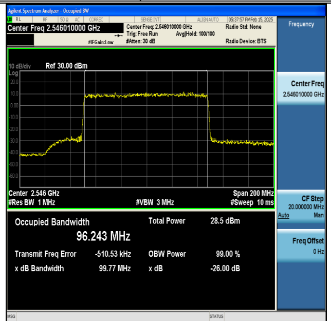
NTNV-DC_66A_n41A-PC3-30-5+100-M+L-QPSK-IDLE- DFT-256QAM-Outer_Full-Ant1-PASS
