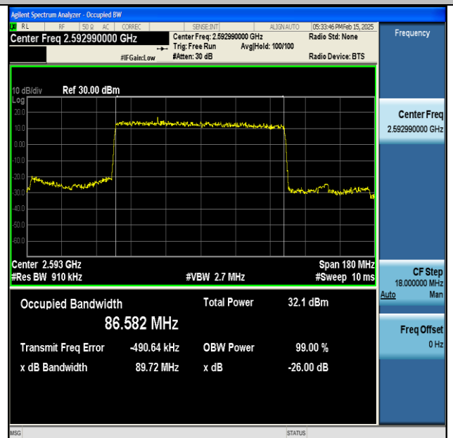
NTNV-DC_66A_n41A-PC3-30-5+90-M+M-QPSK-IDLE-DFT-BPSK-Outet_Full-Ant1-PASS
