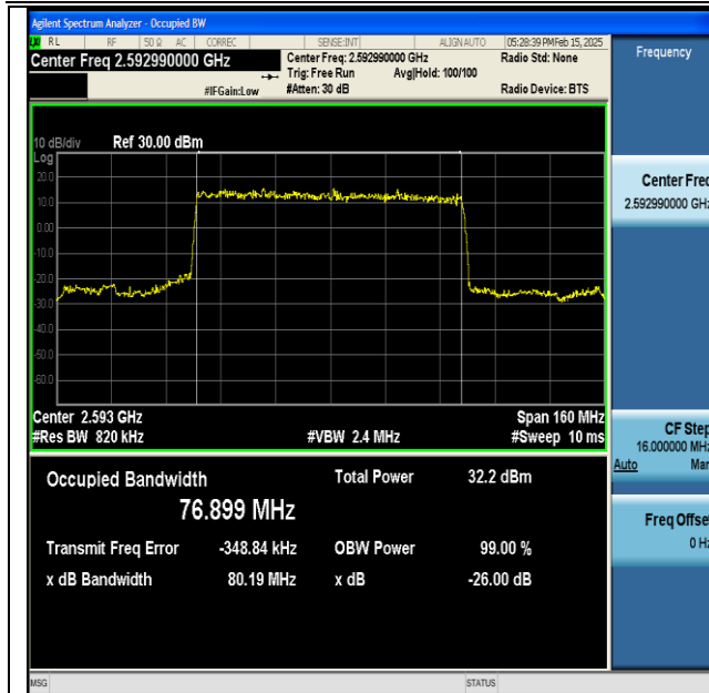
NTNV-DC_66A_n41A-PC3-30-5+80-M+M-QPSK-IDLE-DFT-BPSK-Outer_Full-Ant1-PASS
