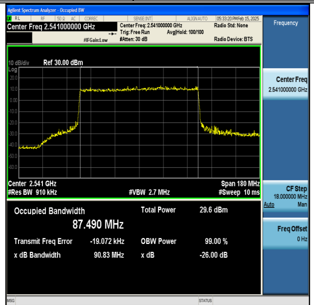
NTNV-DC_66A_n41A-PC3-30-5+90-M+L-QPSK-IDLE-CP-64QAM-Outet_Full-Ant1-PASS
