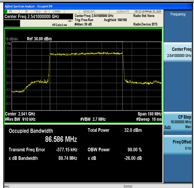
NTNV-DC_66A_n41A-PC3-30-5+90-M+L-QPSK-IDLE- DFT-QPSK-Outer_Full-Ant1-PASS
