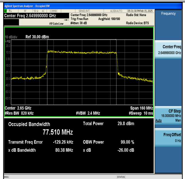
NTNV-DC_66A_n41A-PC3-30-5+80-M+H-QPSK-IDLE- CP-16QAM-Outer_Full-Ant1-PASS
