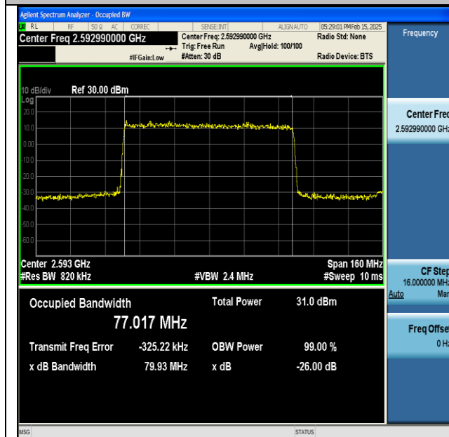
NTNV-DC_66A_n41A-PC3-30-5+80-M+M-QPSK-IDLE-DFT-16QAM-Outer_Full-Ant1-PASS
