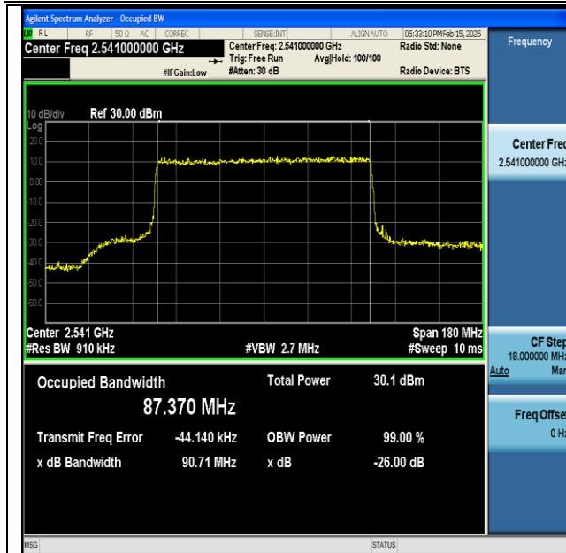
NTNV-DC_66A_n41A-PC3-30-5+90-M+L-QPSK-IDLE-CP-16QAM-Outet_Full-Ant1-PASS
