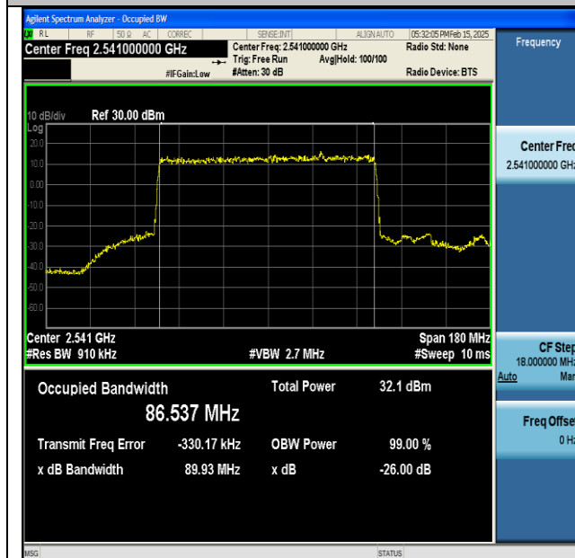
NTNV-DC_66A_n41A-PC3-30-5+90-M+L-QPSK-IDLE- DFT-BPSK-Outer_Full-Ant1-PASS
