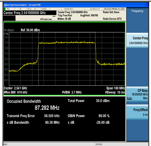
NTNV-DC_66A_n41A-PC3-30-5+90-M+L-QPSK-IDLE-CP-QPSK-Outter_Full-Ant1-PASS
