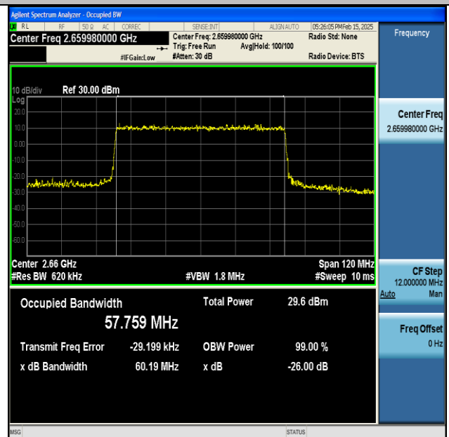
NTNV-DC_66A_n41A-PC3-30-5+60-M+H-QPSK-IDLE- CP-QPSK-Outer_Full-Ant1-PASS
