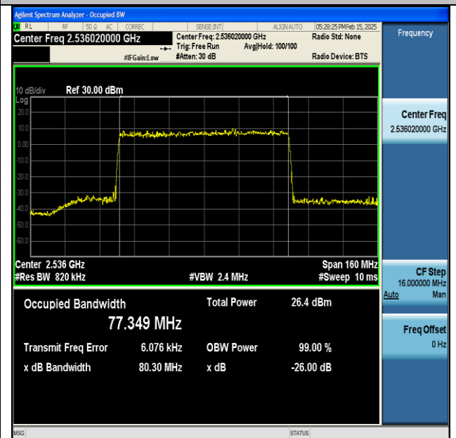
NTNV-DC_66A_n41A-PC3-30-5+80-M+L-QPSK-IDLE-CP-256QAM-Outer_Full-Ant1-PASS
