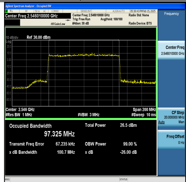
NTNV-DC_66A_n41A-PC3-30-5+100-M+L-QPSK-IDLE-CP-256QAM-Outer_Full-Ant1-PASS
