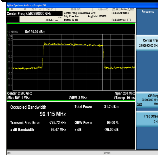
NTNV-DC_66A_n41A-PC3-30-5+100-M+M-QPSK-IDLE-DFT-16QAM-Outter_Full-Ant1-PASS
