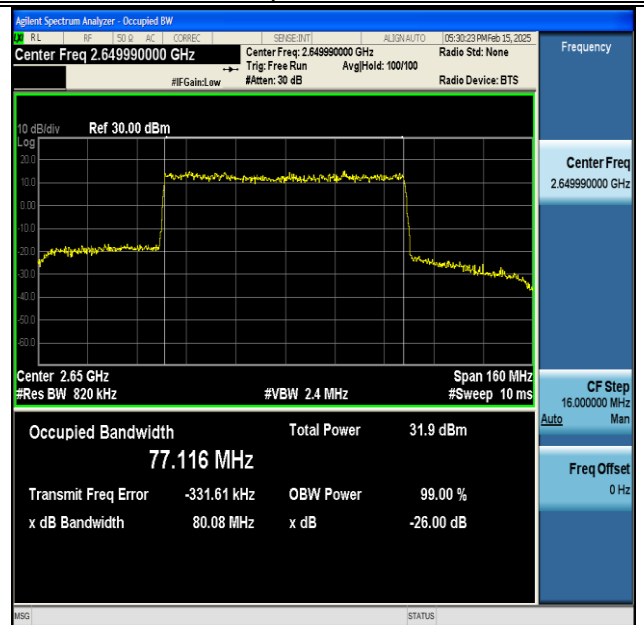
NTNV-DC_66A_n41A-PC3-30-5+80-M+H-QPSK-IDLE- DFT-BPSK-Outer_Full-Ant1-PASS
