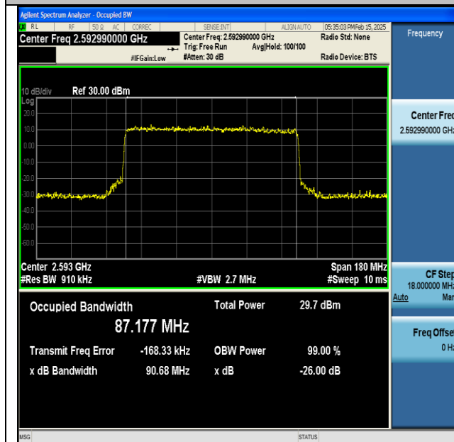
NTNV-DC_66A_n41A-PC3-30-5+90-M+M-QPSK-IDLE-CP-64QAM-Outer_Full-Ant1-PASS
