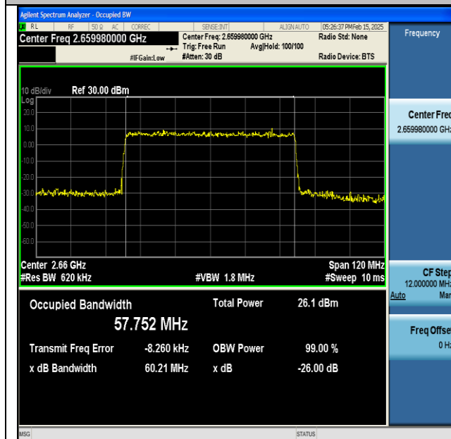
NTNV-DC_66A_n41A-PC3-30-5+60-M+H-QPSK-IDLE- CP-256QAM-Outer_Full-Ant1-PASS
