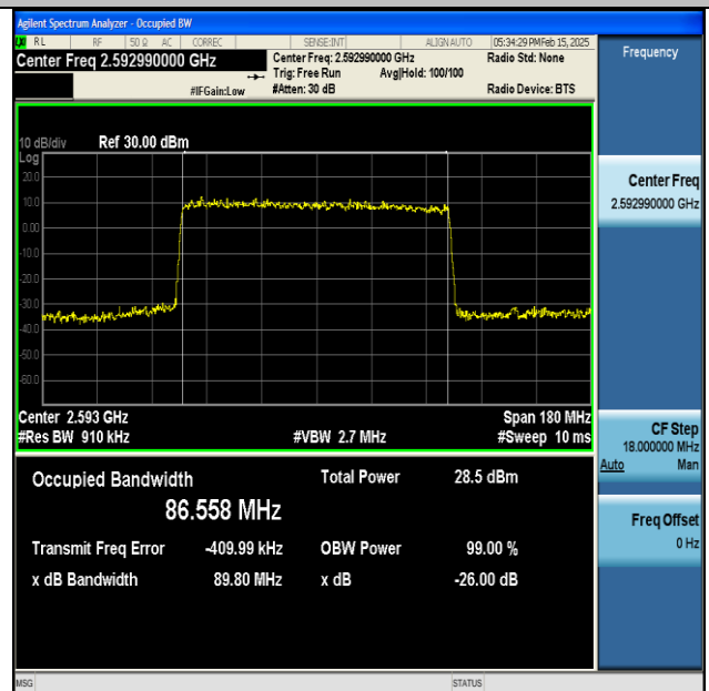
NTNV-DC_66A_n41A-PC3-30-5+90-M+M-QPSK-IDLE- DFT-256QAM-Outer_Full-Ant1-PASS
