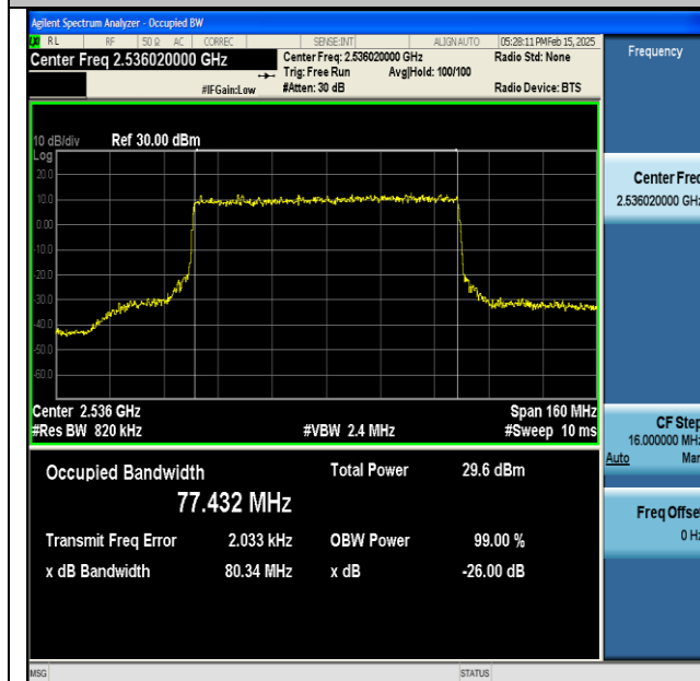
NTNV-DC_66A_n41A-PC3-30-5+80-M+L-QPSK-IDLE-CP-64QAM-Outer_Full-Ant1-PASS
