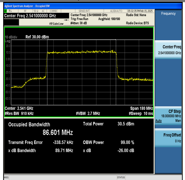
NTNV-DC_66A_n41A-PC3-30-5+90-M+L-QPSK-IDLE-DFT-64QAM-Outter_Full-Ant1-PASS
