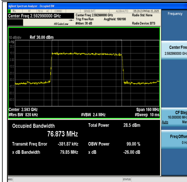
NTNV-DC_66A_n41A-PC3-30-5+80-M+M-QPSK-IDLE- DFT-256QAM-Outer_Full-Ant1-PASS
