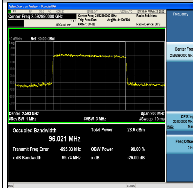
NTNV-DC_66A_n41A-PC3-30-5+100-M+M-QPSK-IDLE-DFT-256QAM-Outter_Full-Ant1-PASS
