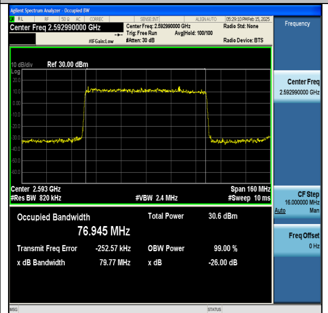
NTNV-DC_66A_n41A-PC3-30-5+80-M+M-QPSK-IDLE-DFT-64QAM-Outer_Full-Ant1-PASS
