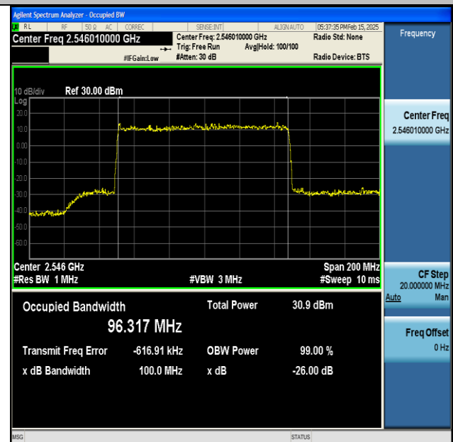
NTNV-DC_66A_n41A-PC3-30-5+100-M+L-QPSK-IDLE-DFT-16QAM-Outer_Full-Ant1-PASS
