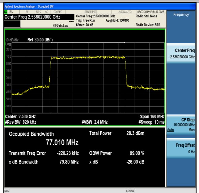
NTNV-DC_66A_n41A-PC3-30-5+80-M+L-QPSK-IDLE- DFT-256QAM-Outer_Full-Ant1-PASS
