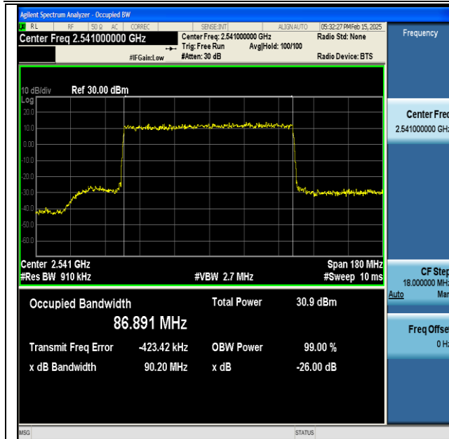
NTNV-DC_66A_n41A-PC3-30-5+90-M+L-QPSK-IDLE-DFT-16QAM-Outter_Full-Ant1-PASS
