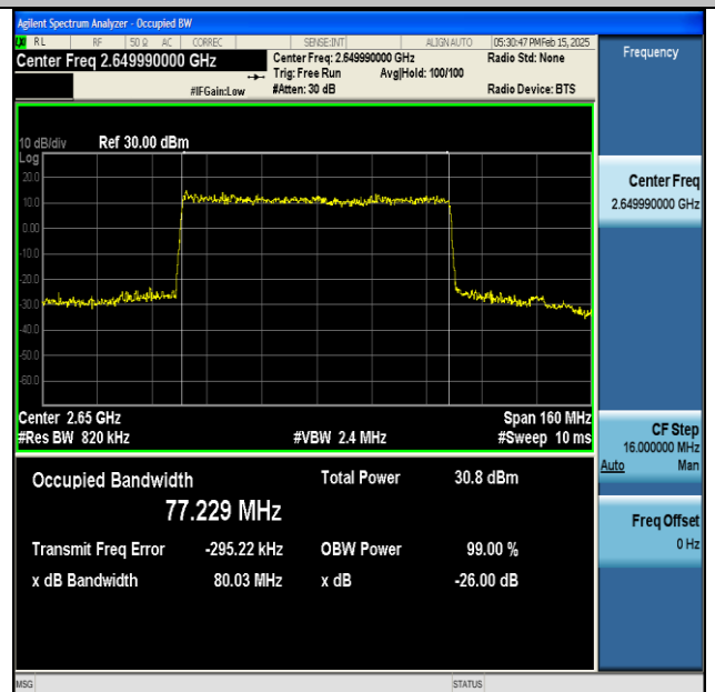
NTNV-DC_66A_n41A-PC3-30-5+80-M+H-QPSK-IDLE- DFT-16QAM-Outer_Full-Ant1-PASS
