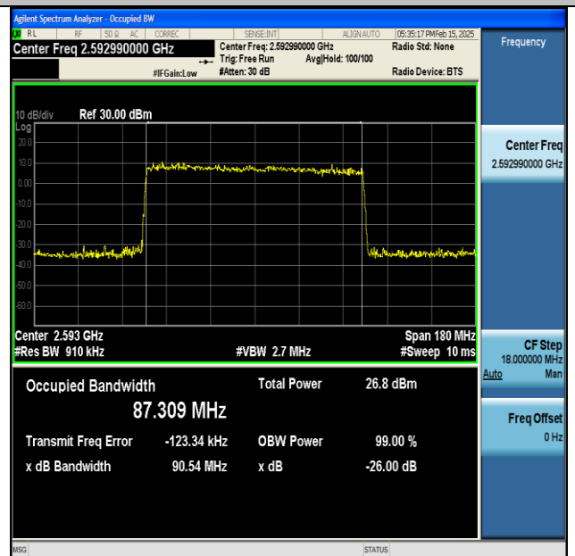
NTNV-DC_66A_n41A-PC3-30-5+90-M+M-QPSK-IDLE-CP-256QAM-Outer_Full-Ant1-PASS
