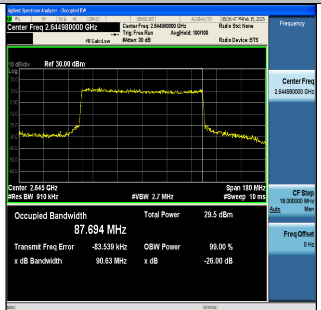
NTNV-DC_66A_n41A-PC3-30-5+90-M+H-QPSK-IDLE- CP-64QAM-Outer_Full-Ant1-PASS
