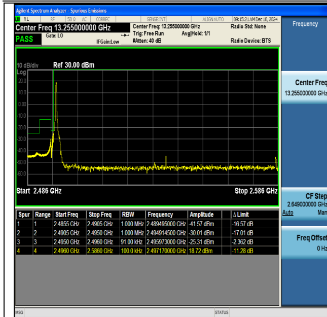
NTNV-DC_66A_n41A-PC3-30-5+90-M+L-QPSK-IDLE- DFT-BPSK-Edge_1RB_Left-PASS
