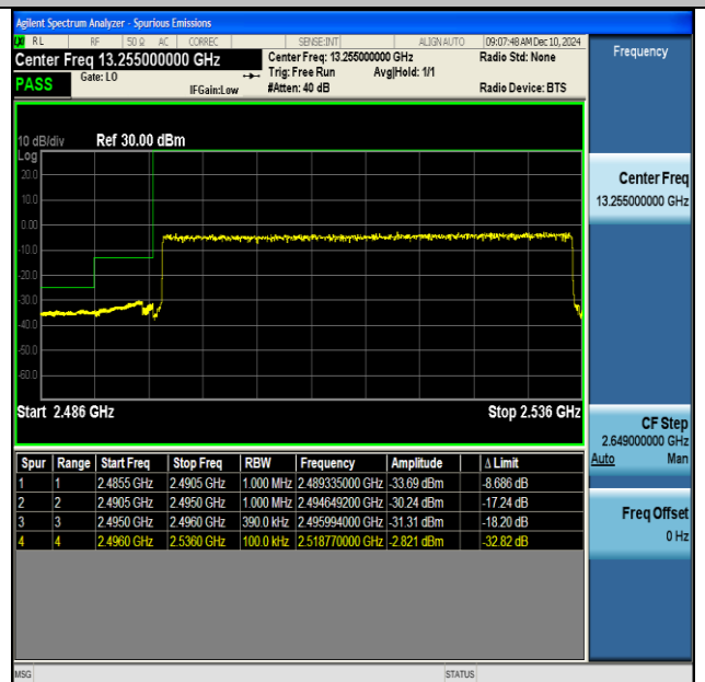
NTNV-DC_66A_n41A-PC3-30-5+40-M+L-QPSK-IDLE- CP-QPSK-Outer_Full-PASS
