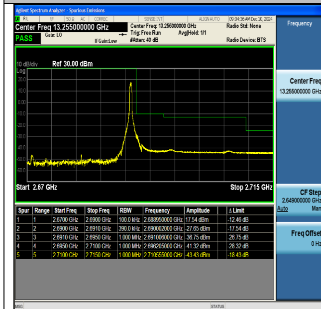
NTNV-DC_66A_n41A-PC3-30-5+20-M+H-QPSK-IDLE-CP- QPSK-Edge_1RB_Right-PASS
