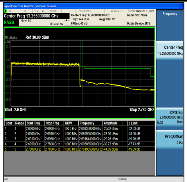
NTNV-DC_66A_n41A-PC3-30-5+90-M+H-QPSK-IDLE- DFT-BPSK-Outer_Full-PASS
