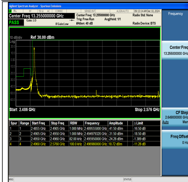
NTNV-DC_66A_n41A-PC3-30-5+80-M+L-QPSK-IDLE- DFT-BPSK-Edge_1RB_Left-PASS
