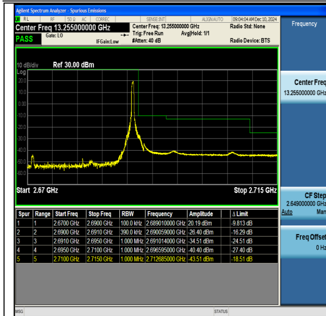
NTNV-DC_66A_n41A-PC3-30-5+20-M+H-QPSK-IDLE- DFT-BPSK-Edge_1RB_Right-PASS
