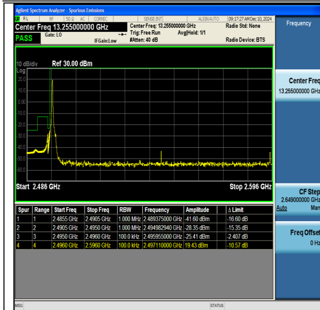
NTNV-DC_66A_n41A-PC3-30-5+100-M+L-QPSK-IDLE- DFT-BPSK-Edge_1RB_Left-PASS
