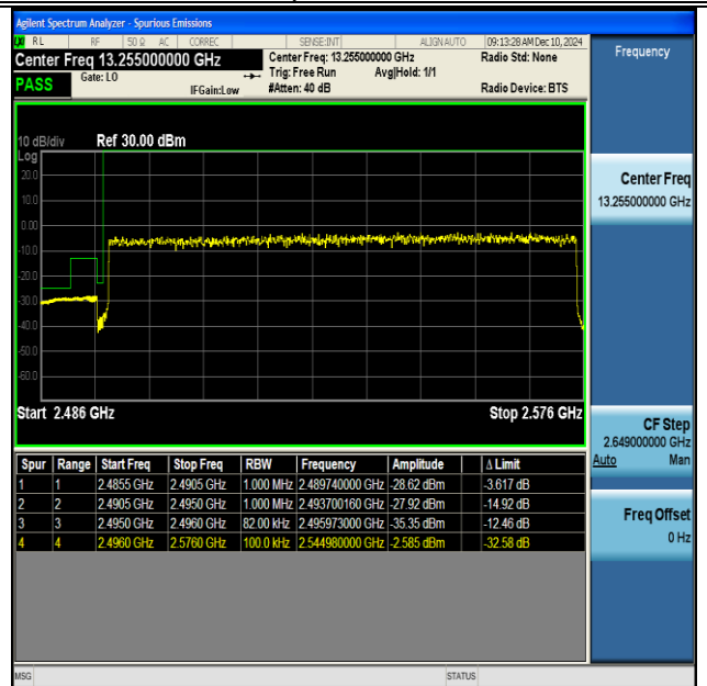
NTNV-DC_66A_n41A-PC3-30-5+80-M+L-QPSK-IDLE- DFT-BPSK-Outer_Full-PASS
