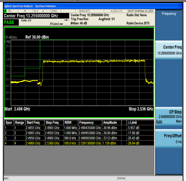
NTNV-DC_66A_n41A-PC3-30-5+40-M+L-QPSK-IDLE- DFT-BPSK-Outer_Full-PASS
