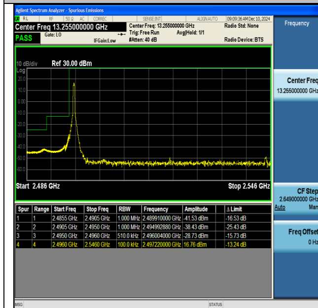
NTNV-DC_66A_n41A-PC3-30-5+50-M+L-QPSK-IDLE-CP- QPSK-Edge_1RB_Left-PASS
