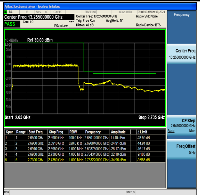
NTNV-DC_66A_n41A-PC3-30-5+40-M+H-QPSK-IDLE- DFT-BPSK-Outer_Full-PASS
