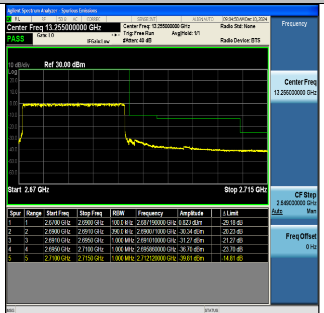
NTNV-DC_66A_n41A-PC3-30-5+20-M+H-QPSK-IDLE- CP-QPSK-Outer_Full-PASS
