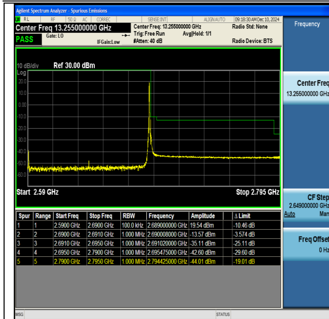
NTNV-DC_66A_n41A-PC3-30-5+100-M+H-QPSK-IDLE- DFT-BPSK-Edge_1RB_Right-PASS
