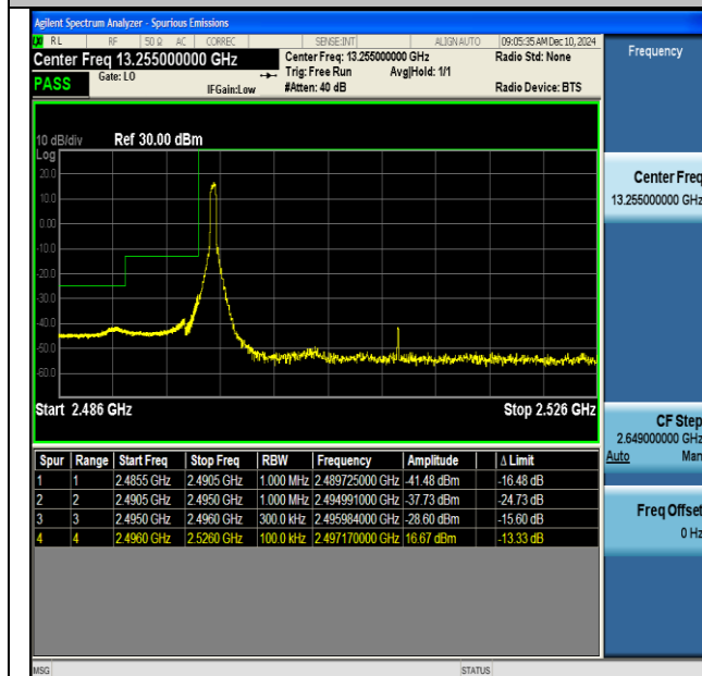
NTNV-DC_66A_n41A-PC3-30-5+30-M+L-QPSK-IDLE-CP- QPSK-Edge_1RB_Left-PASS
