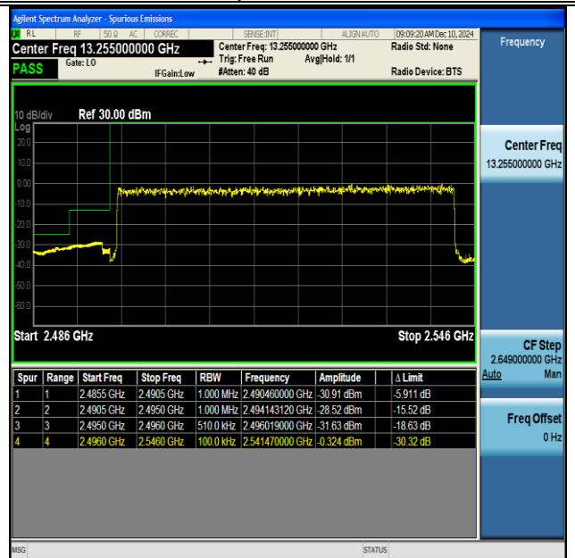
NTNV-DC_66A_n41A-PC3-30-5+50-M+L-QPSK-IDLE- DFT-BPSK-Outer_Full-PASS
