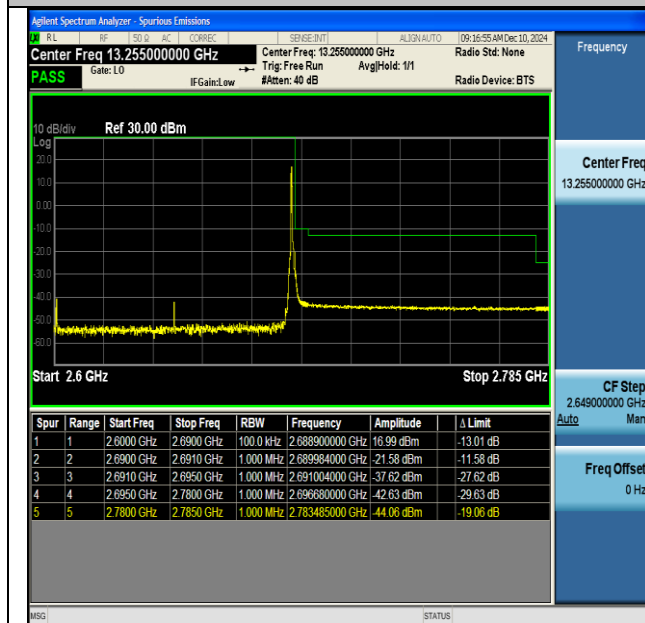
NTNV-DC_66A_n41A-PC3-30-5+90-M+H-QPSK-IDLE-CP- QPSK-Edge_1RB_Right-PASS
