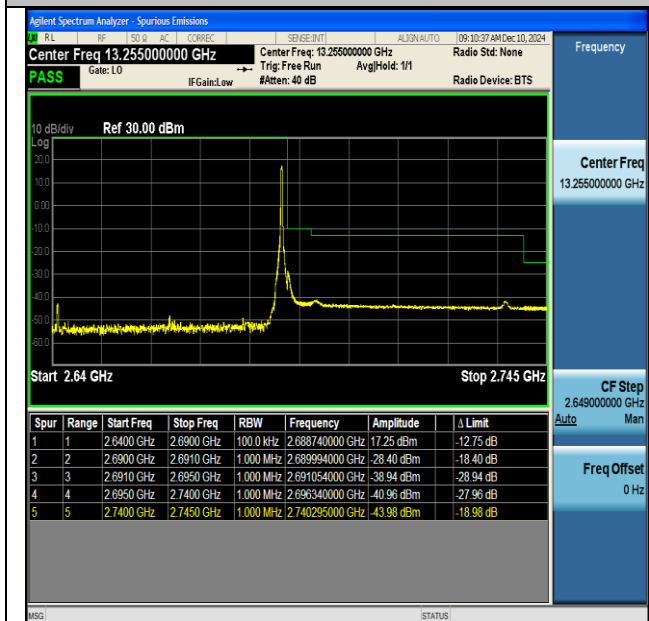
NTNV-DC_66A_n41A-PC3-30-5+50-M+H-QPSK-IDLE-CP- QPSK-Edge_1RB_Right-PASS
