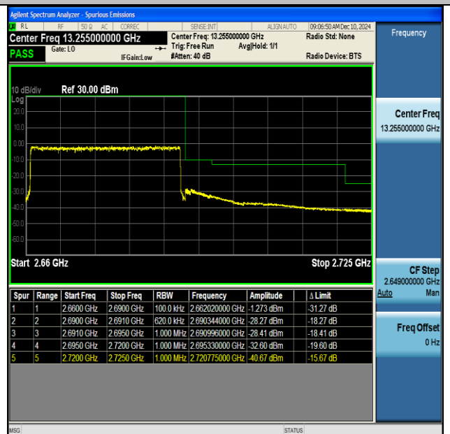
NTNV-DC_66A_n41A-PC3-30-5+30-M+H-QPSK-IDLE- CP-QPSK-Outer_Full-PASS
