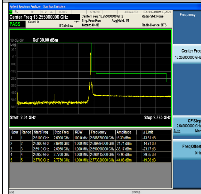
NTNV-DC_66A_n41A-PC3-30-5+80-M+H-QPSK-IDLE-CP- QPSK-Edge_1RB_Right-PASS
