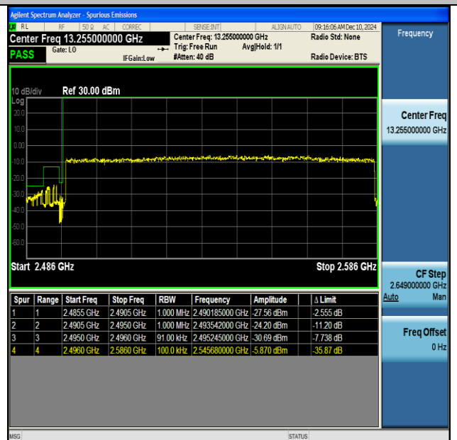
NTNV-DC_66A_n41A-PC3-30-5+90-M+L-QPSK-IDLE- CP-QPSK-Outer_Full-PASS
