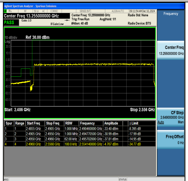
NTNV-DC_66A_n41A-PC3-30-5+60-M+L-QPSK-IDLE- CP-QPSK-Outer_Full-PASS
