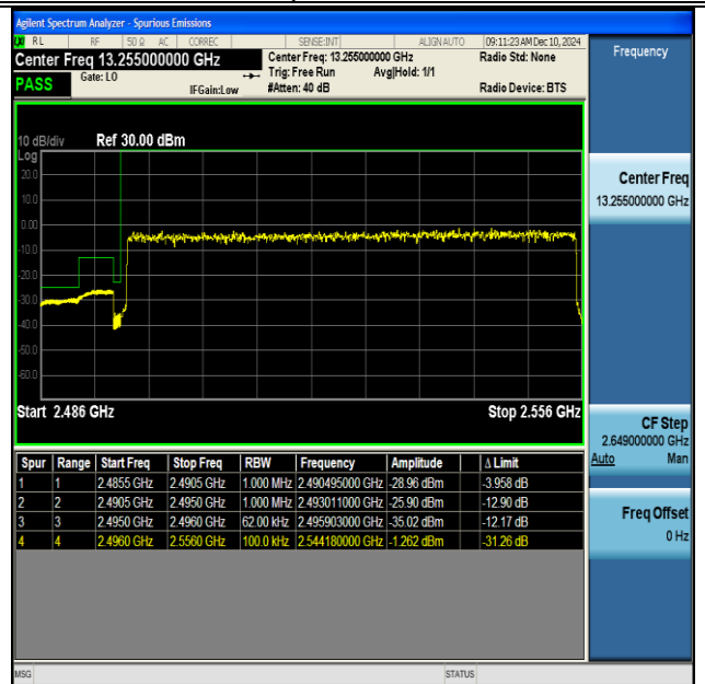
NTNV-DC_66A_n41A-PC3-30-5+60-M+L-QPSK-IDLE- DFT-BPSK-Outer_Full-PASS
