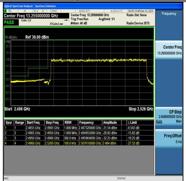
NTNV-DC_66A_n41A-PC3-30-5+30-M+L-QPSK-IDLE- DFT-BPSK-Outer_Full-PASS
