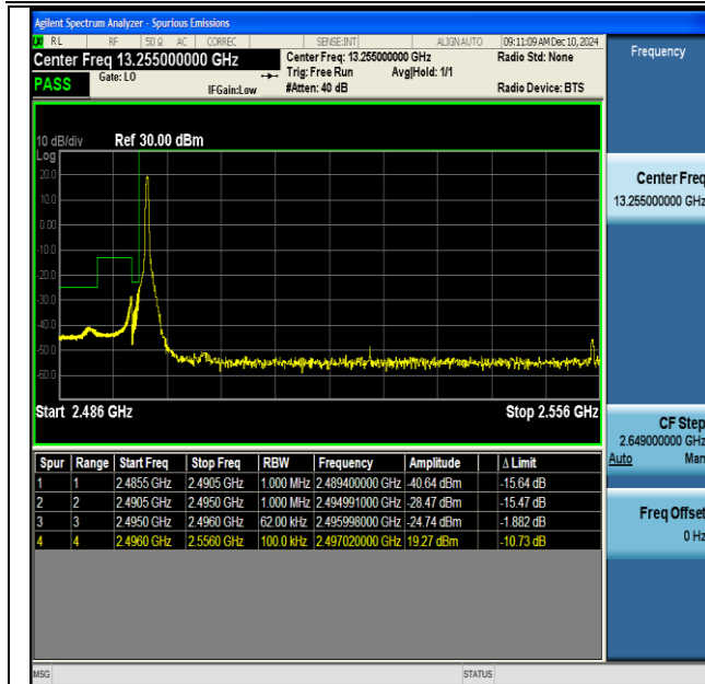
NTNV-DC_66A_n41A-PC3-30-5+60-M+L-QPSK-IDLE- DFT-BPSK-Edge_1RB_Left-PASS
