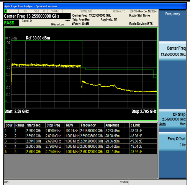
NTNV-DC_66A_n41A-PC3-30-5+100-M+H-QPSK-IDLE- DFT-BPSK-Outer_Full-PASS
