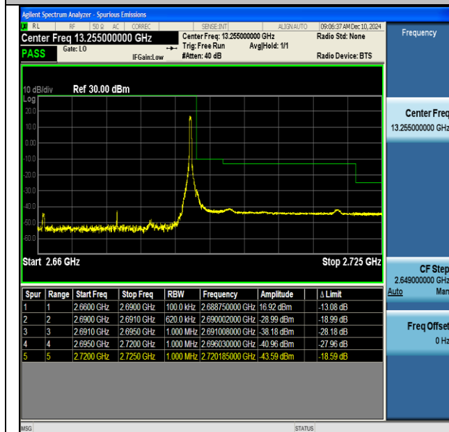
NTNV-DC_66A_n41A-PC3-30-5+30-M+H-QPSK-IDLE-CP- QPSK-Edge_1RB_Right-PASS
