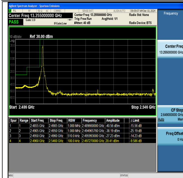
NTNV-DC_66A_n41A-PC3-30-5+50-M+L-QPSK-IDLE- DFT-BPSK-Edge_1RB_Left-PASS
