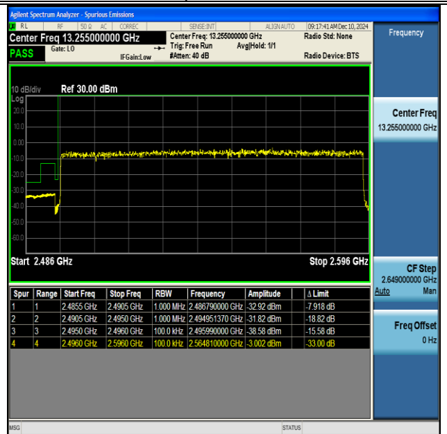
NTNV-DC_66A_n41A-PC3-30-5+100-M+L-QPSK-IDLE- DFT-BPSK-Outer_Full-PASS
