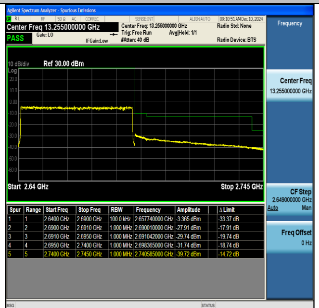
NTNV-DC_66A_n41A-PC3-30-5+50-M+H-QPSK-IDLE- CP-QPSK-Outer_Full-PASS
