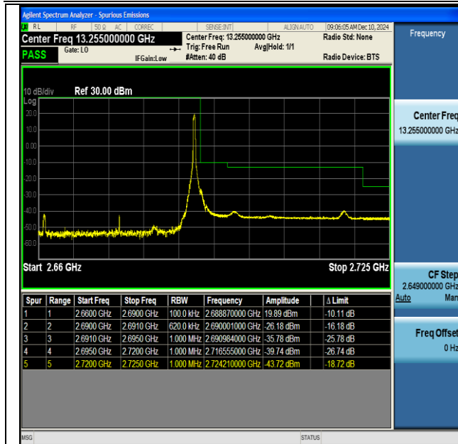
NTNV-DC_66A_n41A-PC3-30-5+30-M+H-QPSK-IDLE- DFT-BPSK-Edge_1RB_Right-PASS
