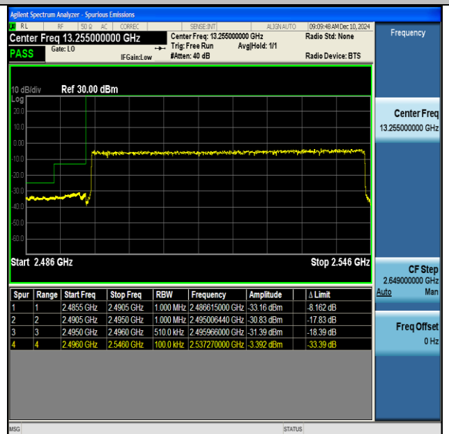
NTNV-DC_66A_n41A-PC3-30-5+50-M+L-QPSK-IDLE- CP-QPSK-Outer_Full-PASS
