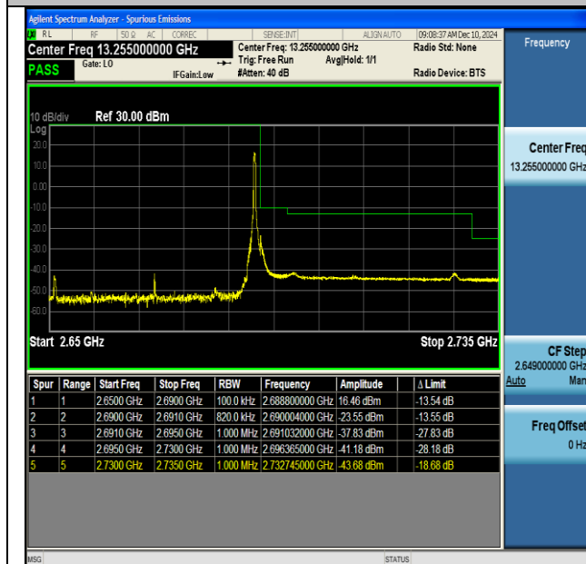
NTNV-DC_66A_n41A-PC3-30-5+40-M+H-QPSK-IDLE-CP- QPSK-Edge_1RB_Right-PASS
