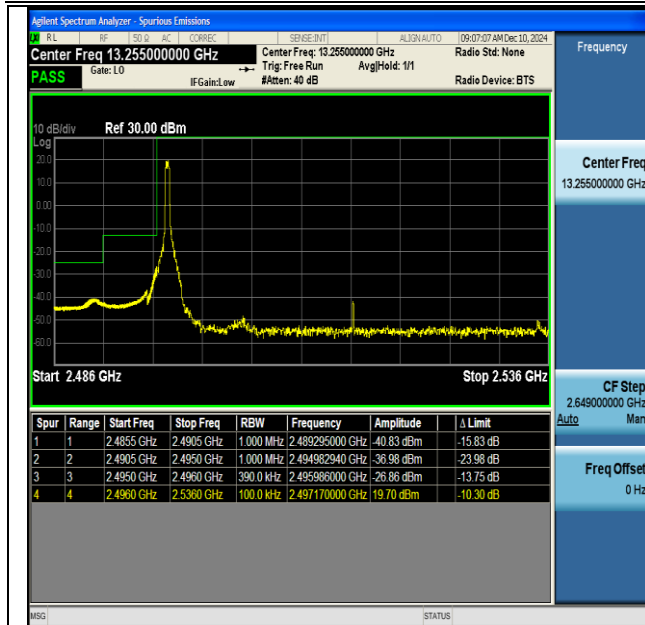
NTNV-DC_66A_n41A-PC3-30-5+40-M+L-QPSK-IDLE- DFT-BPSK-Edge_1RB_Left-PASS
