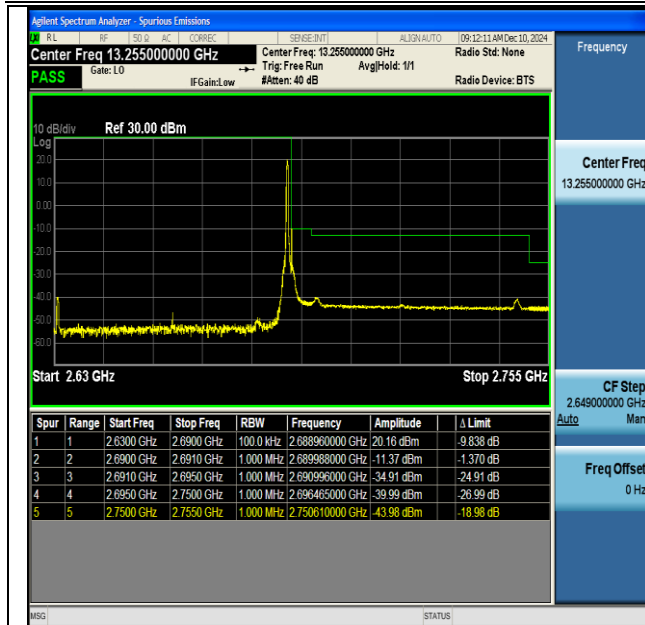
NTNV-DC_66A_n41A-PC3-30-5+60-M+H-QPSK-IDLE- DFT-BPSK-Edge_1RB_Right-PASS
