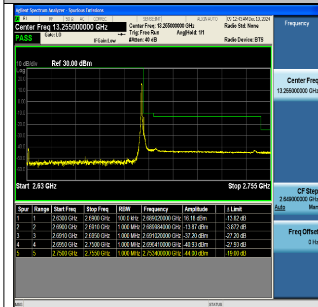
NTNV-DC_66A_n41A-PC3-30-5+60-M+H-QPSK-IDLE-CP- QPSK-Edge_1RB_Right-PASS
