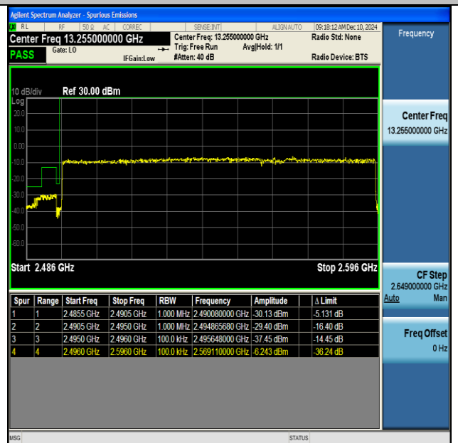
NTNV-DC_66A_n41A-PC3-30-5+100-M+L-QPSK-IDLE- CP-QPSK-Outer_Full-PASS
