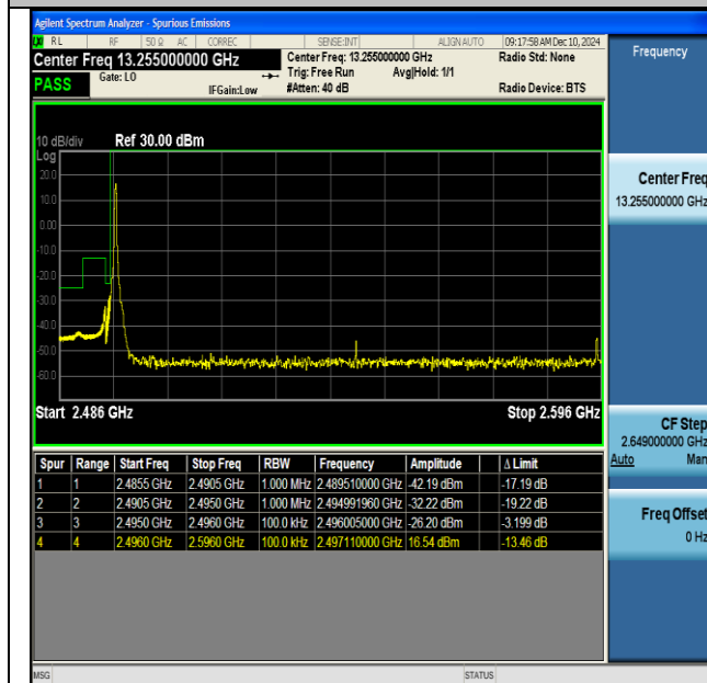
NTNV-DC_66A_n41A-PC3-30-5+100-M+L-QPSK-IDLE- CP-QPSK-Edge_1RB_Left-PASS
