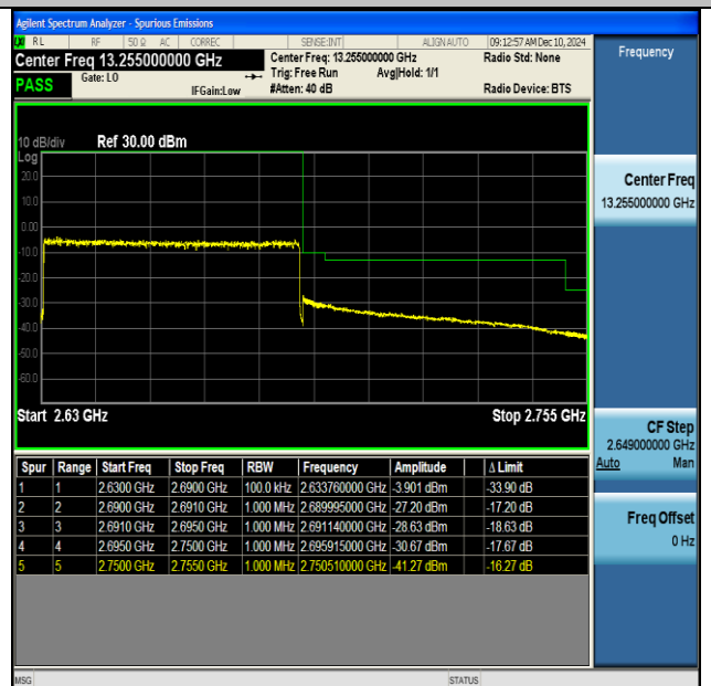
NTNV-DC_66A_n41A-PC3-30-5+60-M+H-QPSK-IDLE- CP-QPSK-Outer_Full-PASS
