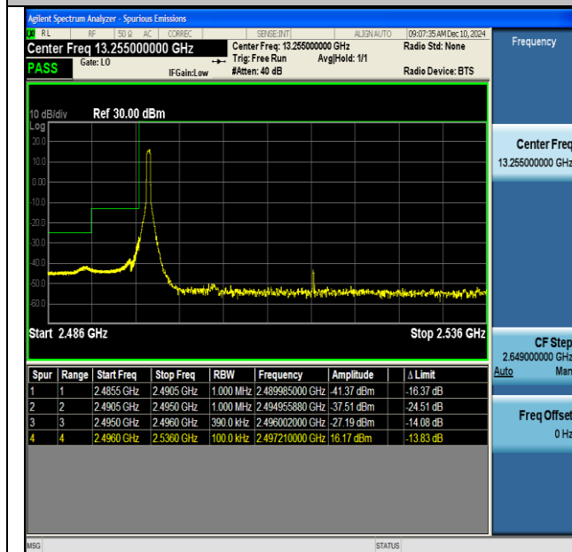
NTNV-DC_66A_n41A-PC3-30-5+40-M+L-QPSK-IDLE-CP- QPSK-Edge_1RB_Left-PASS
