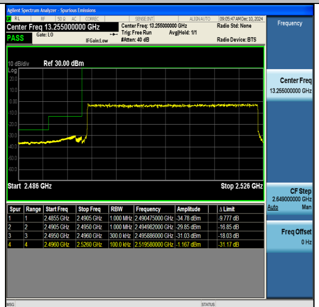
NTNV-DC_66A_n41A-PC3-30-5+30-M+L-QPSK-IDLE- CP-QPSK-Outer_Full-PASS
