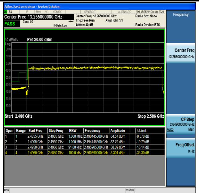
NTNV-DC_66A_n41A-PC3-30-5+90-M+L-QPSK-IDLE- DFT-BPSK-Outer_Full-PASS
