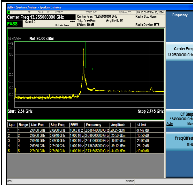
NTNV-DC_66A_n41A-PC3-30-5+50-M+H-QPSK-IDLE- DFT-BPSK-Edge_1RB_Right-PASS
