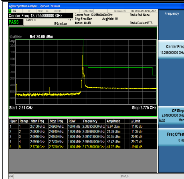
NTNV-DC_66A_n41A-PC3-30-5+80-M+H-QPSK-IDLE- DFT-BPSK-Edge_1RB_Right-PASS
