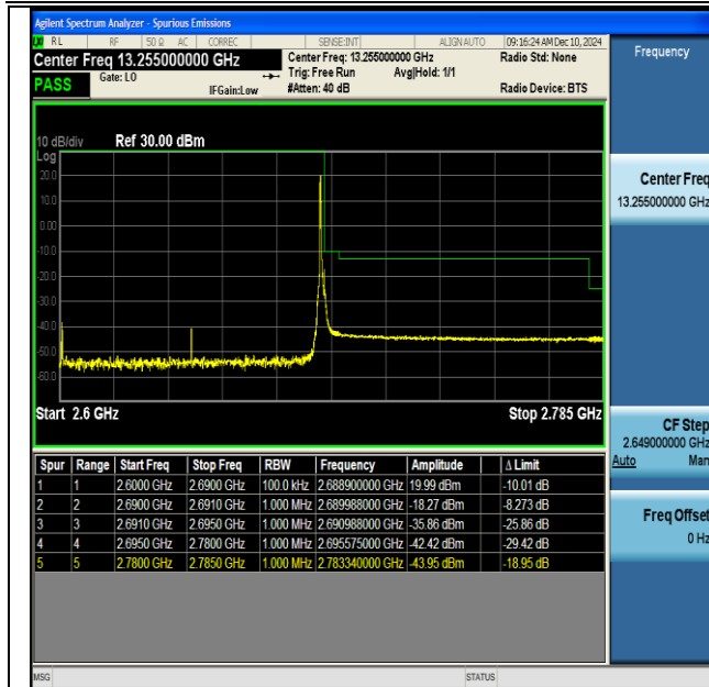
NTNV-DC_66A_n41A-PC3-30-5+90-M+H-QPSK-IDLE- DFT-BPSK-Edge_1RB_Right-PASS
