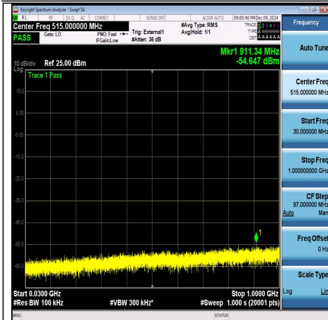
NTNV-DC_66A_n41A-PC3-30-5+100-M+L-QPSK-IDLE- CP-QPSK-Inner_1RB_Left-30-1000-PASS
