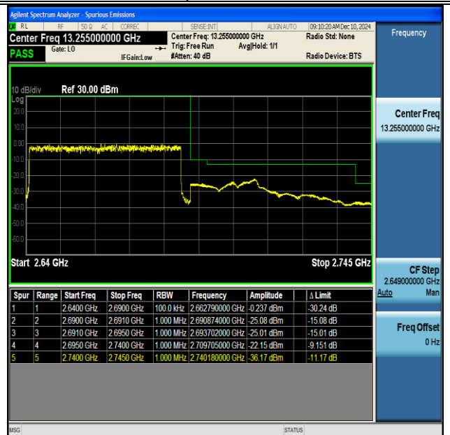
NTNV-DC_66A_n41A-PC3-30-5+50-M+H-QPSK-IDLE- DFT-BPSK-Outer_Full-PASS
