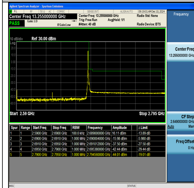
NTNV-DC_66A_n41A-PC3-30-5+100-M+H-QPSK-IDLE- CP-QPSK-Edge_1RB_Right-PASS
