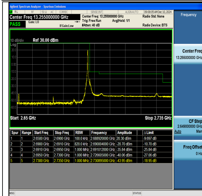
NTNV-DC_66A_n41A-PC3-30-5+40-M+H-QPSK-IDLE- DFT-BPSK-Edge_1RB_Right-PASS
