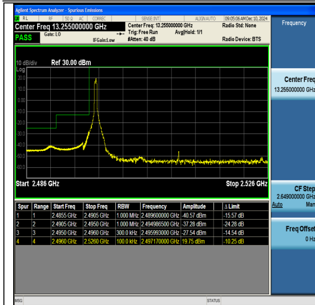
NTNV-DC_66A_n41A-PC3-30-5+30-M+L-QPSK-IDLE- DFT-BPSK-Edge_1RB_Left-PASS
