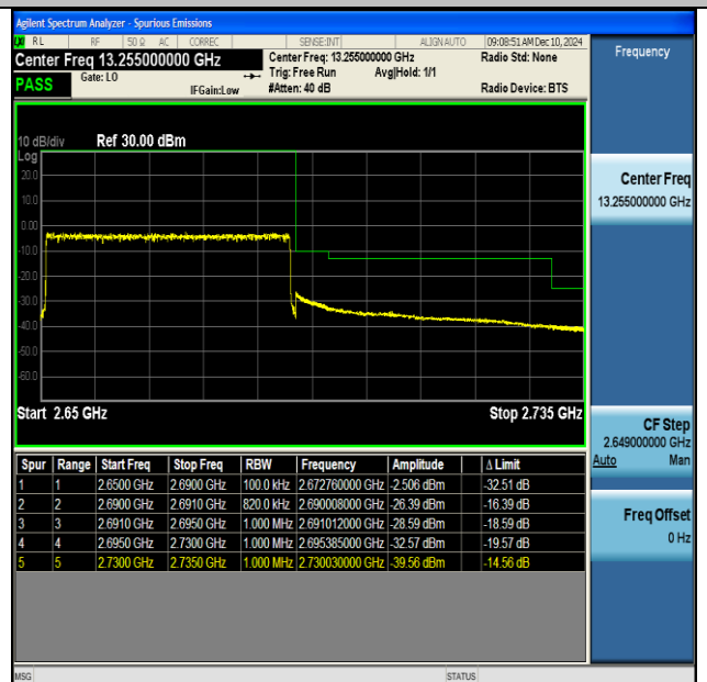
NTNV-DC_66A_n41A-PC3-30-5+40-M+H-QPSK-IDLE- CP-QPSK-Outer_Full-PASS
