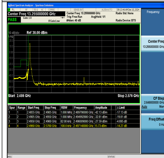
NTNV-DC_66A_n41A-PC3-30-5+80-M+L-QPSK-IDLE-CP- QPSK-Edge_1RB_Left-PASS
