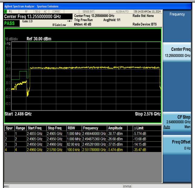
NTNV-DC_66A_n41A-PC3-30-5+80-M+L-QPSK-IDLE- CP-QPSK-Outer_Full-PASS
