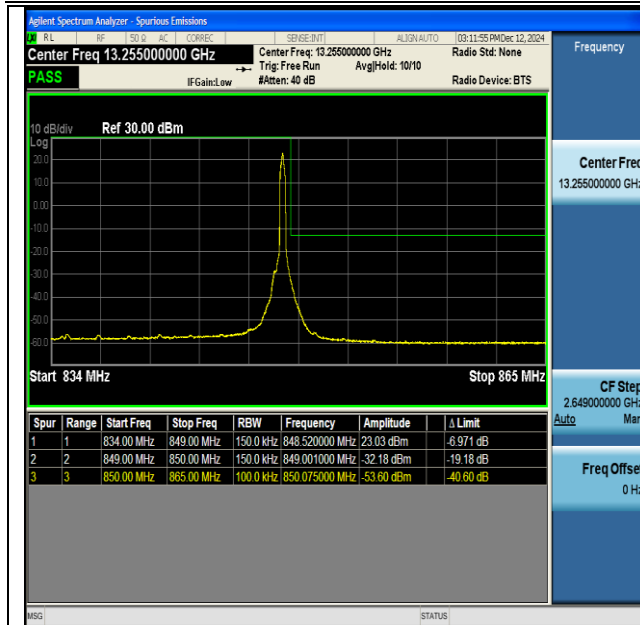
NTNV-DC_66A_n5A-PC3-15-5+15-M+H-QPSK-IDLE-DFT- BPSK-Edge_1RB_Right-PASS
