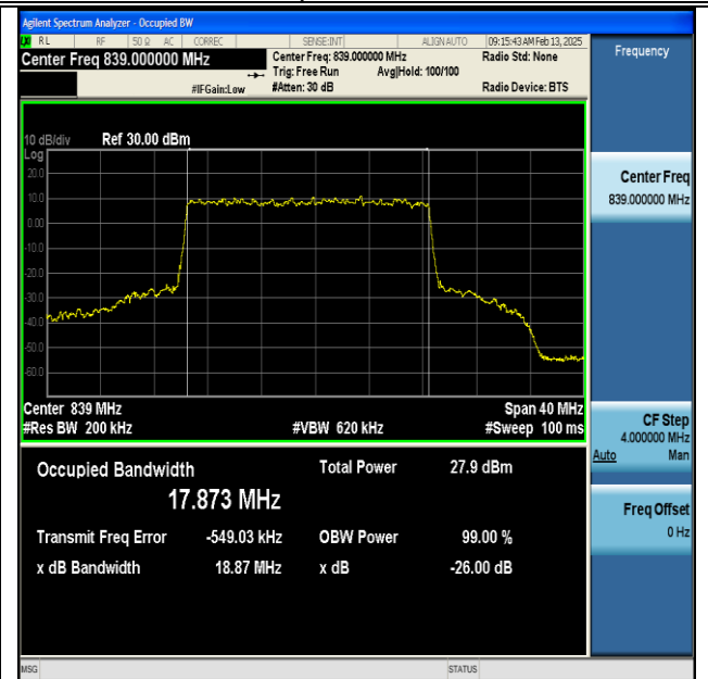
NTNV-DC_66A_n5A-PC3-15-5+20-M+H-QPSK-IDLE-DFT-16QAM-Outet_Full-Ant1-PASS
