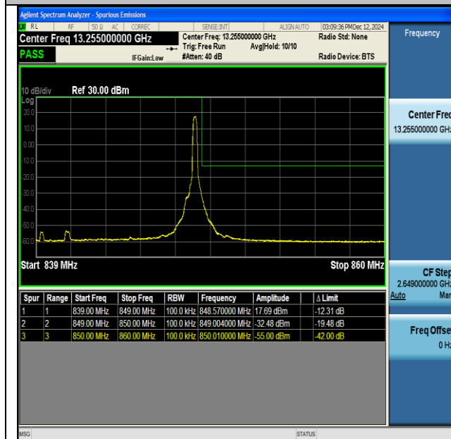
NTNV-DC_66A_n5A-PC3-15-5+10-M+H-QPSK-IDLE-CP- QPSK-Edge_1RB_Right-PASS
