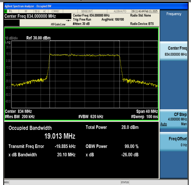
NTNV-DC_66A_n5A-PC3-15-5+20-M+L-QPSK-IDLE-CP-256QAM-Outer_Full-Ant1-PASS
