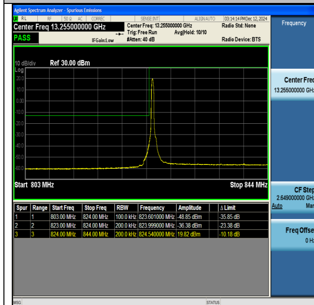
NTNV-DC_66A_n5A-PC3-15-5+20-M+L-QPSK-IDLE-CP- QPSK-Edge_1RB_Left-PASS
