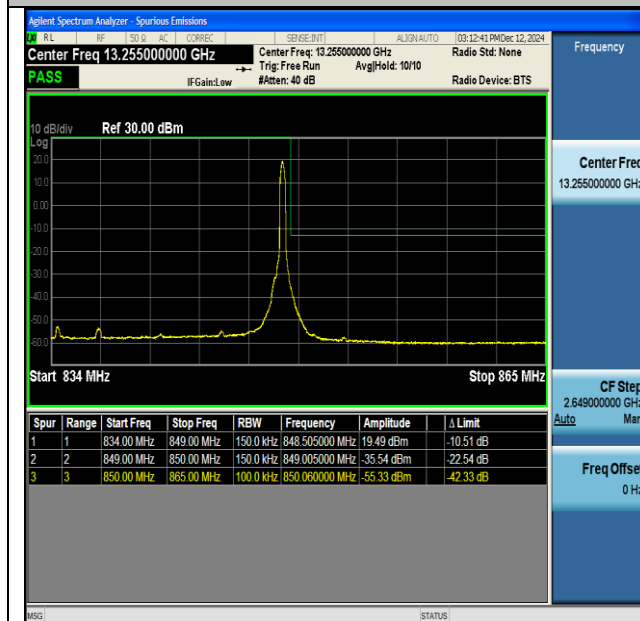
NTNV-DC_66A_n5A-PC3-15-5+15-M+H-QPSK-IDLE-CP- QPSK-Edge_1RB_Right-PASS
