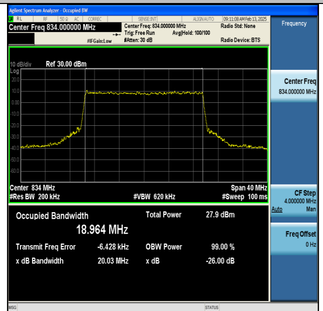
NTNV-DC_66A_n5A-PC3-15-5+20-M+L-QPSK-IDLE-CP-16QAM-Outer_Full-Ant1-PASS
