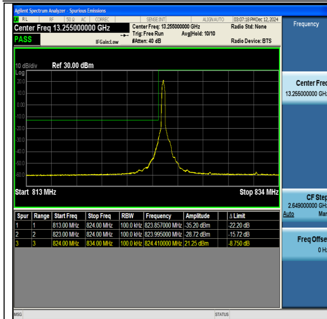
NTNV-DC_66A_n5A-PC3-15-5+10-M+L-QPSK-IDLE-DFT- BPSK-Edge_1RB_Left-PASS
