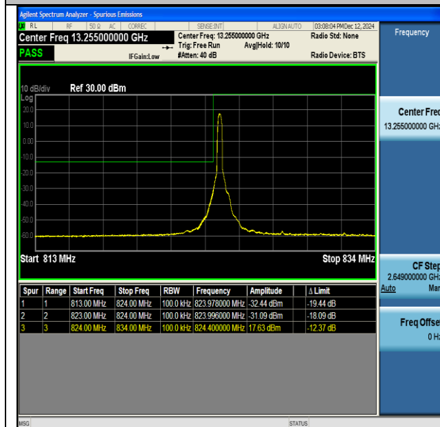
NTNV-DC_66A_n5A-PC3-15-5+10-M+L-QPSK-IDLE-CP- QPSK-Edge_1RB_Left-PASS
