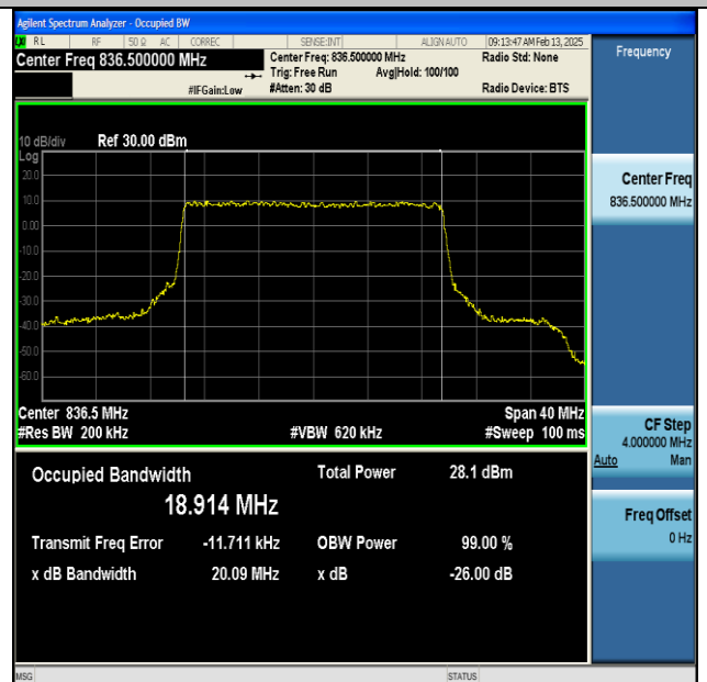
NTNV-DC_66A_n5A-PC3-15-5+20-M+M-QPSK-IDLE-CP- QPSK-Outer_Full-Ant1-PASS
