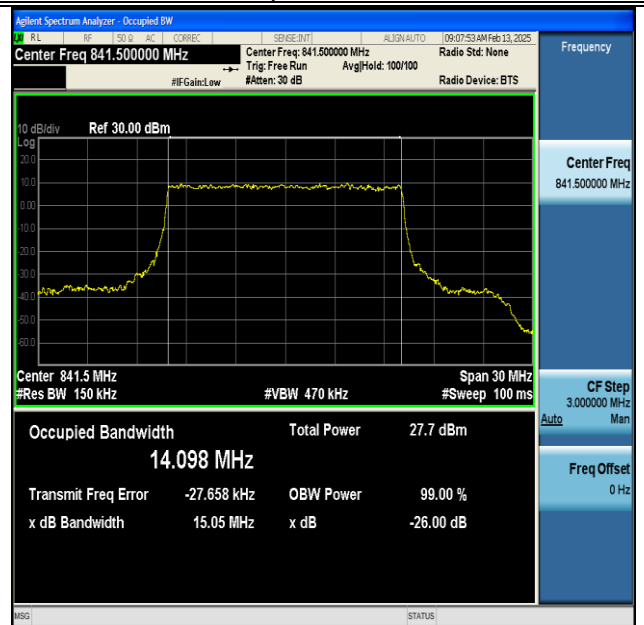
NTNV-DC_66A_n5A-PC3-15-5+15-M+H-QPSK-IDLE-CP- QPSK-Outer_Full-Ant1-PASS
