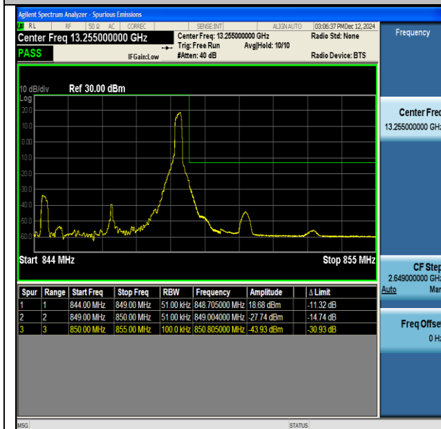
NTNV-DC_66A_n5A-PC3-15-5+5-M+H-QPSK-IDLE-CP- QPSK-Edge_1RB_Right-PASS
