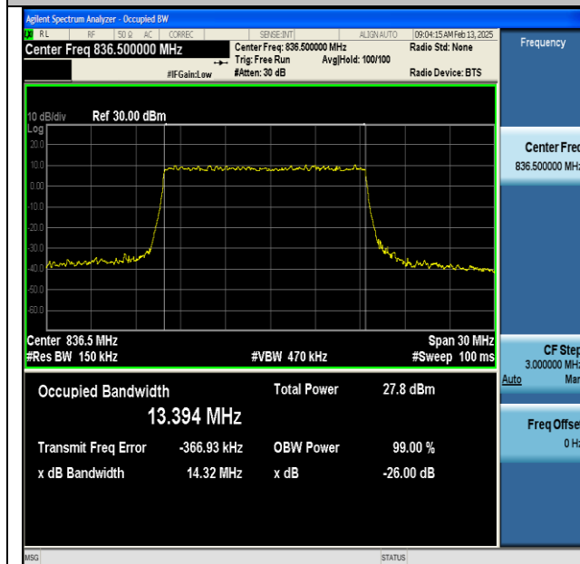
NTNV-DC_66A_n5A-PC3-15-5+15-M+M-QPSK-IDLE- DFT-64QAM-Outer_Full-Ant1-PASS
