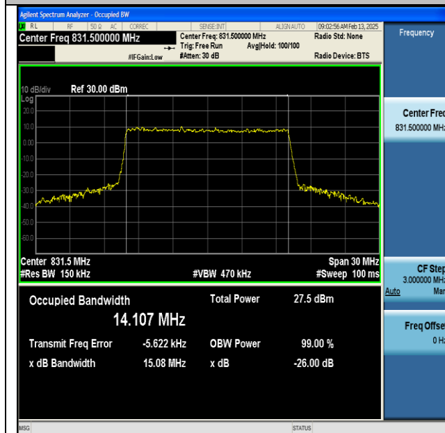
NTNV-DC_66A_n5A-PC3-15-5+15-M+L-QPSK-IDLE-CP-256QAM-Outet_Full-Ant1-PASS
