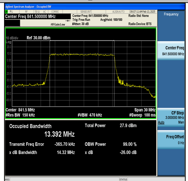
NTNV-DC_66A_n5A-PC3-15-5+15-M+H-QPSK-IDLE-DFT- 64QAM-Outer_Full-Ant1-PASS
