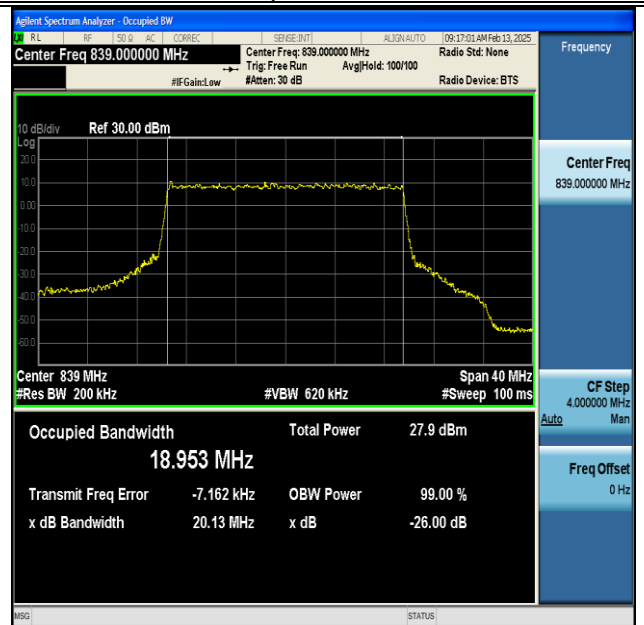
NTNV-DC_66A_n5A-PC3-15-5+20-M+H-QPSK-IDLE-CP-16QAM-Outer_Full-Ant1-PASS
