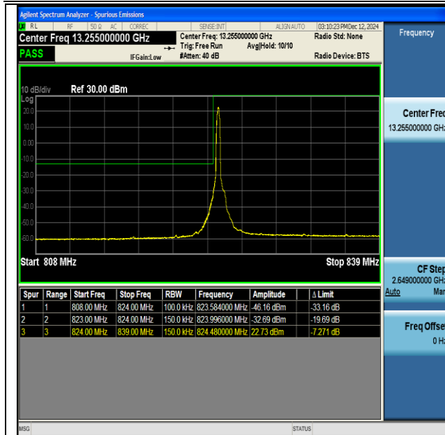
NTNV-DC_66A_n5A-PC3-15-5+15-M+L-QPSK-IDLE-DFT- BPSK-Edge_1RB_Left-PASS
