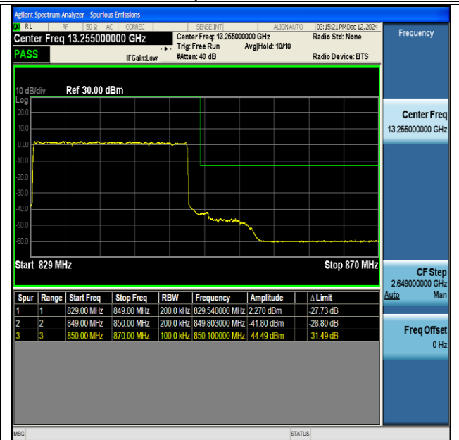
NTNV-DC_66A_n5A-PC3-15-5+20-M+H-QPSK-IDLE-DFT- BPSK-Outer_Full-PASS
