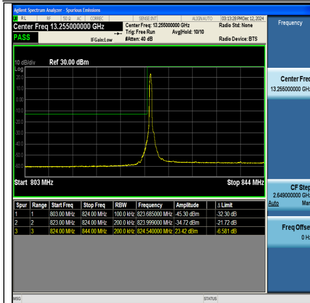
NTNV-DC_66A_n5A-PC3-15-5+20-M+L-QPSK-IDLE-DFT- BPSK-Edge_1RB_Left-PASS
