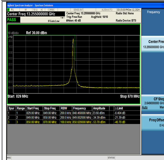
NTNV-DC_66A_n5A-PC3-15-5+20-M+H-QPSK-IDLE-DFT- BPSK-Edge_1RB_Right-PASS
