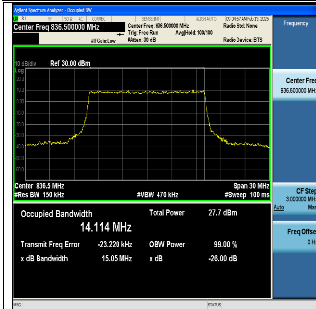
NTNV-DC_66A_n5A-PC3-15-5+15-M+M-QPSK-IDLE-CP-QPSK-Outer_Full-Ant1-PASS
