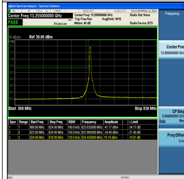
NTNV-DC_66A_n5A-PC3-15-5+15-M+L-QPSK-IDLE-CP- QPSK-Edge_1RB_Left-PASS
