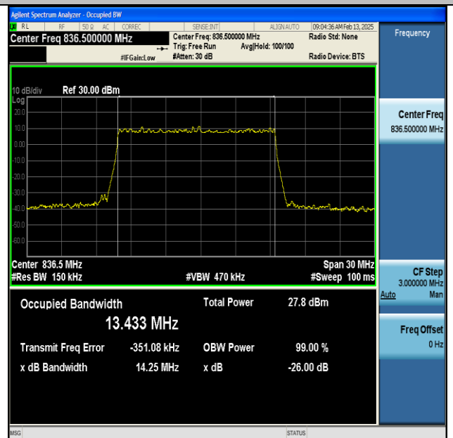
NTNV-DC_66A_n5A-PC3-15-5+15-M+M-QPSK-IDLE- DFT-256QAM-Outer_Full-Ant1-PASS
