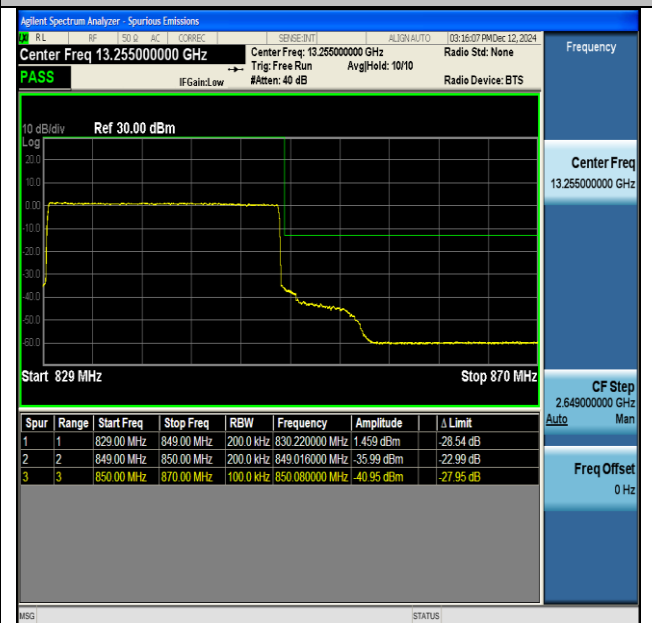
NTNV-DC_66A_n5A-PC3-15-5+20-M+H-QPSK-IDLE-CP- QPSK-Outer_Full-PASS
