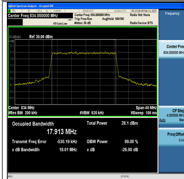
NTNV-DC_66A_n5A-PC3-15-5+20-M+L-QPSK-IDLE-DFT-64QAM-Outer_Full-Ant1-PASS
