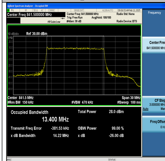
NTNV-DC_66A_n5A-PC3-15-5+15-M+H-QPSK-IDLE-DFT- 16QAM-Outer_Full-Ant1-PASS
