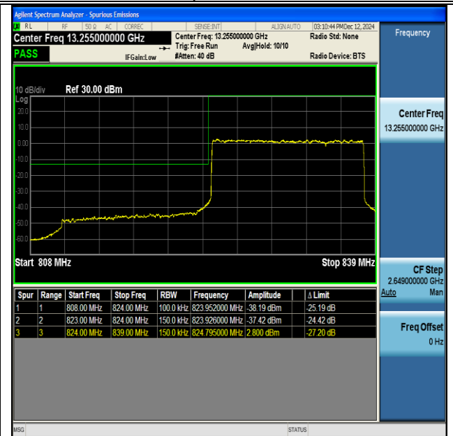
NTNV-DC_66A_n5A-PC3-15-5+15-M+L-QPSK-IDLE-DFT- BPSK-Outer_Full-PASS
