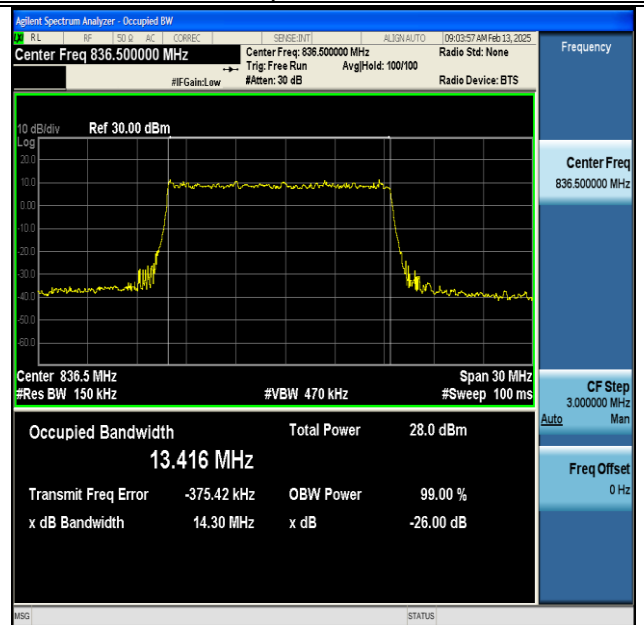
NTNV-DC_66A_n5A-PC3-15-5+15-M+M-QPSK-IDLE- DFT-16QAM-Outer_Full-Ant1-PASS
