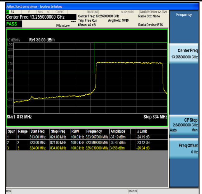
NTNV-DC_66A_n5A-PC3-15-5+10-M+L-QPSK-IDLE-DFT- BPSK-Outer_Full-PASS
