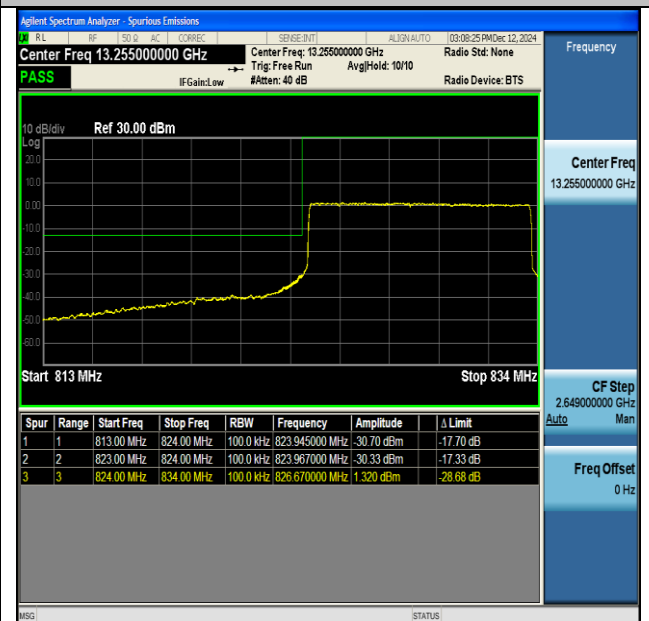
NTNV-DC_66A_n5A-PC3-15-5+10-M+L-QPSK-IDLE-CP- QPSK-Outer_Full-PASS
