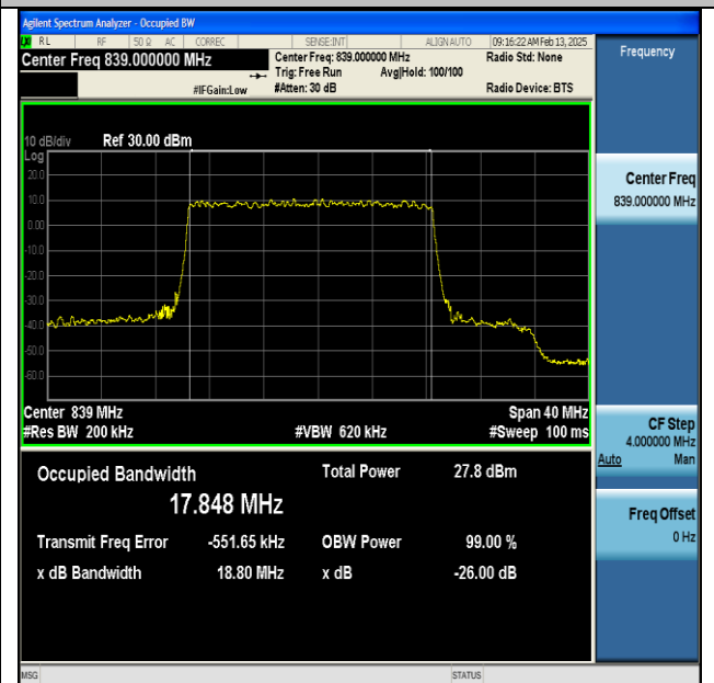
NTNV-DC_66A_n5A-PC3-15-5+20-M+H-QPSK-IDLE-DFT-256QAM-Outet_Full-Ant1-PASS
