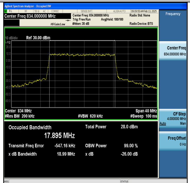
NTNV-DC_66A_n5A-PC3-15-5+20-M+L-QPSK-IDLE-DFT- 16QAM-Outer_Full-Ant1-PASS
