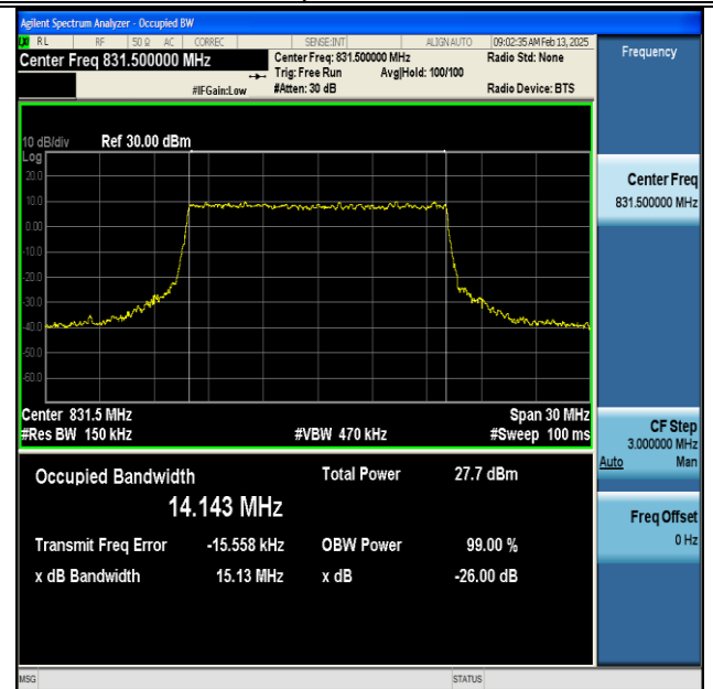
NTNV-DC_66A_n5A-PC3-15-5+15-M+L-QPSK-IDLE-CP-64QAM-Outet_Full-Ant1-PASS
