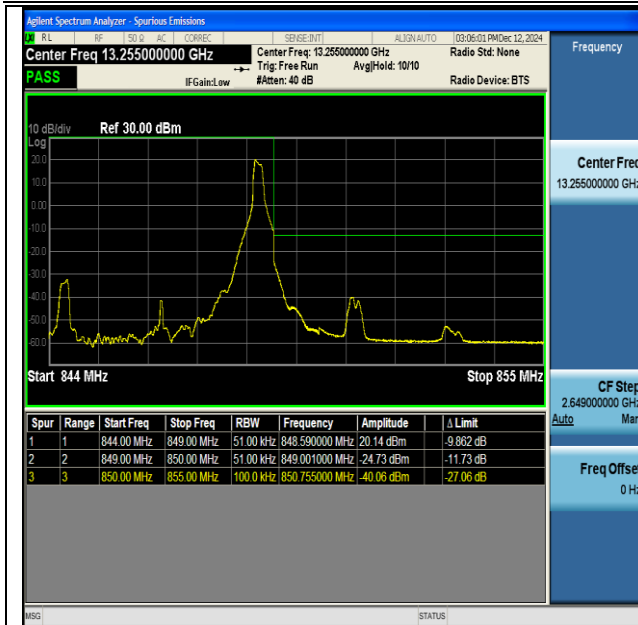
NTNV-DC_66A_n5A-PC3-15-5+5-M+H-QPSK-IDLE-DFT- BPSK-Edge_1RB_Right-PASS
