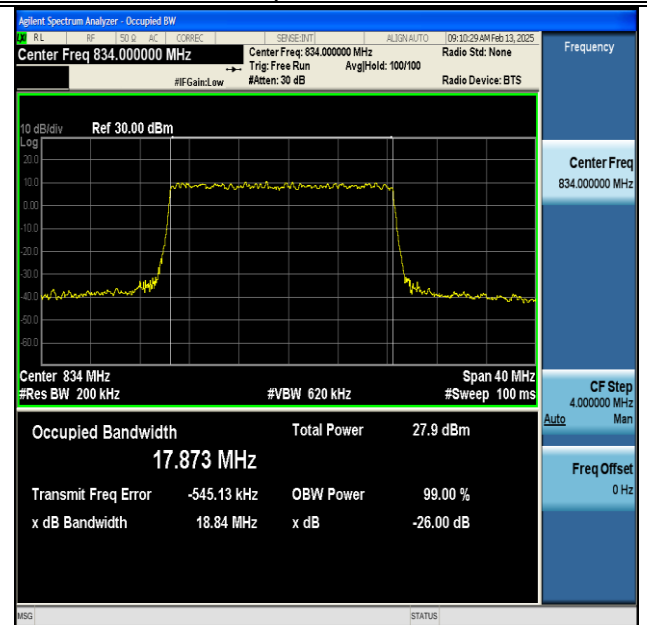
NTNV-DC_66A_n5A-PC3-15-5+20-M+L-QPSK-IDLE-DFT-256QAM-Outer_Full-Ant1-PASS
