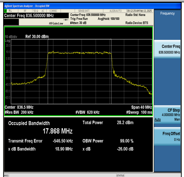
NTNV-DC_66A_n5A-PC3-15-5+20-M+M-QPSK-IDLE-DFT-QPSK-Outer_Full-Ant1-PASS
