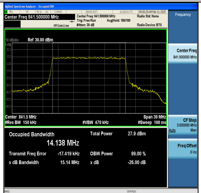
NTNV-DC_66A_n5A-PC3-15-5+15-M+H-QPSK-IDLE-CP- 64QAM-Outer_Full-Ant1-PASS
