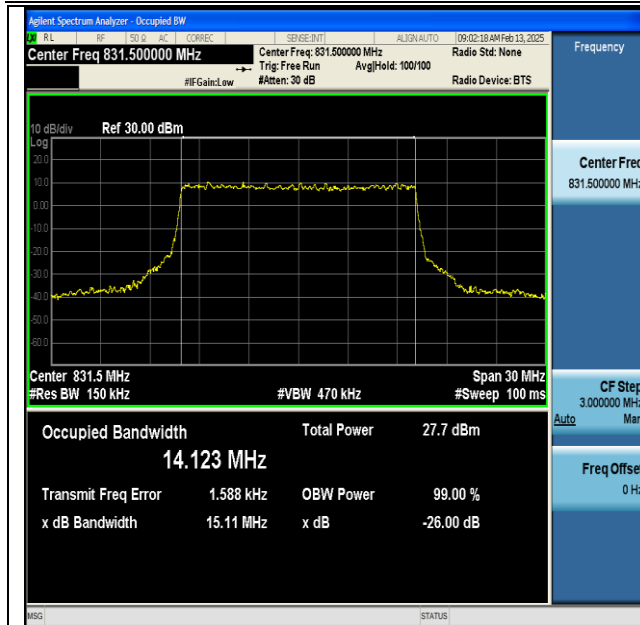
NTNV-DC_66A_n5A-PC3-15-5+15-M+L-QPSK-IDLE-CP-16QAM-Outet_Full-Ant1-PASS
