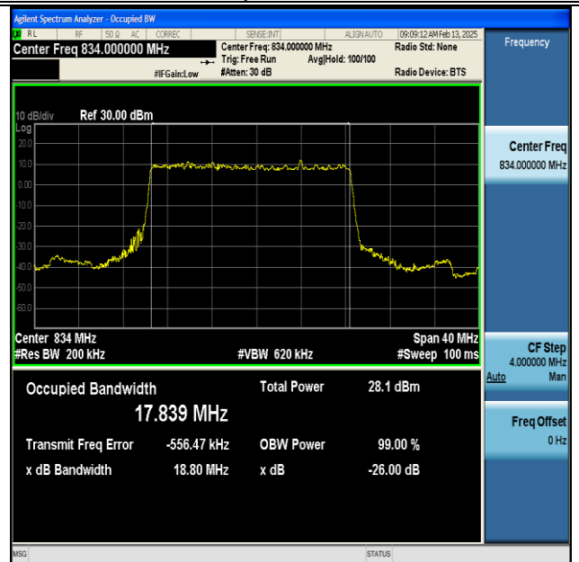
NTNV-DC_66A_n5A-PC3-15-5+20-M+L-QPSK-IDLE-DFT- BPSK-Outer_Full-Ant1-PASS
