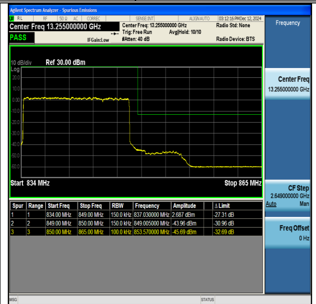
NTNV-DC_66A_n5A-PC3-15-5+15-M+H-QPSK-IDLE-DFT- BPSK-Outer_Full-PASS
