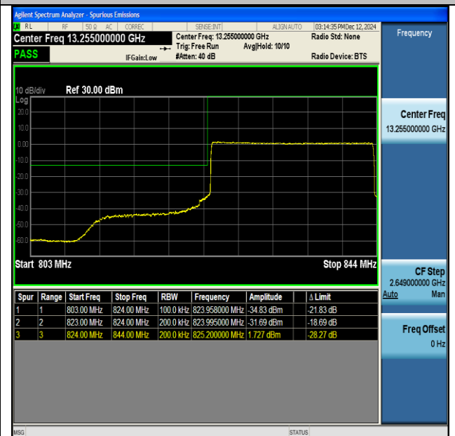
NTNV-DC_66A_n5A-PC3-15-5+20-M+L-QPSK-IDLE-CP- QPSK-Outer_Full-PASS
