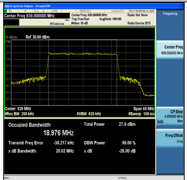
NTNV-DC_66A_n5A-PC3-15-5+20-M+H-QPSK-IDLE-CP-256QAM-Outer_Full-Ant1-PASS
