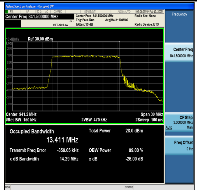
NTNV-DC_66A_n5A-PC3-15-5+15-M+H-QPSK-IDLE-DFT- QPSK-Outer_Full-Ant1-PASS
