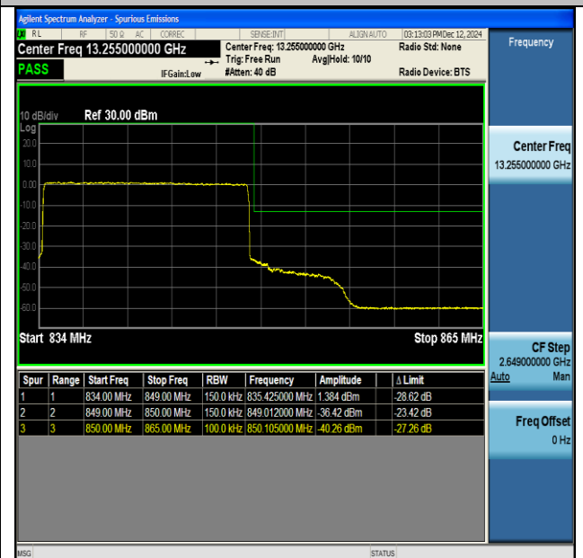
NTNV-DC_66A_n5A-PC3-15-5+15-M+H-QPSK-IDLE-CP- QPSK-Outer_Full-PASS
