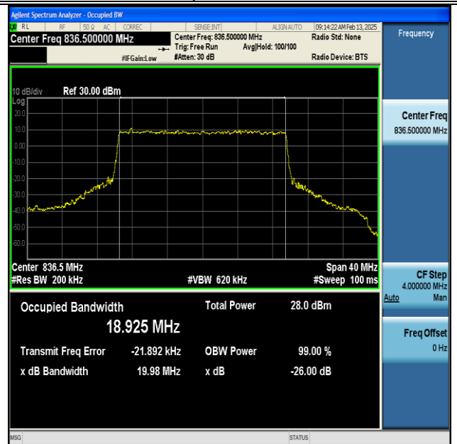
NTNV-DC_66A_n5A-PC3-15-5+20-M+M-QPSK-IDLE-CP-64QAM-Outet_Full-Ant1-PASS
