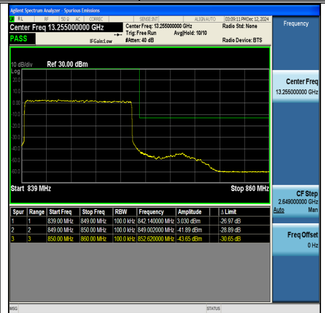
NTNV-DC_66A_n5A-PC3-15-5+10-M+H-QPSK-IDLE-DFT- BPSK-Outer_Full-PASS
