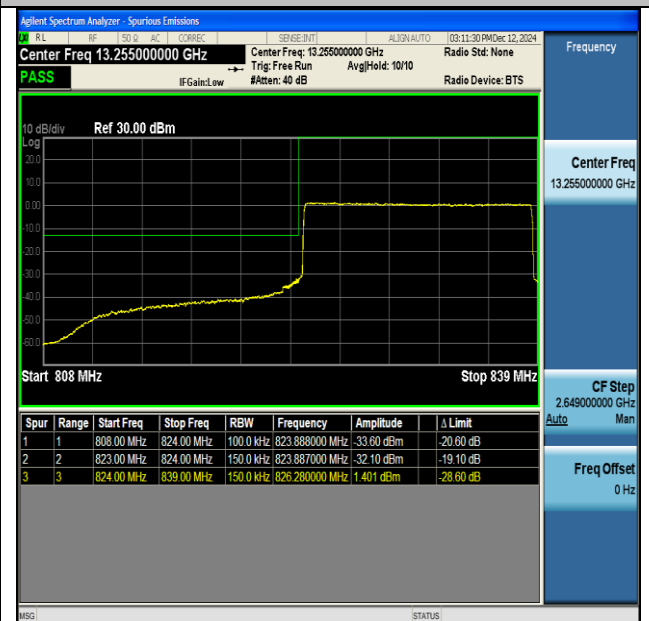
NTNV-DC_66A_n5A-PC3-15-5+15-M+L-QPSK-IDLE-CP- QPSK-Outer_Full-PASS
