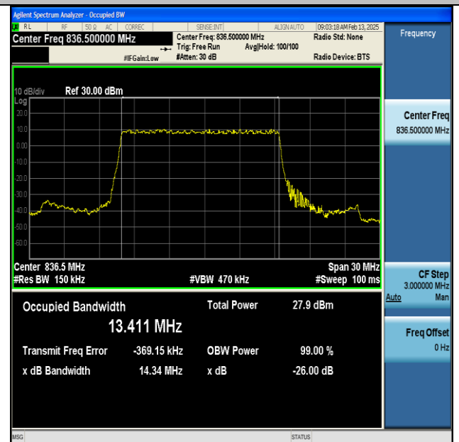
NTNV-DC_66A_n5A-PC3-15-5+15-M+M-QPSK-IDLE-DFT-BPSK-Outet_Full-Ant1-PASS
