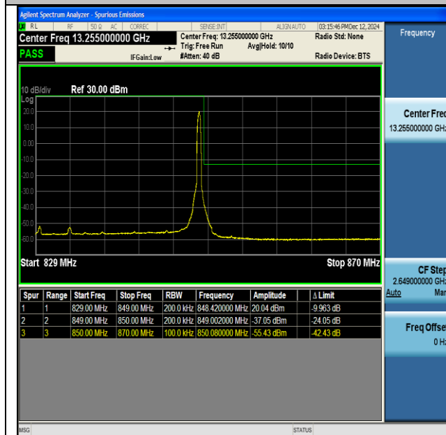
NTNV-DC_66A_n5A-PC3-15-5+20-M+H-QPSK-IDLE-CP- QPSK-Edge_1RB_Right-PASS
