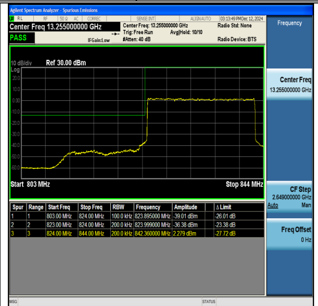
NTNV-DC_66A_n5A-PC3-15-5+20-M+L-QPSK-IDLE-DFT- BPSK-Outer_Full-PASS
