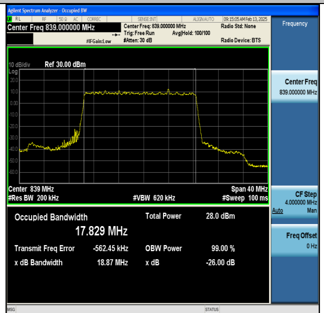
NTNV-DC_66A_n5A-PC3-15-5+20-M+H-QPSK-IDLE-DFT-BPSK-Outet_Full-Ant1-PASS
