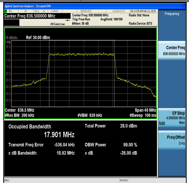
NTNV-DC_66A_n5A-PC3-15-5+20-M+M-QPSK-IDLE- DFT-64QAM-Outer_Full-Ant1-PASS
