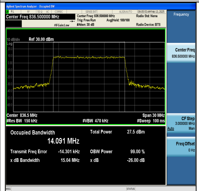
NTNV-DC_66A_n5A-PC3-15-5+15-M+M-QPSK-IDLE-CP-256QAM-Outer_Full-Ant1-PASS
