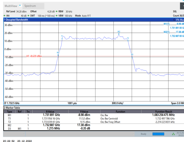
Band4-1.4MHz-QPSK-20175-6RB#0
