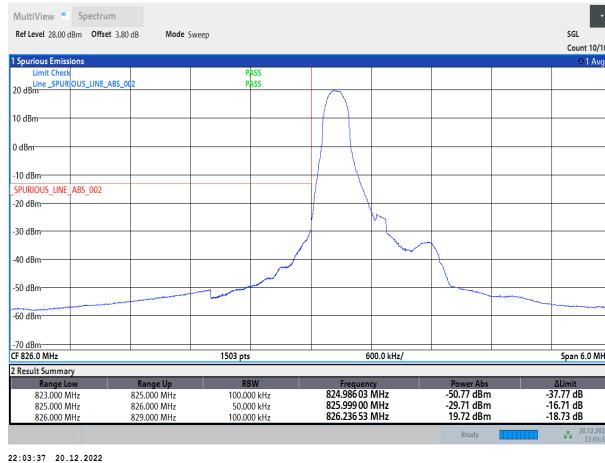
Band5-1.4MHz-QPSK-20427-6RB#0
