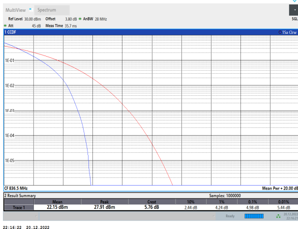
Band5-10MHz-QPSK-20525-50RB#0
