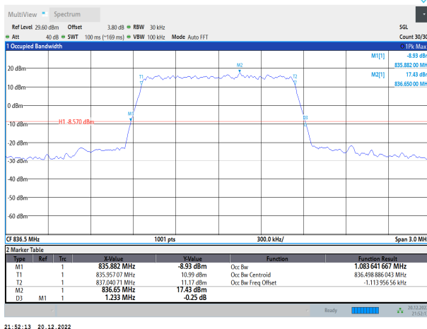
Band5-1.4MHz-QPSK-20525-6RB#0
