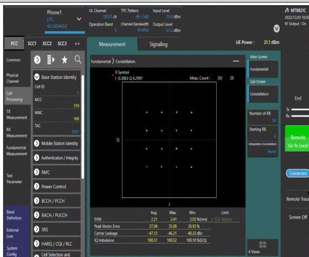
Band5-10MHz-16QAM-20525-50RB#0
