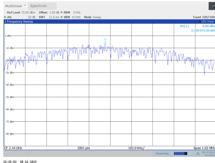
BLE_1M_Ant6_2440
