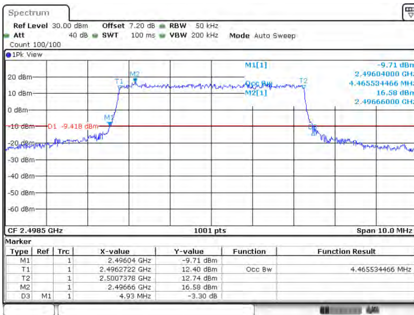
Band41-5MHz-QPSK-39675-25RB#0-4.466
