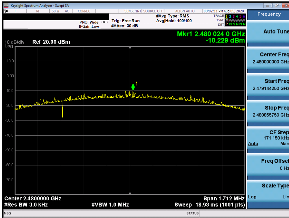
Plot 7-18. Power Spectral Density Plot (Bluetooth (LE), 1Mbps - Ch. 39)
