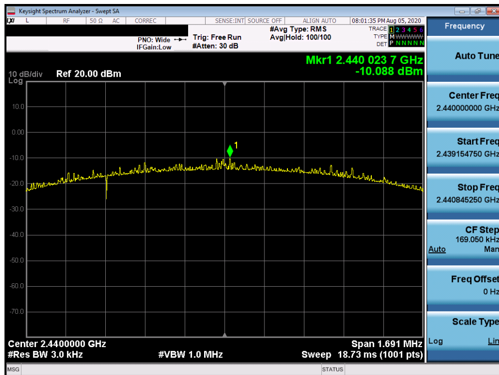
Plot 7-17. Power Spectral Density Plot (Bluetooth (LE), 1Mbps – Ch. 19)
