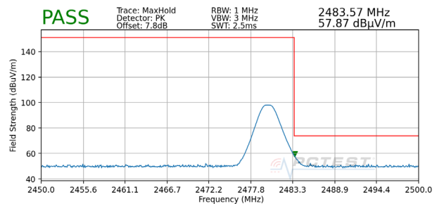
Plot 7-30. Radiated Restricted Upper Band Edge Measurement (Peak)
