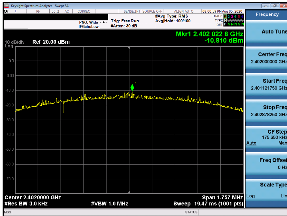
Plot 7-16. Power Spectral Density Plot (Bluetooth (LE), 1Mbps – Ch. 0)
