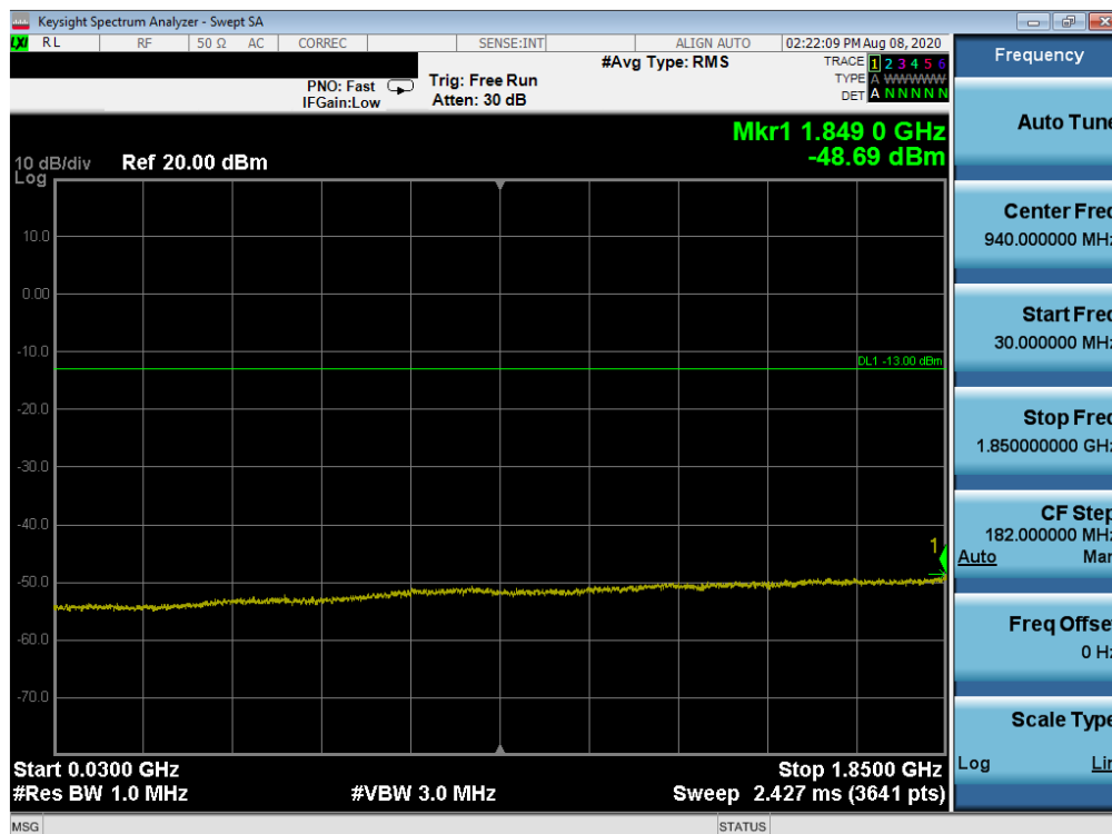
Plot 7-41. Conducted Spurious Plot (LTE Band 25/2 - 20MHz QPSK - RB Size 1, RB Offset 0 - Mid Channel)
