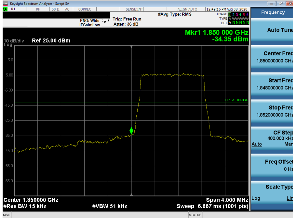
Plot 7-86. Lower Band Edge Plot (LTE Band 25/2 – 1.4MHz QPSK – Full RB Configuration)
