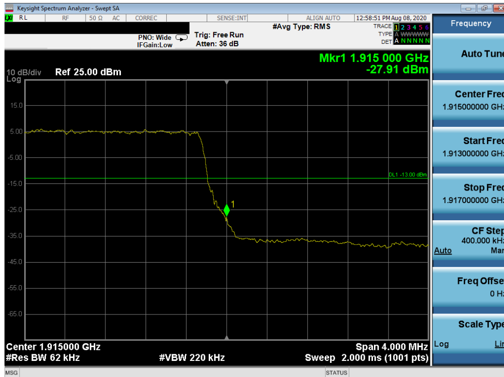
Plot 7-78. Upper Band Edge Plot (LTE Band 25 - 5MHz QPSK – Full RB Configuration)
