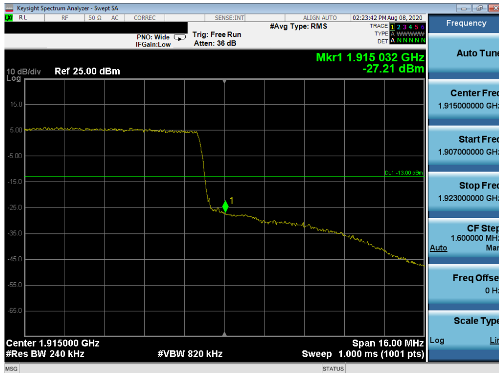
Plot 7-60. Upper Band Edge Plot (LTE Band 25 - 20MHz QPSK – Full RB Configuration)
