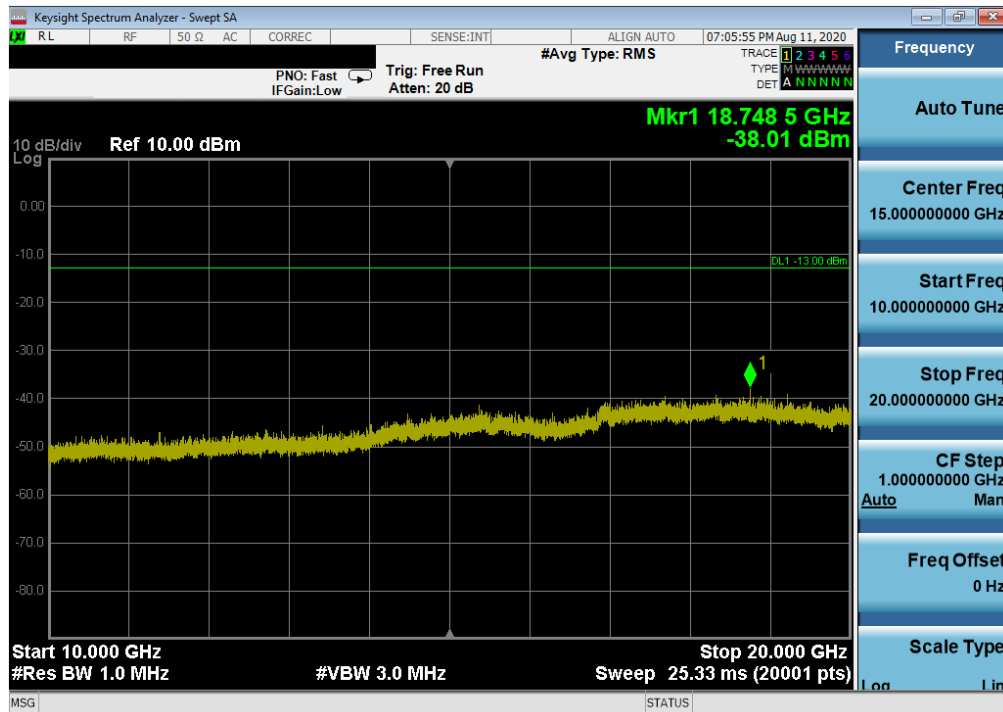
Plot 7-31. Conducted Spurious Plot (GPRS Ch. 810)
