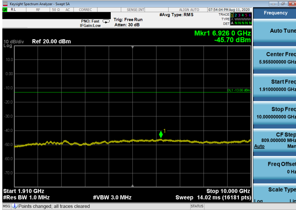
Plot 7-31. Conducted Spurious Plot (WCDMA Ch. 9400)
