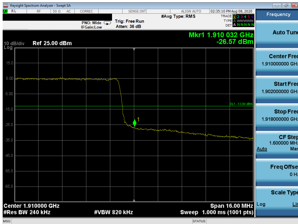
Plot 7-58. Upper Band Edge Plot (LTE Band 2 - 20MHz QPSK – Full RB Configuration)
