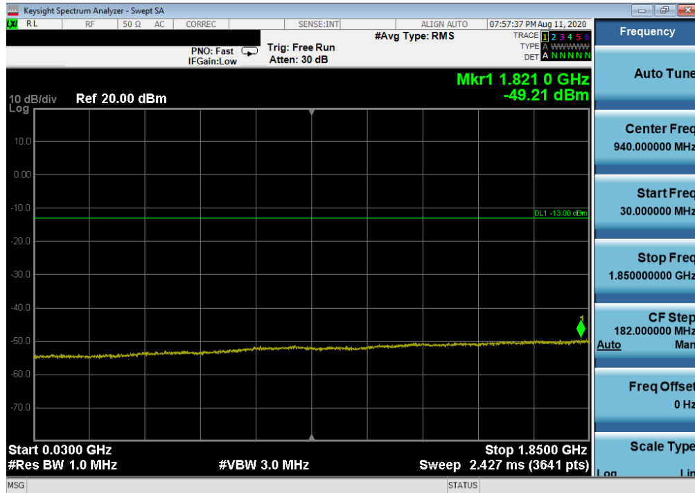
Plot 7-31. Conducted Spurious Plot (WCDMA Ch. 9538)
