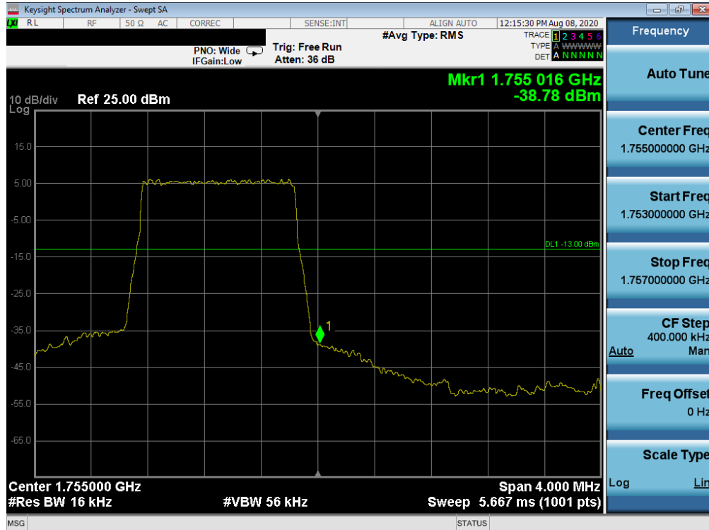
Plot 7-108. Upper Band Edge Plot (LTE Band 4 – 1.4MHz QPSK – Full RB Configuration)
