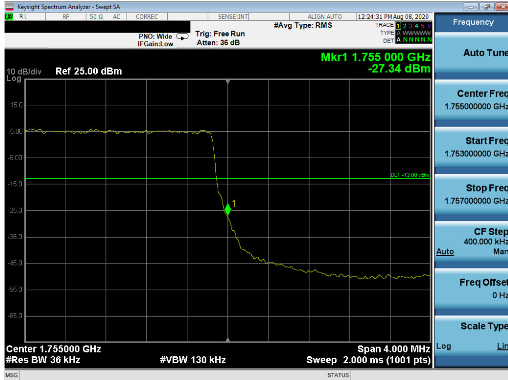
Plot 7-102. Upper Band Edge Plot (LTE Band 4 - 3MHz QPSK – Full RB Configuration)
