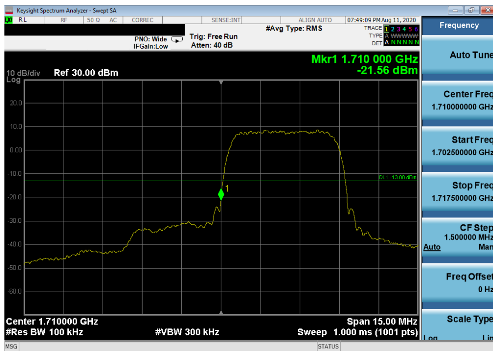
Plot 7-72. Lower Band Edge Plot (WCDMA AWS – Ch. 1312)
