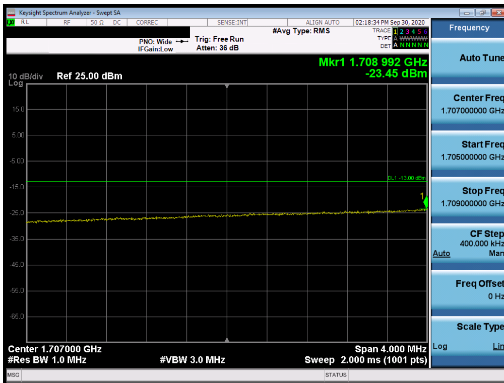
Plot 7-83. Lower Extended Band Edge Plot (LTE Band 66/4 - 15MHz QPSK – Full RB Configuration)
