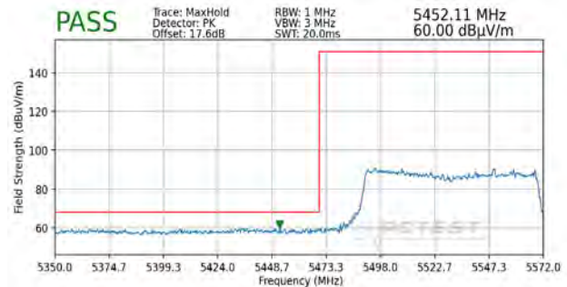
Plot 7-323. Radiated Lower Band Edge Plot SISO ANT2 (Peak - UNII Band 2C)
