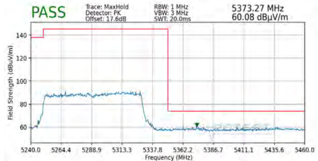
Plot 7-321. Radiated Upper Band Edge Plot SISO ANT2 (Peak – UNII Band 2A)
