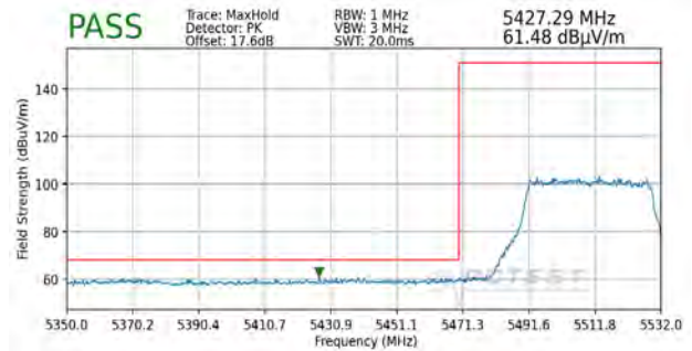
Plot 7-337. Radiated Lower Band Edge Plot MIMO (Peak – UNII Band 2C)
