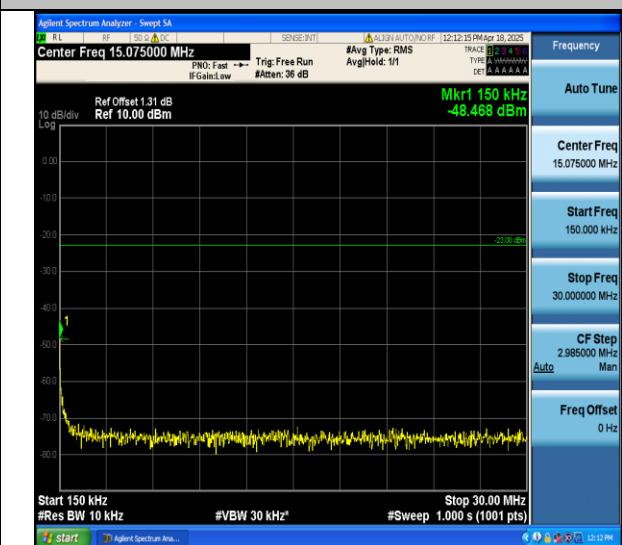
Band V-4233-0.15~30MHz-PASS
