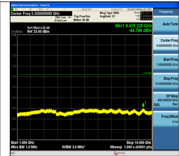
Band V-4182-1000~10000MHz-PASS
