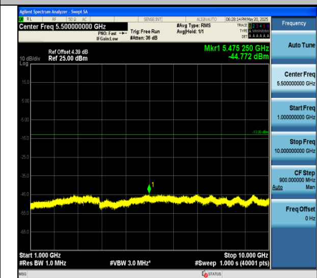
Band V-4233-1000~10000MHz-PASS
