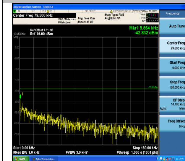
Band V-4233-0.009~0.15MHz-PASS
