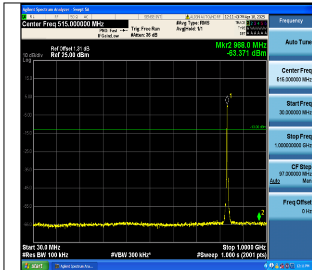
Band V-4182-30~1000MHz-PASS
