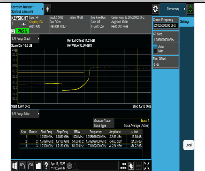
Band4-5MHz-QPSK-19975-25RB#0-PASS
