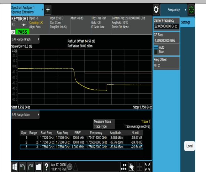
Band4-10MHz-QPSK-20350-50RB#0-PASS
