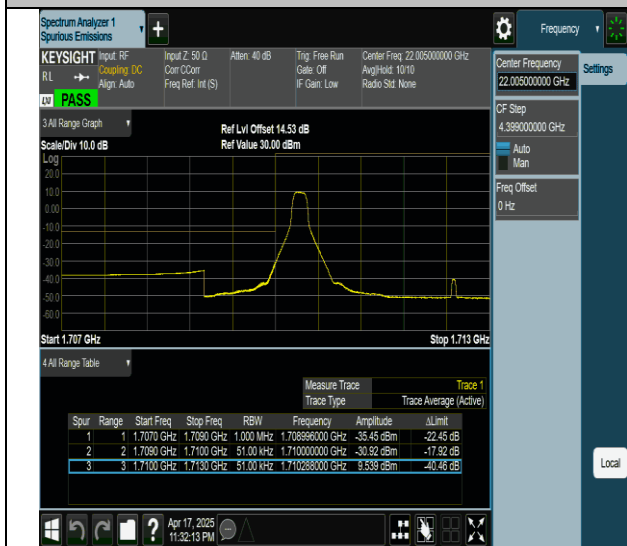
Band4-5MHz-QPSK-19975-1RB#0-PASS
